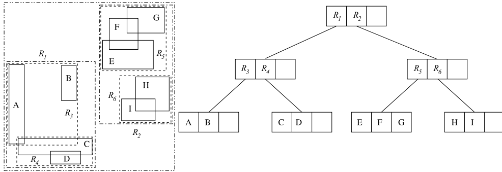
R-Trees, Figure 1
