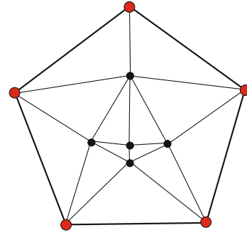
Dilation of Geometric Networks, Figure 3 The best known embedding for S_5
