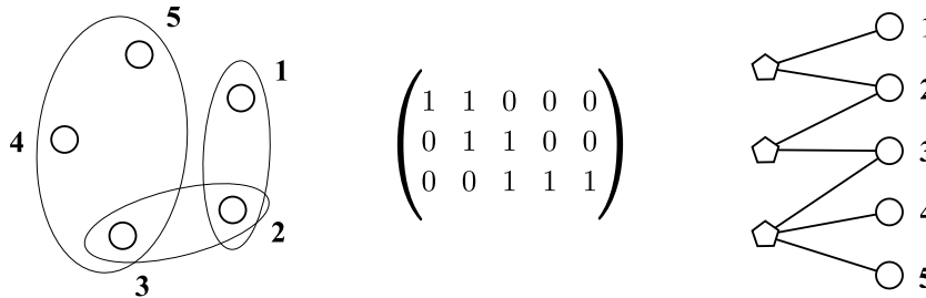
Graph Isomorphism, Figure 3
