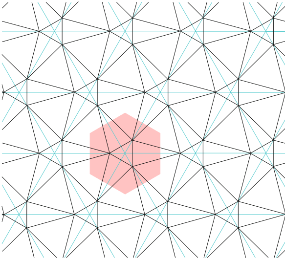
Dilation of Geometric Networks, Figure 2 A network of dilation \sim 1.1247
