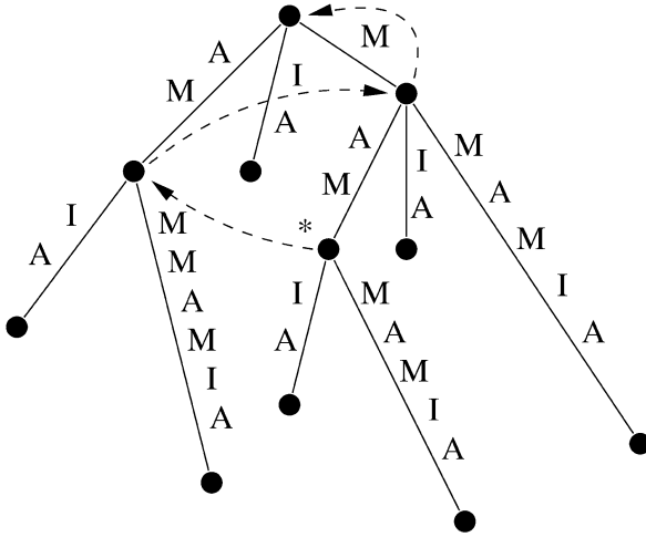
Suffix Tree Construction in RAM, Figure 1 The suffix tree for the string S = MAMMAMIA . Dashed arrows denote suffix links that are employed by all efficient suffix tree construction algorithms
