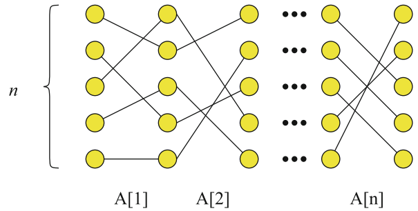
Lower Bounds for Dynamic Connectivity, Figure 1 Constructing an instance of dynamic connectivity that mimics the partial-sums problem
