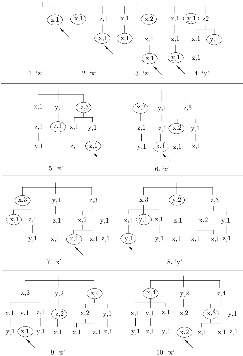
Figure 2.74: Ten Tries of "zxzyzxyzx".
