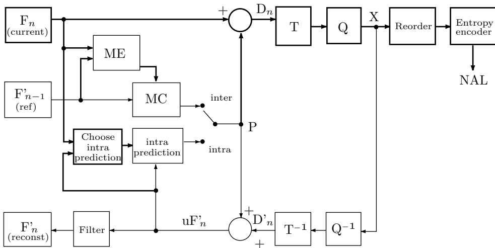
Figure 6.40: H.264 Encoder.
