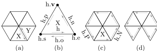
Figure 8.44: Manipulating Half-Edges.
