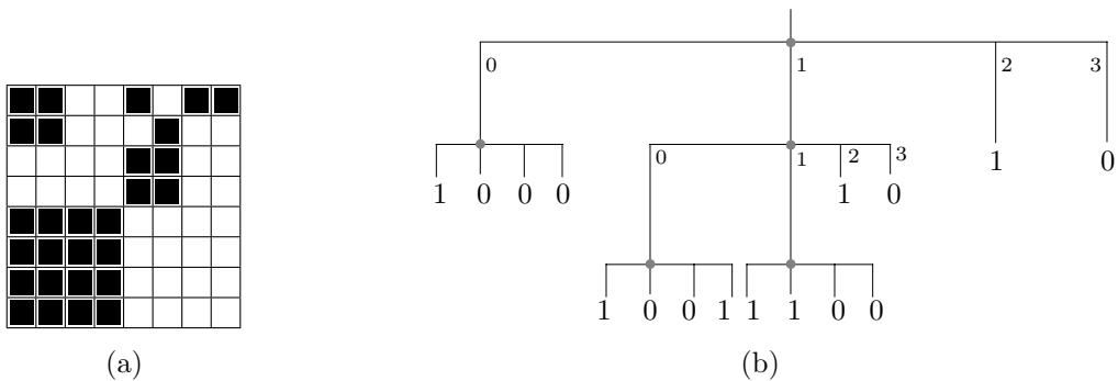
Figure 4.148: A Quadtree.
