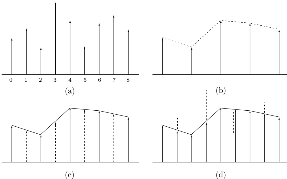
Figure 5.48: Linear Prediction.
