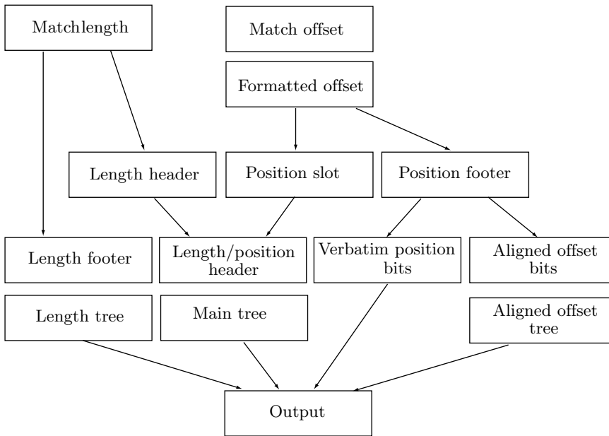
Figure 3.9: LZ78 Processing of Offsets and Lengths.
