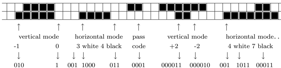
Figure Ans.14: Two-Dimensional Coding Example.
