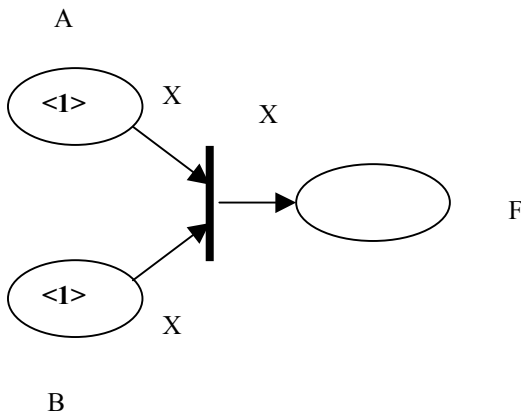
Fig. 22.13: A Petri net representing AND-Parallelism.
