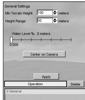
Figure 12.15 Terraform Editor.
