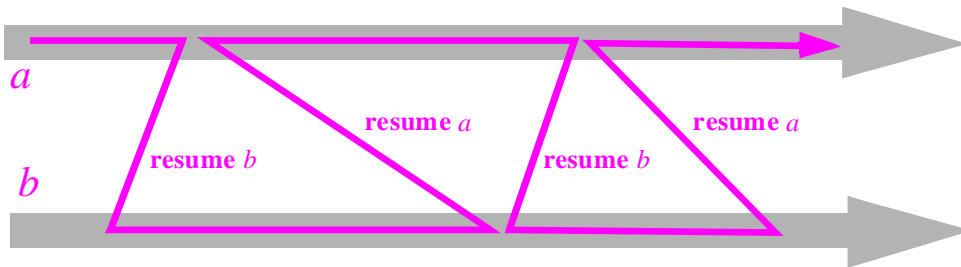
Coroutine sequencing
