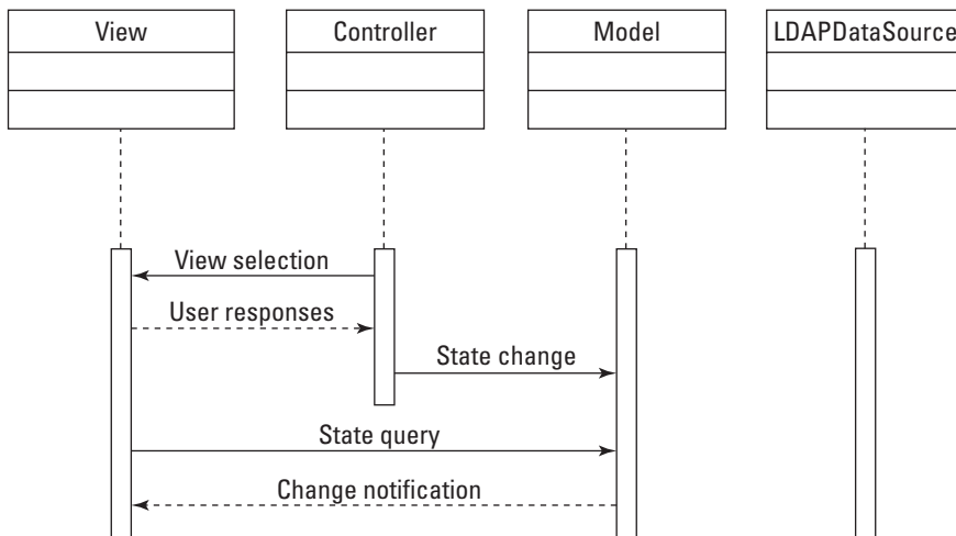
Figure 23-10: Sequence diagram for the MVC pattern
