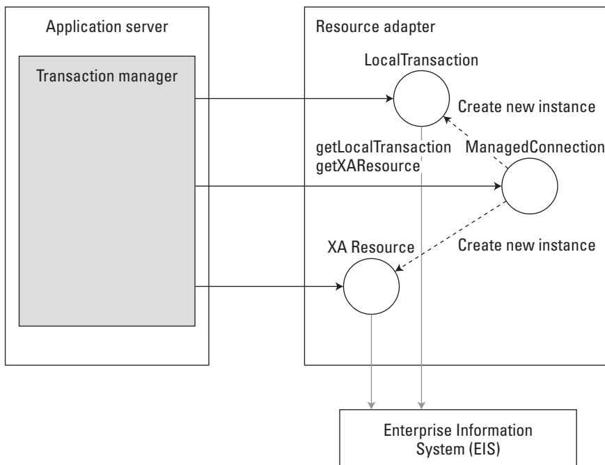
Figure 19-6: Transaction-management interfaces
