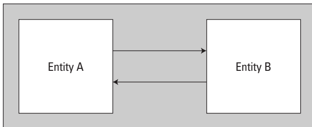
Figure 16-5: Bidirectional relationship
