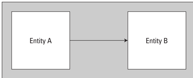
Figure 16-4: Unidirectional relationship
