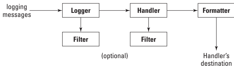
Figure 28-2: Logging architecture
