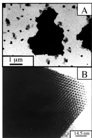
Fig. 22.3. TEM images obtained during deposition of a very concentrated solution of silver sulfide nanocrystals ( 6 \times 10^{18} particles/ml). (A) A large number of 3D \text{Ag}_2\text{S} nanoparticles. (B) High-magnification observation of one crystal [19]
