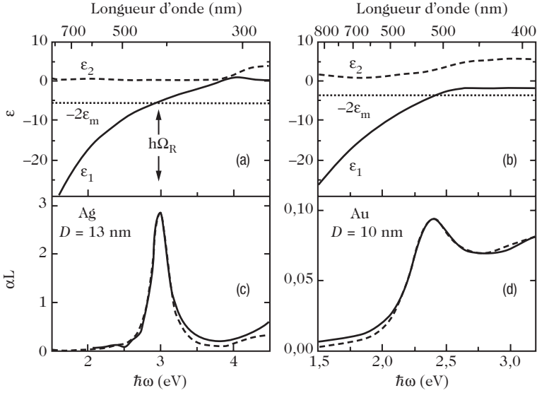
Fig. 7.4. (a) Dispersion of the real and imaginary parts of the dielectric constant for silver and for the glass Ba0–P 2 O 5 , \varepsilon_m \approx 2.75 . (b) Dispersion of the dielectric constant for gold and for water \varepsilon_m \approx 1.77 . (c) and (d) Measured ( continuous curves ) and calculated ( dotted curves ) absorption spectra for silver nanoparticles ( D = 13 nm) dispersed in the glass Ba0–P 2 O 5 and gold nanoparticles ( D = 10 nm) dispersed in water. The approximate resonance condition in the quasi-static approximation is indicated: \varepsilon_1(\Omega_R) = -2\varepsilon_m
