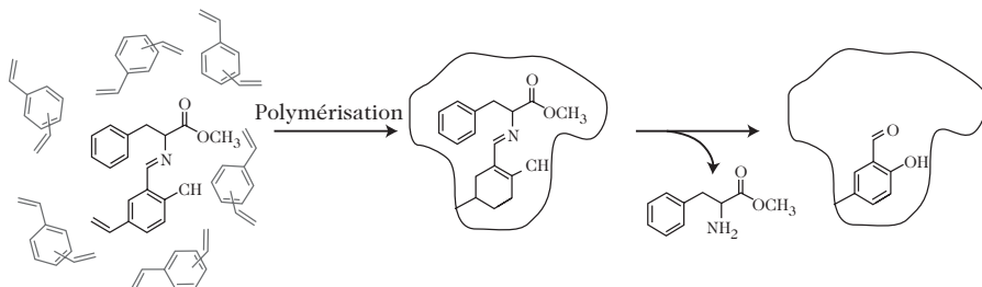
Fig. 27.3. Molecular imprinting by the covalent approach. From [13]
