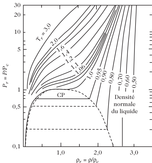
Fig. 20.2. Pressure–density diagram for CO 2 [3]
