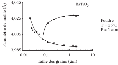
Fig. 28.5. Lattice parameters of BaTiO 3 in the powdered state, at 25°C and at standard atmospheric pressure, as a function of grain size [2]
