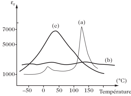
Fig. 28.3. Curves \epsilon_r = f(T) for a pure BaTiO 3 ceramic (a) and for X7R (b) and Z5U (c) ceramics
