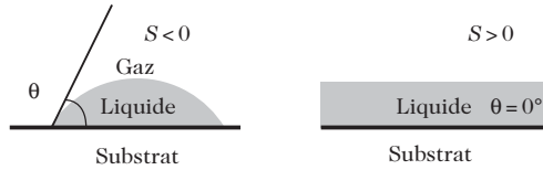
Fig. 22.6. Partial and total wetting
