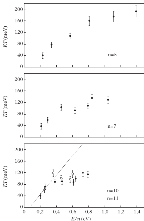
Fig. 3.16. Heat curves of \text{Sr}_n^+ determined from kinetic energies released by evaporation of strontium atoms. Taken from [27]
