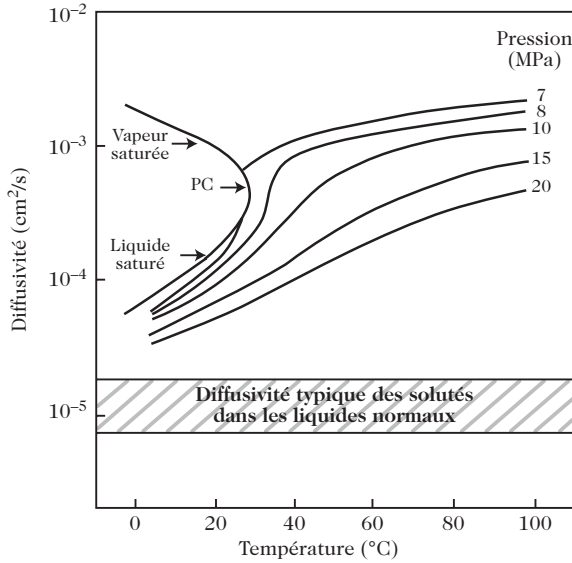
Fig. 20.4. Temperature dependence of the diffusivity at different pressures for a solute in CO 2 [10]
