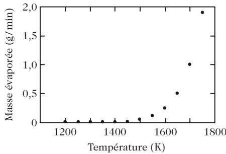
Fig. 16.17. Evaporated mass of copper as a function of the temperature for an evaporation area of 15 cm 2
