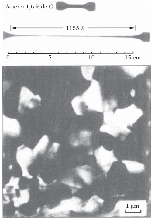
Fig. 9.1. Example of superplastic behaviour of an ultrahigh carbon steel. In this case, superplasticity is caused by the presence of fine spheroidal precipitates of cementite ( Fe_3C ) dispersed in a fine-grained ferritic matrix. Top: Test bar under tension before and after tests at 973 K with an imposed strain rate of 1.7 \times 10^{-4} s^{-1} . Bottom: Associated microstructure. Black particles are iron carbide and the light background is made from pure iron ( \alpha iron) or ferrite (solid \alpha solution). Taken from [12]
