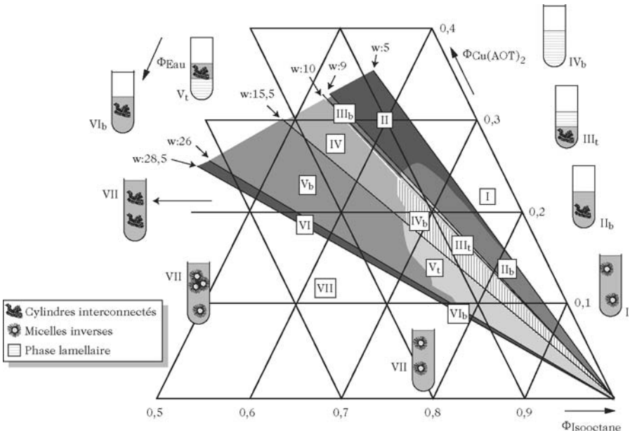
Fig. 18.6. Phase diagram of the water/Cu(AOT) 2 /isooctane ternary system. By gradually increasing the amount of water in a solution of Cu(AOT) 2 in isooctane, seven regions appear in the phase diagram. Each corresponds to a different association of phases. The boundaries of each region appear along a line of constant w = [H_2O]/[SA] , i.e., a line of constant water content. These transitions correspond to discontinuities in the level of surfactant hydration in the complex fluid. They are numbered from I to VII, with two- and three-phase systems indicated by b or t, respectively
