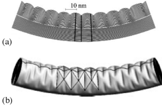
Fig. 8.32. Undulations of a 34-walled carbon nanotube. (a) Experimental observation in the plane of the tube axis [49]. (b) 3D simulation of the same [48]
