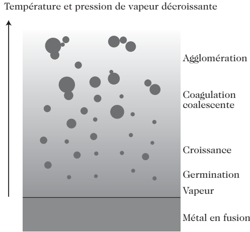
Fig. 16.11. Successive stages in the condensation of a gas when it occurs in a temperature gradient
