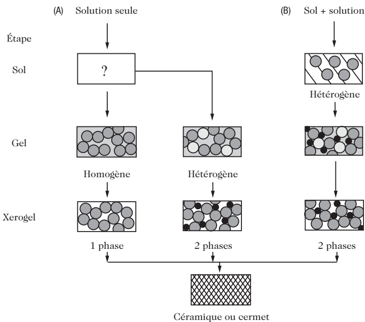
Fig. 17.3. Methods for preparing two-phase xerogels [1]. (A) All constituents are mixed together at the same time. (B) A solution is added to a sol. The question mark indicates that the sol can lead to a homogeneous or a heterogeneous gel depending on the chemical composition or the temperature (see text for details)
