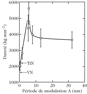
Fig. 24.2. Hardness as a function of the period \Lambda for TiN/VN multilayers epitaxied in the [100] direction. The TiN and VN layers have the same thickness [5]
