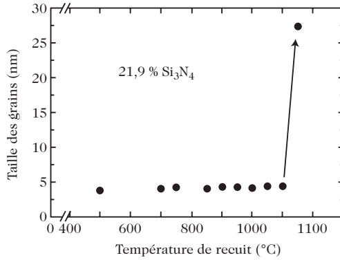
Fig. 24.4. Evolution of the grain size of a nanocomposite nc-TiN/a-Si 3 N 4 coating (hardness 48 GPa) when annealed in a hydrogen atmosphere ( p_{H_2} = 10^3 Pa) [16]
