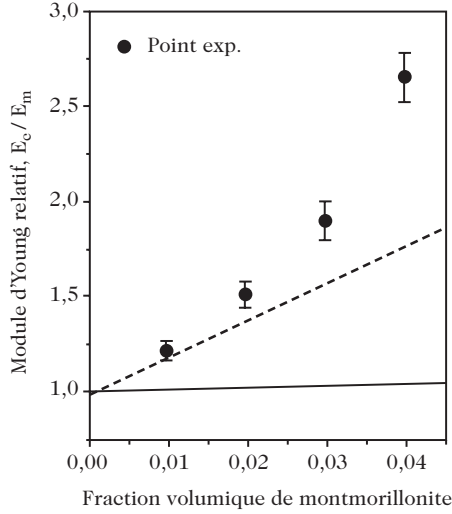
Fig. 14.16. Dependence of the relative Young’s modulus of nylon–montmorillonite nanocomposites on the volume fraction of nanoparticles. Also indicated are the predictions corresponding to the lower and upper bounds deduced from a mixing law. From [6]
