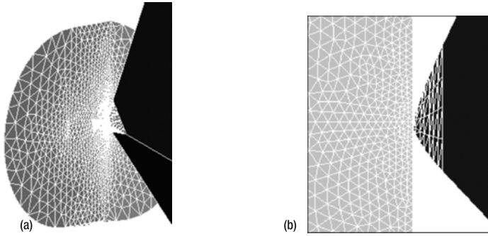
Fig. 8.29. Nanoindentation. Mesh
