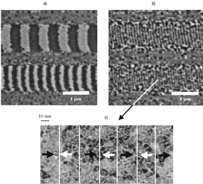
Fig. 28.10. Recording data in a magnetic material
