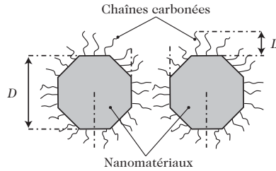
Fig. 22.12. Definition of the determining parameter \chi for the crystal structure of a 3D arrangement of nanomaterials coated by carbon chains: \chi = 2L/D
