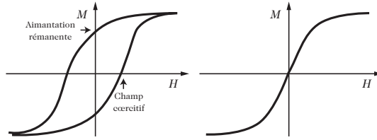
Fig. 23.2. Magnetisation curves of assemblies of ( left ) ferromagnetic and ( right ) superparamagnetic particles. The remanent magnetisation and coercive field disappear for superparamagnetic particles
