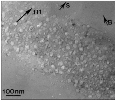
Fig. 25.10. TEM image showing a cross-section of a layer of bubbles obtained by implanting 1 \times 10^{17} \text{ He}^+/\text{cm}^2 at 1.6 MeV in a silicon monocrystal and annealing for 17 hr at 800^\circ\text{C} . From [30]
