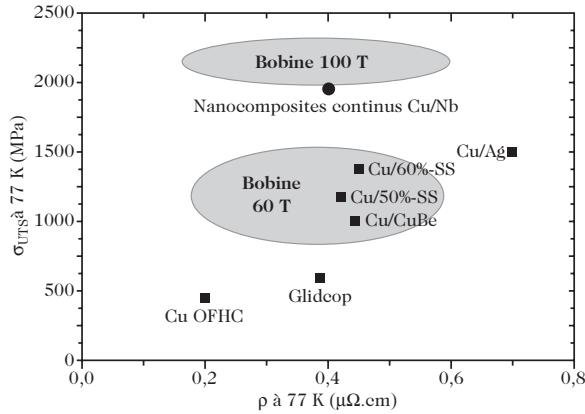
Fig. 30.17. State-of-the-art materials available for making coils for long-pulse magnetic fields: Cu OFHC (oxygen-free high conductivity copper), Glidcop (copper reinforced by \text{Al}_2\text{O}_3 particles), Cu/CuBe (copper/CuBe alloy macrocomposite), Cu/SS (copper/stainless steel macrocomposite), Cu/Ag (eutectic copper/silver alloy)
