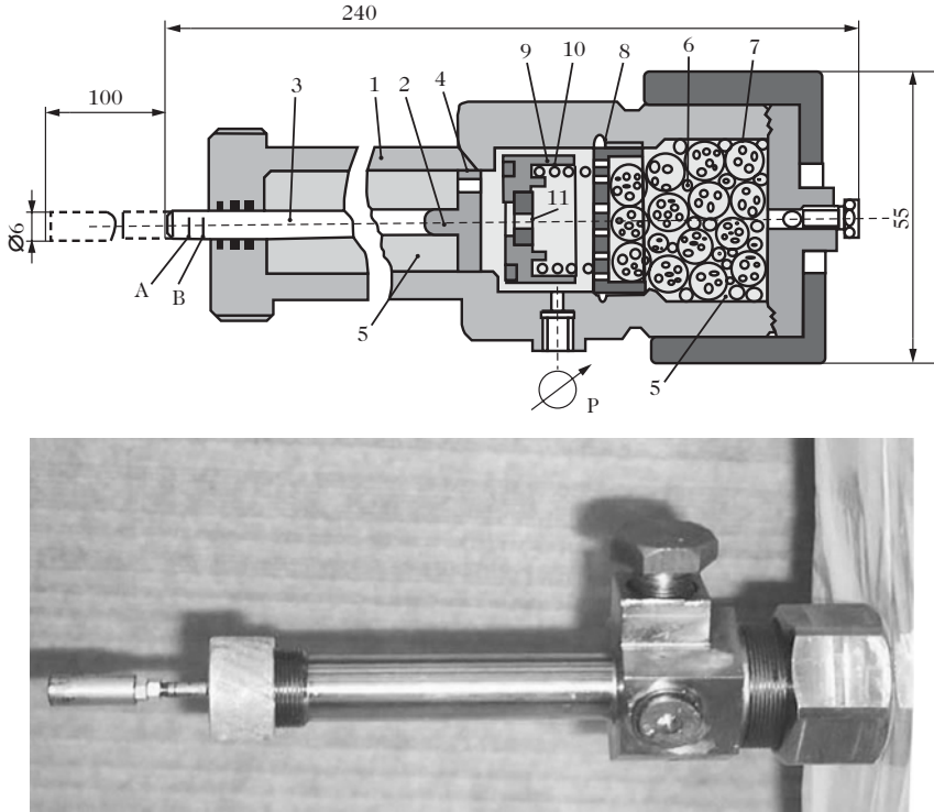
Fig. 30.16. Actuator for opening solar panels [18]. Upper: Diagram showing (1) cylindrical body, (2) piston, (3) spindle with markers A and B, (4) opening in the piston, (5) hydraulic oil, (6) porous matrix + non-wetting liquid, (7) flexible envelopes, (8) separation grid, (9) one-way valve, (10) spring, (11) diaphragm. Lower: Photograph
