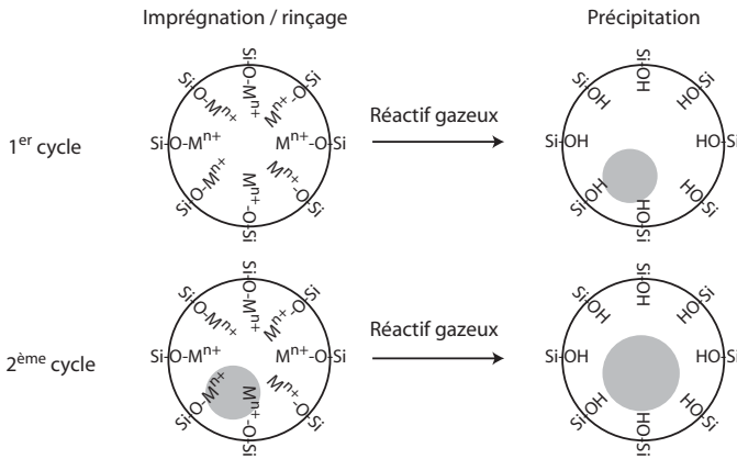
Fig. 25.4. Schematic representation of the general process for growing nanoparticles in mesoporous silica films. From [16]
