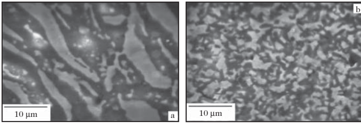
Fig. 30.3. SEM images of consolidated \text{Al}_2\text{O}_3\text{-Cr} 36% composites produced by (a) direct milling for 2 h and (b) reactive milling for 4 h [6]
