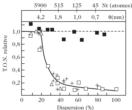
Fig. 10.10. Relative variation of the turn-over number (TON), i.e., the number of molecules transformed per surface atom and per unit time in given reaction conditions, as a function of the dispersion for hydrogenation of butene-1 ( black squares ), butyne-1 ( white squares ), butadiene-1,3 ( plus signs ), and isoprene ( white triangles ). \theta is the particle size and N_t is the total number of metal atoms in a particle of size \theta [34]
