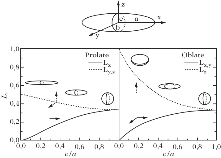
Fig. 7.11. Shape factors for prolate ellipsoids ( a \geq b = c, L_x \leq L_y = L_z ) and oblate ellipsoids ( a = b \geq c, L_x = L_y \leq L_z ) as a function of the ratio of the minor to major axes c/a . Polarisation directions x, y or z are shown. Different nanoparticle shapes are illustrated
