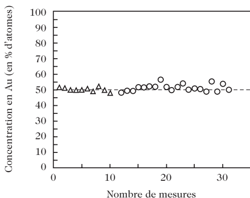
Fig. 10.14. Concentration of gold in a collection of Au–Ni clusters produced by laser vaporisation from an Au 50 Ni 50 rod (in % of atoms). Triangles and circles correspond to analysis of broad regions or individual particles, respectively [45]
