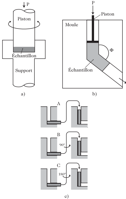
Fig. 19.9. Equipment for high-strain processing (a) under torsion, (b) by the angled tube method. (c) Different channels for the angled tube method. Channel A: direct. Channel B: with 90° rotation. Channel C: with rotation through 180°. From [23]
