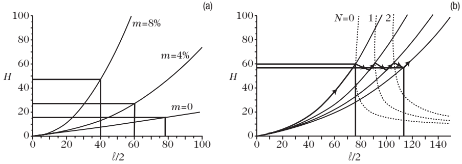
Fig. 1.13. Equilibrium shapes of stressed crystals. The profile of the crystals is represented for different values of the lattice mismatch m . Continuous curves represent the locus of intersection of the upper edge with the plane of the figure. (a) Stressed crystals. (b) Above a critical size, the crystals relax plastically through the successive appearance of dislocations. Dotted curves represent the thermodynamic criterion for the appearance of dislocations of order N ( = 0, 1, 2, \dots ). Taken from Müller and Kern [22]
