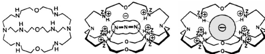
Fig. 13.4. Coordination of the anion N_3^- and a halide-type spherical anion by the hexaprotated bis-tren cryptand [9]
