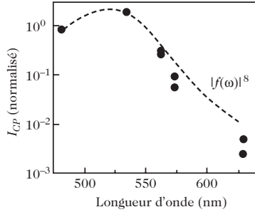
Fig. 7.14. Dispersion of the intensity I_{pc}(\omega) produced near the surface plasmon resonance in a nonlinear optical study of phase conjugation in a gold colloid solution. I_{pc} is proportional to |\chi^{(3)}(\omega, -\omega, \omega)|^2 and hence to |f(\omega)|^8 [31]
