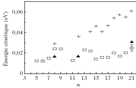
Fig. 3.15. Translational ( \square ) and total (+) kinetic energies released during evaporation of \text{Na}_n^+ clusters. The anharmonic PST calculation is shown by triangles . Taken from [26]
