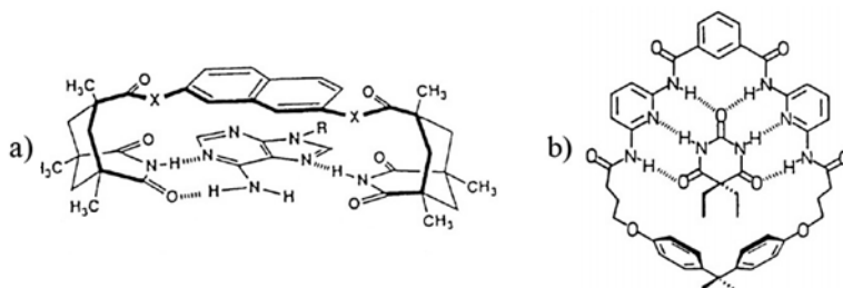
Fig. 13.3. (a) Adenine molecule complexed by an appropriate receptor using a network of hydrogen bonds. (b) Barbituric acid molecule coordinated by a cyclic receptor using a network of hydrogen bonds
