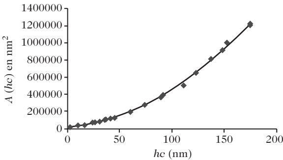
Fig. 8.15. Area function for a Berkovich indenter
