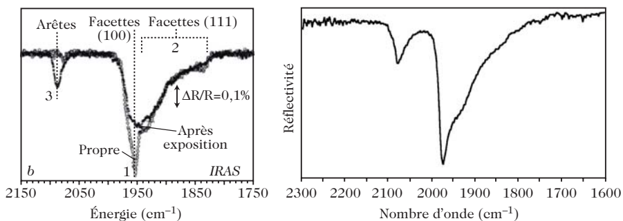
Fig. 10.9. Left : IRRAS spectrum of CO adsorbed at 300 K on clean Pd/Al 2 O 3 /NiAl (110) ( white circles ) and after exposure to methanol ( black circles ) [31, 32]. Right : IRTF spectrum of CO adsorbed on a Pd catalyst (0.5 wt%)/Si 3 N 4 (average diameter 4–5 nm)
