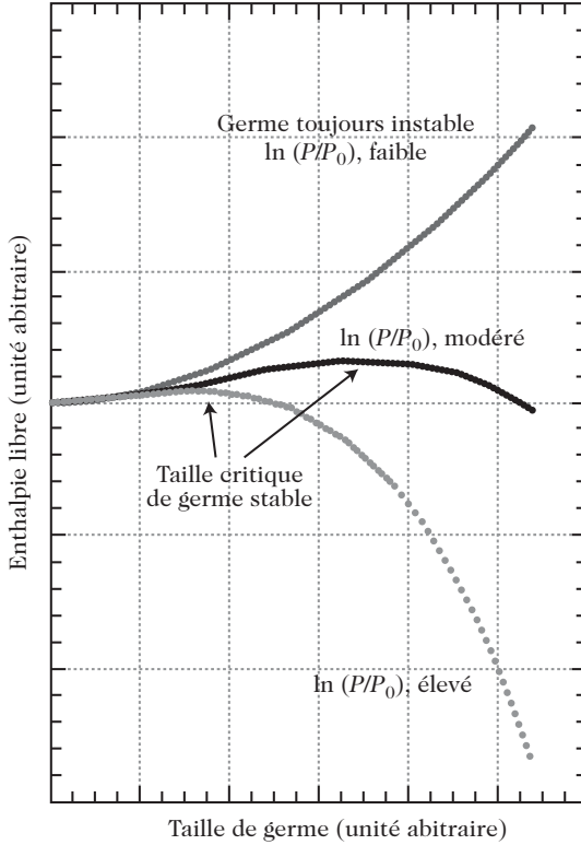
Fig. 16.9. Relation between germ stability and the degree of supersaturation, illustrated by representing the free enthalpy of the germs as a function of their size. If the ratio P/P_0 is too small ( upper curve ), there are no stable germs and condensation does not proceed. When the ratio P/P_0 is high enough, stable germs can form. Their size, given at the maximum of the free enthalpy curve, will decrease as P/P_0 increases (from the middle curve to the lower curve )
