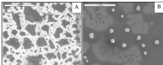
Fig. 22.8. Scanning electron microscope observations of Ag 2 S particles deposited (A) on molybdenum sulfide, a substrate producing attractive forces, and (B) on cleaved graphite, a substrate producing repulsive forces. (A) Extensive bright zones correspond to monolayers of nanocrystals with spaces (dark zones corresponding to naked substrate). (B) Broad bright zones correspond to monolayers of nanocrystals surrounded by dark zones corresponding to naked substrate. In the dark zones, brighter spots are observed, corresponding to 3D arrangements of nanocrystals. Taken from [31] © 2000 American Chemical Society
