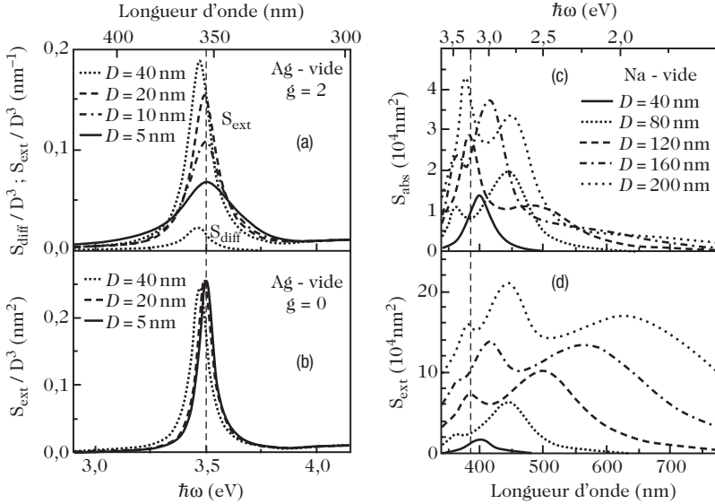
Fig. 7.9. (a) and (b) Spectra of the extinction cross-section S_{\text{ext}} and scattering cross-section S_{\text{scatt}} for silver nanoparticles of diameters D = 5, 10, 20 and 40 nm in vacuum, calculated using the Mie model and a dielectric constant that has been corrected ( g = 2 ) or not ( g = 0 ) for surface effects [see (7.17)]. The broadening and reduction in maximal amplitude of S_{\text{ext}} at small sizes is a consequence of this correction. For g = 0 , S_{\text{ext}} \propto D^3 in the quasi-static approximation. (c) and (d) S_{\text{abs}} and S_{\text{ext}} for sodium nanoparticles of diameter D = 40, 80, 120, 160 and 200 nm [17]. Vertical lines indicate \hbar\Omega_{\text{R}}^{\text{qs}} , calculated using the Mie theory in the dipole approximation, or equivalently, in the quasi-static approximation
