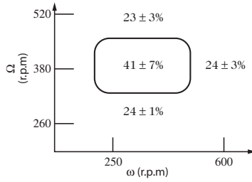
Fig. 19.4. Determining the parameter range leading to amorphisation of Ni 3 Al, for a planetary mill. The rate of rotation of the turntable (revolutions per minute) is plotted on the vertical axis . Volume fractions of the amorphous phase are indicated directly on the figure. These fractions are determined by X-ray diffraction [2]
