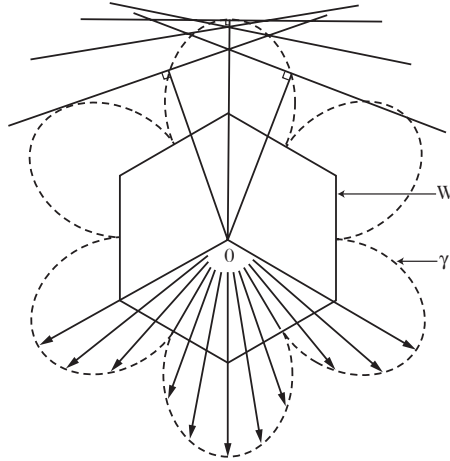
Fig. 1.4. Wulff construction of the equilibrium shape of a crystal from the \gamma -graph (dashed curve). O is the center of the crystal. The hexagon represents a projection of the equilibrium shape of the crystal (Wulff polyhedron). From [11]
