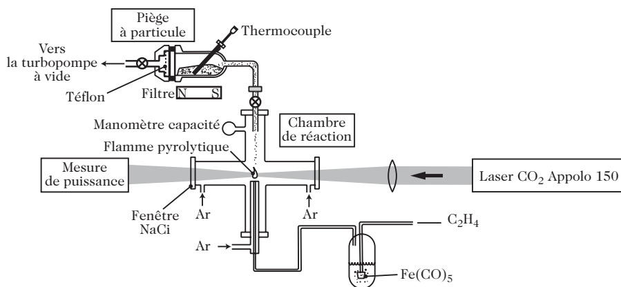
Fig. 16.23. Setup for synthesising a nanopowder by laser pyrolysis [26]. Synthesis of iron and carbon compounds
