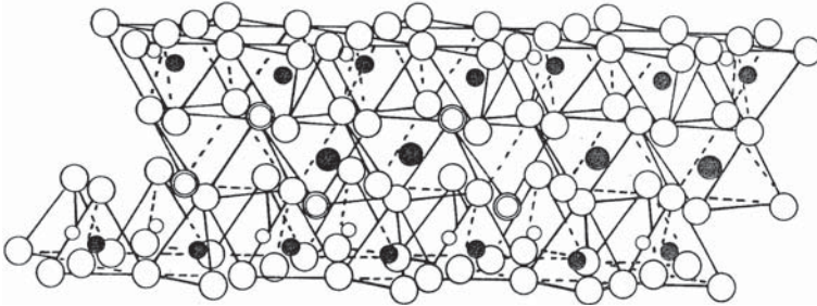
Fig. 14.6. Structure of dioctahedral 2:1 phyllosilicate sheets, e.g., montmorillonite. The sheets carry a negative charge due to substitutions of cations of given valence by cations of lower valence. The interlayer space is occupied by water molecules and, in natural clays, by Na^+ , Ca^{2+} or Mg^{2+} cations
