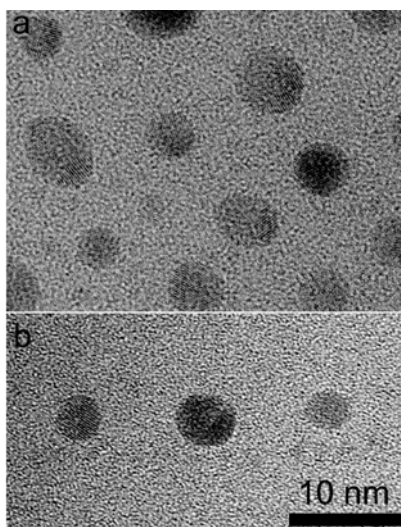
Fig. 25.14. TEM images of silver nanoparticles embedded in \text{Al}_2\text{O}_3 , obtained by pulsed laser deposition. (a) Top view. (b) Cross-sectional view. Taken from [44]
