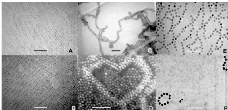
Fig. 23.7. Transmission electron microscope images of a monolayer (A), (C), (E), and a bilayer (B), (D), (F), of cobalt nanocrystals. Particle diameters: (A) and (B) 10 nm, (C) and (D) 12 nm, (E) and (F) 16 nm. Scale bars 100 nm. Taken from [5] © 2001 AAAS
