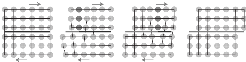
Fig. 8.5. Motion of an edge dislocation. The dislocation line runs perpendicular to the plane of the figure and marks the boundary between the region already sheared ( light grey ) and the unsheared region ( dark grey )
