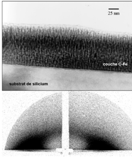
Fig. 25.12. TEM ( top ) and GISAXS ( bottom ) images of a thin film of iron clusters embedded in a carbon matrix, obtained by ion codeposition. The columnar structure of the clusters observed in the TEM image is confirmed by the elliptical shape of the small-angle scattering ring in the GISAXS image. From [34] © 2000 American Institute of Physics
