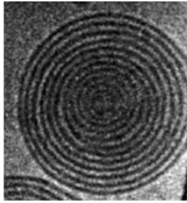
Fig. 31.3. Multilamellar phospholipid vesicles obtained by shearing a lamellar phase and dispersing in water [4]
