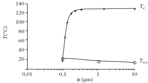
Fig. 28.6. Temperatures T_{ot} and T_c of the orthorhombic–tetragonal and tetragonal–cubic phase transitions, respectively, as a function of grain size for BaTiO 3 powders at standard atmospheric pressure [3]
