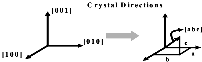
Figure 1-15 Nomenclature of crystal directions.
