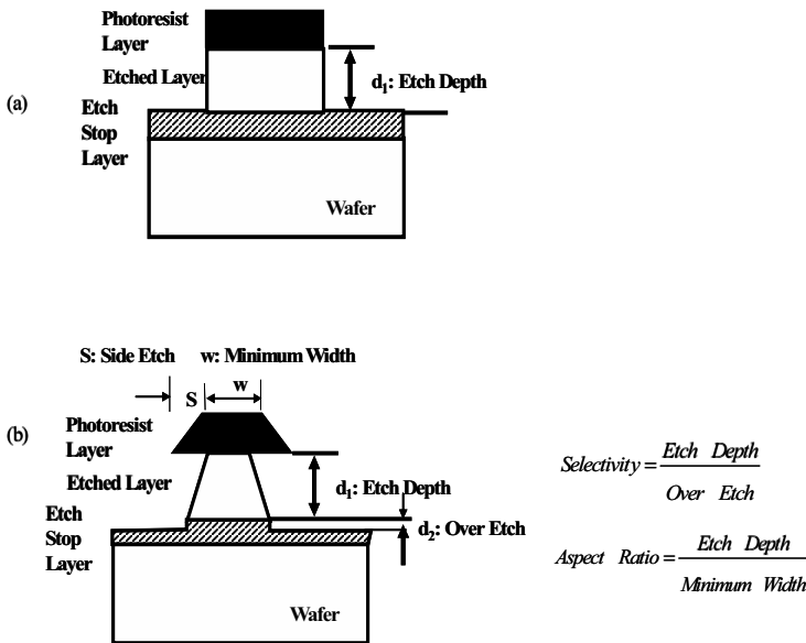
Figure 1-5. Pattern transfer definition. (a) Ideal. (b) Realistic. (After [25].)
