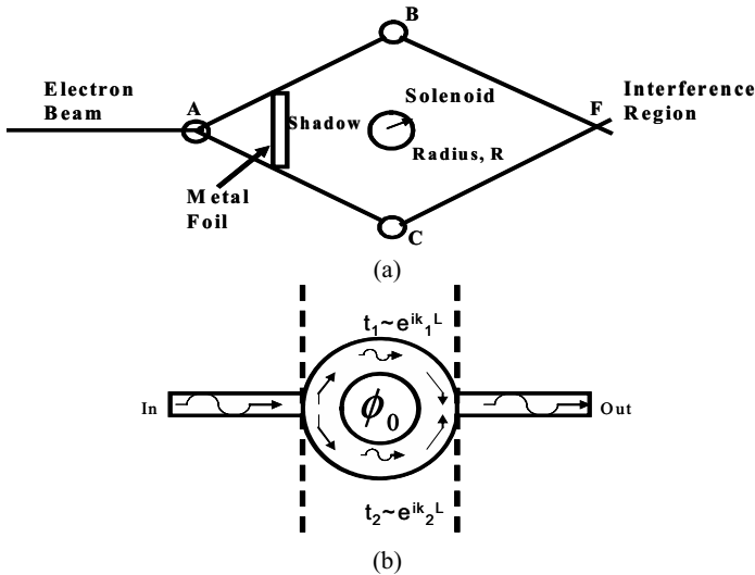
Figure 3-7. (a) Aharonov-Bohm-effect electron wave interference setup. (After [125].) (b) Sketch of metallic ring implementation.
