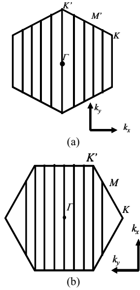
Figure 3-16 (a) A 1D band structure lies at each of the discrete values of k_x for a (5, 5) armchair CNT, dictated by the circumferential quantization in this direction. The armchair CNT is metallic. (b) A 1D band structure lies at each of the discrete values of k_y for a (9, 0) zigzag CNT, dictated by the circumferential quantization in this direction. The zigzag CNT is semiconducting. (After [46].)
