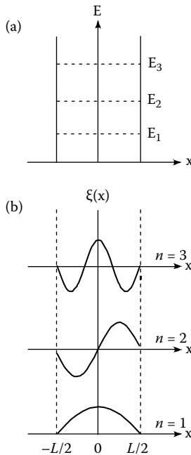
FIGURE 2.5 (a) One-dimensional well potential with infinite height and several energy eigenstates represented by dashed lines, (b) corresponding envelope functions.
