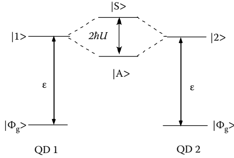
FIGURE 2.8 Symmetric and antisymmetric states, |S\rangle and |A\rangle , generated by the interaction between energy levels |1\rangle and |2\rangle of QDs 1 and 2, respectively.
