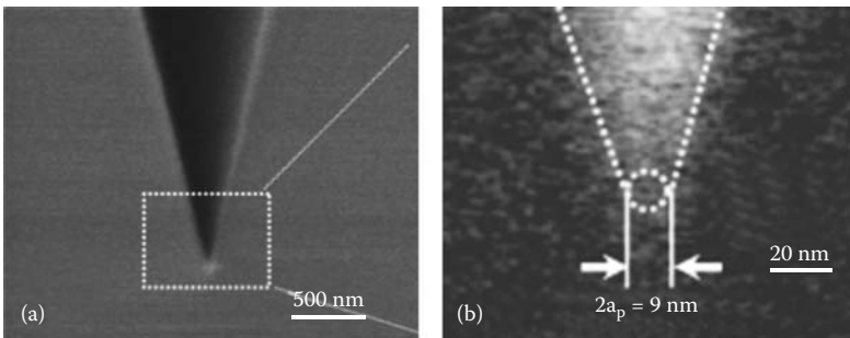
FIGURE 4.4 SEM images of an ultraviolet fiber probe. The magnified image of (a) is shown in (b). 2a_p : apex diameter.
