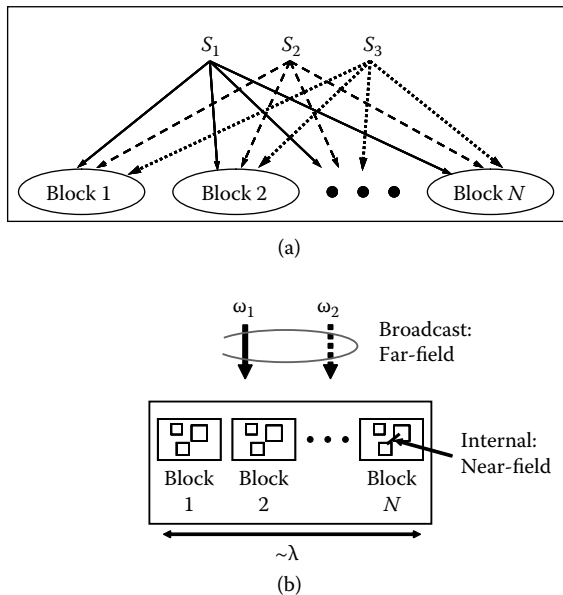
FIGURE 5.3 (a) Broadcast interconnects for parallel processing. (b) Their nanophotonic implementation using near-field interaction between QDs for internal functions and far-field excitation for identical data input (broadcast) to nanophotonic devices within a diffraction-limit-sized area.
