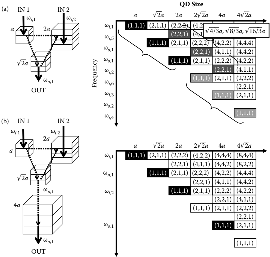
FIGURE 5.4 Frequency partitioning among external and internal channels, and examples in (a) multiple implementations of 3-dot nanophotonic switches, and (b) 4-dot configuration for sum of products.
