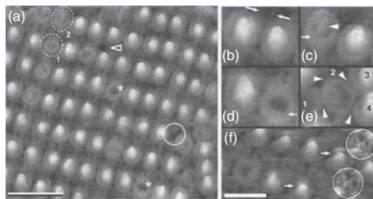
Figure 9.1 (a) High-resolution AFM image of a two-dimensional crystal of RC–LH1 complexes. The broken circle (1) and the ellipse (2) mark complexes that lack the RC–H subunit. The asterisks denote ‘empty’ LH1 complexes that completely lack the RC seen from the cytoplasmic side. The arrow denotes a missing RC seen from the periplasmic side. (b) to (e) show a variety of complexes at higher magnification. (f) shows the periplasmic side of the RC–LH1 complex imaged at higher load. The scale bars are 40 nm in (a) and 15 nm in (f). Reproduced with permission from D. Fotiadis et al. , J. Biol. Chem 279 , 2063 (2004)
