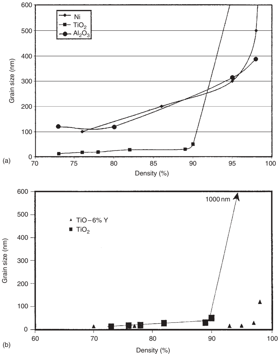
Figure 5.9 The effect of compact density on grain growth for (a) nanocrystalline Ni, \text{TiO}_2 and \text{Al}_2\text{O}_3 and (b) for TiO doped with 6% yttrium and \text{TiO}_2 showing a possible solute drag effect on grain growth. After J. Groza, Consolidation methods, in Nanostructured Materials: Processing Properties and Applications , ed. C. C. Koch, 2003. Reproduced by permission of IOP Publishing Limited
