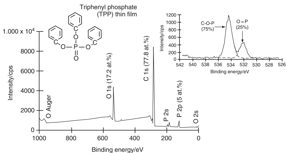
Figure 2.25 Schematic XPS spectrum from a triphenyl phosphate polymer film: (a) survey scan showing the elemental composition (in at %) and (b) high-resolution scan of the oxygen 1s peak showing two chemical states of oxygen and their relative proportions
