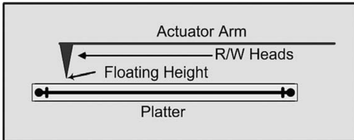
FIGURE F.2 Floating height is the distance between the R/W heads on a drive and the platter while the drive is spinning.
