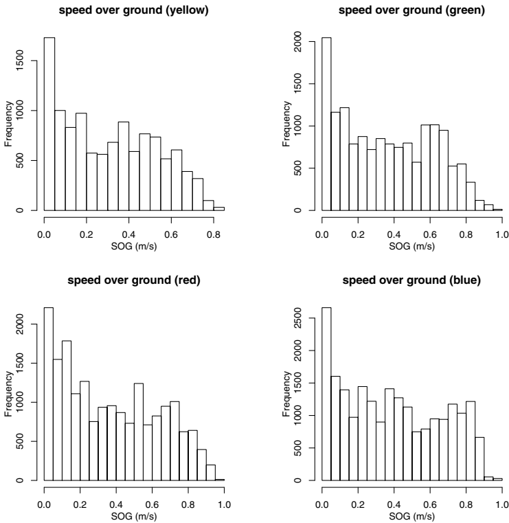
Fig. 9 Histograms showing the typical boat speed distribution during the tests. The plots indicate that the boats reach comparable speeds. Note that the yellow boat started the course later and the wind calmed down towards the end of our test.
