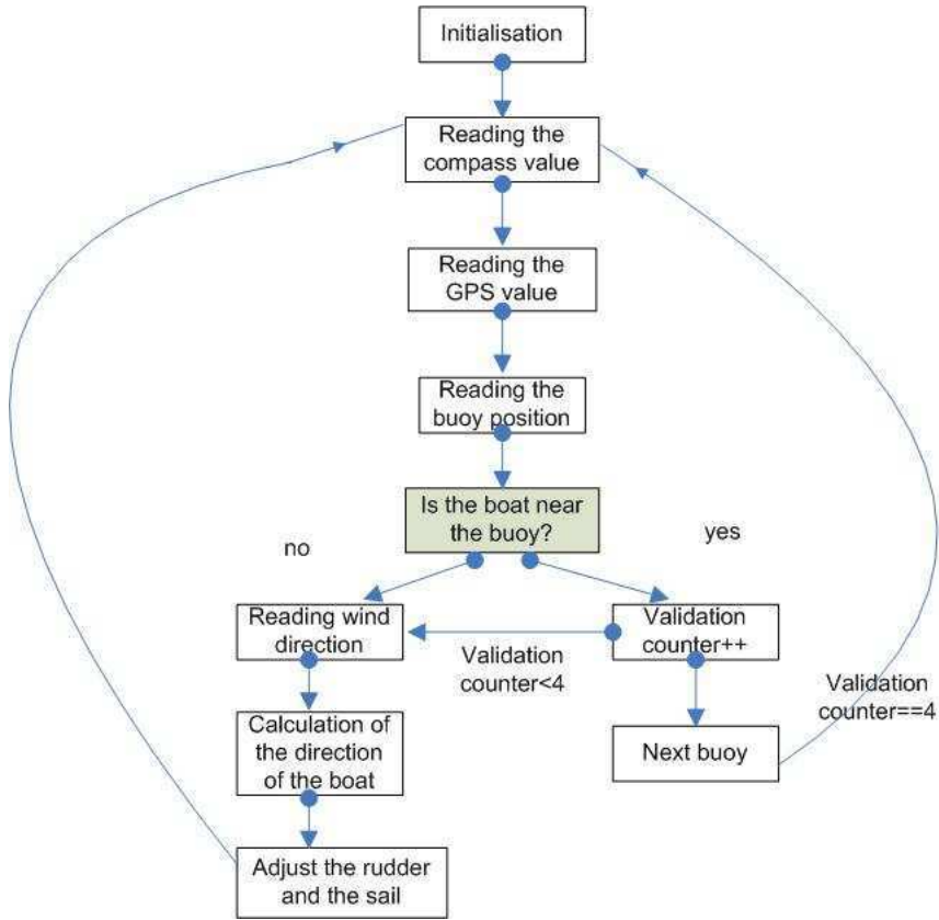
Fig. 7 Navigation algorithm
