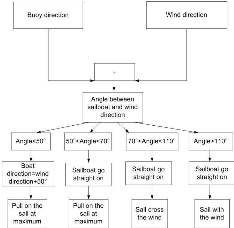
Fig. 8 Direction algorithm
