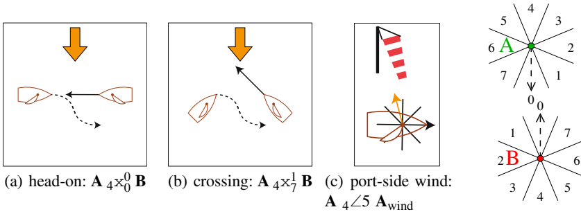
Fig. 5 Two sailing vessels in a head-on and a crossing situation and the advised collision avoidance behavior Fig. 6 An example relation for OPRA_4^x : A \text{ }_4 \times_0^0 \text{ } B
