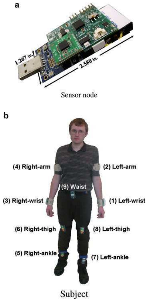
Fig. 5.1 (a) A sensor node composed of processing unit and custom-designed sensor board. The motion sensor board has a triaxial accelerometer and a biaxial gyroscope. Sensor node and subject (b) A subject wearing nine sensor nodes
