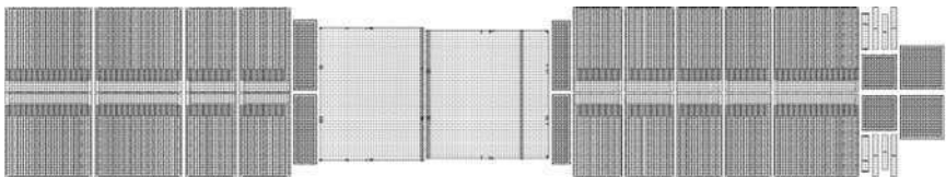
Fig. 1.25 Placement for a telescopic opamp with gain-boost amplifiers
