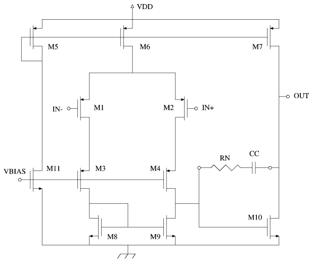
Fig. 1.1 Schematic of a two-stage Miller compensated opamp with asymmetric output stage
