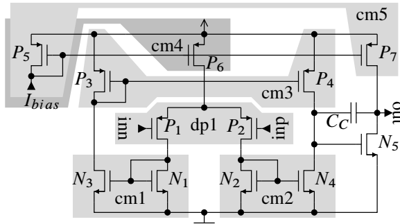
Fig. 3.10 A simple amplifier with recognized building blocks
