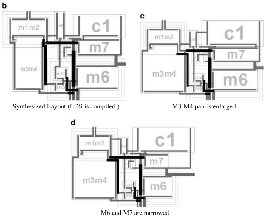
Fig. 4.25 LDS code for the OPAMP of (a) is used to synthesize the layouts in (b), (c), and (d)
