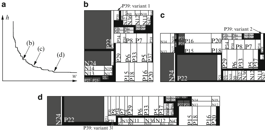
Fig. 3.39 Example 5 ([37], © IEEE 2008): placements (b)–(d) and the corresponding shape function (a)
