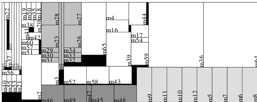
Fig. 3.40 Result of “biasynth_2p4g” obtained by Plantage ([37], © IEEE 2008) (time: 5.6 min, area usage: 104.96%)
