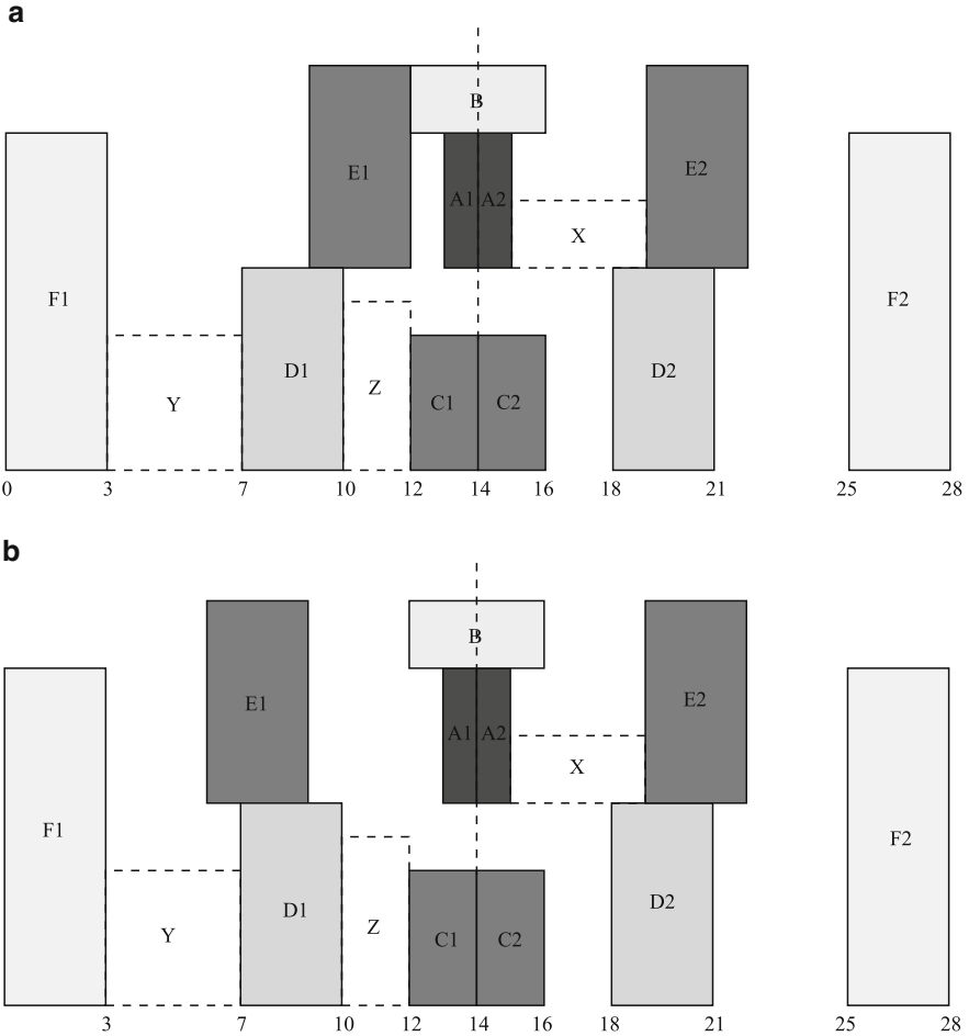
Fig. 1.21 Placements of the symmetric-feasible sequence-pair (F_1 E_1 B A_1 A_2 X E_2 Y D_1 Z C_1 C_2 D_2 F_2, F_1 Y D_1 Z C_1 C_2 D_2 E_1 A_1 A_2 B X E_2 F_2) after the sweep-to-the-right (Step 3x) and after the sweep-to-the-left traversal (Step 4x)
