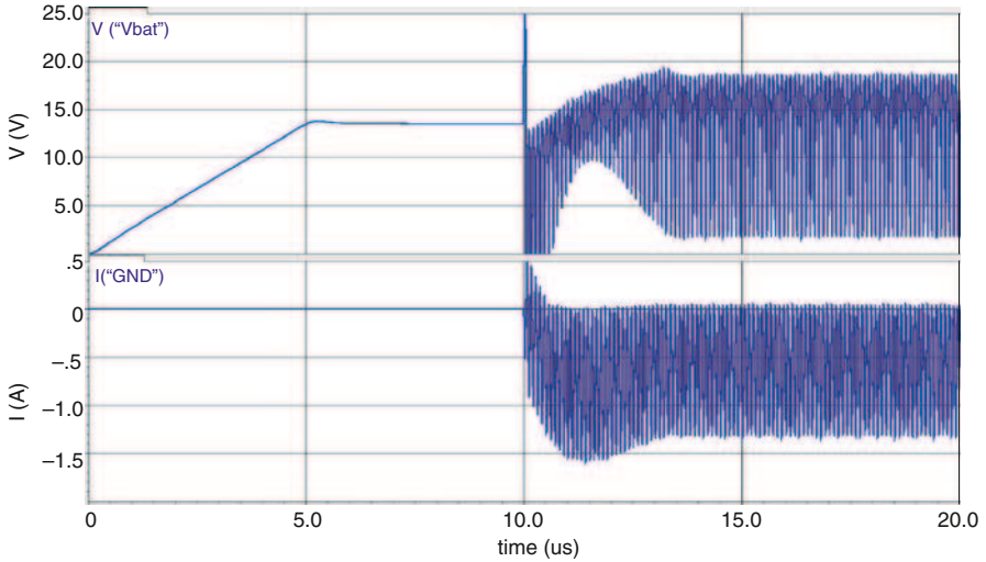
Fig. 8 DPI simulation result of the impedance reduction circuit for 10 MHz and 37 dBm ( V_{\text{BAT}} , I_{\text{GND}} )
