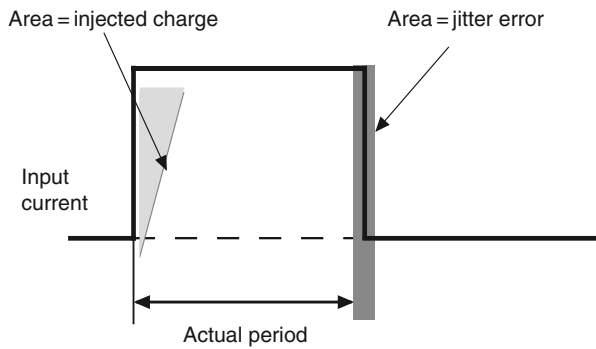
Fig. 19 Jitter sensitivity
