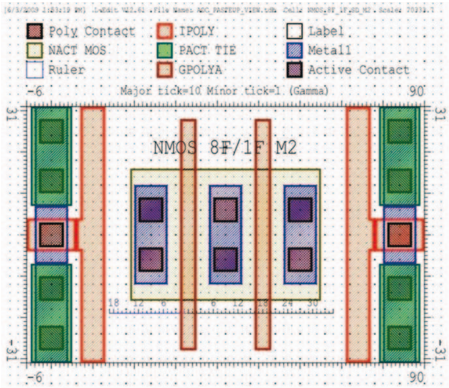
Fig. 7 Basic device design accommodates up to L=2 \text{ F} , has close tie spacing to achieve good HF performance. Dummy gate connects to metal Vss between vertical tie split to achieve gate pattern uniformity. Dimensionless GAMMA ( \Gamma ) units are used where 1\Gamma=0.01 \mu\text{m} at the 32 nm node. Minimum gate extension is 12 \Gamma at 45 nm and beyond to avoid gate-end rounding effects
