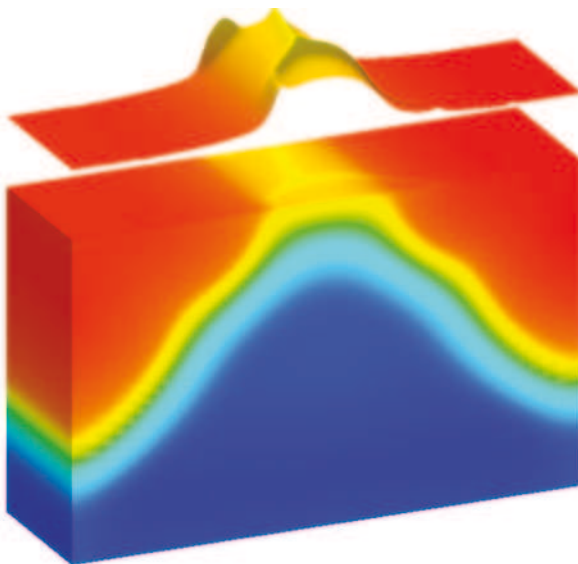
Fig. 9 Potential distribution in a 35 nm MOSFET subject to PSG
