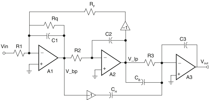
Fig. 3 Active-RC loop filter with feed-forward trajectories
