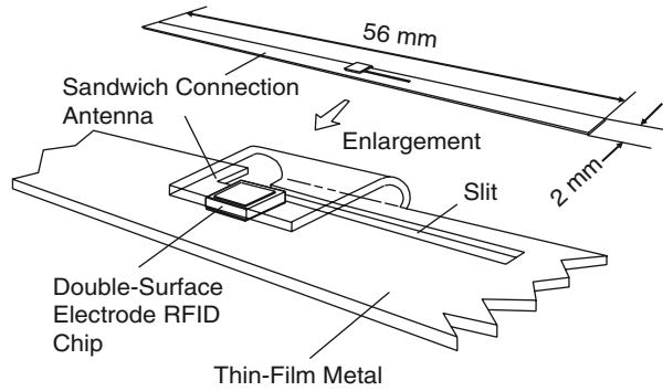
Fig. 7 Antenna connection technology of ultra-small RFID chip. The double-surface electrode RFID chip can be easily connected to the antenna without precise positioning
