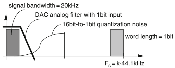
Fig. 5 Signal spectrum at the \Sigma\Delta modulator output
