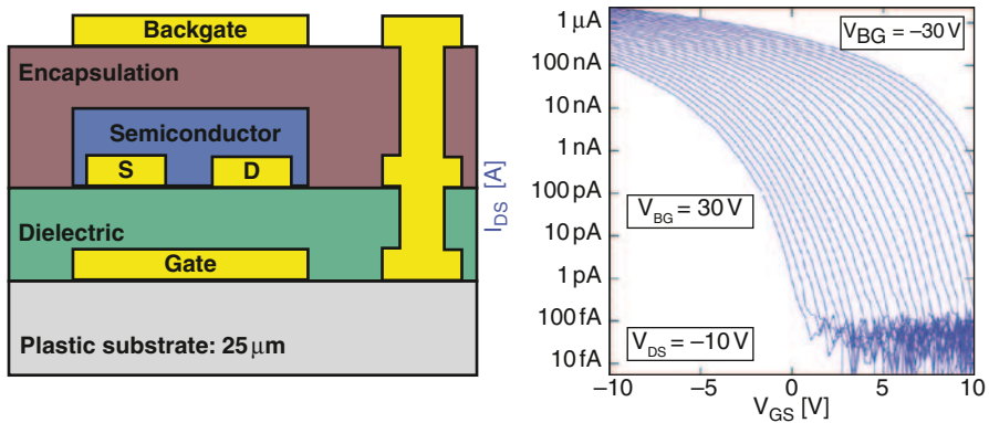
Fig. 12 Cross-section of the dual-gate OTFT technology (left) and a typical measured transfer characteristic of this OTFT when using the backgate as V_T -control gate (right). The channel width equals 140 \mu\text{m} , the channel length 5 \mu\text{m}
