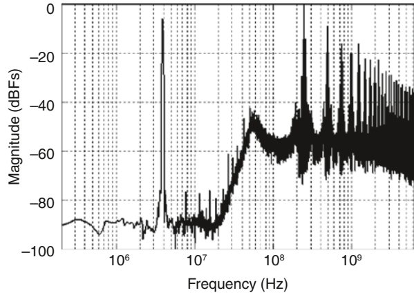
Fig. 7 Measured output spectrum of the modulator
