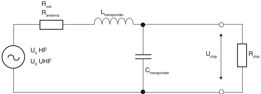
Fig. 2 UHF and HF equivalent resonance circuit
