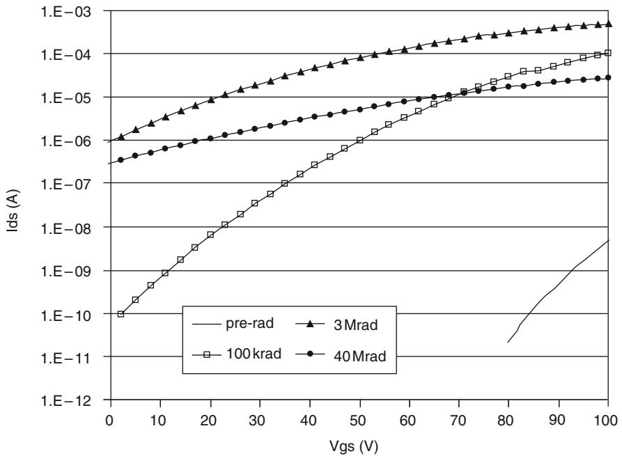
Fig. 4 Current flowing in a FOXFET using n-well as drain and n+ diffusion as source, and polysilicon gate (W/L = 200/0.03 μm) before and after exposure to TID up to 40 Mrad(SiO 2 )
