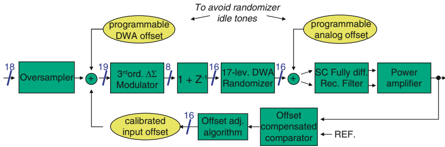
Fig. 33 DAC block diagram with offset compensation circuit
