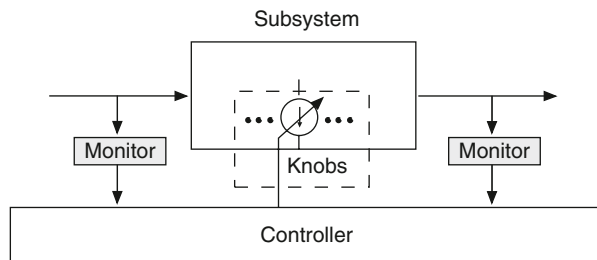
Fig. 9 Principle schematic of knobs and monitors concept to overcome degradation and failures
