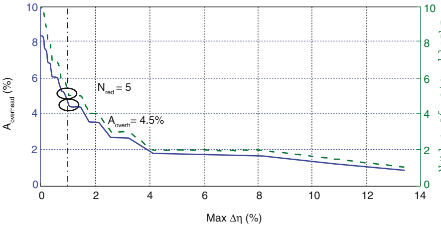
Fig. 12 Trade-off between area overhead and granularity of the extra subtransistors, which is directly related to the allowed “ripple” Δη on the power efficiency [23]
