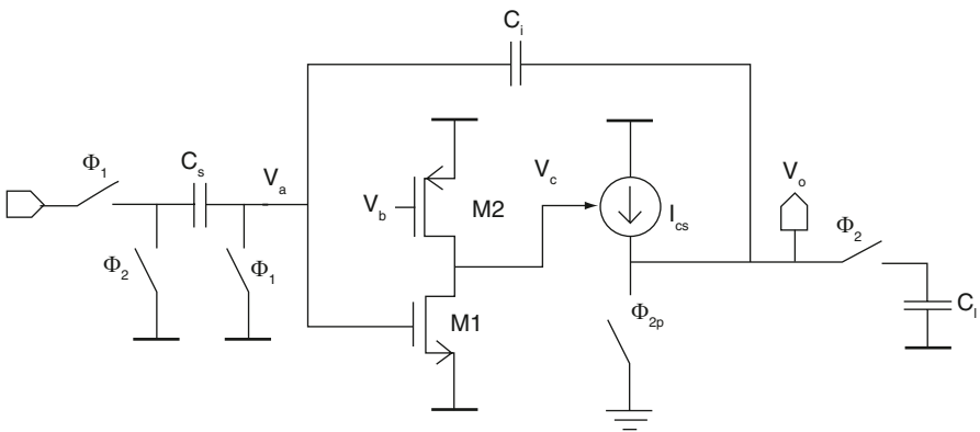
Fig. 5 A zero-crossing based switched-capacitor integrator
