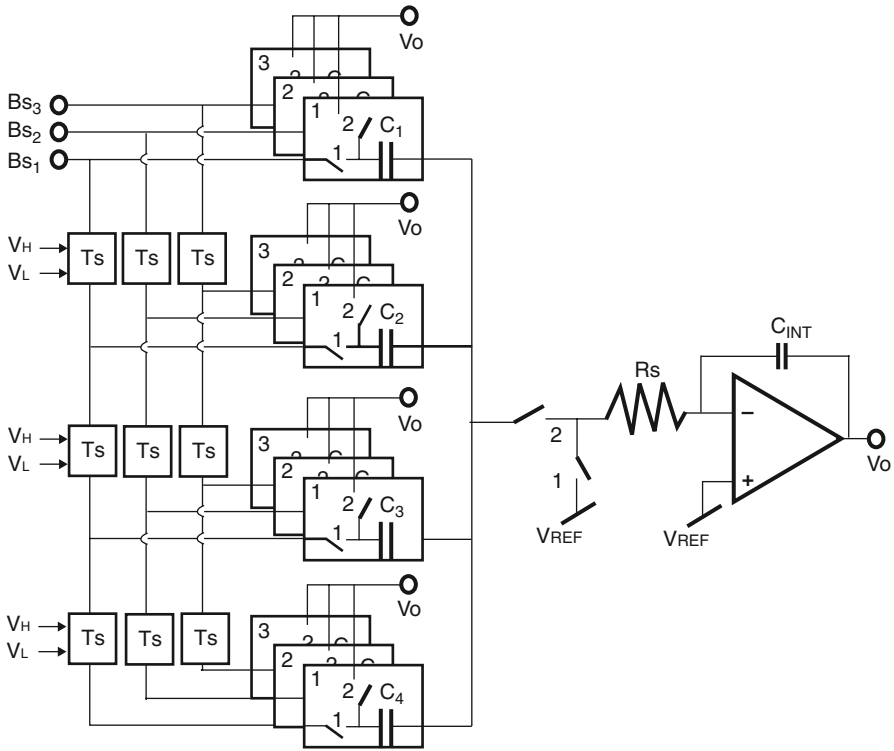
Fig. 17 Single-ended audio-DAC
