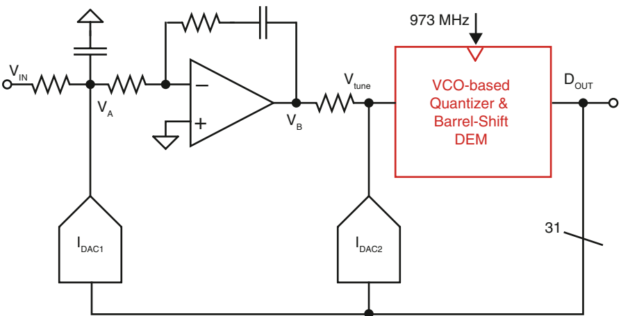
Fig. 9 A simple continuous-time Sigma-Delta ADC topology offering third order quantization noise shaping with only one opamp
