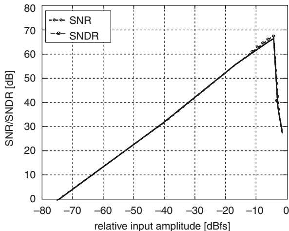
Fig. 12 Measured SNR and SNDR as function of input signal amplitude
