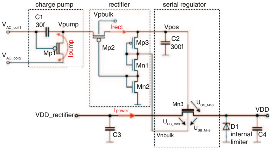
Fig. 9 High voltage blocker as DC/DC down-converter
