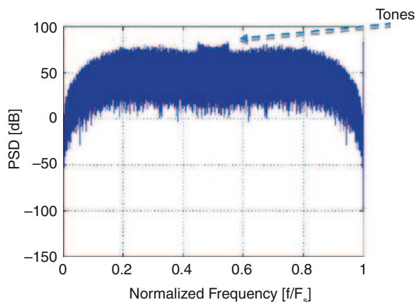
Fig. 8 Signal spectrum at the ΣΔ modulator output
