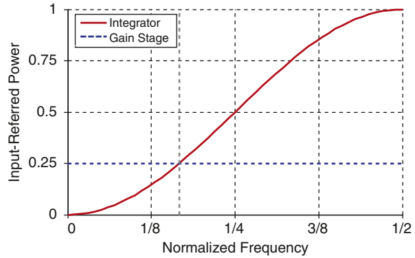
Fig. 10 Input-referred noise comparison between a gain and integrator stage
