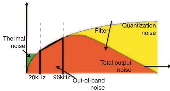
Fig. 11 Signal spectrum at the analog filter output
