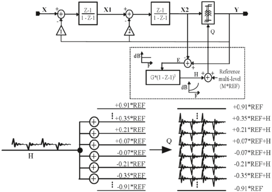
Fig. 28 Modified \Sigma\Delta for idle-tone reduction
