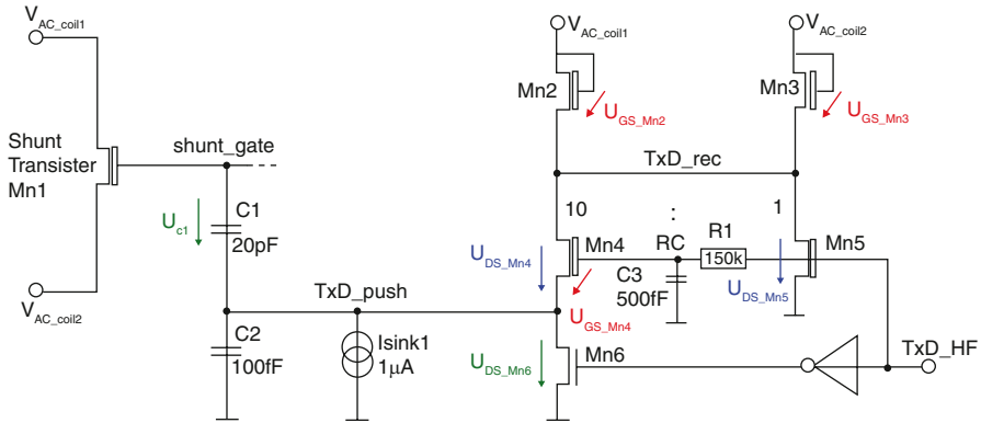
Fig. 19 Shunt and TxD unit
