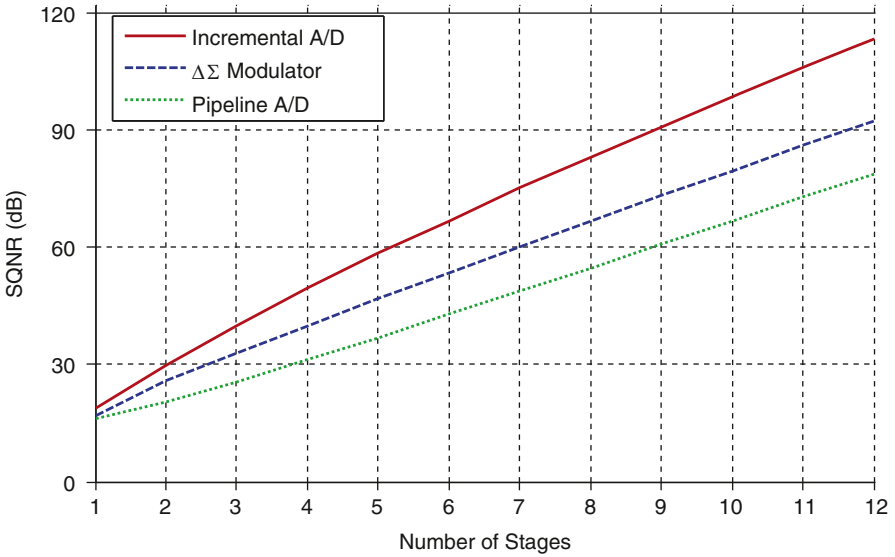
Fig. 14 Simulated SQNR vs. Number of Stages at an OSR of 3
