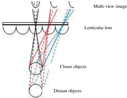
Fig. 8. Relationship between Lenticular lens and object
