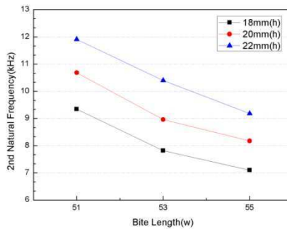
Fig. 4. Second resonant frequency of the tool holder in PZT excitation
