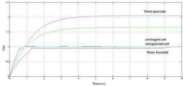
Fig. 11. Output response due to membership shapes variation
