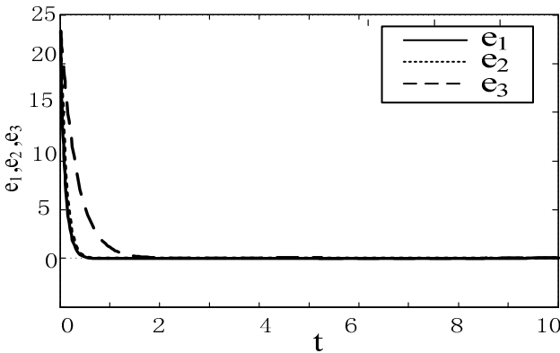
Fig. 2. (a) the errors of e_1, e_2 converge to zero about 0.6s, and the e_3 converges to zero about 1.5s. (b) the x_2 of system (4) synchronized to the x_1 of the system (3). This shows that the identical fractional-order Chen systems can be synchronized.
