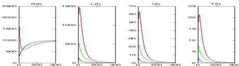
Fig. 1. Globally asymptotically stable of the disease free equilibrium E_0 for system (1)
