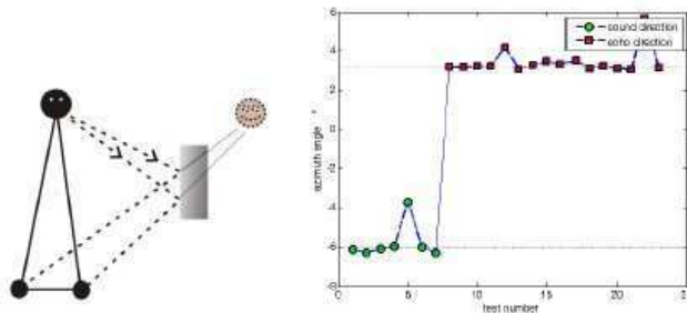
Fig. 2. (a) The echo scenario with rection from a nearby object. The rection of the soundwave shifted the phase. The position of the object is "mirrored" to the other side. (b Sound direction. 25 groups of sound wave amplitude are acquired before FFT process during a sound buzz in 1 second.
