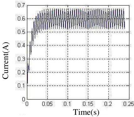
Fig. 2. The current curve with compensation network
