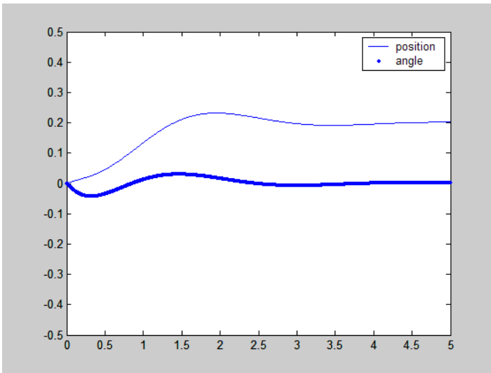
Fig. 1. Position and angle in robust stabilization (the nominal system)
