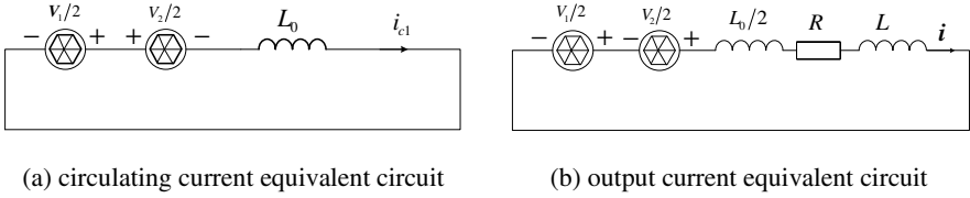
Fig. 2. Equivalent circuit of parallel inverter system
