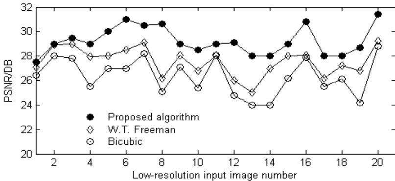
Fig. 2. PSNR comparison results
