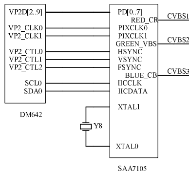
Fig. 3. Connection between SAA7105 and TM320DM642
