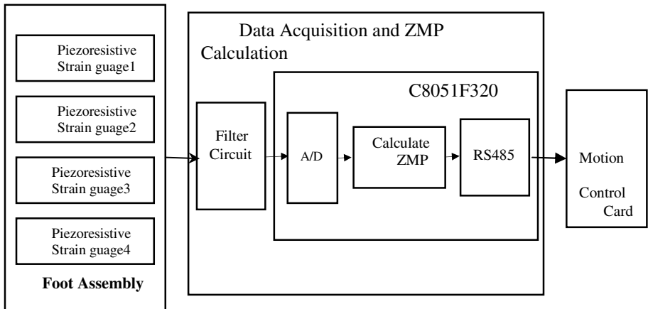
Fig. 5. Block Diagram of ZMP sensory system
