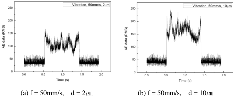
Fig. 11. AE signal for vibration cutting
