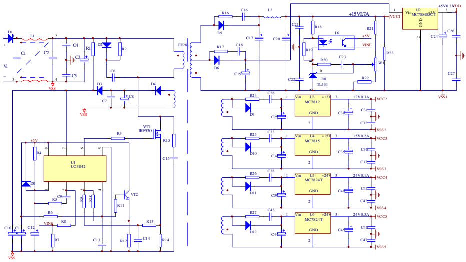
Fig. 2. Main circuit
