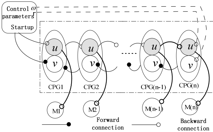
Fig. 9. The Robotic control system based on the CPG control system
