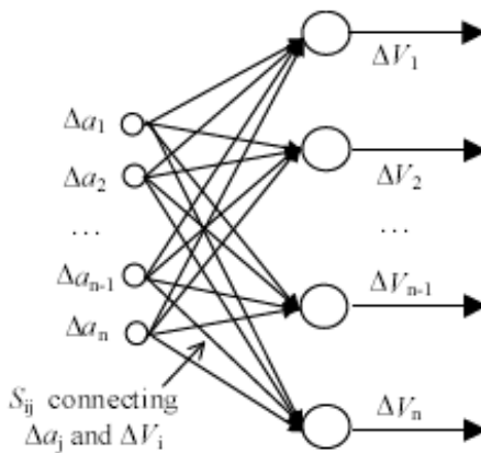
Fig. 1. The neural network used for sensitivity evaluation
