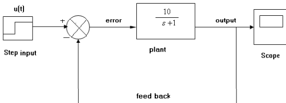
Fig. 1. Closed loop output model
