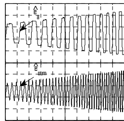
Fig. 11. Estimation waveforms of \hat{e}_a and \hat{e}_{sum} (20V/div; 60ms/div;)
