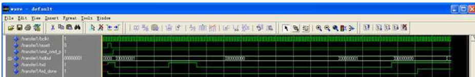
Fig. 3. The simulation waveform of UART transmitter
