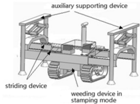
Fig. 1. Structure of weeding robot
