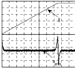
Fig. 8. Waveforms of speed estimation and speed error ( n^* : 160rpm/div; n_{err}^* : 2rpm/div; t : 100ms/div;)
