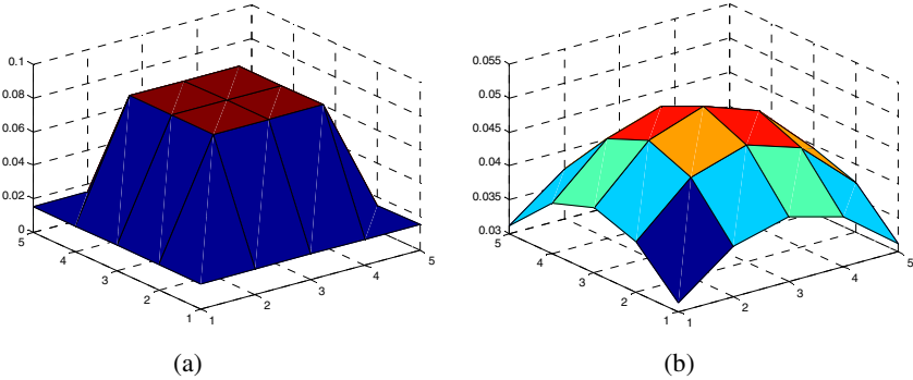
Fig. 1. Gaussian kernel (a) and Kaiser Window function (b)
