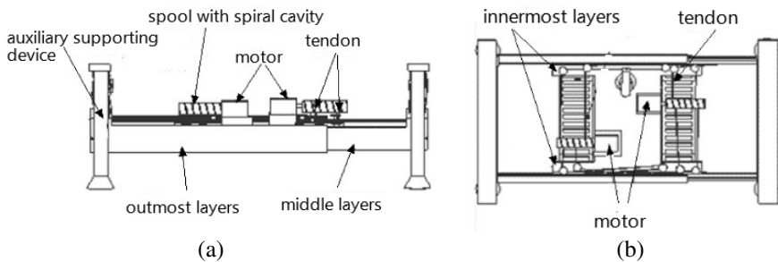
Fig. 8. Striding device
