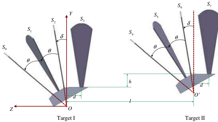
Fig. 1. Geometry relation between target I and II
