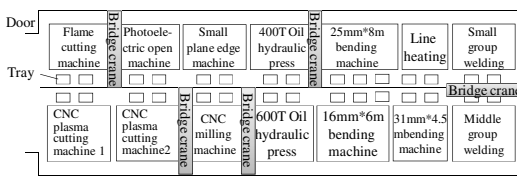
Fig. 6. Steel machining plant layout plan
