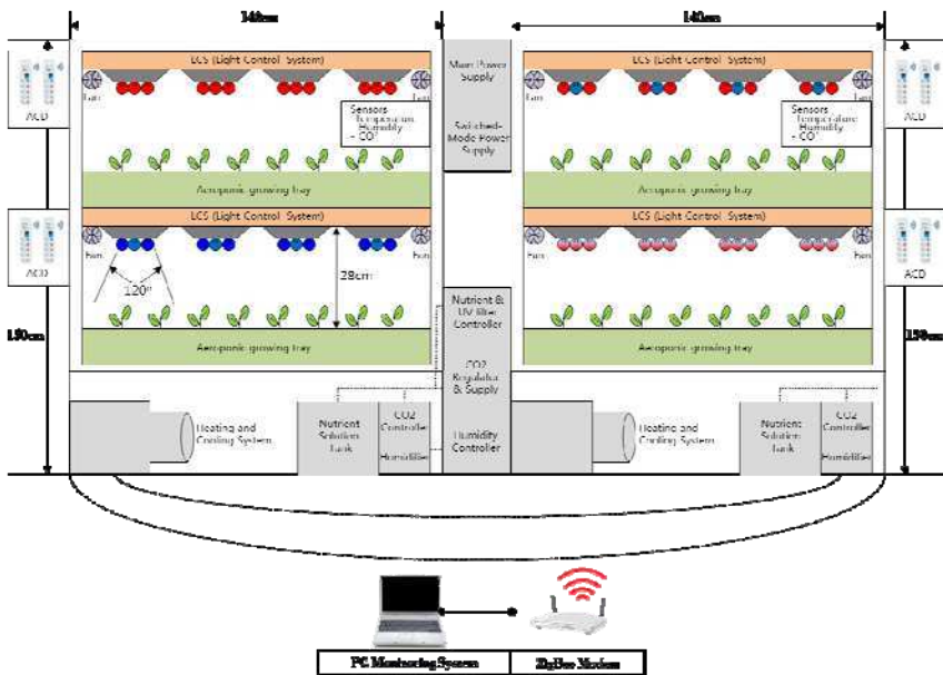
Fig. 1. Plant Cultivation System Building
