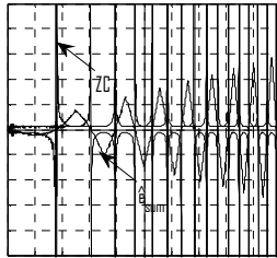
Fig. 9. Waveforms of \hat{e}_{sum} and ZC(\hat{e}_{sum}^*: 10v/div; ZC: 20ms/div; t: 1V/div)
