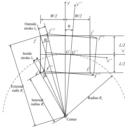
Fig. 3. Curved path stroke
