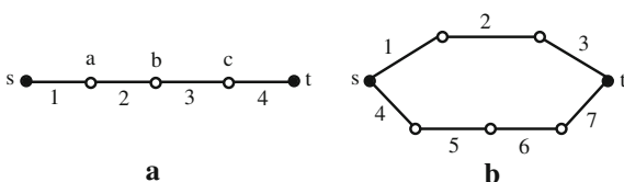
Fig. 1.2 Representation of a series system (a) and parallel connection of series systems (b)
