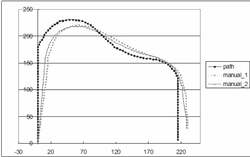
Fig. 8. Tracks of manual mode trials
