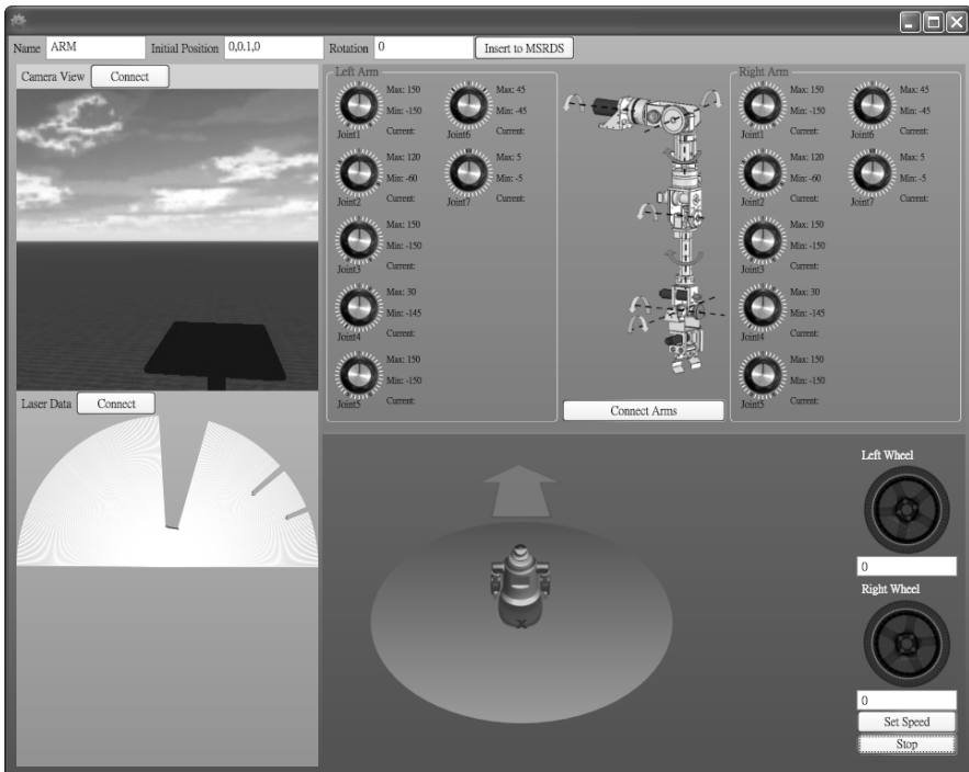
Fig. 8. User interface of the developed robot unit module
