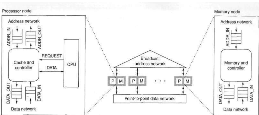
Figure 4.39 Snooping system with switched interconnect.
