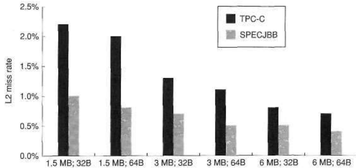
Figure 4.27 Change in the L2 miss rate with variation in cache size and block size. Both TPC-C and SPECJBB are run with all eight cores and four threads per core. Recall that TI has a 3 MB L2 with 64-byte lines.
