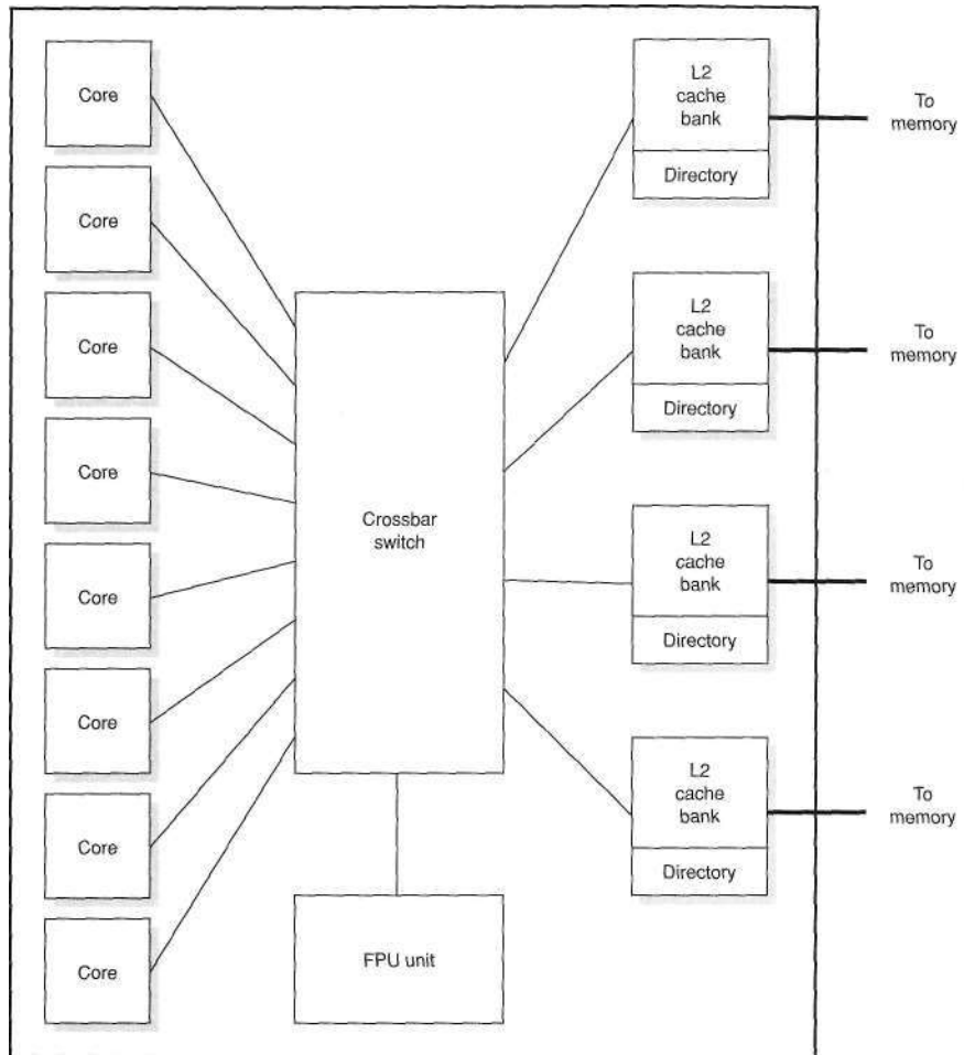
Figure 4.24 The TI processor. Each core supports four threads and has its own level 1 caches (16 KB for instructions and 8 KB for data). The level 2 caches total 3 MB and are effectively 12-way associative. The caches are interleaved by 64-byte cache lines.
