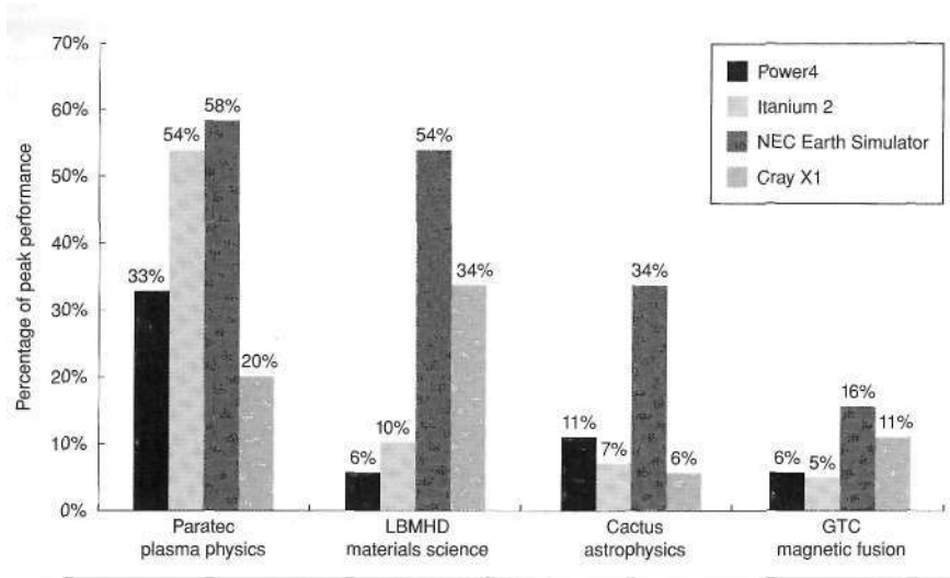
Figure 1.20 Percentage of peak performance for four programs on four multiprocessors scaled to 64 processors. The Earth Simulator and X1 are vector processors. (See Appendix F) Not only did they deliver a higher fraction of peak performance, they had the highest peak performance and the lowest clock rates. Except for the Paratec program, the Power 4 and Itanium 2 systems deliver between 5% and 10% of their peak. From Oliker et al. [2004].
