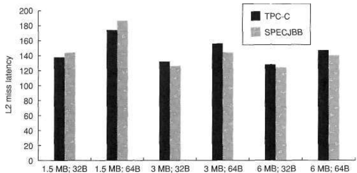
Figure 4.28 The change in the miss latency of the L2 cache as the cache size and block size are changed. Although TPC-C has a significantly higher miss rate, its miss penalty is only slightly higher. This is because SPECJBB has a much higher dirty miss rate, requiring L2 cache lines to be written back with high frequency. Recall that TI has a 3 MB L2 with 64-byte lines.
