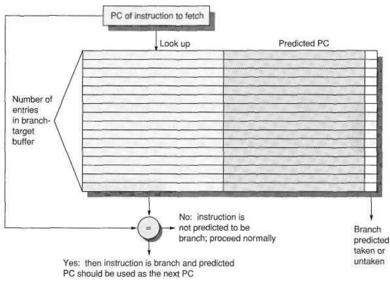
Figure 2.22 A branch-target buffer. The PC of the instruction being fetched is matched against a set of instruction addresses stored in the first column; these represent the addresses of known branches. If the PC matches one of these entries, then the instruction being fetched is a taken branch, and the second field, predicted PC, contains the prediction for the next PC after the branch. Fetching begins immediately at that address. The third field, which is optional, may be used for extra prediction state bits.
