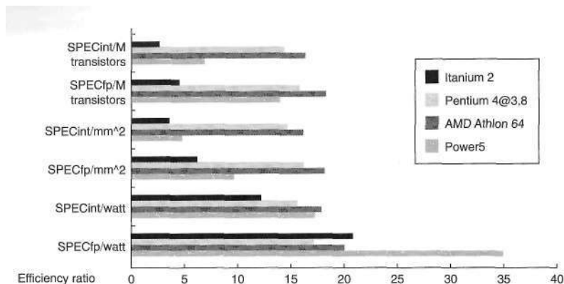
Figure 3.13 Efficiency measures for four multiple-issue processors. In the case of Power5, a single die includes two processor cores, so we estimate the single-core metrics as power = 80 W, area = 290 mm 2 , and transistor count = 200M.
