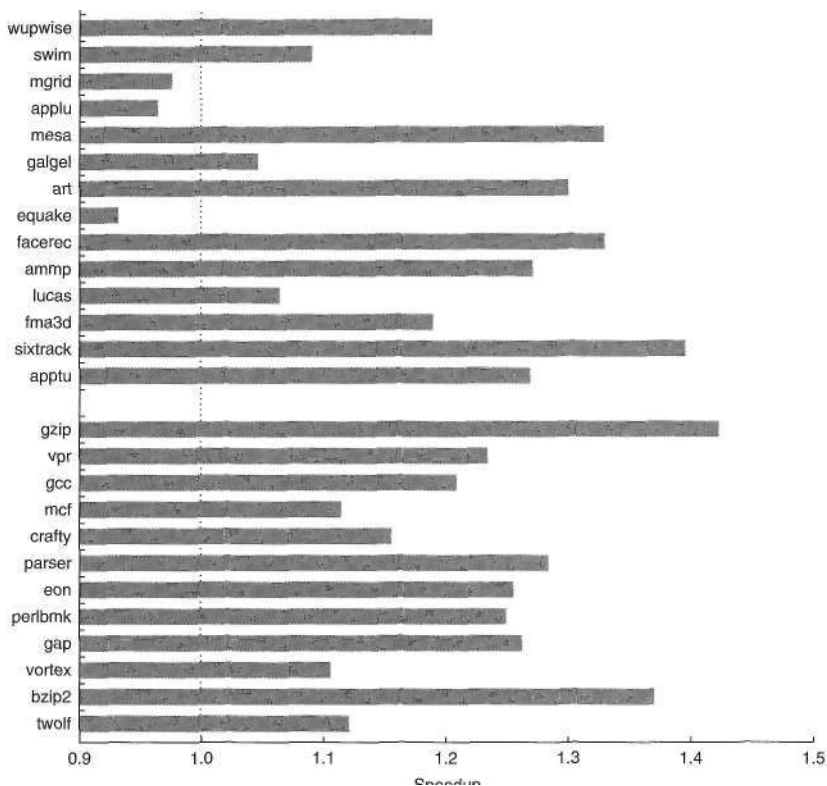
Figure 3.9 A comparison of SMT and single-thread (ST) performance on the 8-processor IBM eServer p5 575.
