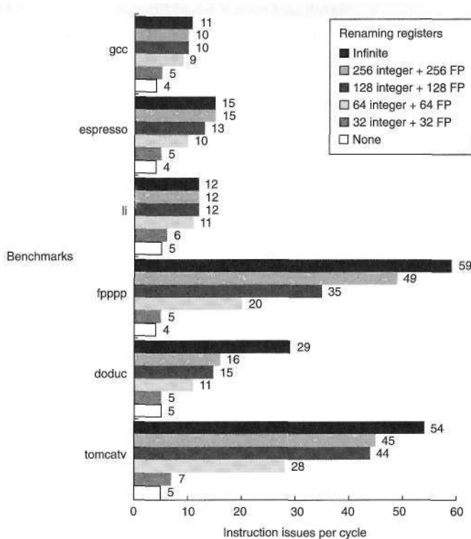
Figure 3.5 The reduction in available parallelism is significant when fewer than an unbounded number of renaming registers are available. Both the number of FP registers and the number of GP registers are increased by the number shown on the x-axis. So, the entry corresponding to "128 integer + 128 FP" has a total of 128 + 128 + 64 = 320 registers (128 for integer renaming, 128 for FP renaming, and 64 integer and FP registers present in the MIPS architecture). The effect is most dramatic on the FP programs, although having only 32 extra integer and 32 extra FP registers has a significant impact on all the programs. For the integer programs, the impact of having more than 64 extra registers is not seen here. To use more than 64 registers requires uncovering lots of parallelism, which for the integer programs requires essentially perfect branch prediction.
