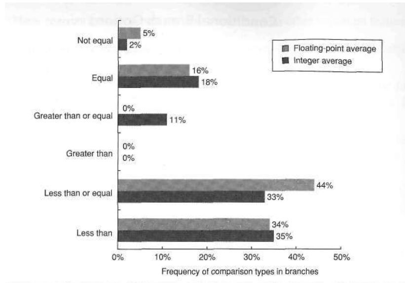
Figure B.17 Frequency of different types of compares in conditional branches. Less than (or equal) branches dominate this combination of compiler and architecture. These measurements include both the integer and floating-point compares in branches. The programs and computer used to collect these statistics are the same as those in Figure B.8.
