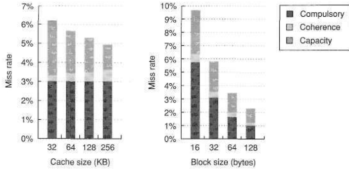
Figure 4.17 The components of the kernel data miss rate change as the LI data cache size is increased from 32 KB to 256 KB, when the multiprogramming workload is run on eight processors. The compulsory miss rate component stays constant, since it is unaffected by cache size. The capacity component drops by more than a factor of 2, while the coherence component nearly doubles. The increase in coherence misses occurs because the probability of a miss being caused by an invalidation increases with cache size, since fewer entries are bumped due to capacity. As we would expect, the increasing block size of the LI data cache substantially reduces the compulsory miss rate in the kernel references. It also has a significant impact on the capacity miss rate, decreasing it by a factor of 2.4 over the range of block sizes. The increased block size has a small reduction in coherence traffic, which appears to stabilize at 64 bytes, with no change in the coherence miss rate in going to 128-byte lines. Because there are not significant reductions in the coherence miss rate as the block size increases, the fraction of the miss rate due to coherence grows from about 7% to about 15%.
