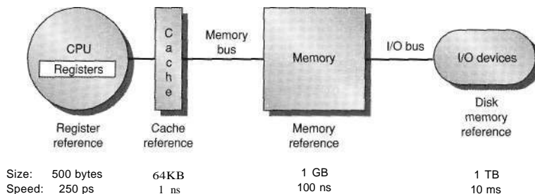
Figure 5.1 The levels in a typical memory hierarchy in embedded, desktop, and server computers. As we move farther away from the processor, the memory in the level below becomes slower and larger. Note that the time units change by factors of 10—from picoseconds to milliseconds—and that the size units change by factors of 1000—from bytes to terabytes.
