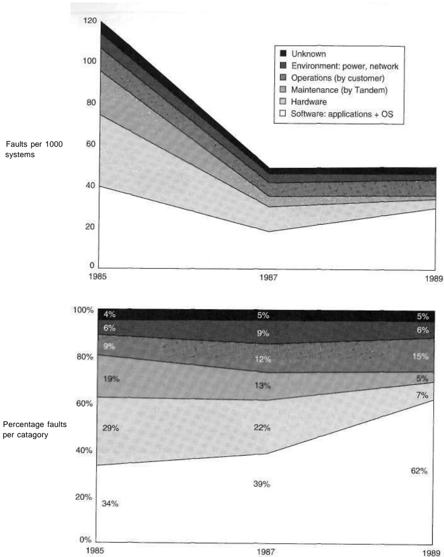
Figure 6.7 Faults in Tandem between 1985 and 1989. Gray [1990] collected these data for the fault-tolerant Tandem computers based on reports of component failures by customers.
