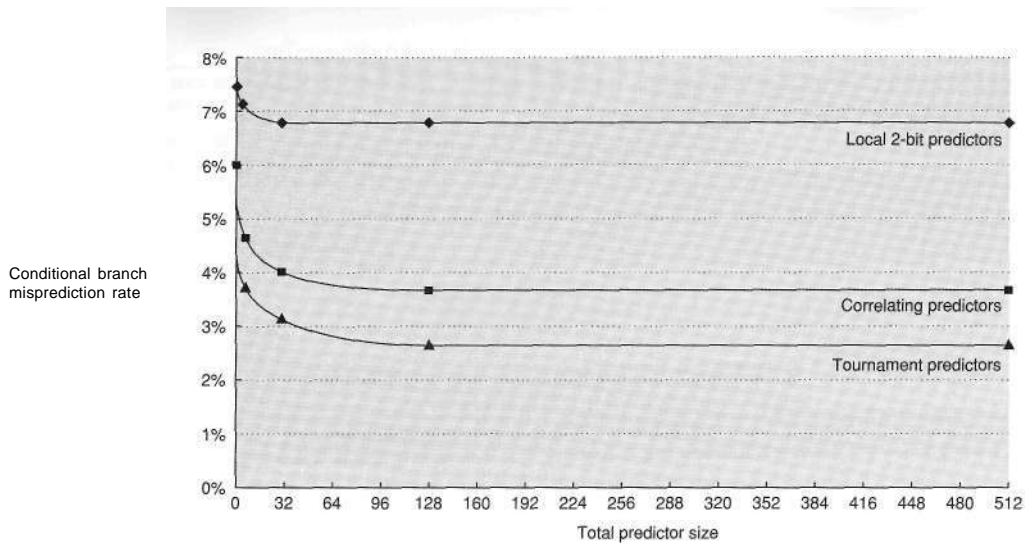
Figure 2.8 The misprediction rate for three different predictors on SPEC89 as the total number of bits is increased. The predictors are a local 2-bit predictor, a correlating predictor, which is optimally structured in its use of global and local information at each point in the graph, and a tournament predictor. Although this data is for an older version of SPEC, data for more recent SPEC benchmarks would show similar behavior, perhaps converging to an asymptotic limit at slightly larger predictor sizes.
