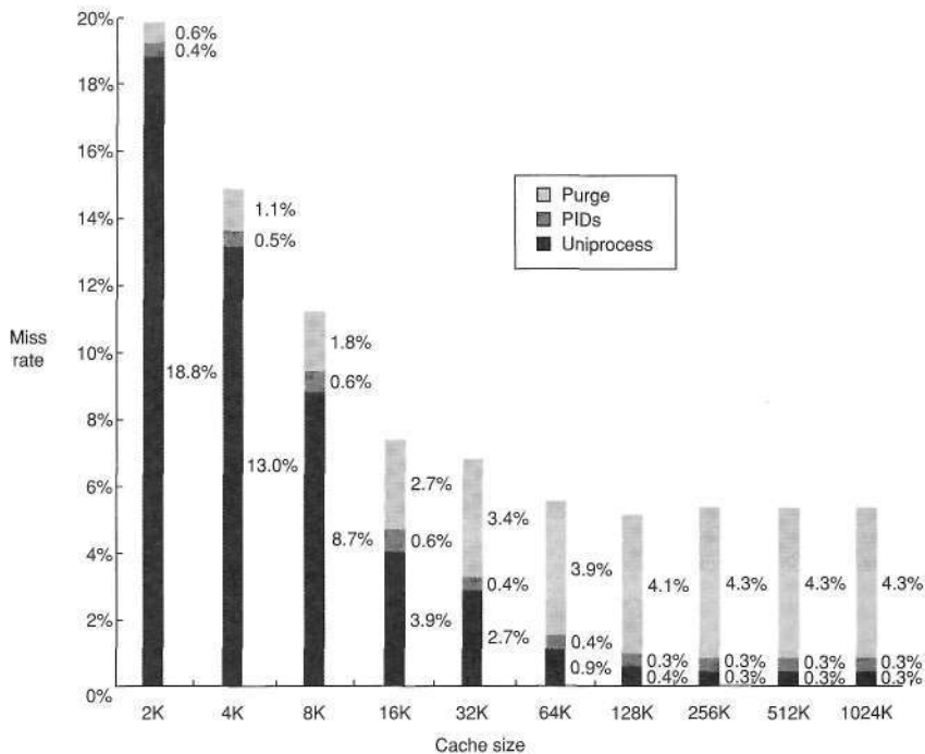
Figure C.16 Miss rate versus virtually addressed cache size of a program measured three ways: without process switches (uniprocess), with process switches using a process-identifier tag (PID), and with process switches but without PIDs (purge). PIDs increase the uniprocess absolute miss rate by 0.3% to 0.6% and save 0.6% to 4.3% over purging. Agarwal [1987] collected these statistics for the Ultrix operating system running on a VAX, assuming direct-mapped caches with a block size of 16 bytes. Note that the miss rate goes up from 128K to 256K. Such nonintuitive behavior can occur in caches because changing size changes the mapping of memory blocks onto cache blocks, which can change the conflict miss rate.
