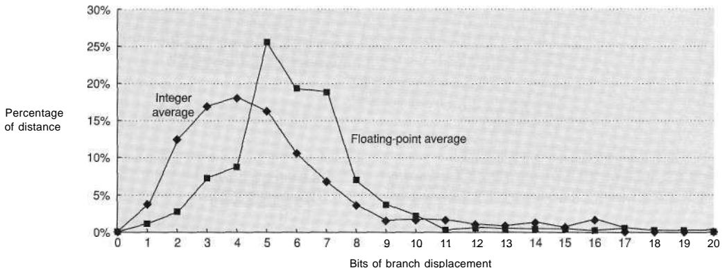
Figure B.15 Branch distances in terms of number of instructions between the target and the branch instruction.
