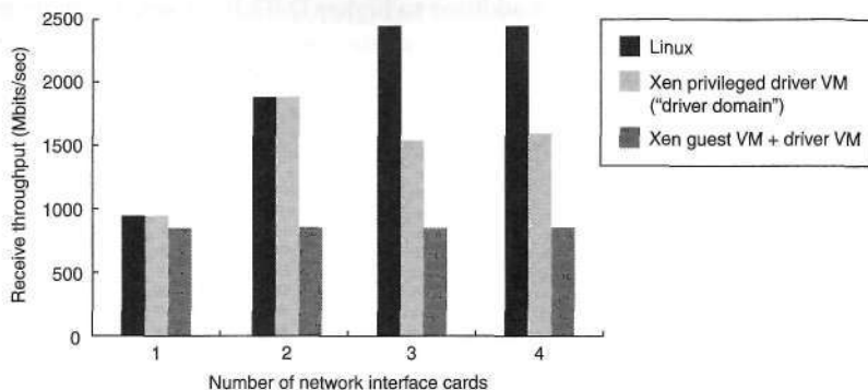
Figure 5.16 TCP receive performance in Mb/s/sec for native Linux versus two configurations of Xen. Guest VM + driver VM is the conventional configuration [Menon et al. 2005]. The experiments were performed on a Dell PowerEdge 1600SC running a 2.4 GHz Xeon server with 1 GB RAM, and four Intel Pro-1000 Gigabit Ethernet NIC, running Linux version 2.6.10 and Xen version 2.0.3.
