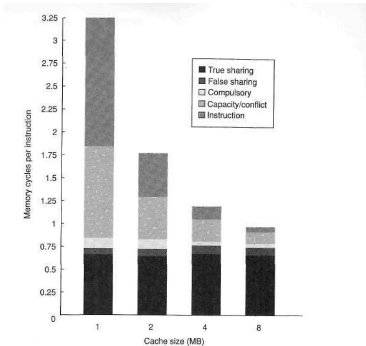
Figure 4.12 The contributing causes of memory access cycles shift as the cache size is increased. The L3 cache is simulated as two-way set associative.
