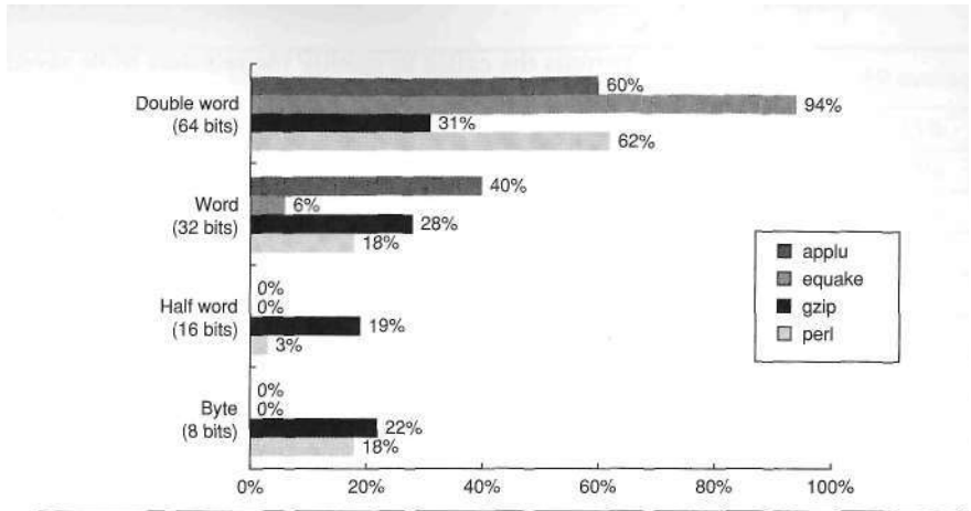
Figure B.29 Data reference size of four programs from SPEC2000. Although you can calculate an average size, it would be hard to claim the average is typical of programs.
