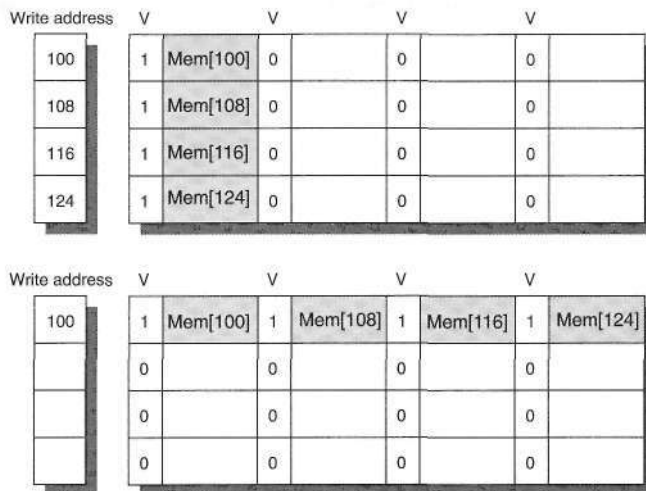
Figure 5.7 To illustrate write merging, the write buffer on top does not use it while the write buffer on the bottom does. The four writes are merged into a single buffer entry with write merging; without it, the buffer is full even though three-fourths of each entry is wasted. The buffer has four entries, and each entry holds four 64-bit words. The address for each entry is on the left, with a valid bit (V) indicating whether the next sequential 8 bytes in this entry are occupied. (Without write merging, the words to the right in the upper part of the figure would only be used for instructions that wrote multiple words at the same time.)
