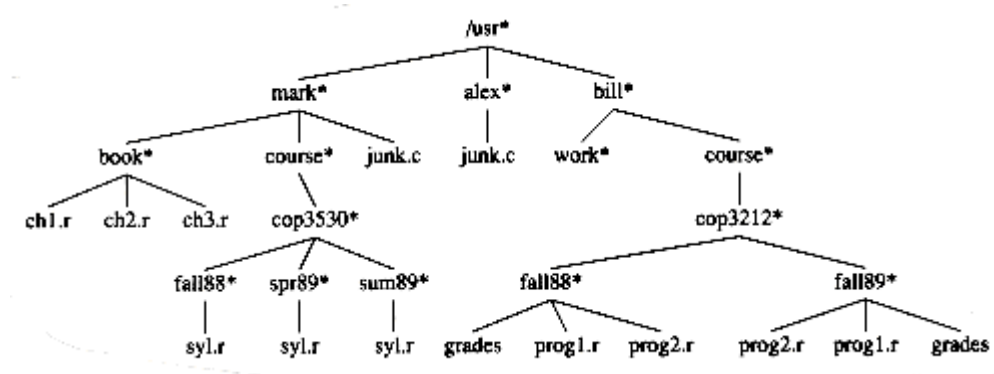
Figure 4.5 Unix directory
