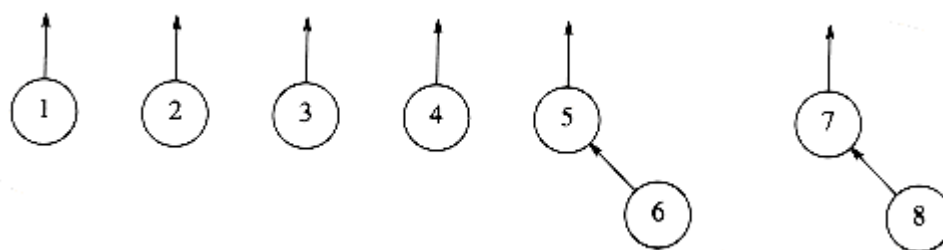
Figure 8.3 After union (7, 8)
