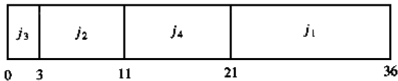
Figure 10.3 Schedule #2 (optimal)
