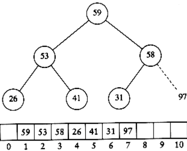
Figure 7.7 Heap after first delete_max
