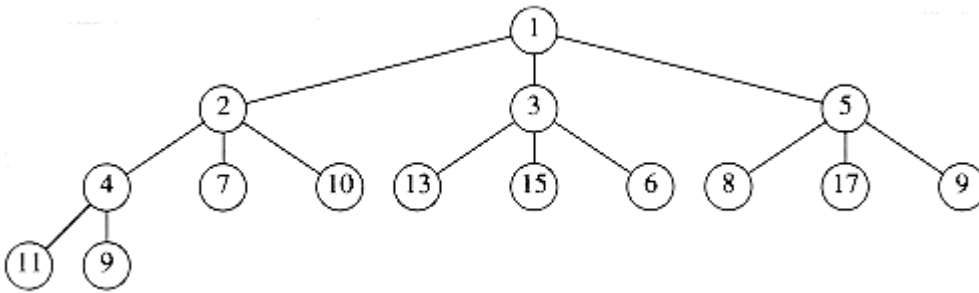
Figure 6.19 A d-heap
