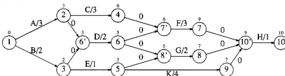
Figure 9.35 Event-node graph
