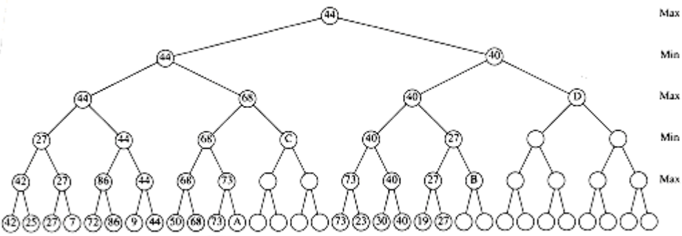
Figure 10.70 A pruned game tree
