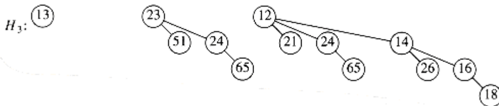
Figure 6.49 Result of \text{delete\_min}(H_3)
