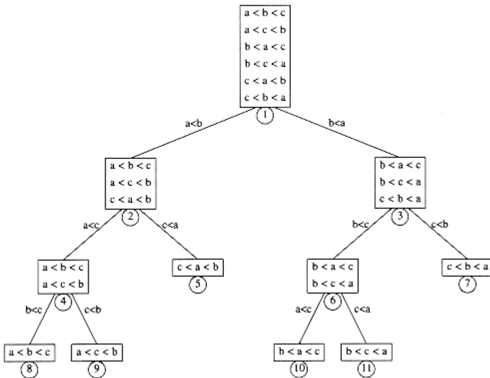
Figure 7.17 A decision tree for three-element insertion sort
