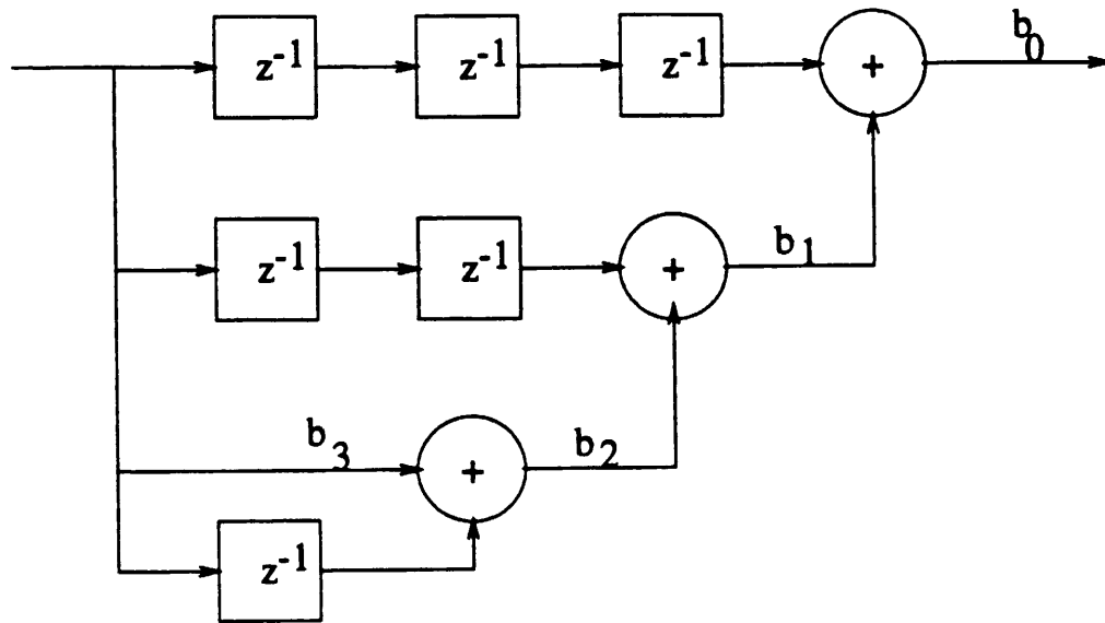
Figure 7.41: Structure of H(z) = b_0 z^{-3} + b_0 b_1 z^{-2} + b_0 b_1 b_2 z^{-1} + b_0 b_1 b_2 b_3
