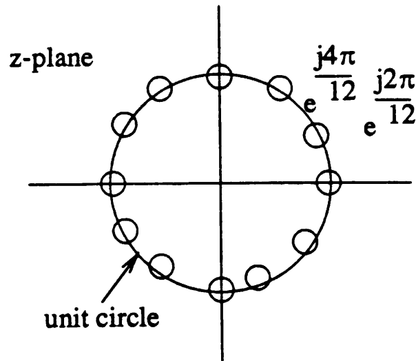
Roots for N=12
