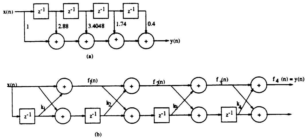
Figure 7.3: (a) Direct form. (b) Lattice form
