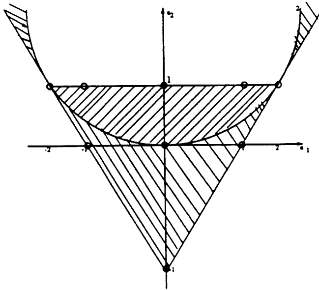
The stable area of (q, a_2)
