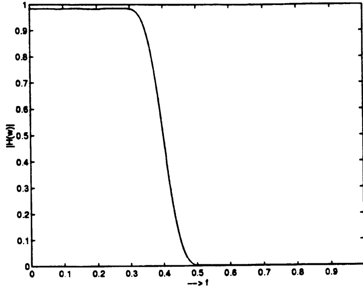
Figure 8.18: M=37 FIR filter designed by window method with Hamming window
