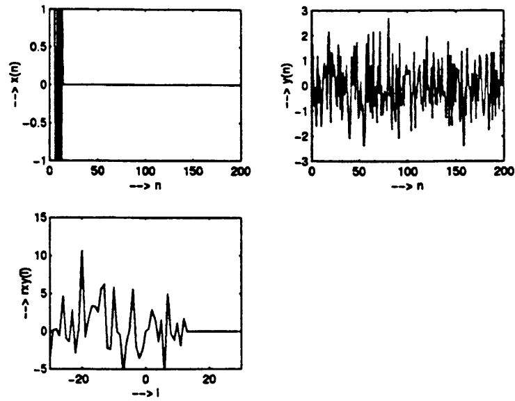
Figure 2.9: variance = 1
