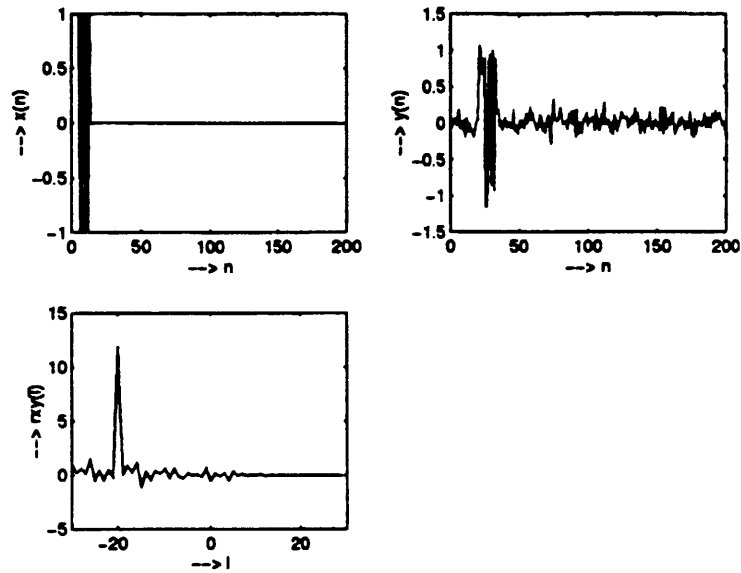
Figure 2.7: variance = 0.01
