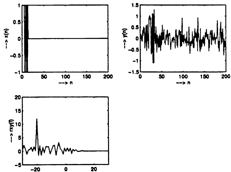
Figure 2.8: variance = 0.1
