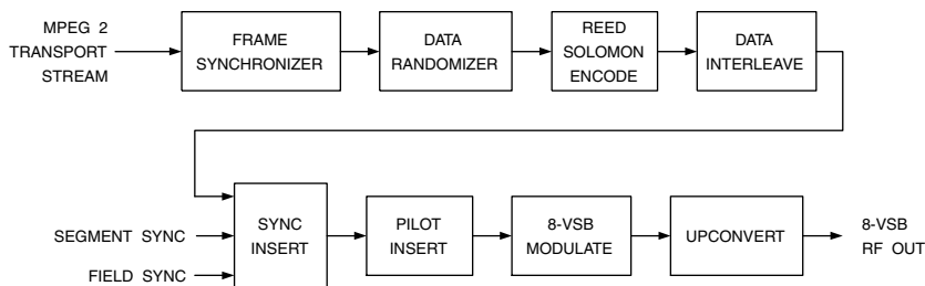
Figure 15.2. Simplified Block Diagram of a 8-VSB Modulator.
