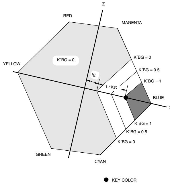
Figure 7.25. Background Key Generation.
