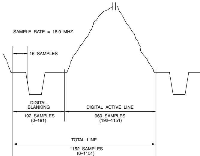
Figure 4.17. 576i Analog - Digital Relationship (16:9 Aspect Ratio, 25 Hz Refresh, 18 MHz Sample Clock).
