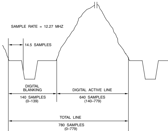
Figure 4.5. 480i Analog - Digital Relationship (4:3 Aspect Ratio, 29.97 Hz Refresh, 12.27 MHz Sample Clock).
