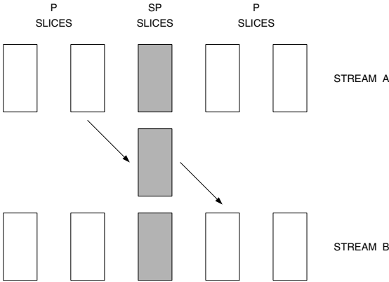
Figure 14.6. Using SP Slices to Switch to Another Stream.
