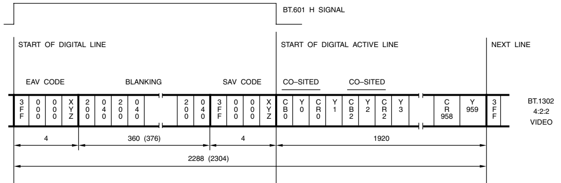
Figure 6.10. BT.1302 and SMPTE 267M Parallel Interface Data For One Scan Line. 480i; 4:2:2 YCbCr; 960 active samples per line; 36 MHz clock; 10-bit system. The values for 576i systems are shown in parentheses.
