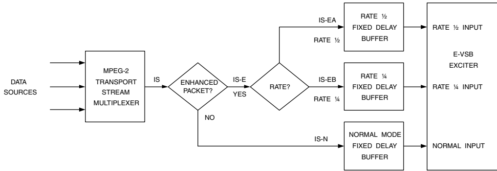
Figure 15.3. ATSC E-VSBS Head-end Model.
