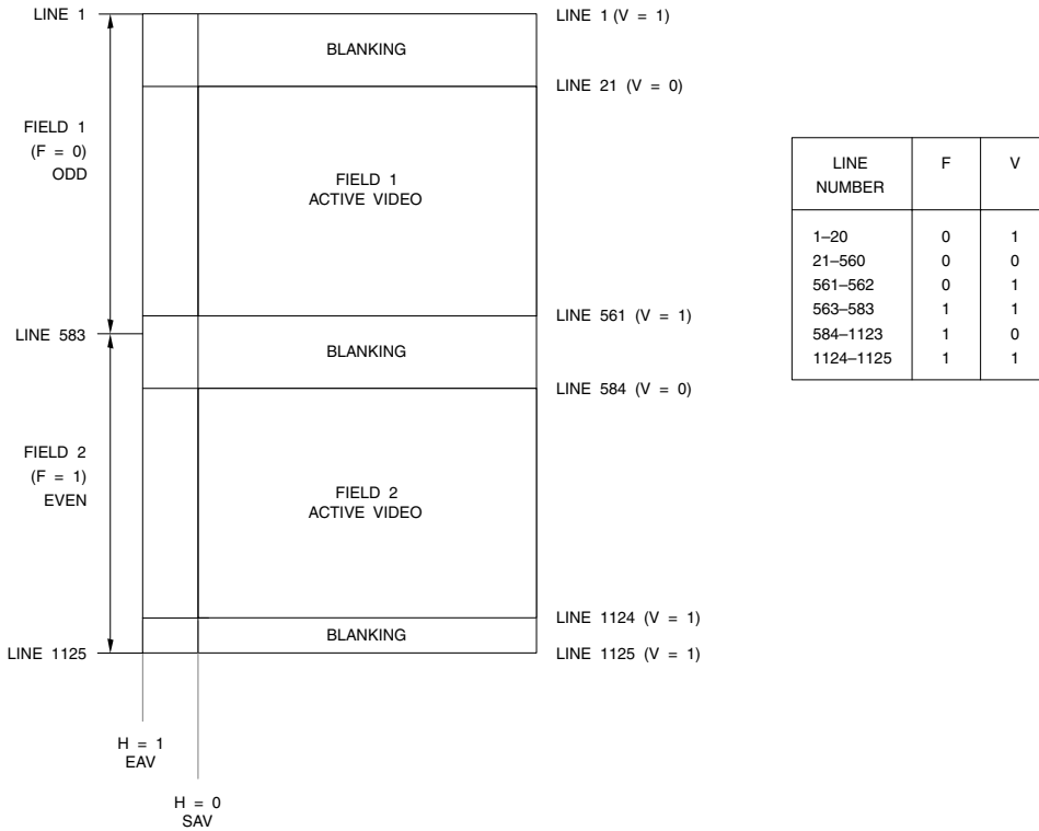
Figure 4.34. 1080i Digital Vertical Timing (1080 Active Lines). F and V change state at the EAV sequence at the beginning of the digital line. Note that the digital line number changes state prior to start of horizontal sync, as shown in Figures 4.32 and 4.33.
