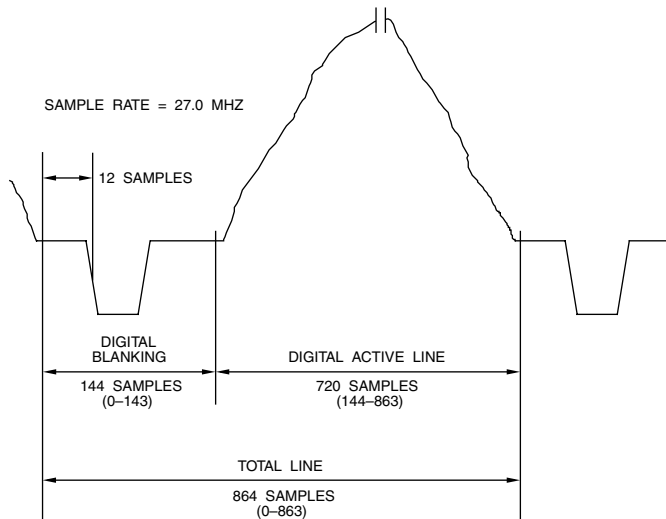
Figure 4.21. 576p Analog - Digital Relationship (4:3 Aspect Ratio, 50 Hz Refresh, 27 MHz Sample Clock).
