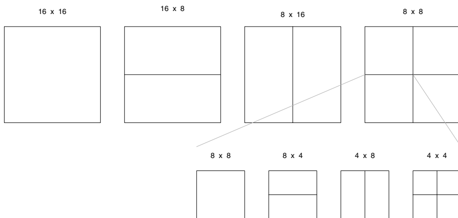
Figure 14.5. Segmentations of H.264 Macroblocks for Motion Compensation. Top: segmentation of macroblocks. Bottom: segmentation of 8 × 8 partitions.
