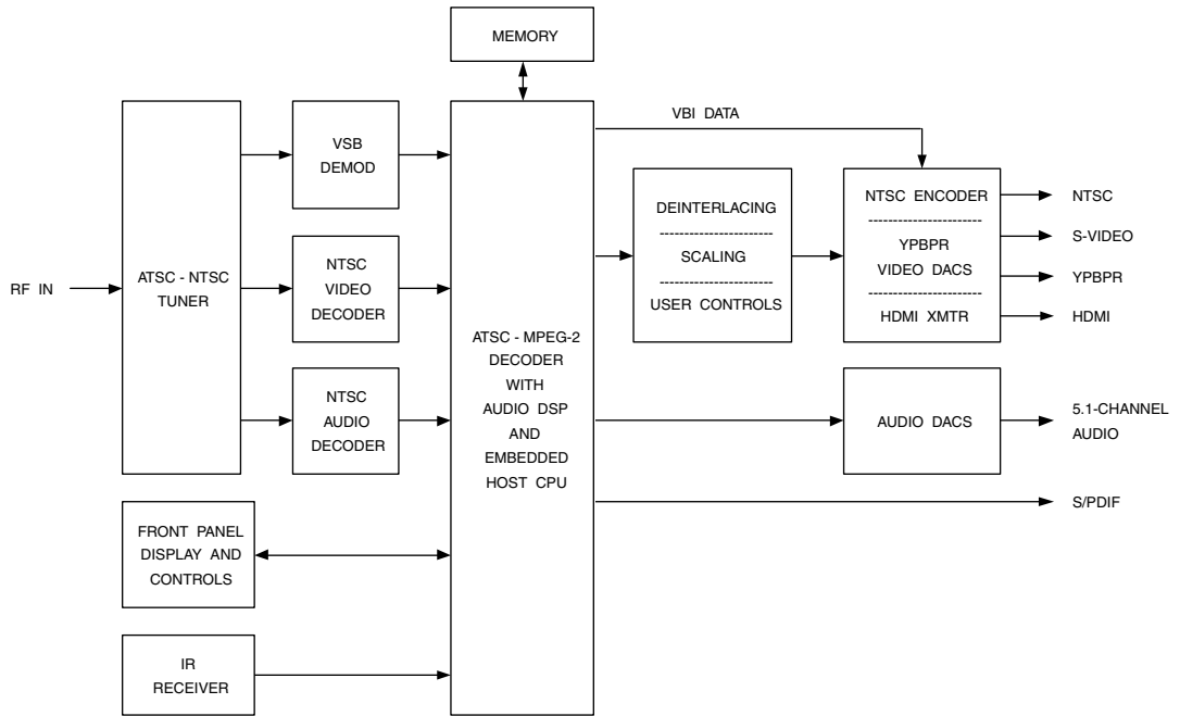
Figure 15.5. Typical ATSC Receiver Set-top Box Block Diagram.
