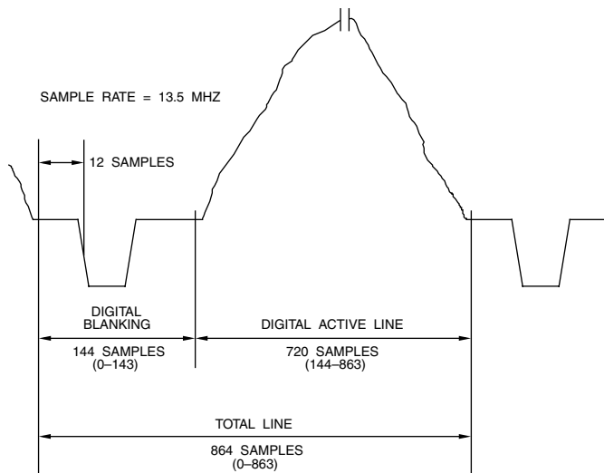
Figure 4.16. 576i Analog - Digital Relationship (4:3 Aspect Ratio, 25 Hz Refresh, 13.5 MHz Sample Clock).
