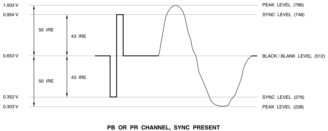
Figure 5.11. SMPTE 274M and 296M HDTV Analog YPbPr Levels. Sync on YPbPr.
