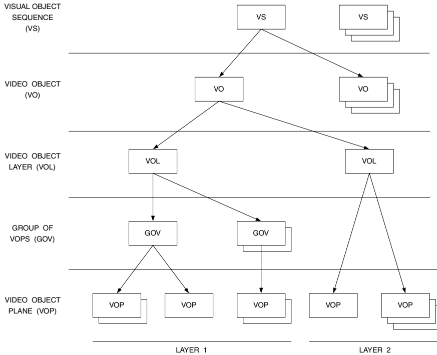
Figure 14.1. Example MPEG-4 Video Bitstream Logical Structure.
