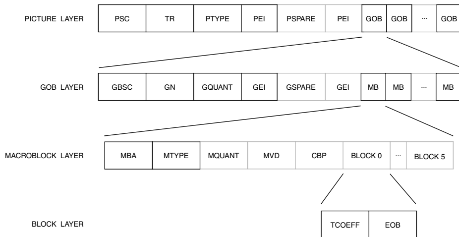
Figure 10.6. H.261 Video Bitstream Layer Structures.
