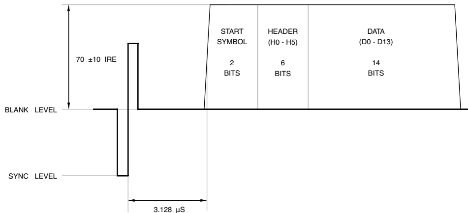
Figure 5.12. EIA-805 and EIA-J CPR-1204-2 720p Line 24 CGMS Timing.
