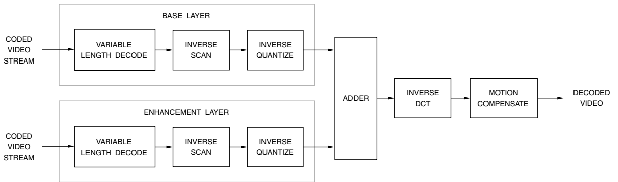
Figure 13.32. Simplified MPEG-2 SNR Scalability Decoder Block Diagram.
