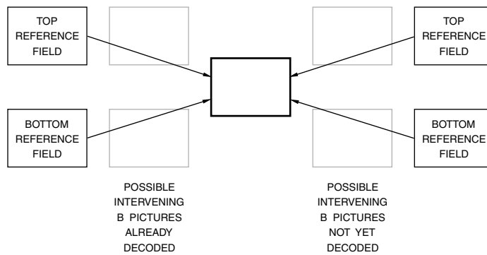
Figure 13.18. Field Prediction of B Field or Frame Pictures.
