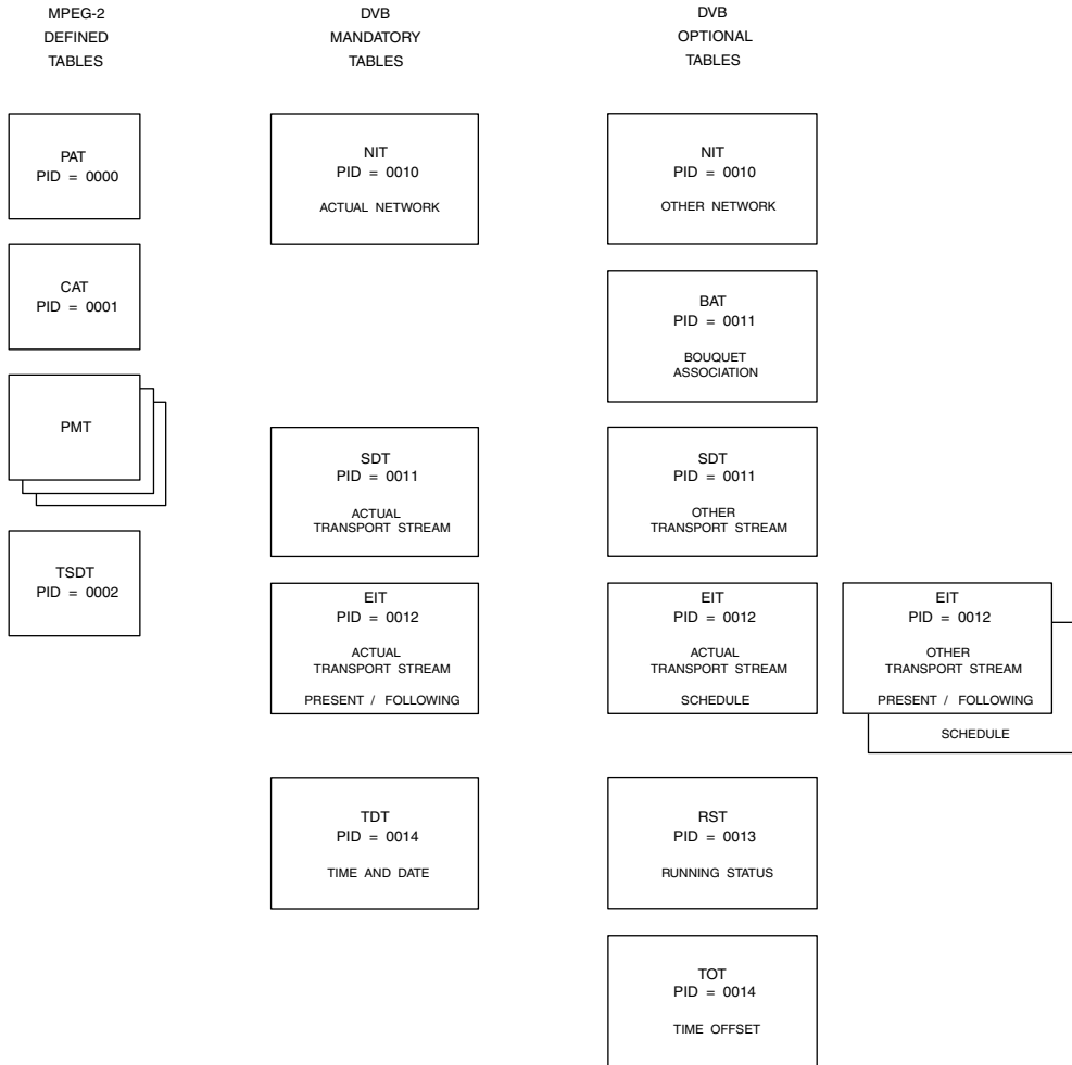
Figure 17.1. DVB SI Table Relationships.
