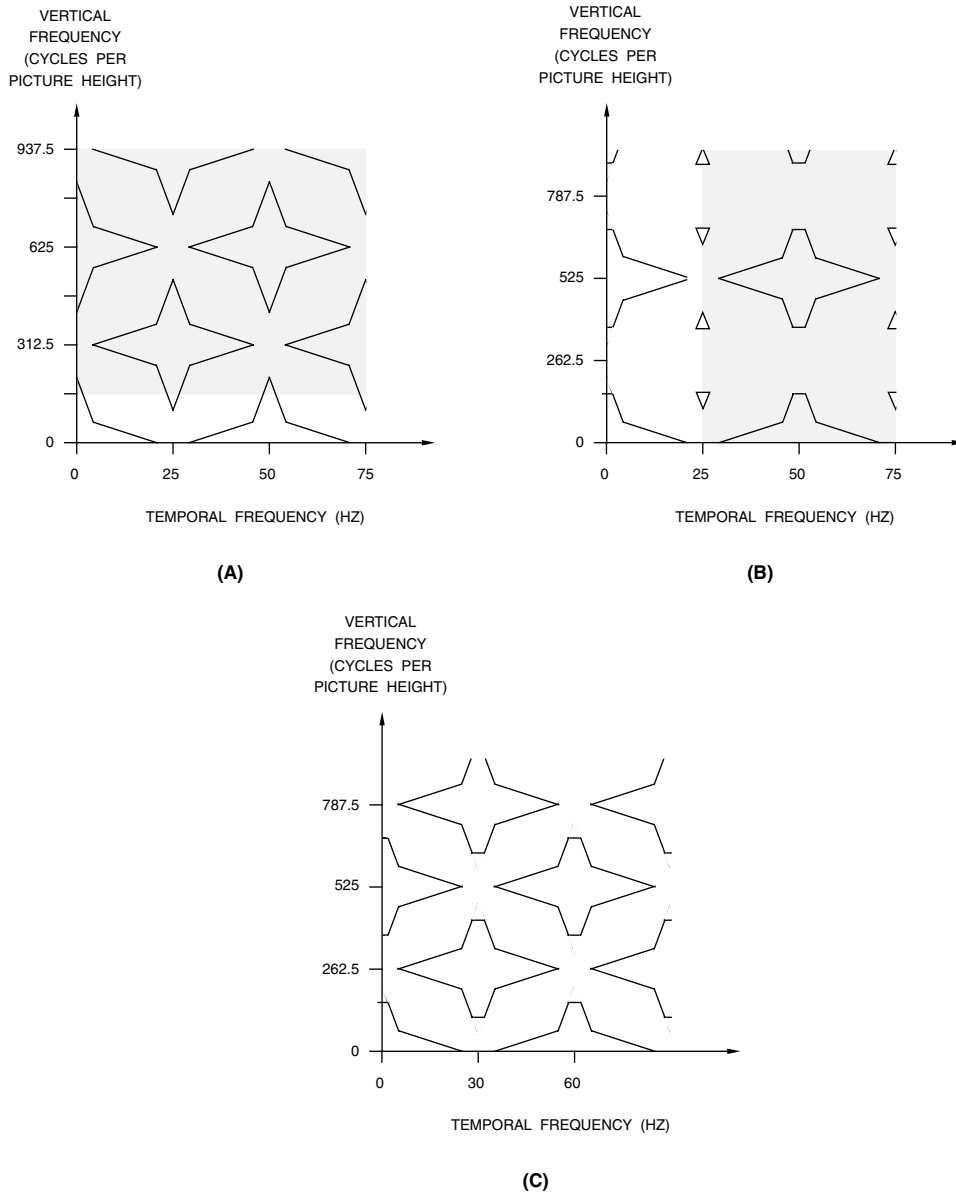
Figure 7.42. Spectral Representation of Vertical, Followed by Temporal, Interpolation. (a) Vertical lowpass filtering. (b) Resampling to intermediate sequential format and temporal lowpass filtering. (c) Resampling to final standard.
