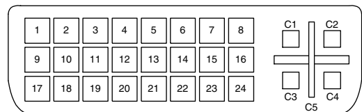
Figure 6.47. DVI-I Connector.
