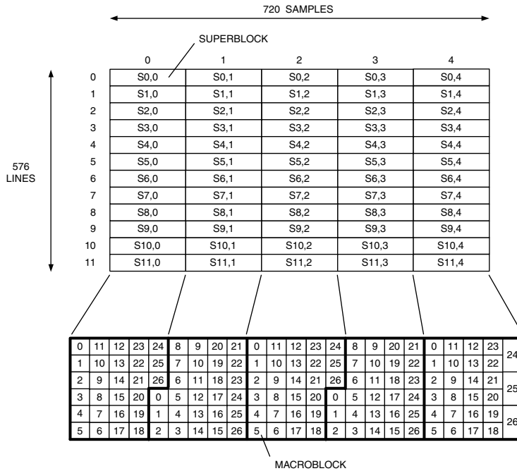
Figure 11.10. Relationship Between Super Blocks and Macroblocks (4:1:1 YCbCr, 720 × 576i).
