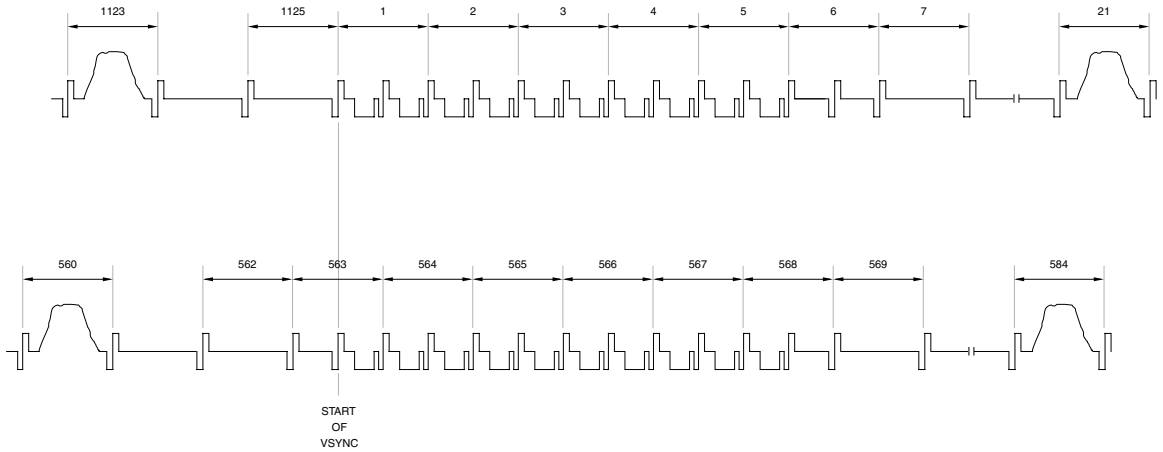
Figure 4.30. 1080i Vertical Interval Timing.
