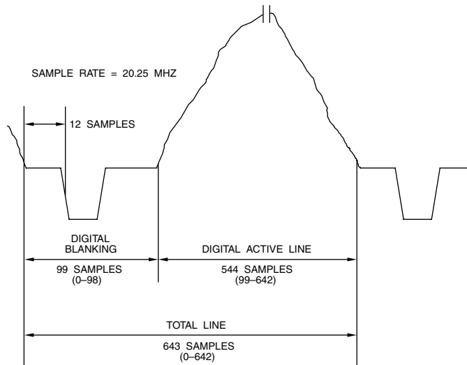
Figure 4.12. 480p Analog - Digital Relationship (4:3 Aspect Ratio, 59.94 Hz Refresh, 20.25 MHz Sample Clock).
