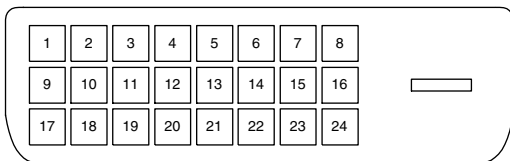
Figure 6.46. DVI-D Connector.
