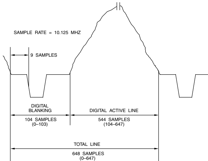
Figure 4.19. 576i Analog - Digital Relationship (4:3 Aspect Ratio, 25 Hz Refresh, 10.125 MHz Sample Clock).
