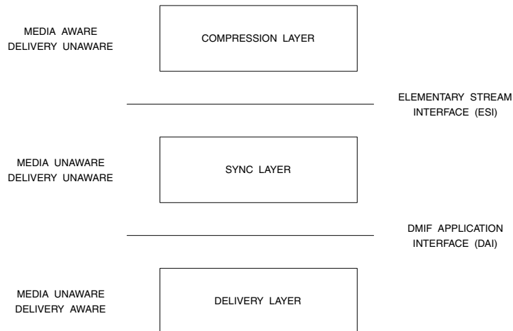
Figure 14.4. Relationship Between the MPEG-4 Compression, Sync and Delivery Layers.
