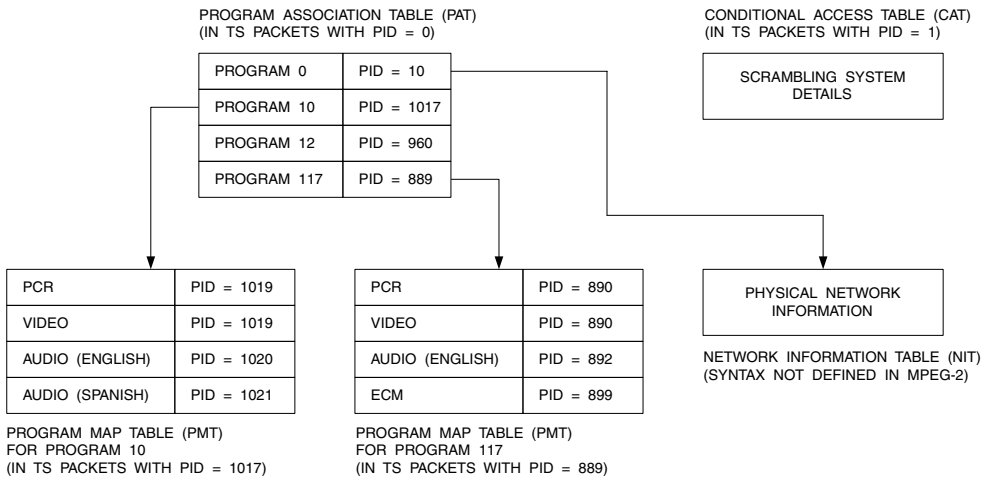
Figure 13.24. MPEG-2 PAT and PMT Example.
