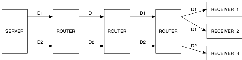
Figure 19.3. Multicast Example. One copy of the same data (D1) is multicast to receivers 1 and 2. Note the bandwidth savings locally and across the networks as the number of receivers increases.
