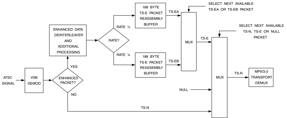
Figure 15.4. ATSC E-VSBS Receiver Model.
