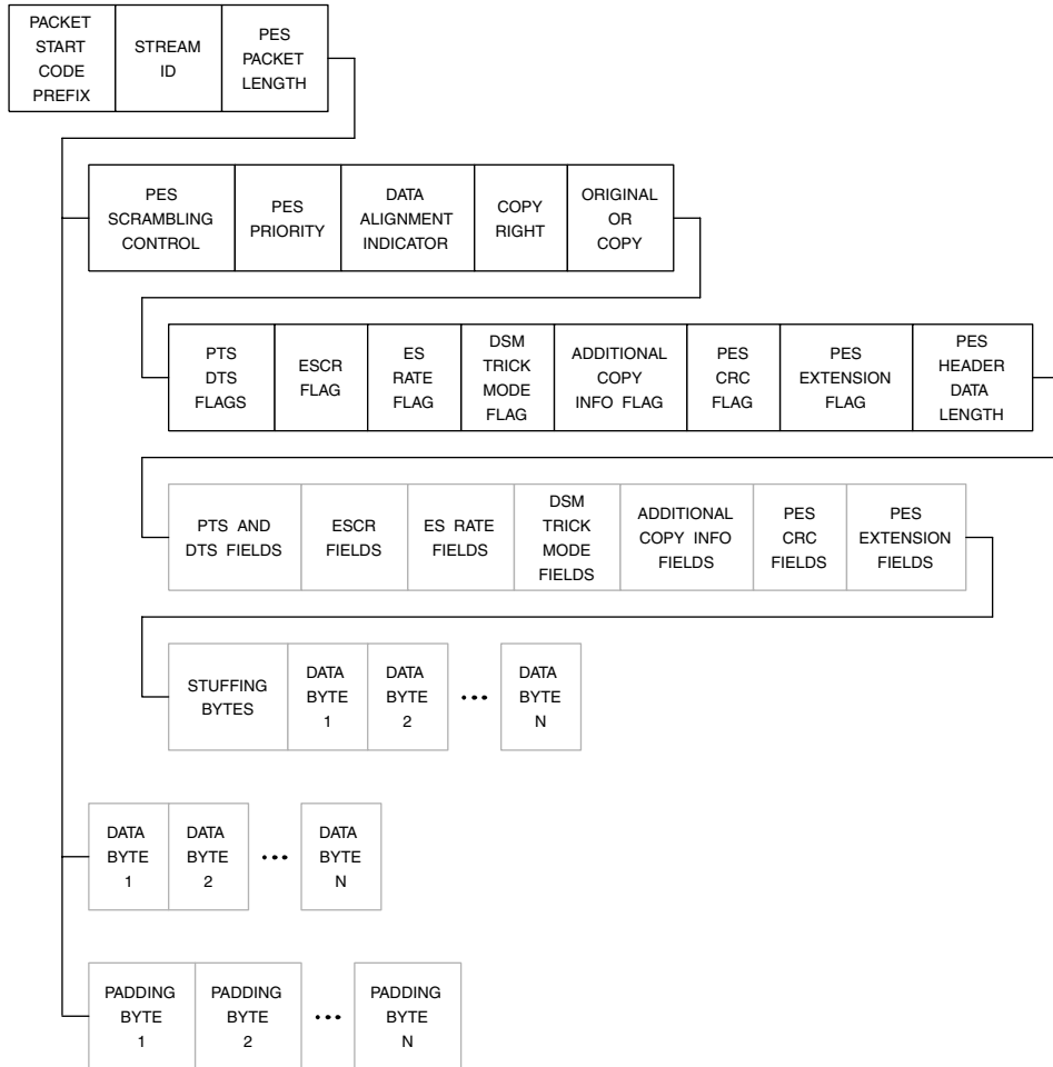
Figure 13.21. MPEG-2 PES Packet Structure. Marker and reserved bits not shown.
