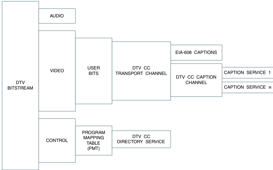
Figure 13.25. DTV Closed Captioning Data in MPEG-2 Bitstream.
