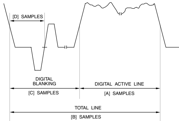
Figure 4.33. General 1080i Analog - Digital Relationship.
