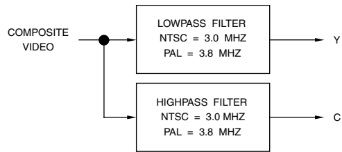
Figure 9.34. Typical Simple Y/C Separator.
