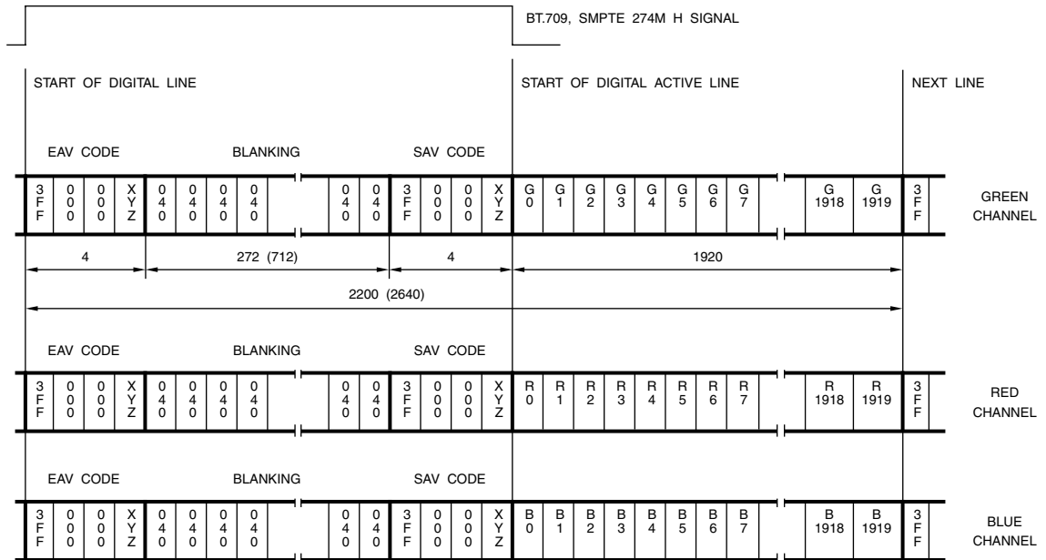
Figure 6.18. BT.1120 and SMPTE 274M Parallel Interface Data For One Scan Line. 1080i; 29.97-, 30-, 59.94-, and 60-Hz systems; R'G'B'; 1920 active samples per line; 74.176, 74.25, 148.35, or 148.5 MHz clock; 10-bit system. The values for 25- and 50-Hz systems are shown in parentheses.
