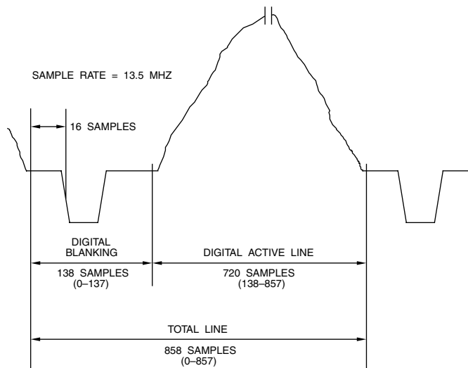
Figure 4.3. 480i Analog - Digital Relationship (4:3 Aspect Ratio, 29.97 Hz Refresh, 13.5 MHz Sample Clock).
