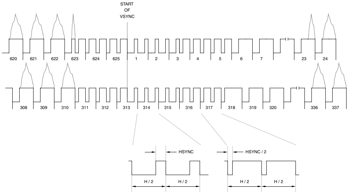
Figure 4.14. 576i Vertical Interval Timing.
