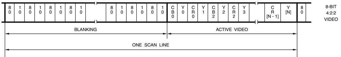
Figure 6.37. 8-Bit 4:2:2 YCbCr Data Format.
