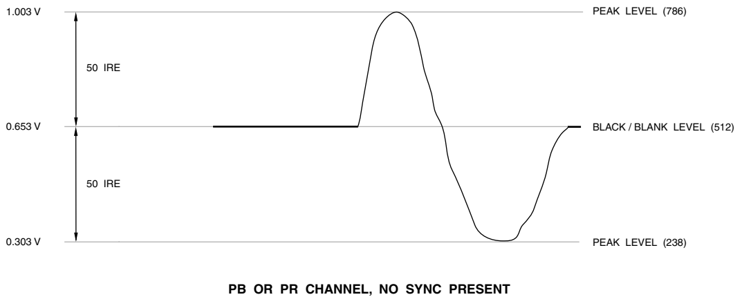
Figure 5.10. EIA-770.3 HDTV Analog YPbPr Levels. Sync on Y.
