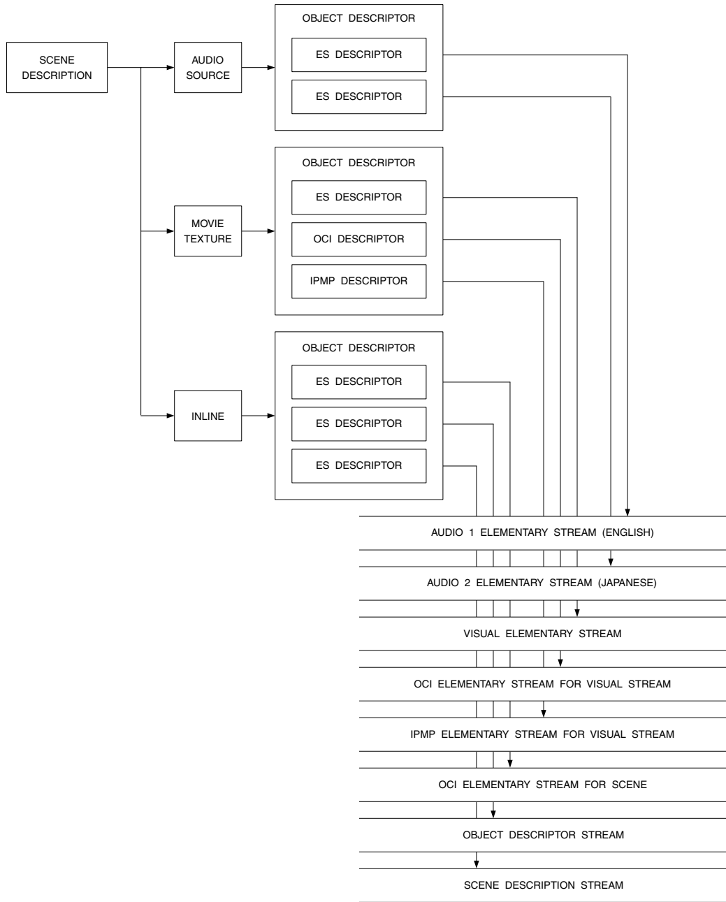
Figure 14.2. Linking Elementary Streams to a Scene.
