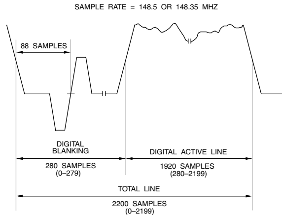
Figure 4.35. 1080p Analog - Digital Relationship (16:9 Aspect Ratio, 59.94 Hz Refresh, 148.35 MHz Sample Clock and 60 Hz Refresh, 148.5 MHz Sample Clock).
