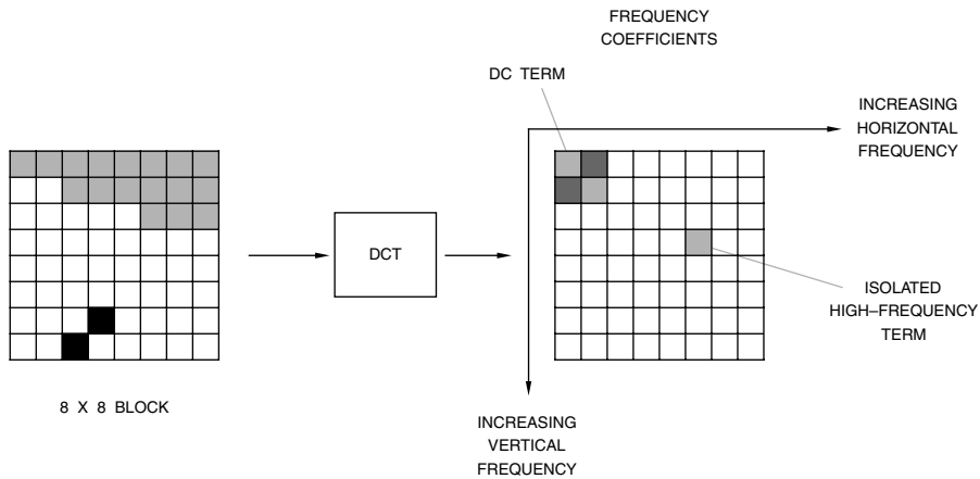
Figure 7.56. The DCT Processes the 8 × 8 Block of Samples or Error Terms to Generate an 8 × 8 Block of DCT Coefficients.
