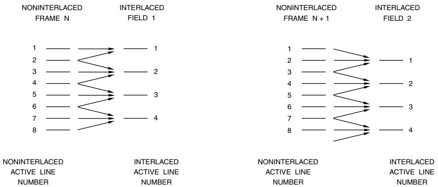
Figure 7.48. Noninterlaced-to-Interlaced Conversion Using 3-Line Vertical Filtering.
