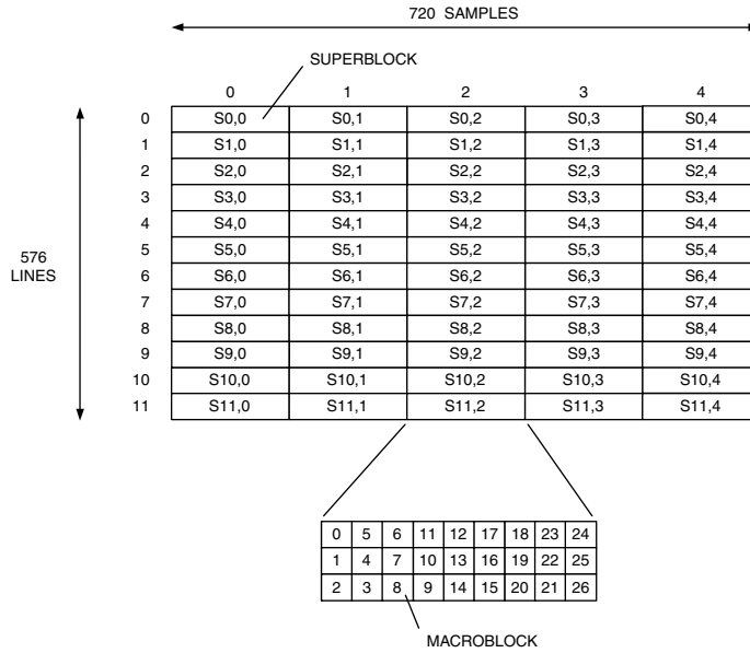
Figure 11.9. Relationship Between Super Blocks and Macroblocks (4:2:0 YCbCr, 720 × 576i).
