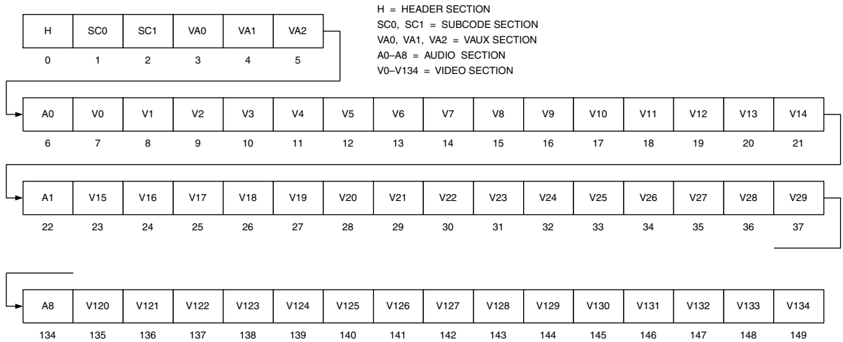
Figure 11.15. DIF Sequence Detail.
