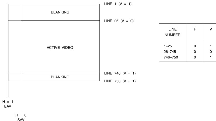
Figure 4.29. 720p Digital Vertical Timing (720 Active Lines). V changes state at the EAV sequence at the beginning of the digital line. Note that the digital line number changes state prior to start of horizontal sync, as shown in Figures 4.27 and 4.28.
