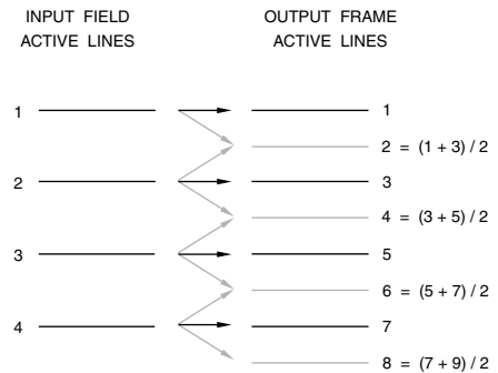
Figure 7.50. Deinterlacing Using Scan Line Interpolation. New scan lines are generated by averaging the previous and next active scan lines.
