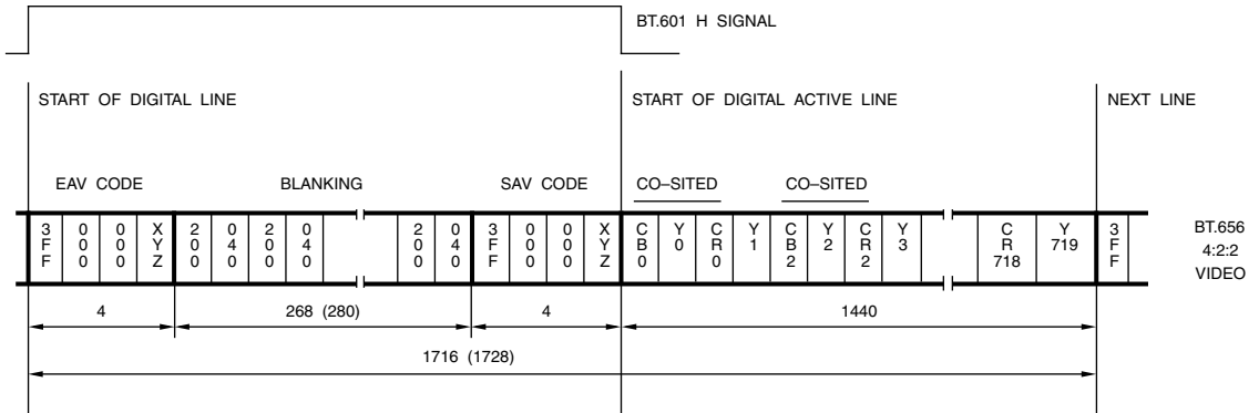
Figure 6.9. BT.656 and SMPTE 125M Parallel Interface Data For One Scan Line. 480i; 4:2:2 YCbCr; 720 active samples per line; 27 MHz clock; 10-bit system. The values for 576i systems are shown in parentheses.
