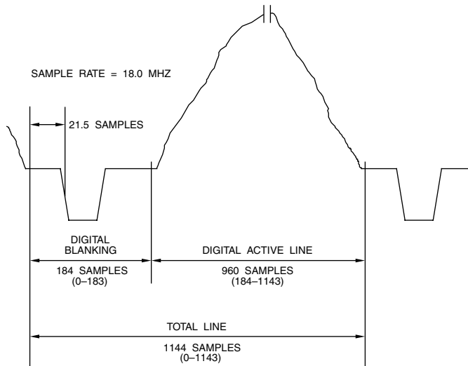
Figure 4.4. 480i Analog - Digital Relationship (16:9 Aspect Ratio, 29.97 Hz Refresh, 18 MHz Sample Clock).
