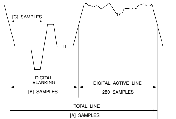
Figure 4.28. General 720p Analog - Digital Relationship.
