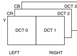
Figure 11.4. 4:2:2 Macroblock Arrangement.
