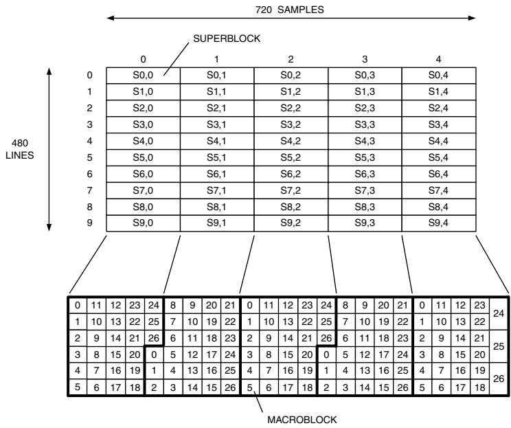
Figure 11.7. Relationship Between Super Blocks and Macroblocks (4:1:1 YCbCr, 720 × 480i).
