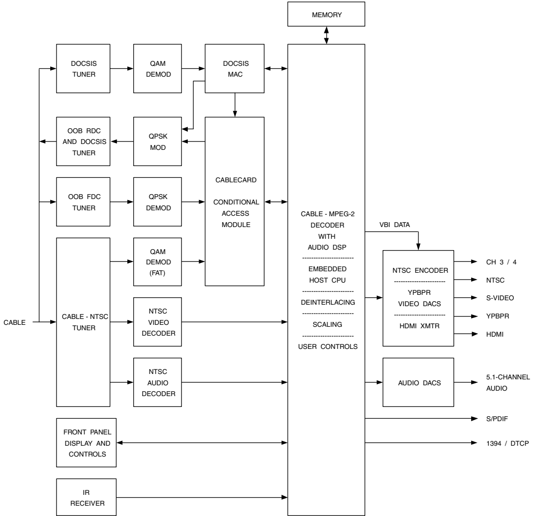
Figure 16.2. OpenCable™ Receiver Set-top Box Block Diagram.
