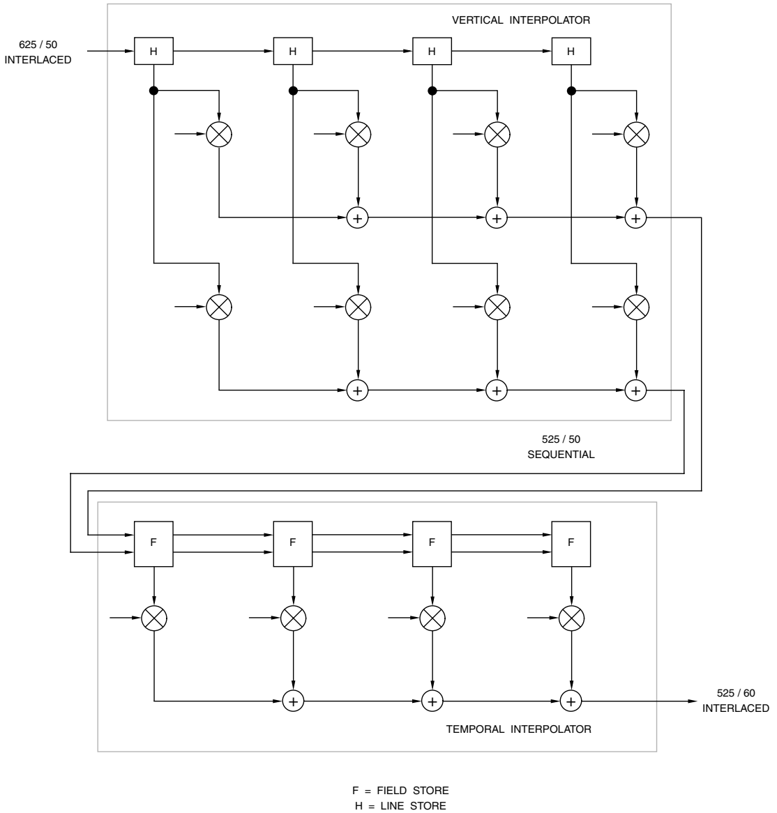
Figure 7.41. Typical 625/50 to 525/60 Conversion Using Vertical, Followed by Temporal, Interpolation.
