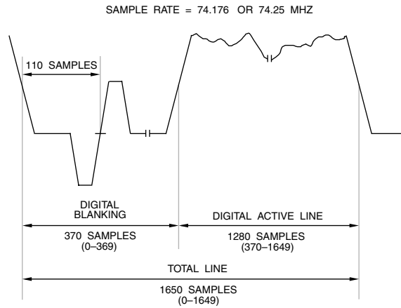
Figure 4.27. 720p Analog - Digital Relationship (16:9 Aspect Ratio, 59.94 Hz Refresh, 74.176 MHz Sample Clock and 60 Hz Refresh, 74.25 MHz Sample Clock).
