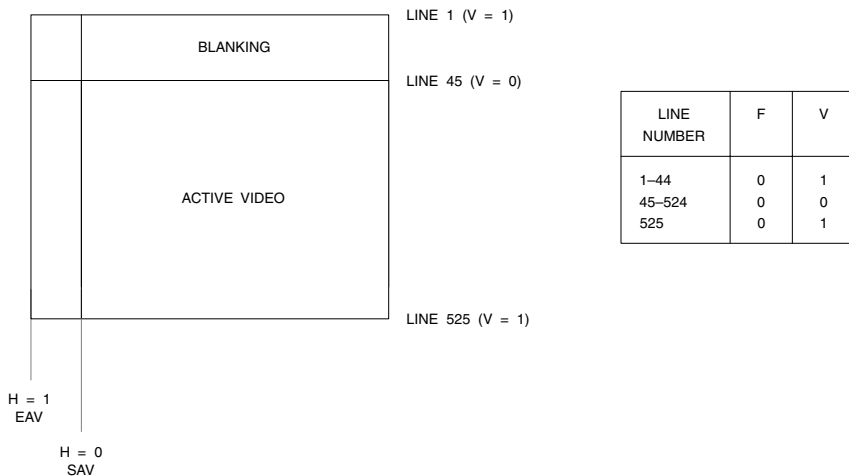
Figure 4.13. 480p Digital Vertical Timing (480 Active Lines). V changes state at the EAV sequence at the beginning of the digital line. Note that the digital line number changes state prior to start of horizontal sync, as shown in Figures 4.9 through 4.12.
