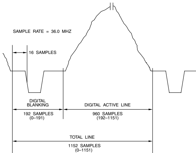
Figure 4.22. 576p Analog - Digital Relationship (16:9 Aspect Ratio, 50 Hz Refresh, 36 MHz Sample Clock).
