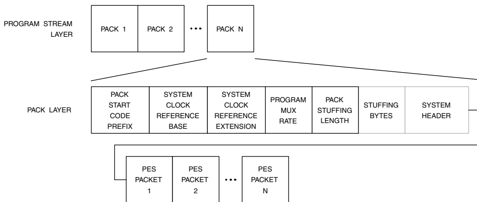
Figure 13.22. MPEG-2 Program Stream Structure. Marker and reserved bits not shown.
