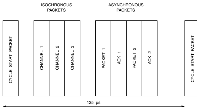
Figure 6.56. IEEE 1394 Isochronous and Asynchronous Packets.
