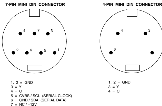
Figure 5.1. S-Video Connector and Signal Names.
