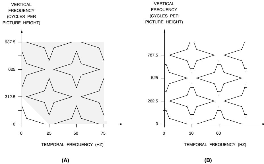
Figure 7.44. Spectral Representation of Combined Vertical and Temporal Interpolation. (a) Two-dimensional lowpass filtering. (b) Resampling to final standard.
