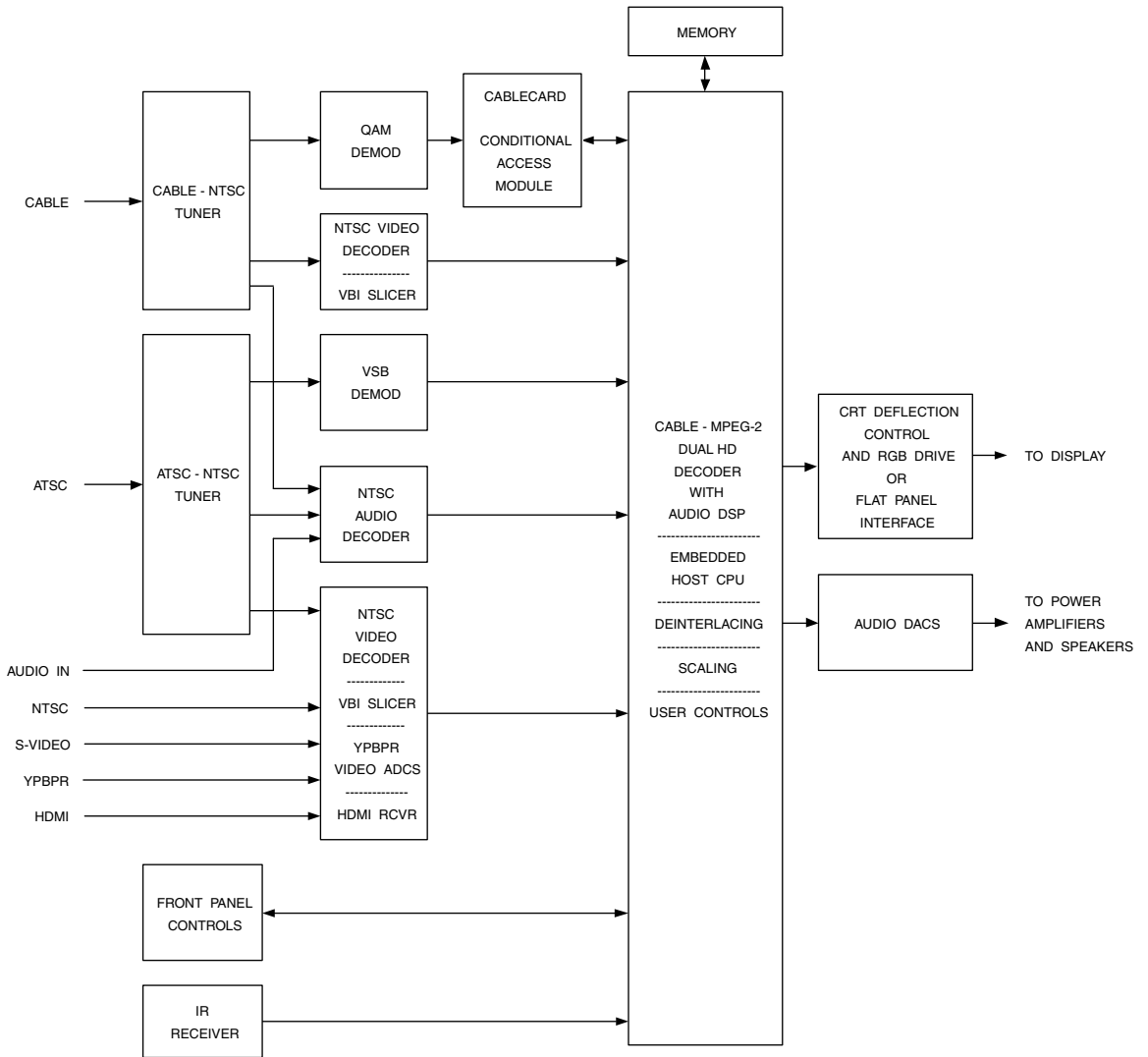
Figure 16.3. OpenCable™ Receiver Inside a Digital Television
