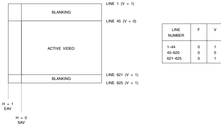
Figure 4.25. 576p Digital Vertical Timing (576 Active Lines). V changes state at the EAV sequence at the beginning of the digital line. Note that the digital line number changes state prior to start of horizontal sync, as shown in Figures 4.21 through 4.24.
