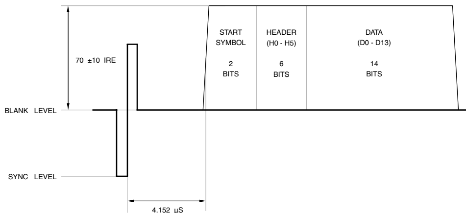
Figure 5.13. EIA-805 and EIA-J CPR-1204-2 1080i Lines 19 and 582 CGMS Timing.
