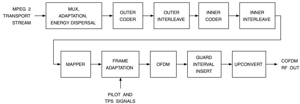
Figure 17.2. Simplified Block Diagram of a COFDM Modulator.
