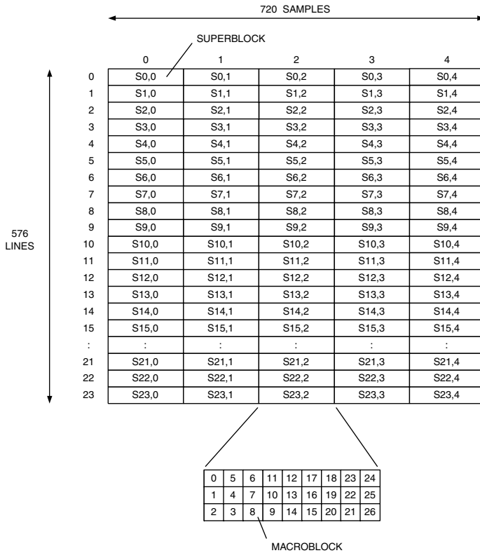
Figure 11.11. Relationship Between Super Blocks and Macroblocks (4:2:2 YCbCr, 720 × 576i).
