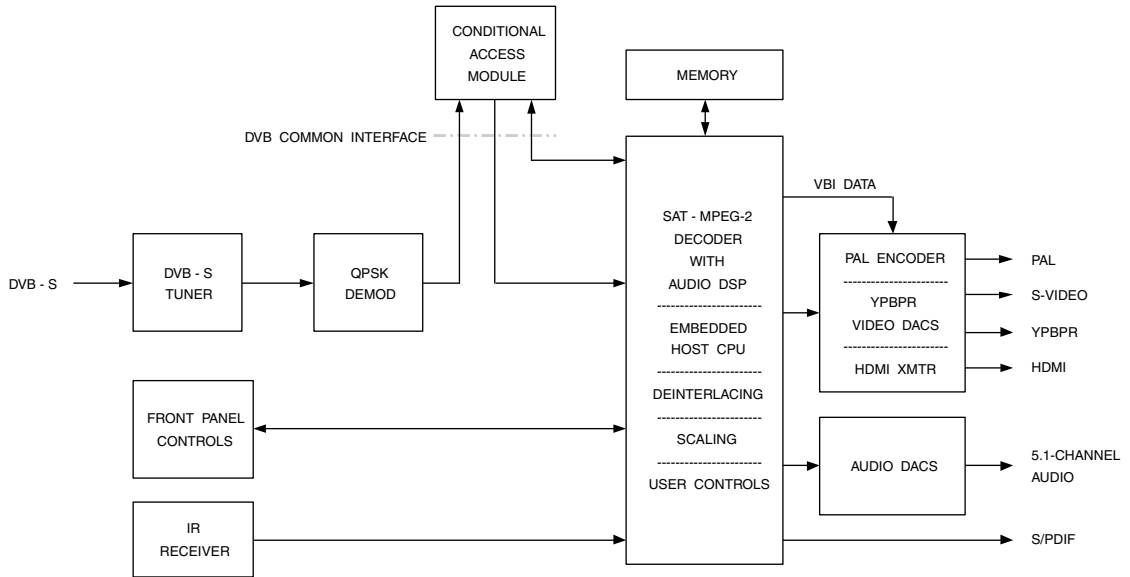
Figure 17.3. DVB Receiver Set-top Box Block Diagram (Multicrypt).
