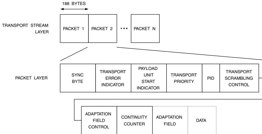
Figure 13.23. MPEG-2 Transport Stream Structure. Marker and reserved bits not shown.
