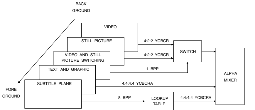
Figure 18.1. ISDB 5-Plane Video/Graphics Standard.
