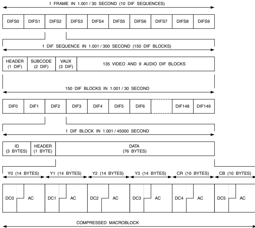
Figure 11.14. Packet Formatting for 25 Mbps 4:1:1 YCbCr 720 x 480i Systems.
