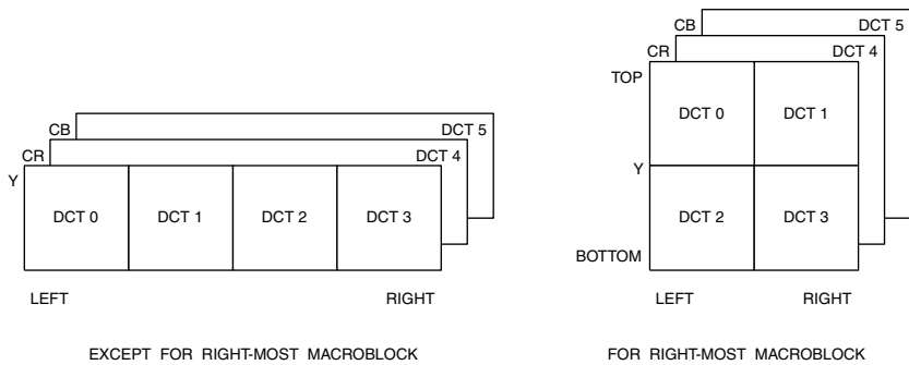
Figure 11.5. 4:1:1 Macroblock Arrangement.
