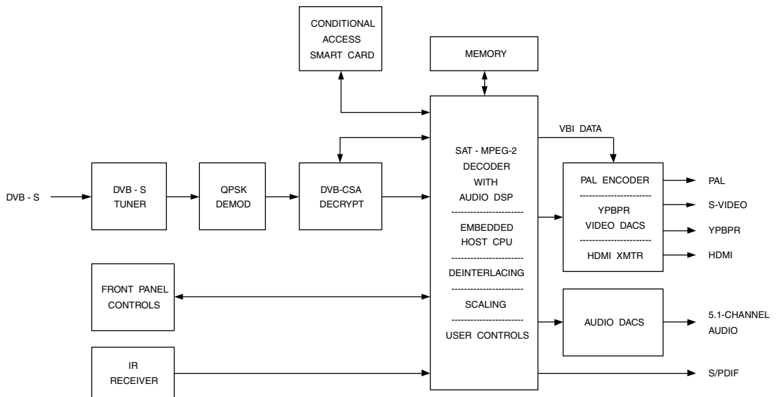
Figure 17.4. DVB Receiver Set-top Box Block Diagram (Simulcrypt).
