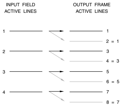
Figure 7.49. Deinterlacing Using Scan Line Duplication. New scan lines are generated by duplicating the active scan line above it.
