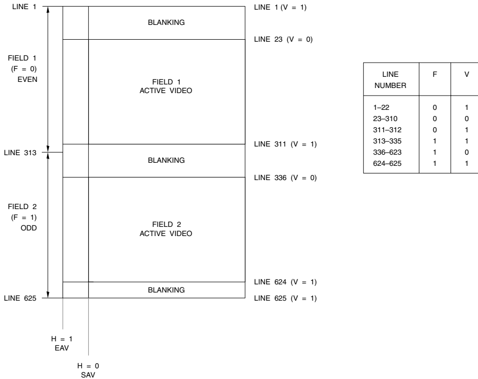
Figure 4.20. 576i Digital Vertical Timing (576 Active Lines). F and V change state at the EAV sequence at the beginning of the digital line. Note that the digital line number changes state prior to start of horizontal sync, as shown in Figures 4.16 through 4.19.
