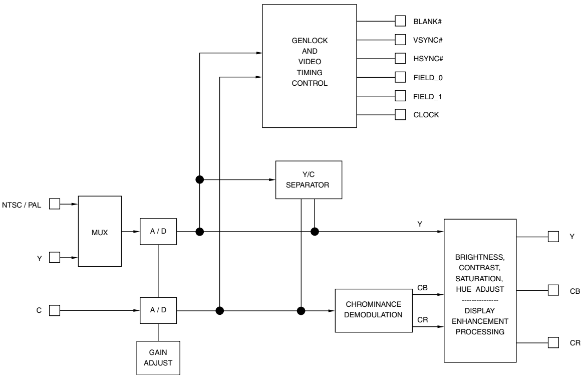
Figure 9.21. Typical NTSC/PAL Digital Decoder Implementation.
