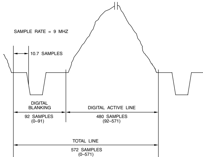
Figure 4.7. 480i Analog - Digital Relationship (4:3 Aspect Ratio, 29.97 Hz Refresh, 9 MHz Sample Clock).
