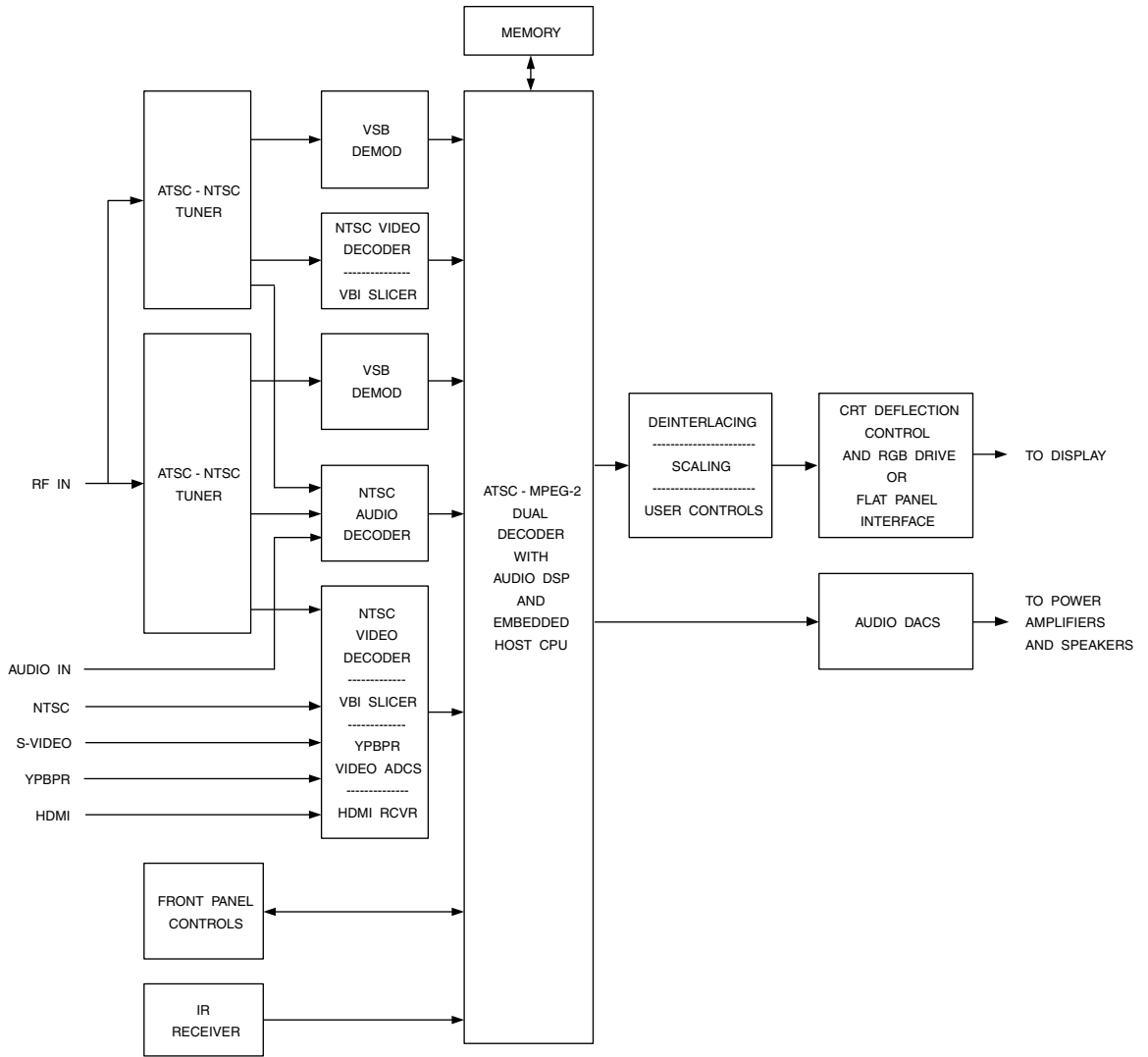
Figure 15.6. Typical ATSC Digital Television Block Diagram.
