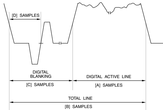
Figure 4.36. General 1080p Analog - Digital Relationship.
