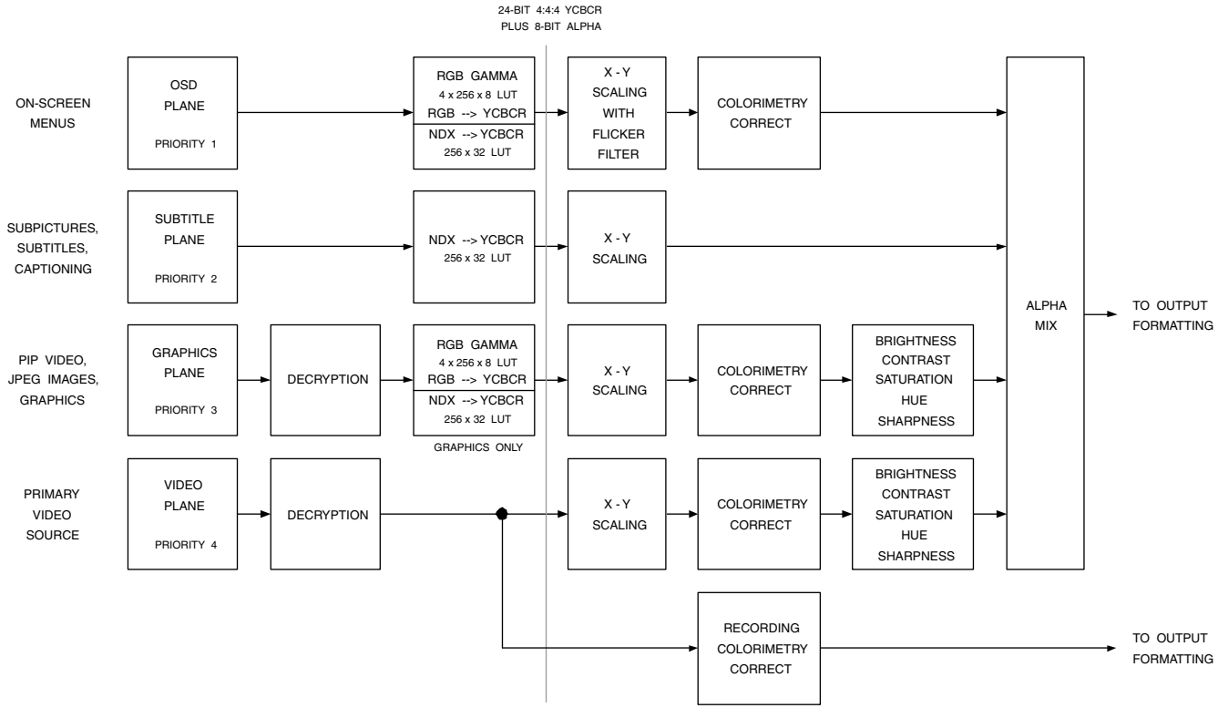
Figure 7.62. Video Composition Simplified Block Diagram.
