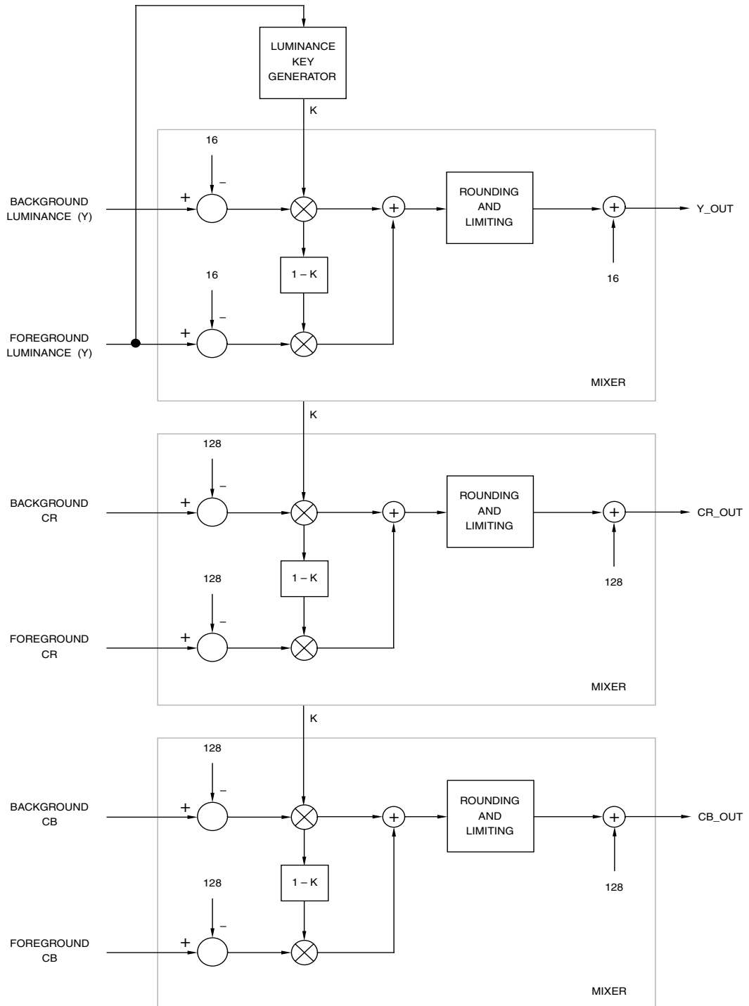
Figure 7.17. Luminance Keying of Two YCbCr Video Signals.
