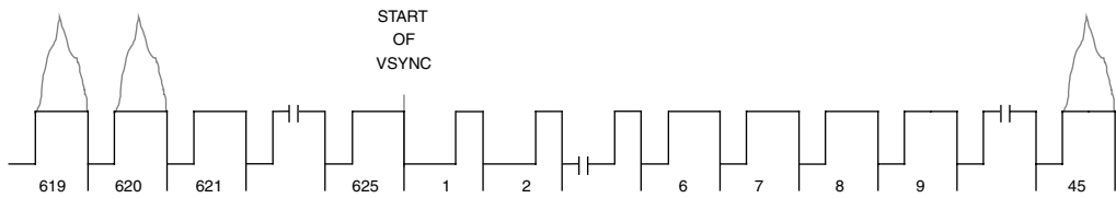
Figure 4.15. 576p Vertical Interval Timing.
