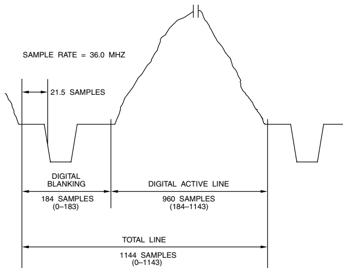
Figure 4.10. 480p Analog - Digital Relationship (16:9 Aspect Ratio, 59.94 Hz Refresh, 36 MHz Sample Clock).
