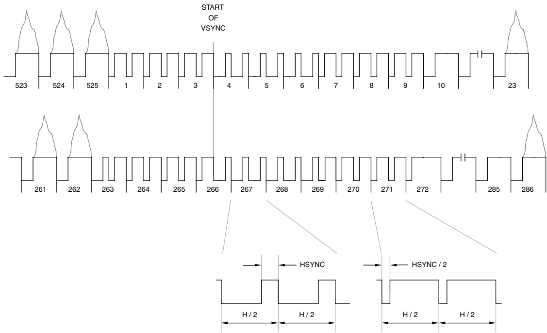
Figure 4.1. 480i Vertical Interval Timing.
