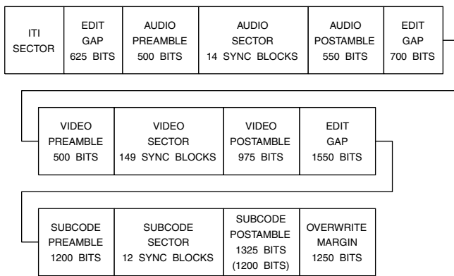
Figure 11.1. Sector Arrangement for One Track for a 480i System. The total bits per track, excluding the overwrite margin, is 134,975 (134,850). There are 10 (12) of these tracks per video frame. 576i system parameters (if different) are shown in parentheses.
