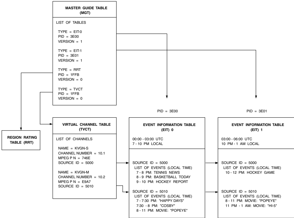
Figure 15.1. ATSC PSIP Table Relationships.
