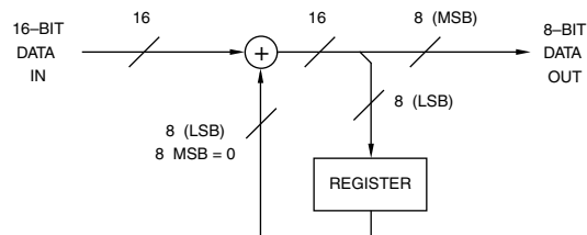
Figure 7.1. Error Feedback Rounding.
