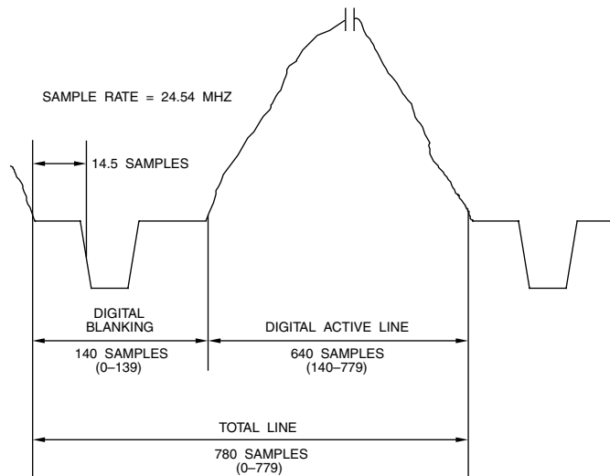
Figure 4.11. 480p Analog - Digital Relationship (4:3 Aspect Ratio, 59.94 Hz Refresh, 24.54 MHz Sample Clock).
