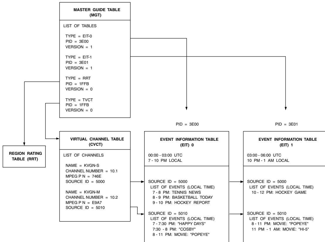
Figure 16.1. OpenCable™ In-Band SI Table Relationships.
