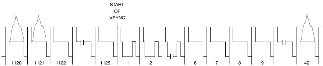
Figure 4.31. 1080p Vertical Interval Timing.
