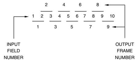
Figure 7.52. Producing Deinterlaced Frames at Field Rates.
