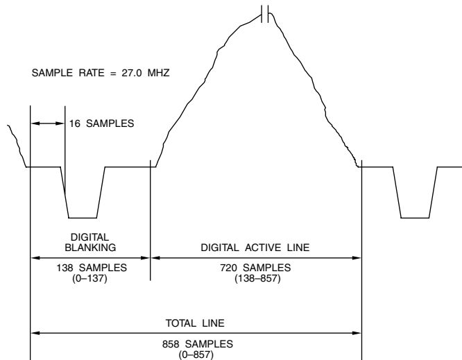
Figure 4.9. 480p Analog - Digital Relationship (4:3 Aspect Ratio, 59.94 Hz Refresh, 27 MHz Sample Clock).
