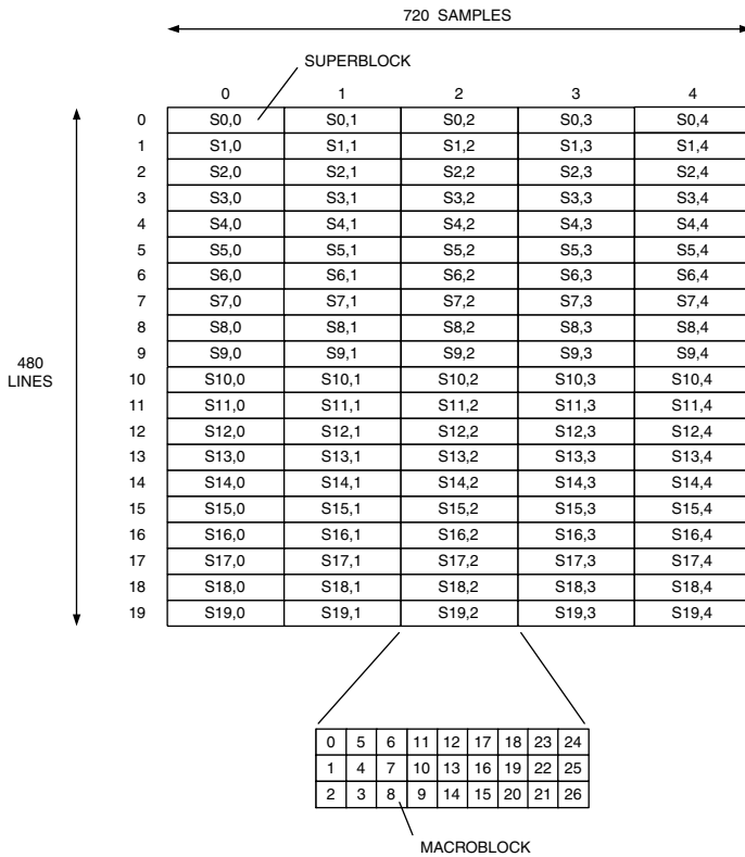
Figure 11.8. Relationship Between Super Blocks and Macroblocks (4:2:2 YCbCr, 720 × 480i).
