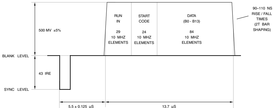
Figure 5.9. IEC 62375 576p Line 43 CGMS Timing.
