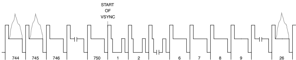
Figure 4.26. 720p Vertical Interval Timing.
