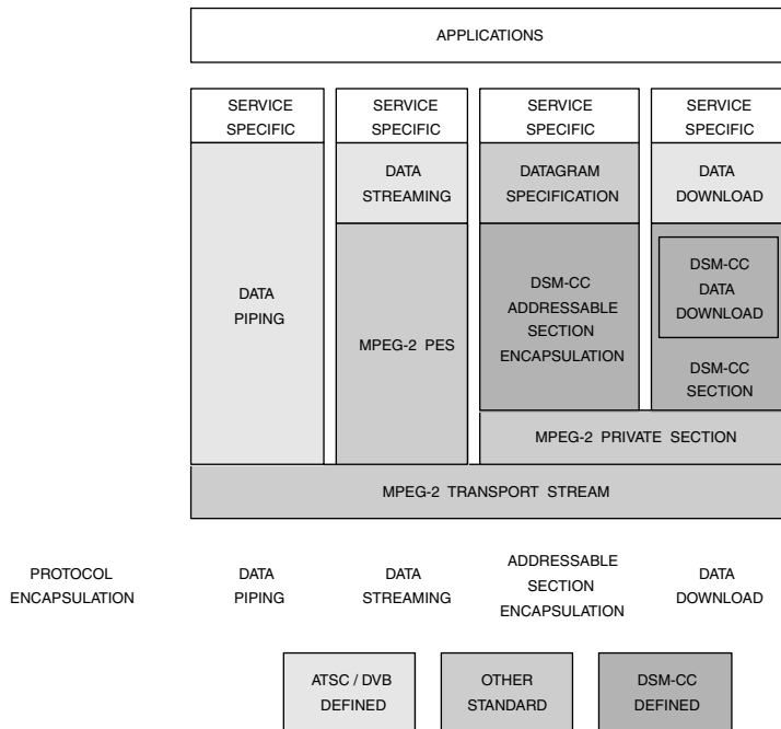
Figure 13.29. Encapsulation Overview.
