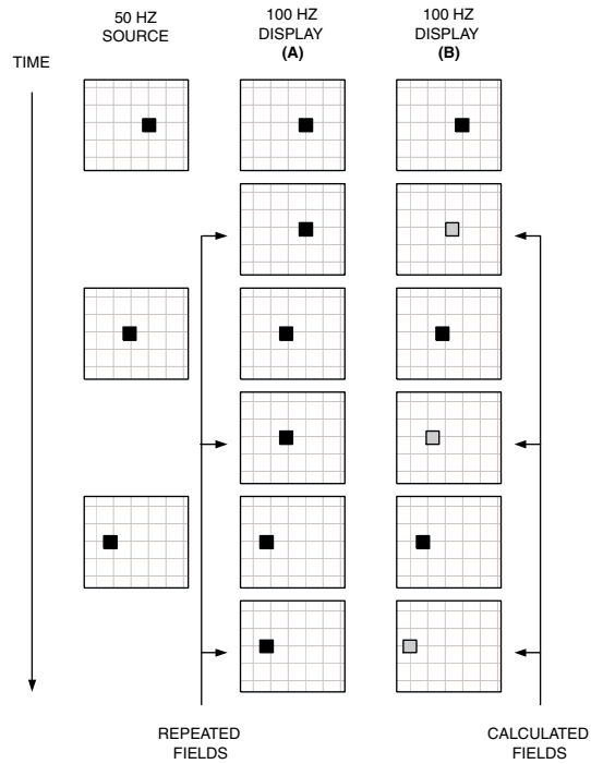
Figure 7.45. 50 Hz to 100 Hz (Double Scan Interlaced) Techniques.
