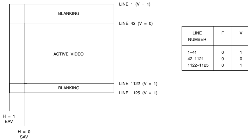
Figure 4.37. 1080p Digital Vertical Timing (1080 Active Lines). V changes state at the EAV sequence at the beginning of the digital line. Note that the digital line number changes state prior to start of horizontal sync, as shown in Figures 4.35 and 4.36.
