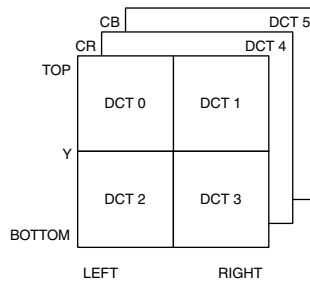
Figure 11.6. 4:2:0 Macroblock Arrangement.
