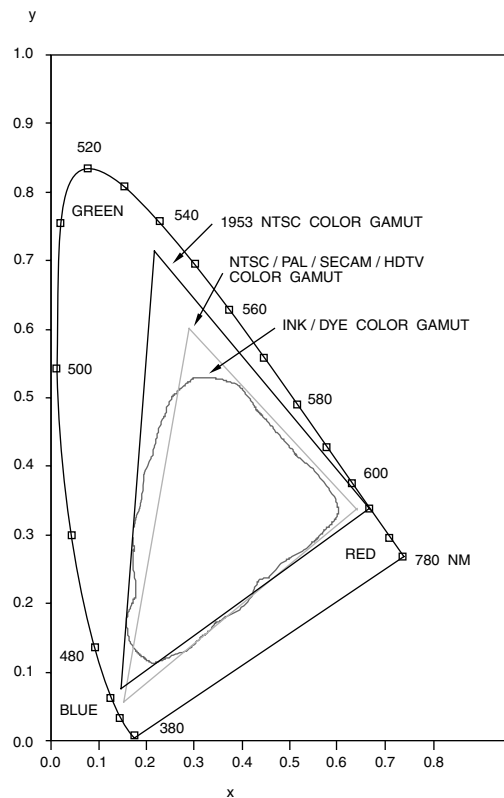
Figure 3.15. CIE 1931 Chromaticity Diagram Showing Various Color Gamuts.
