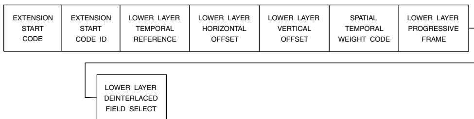
Figure 13.13. MPEG-2 Picture Spatial Scalable Extension Structure. Marker bits not shown.
