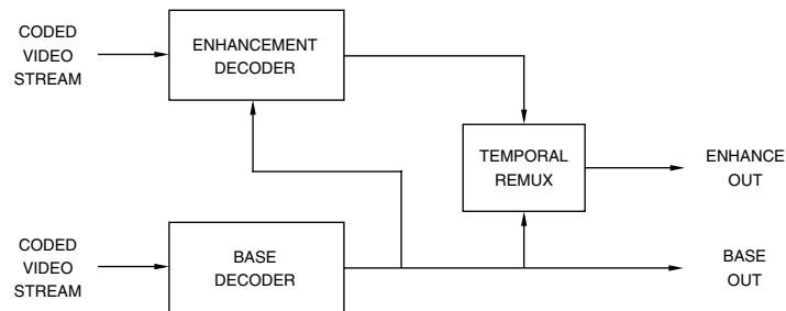
Figure 13.33. Simplified MPEG-2 Temporal Scalability Decoder Block Diagram.
