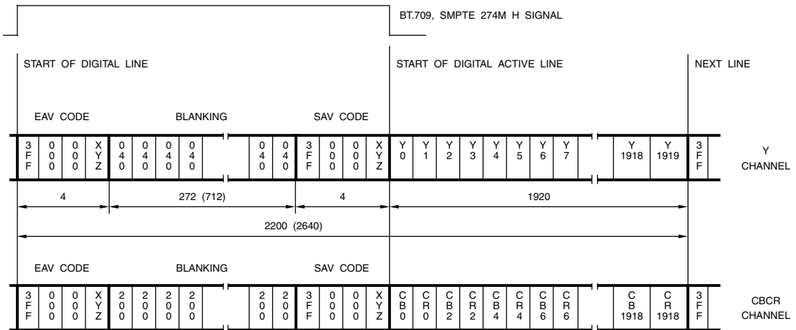
Figure 6.16. BT.1120 and SMPTE 274M Parallel Interface Data For One Scan Line. 1080i; 29.97-, 30-, 59.94-, and 60-Hz systems; 4:2:2 YCbCr; 1920 active samples per line; 74.176, 74.25, 148.35, or 148.5 MHz clock; 10-bit system. The values for 25- and 50-Hz systems are shown in parentheses.
