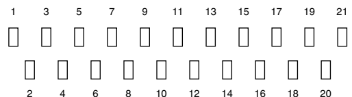
Figure 5.2. SCART Connector.
