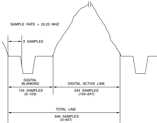
Figure 4.24. 576p Analog - Digital Relationship (4:3 Aspect Ratio, 50 Hz Refresh, 20.25 MHz Sample Clock).
