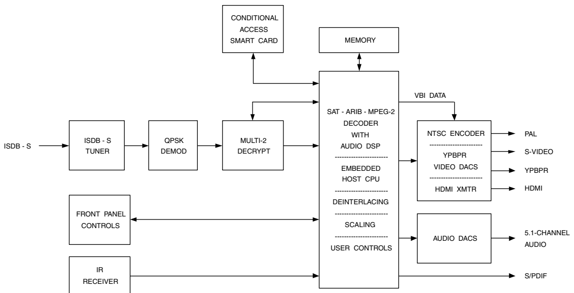
Figure 18.2. ISDB Receiver Set-top Box Block Diagram.
