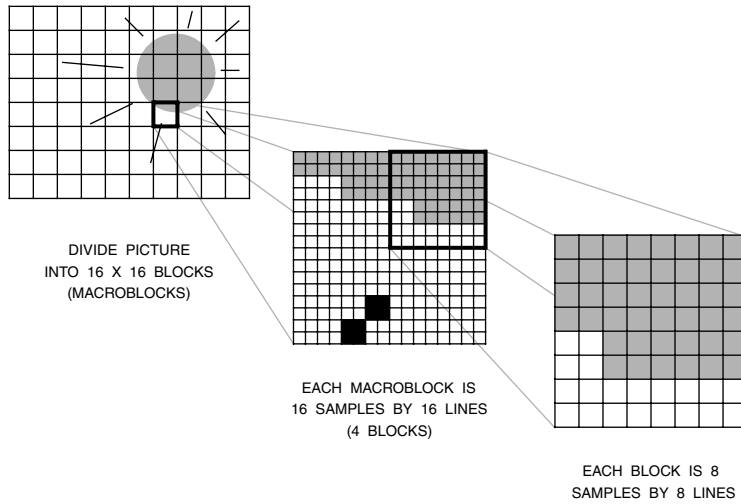
Figure 7.55. The Relationship between Macroblocks and Blocks.
