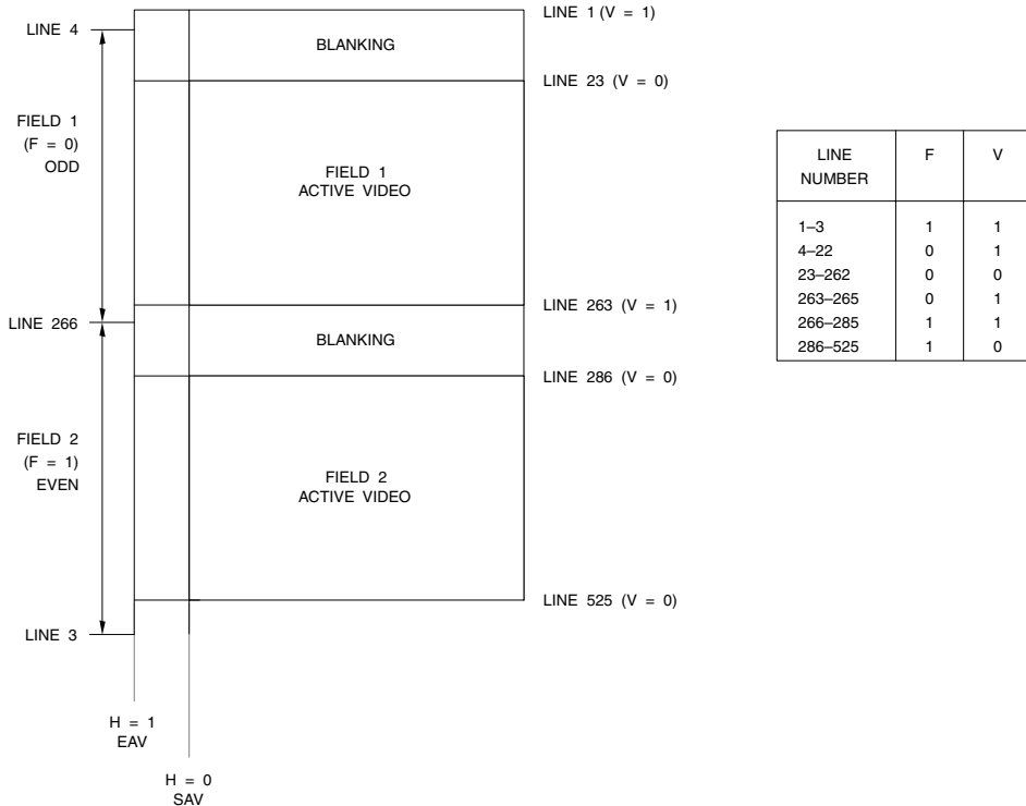
Figure 4.8. 480i Digital Vertical Timing (480 Active Lines). F and V change state at the EAV sequence at the beginning of the digital line. Note that the digital line number changes state prior to start of horizontal sync, as shown in Figures 4.3 through 4.7.
