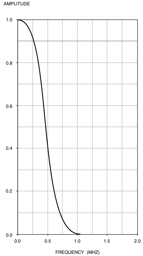
Figure 9.5. Typical 0.6-MHz Lowpass Digital Filter Characteristics.
