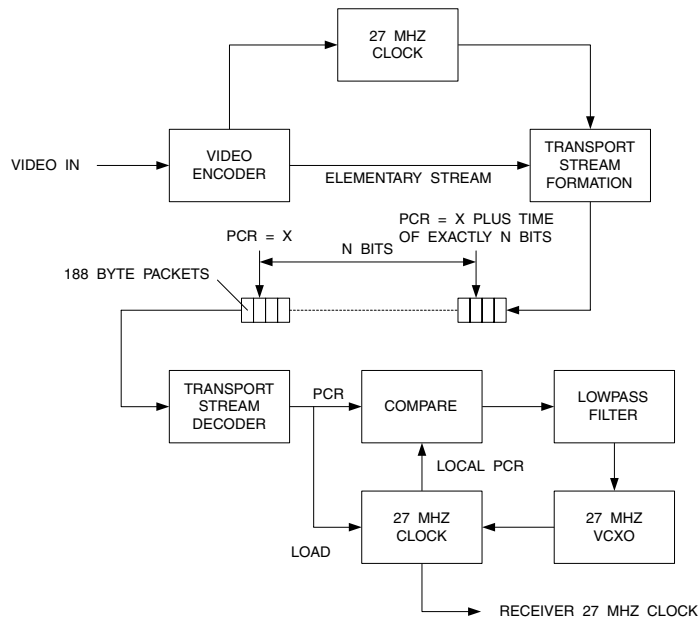
Figure 13.34. 27 MHz Clock Generation by MPEG-2 Decoder.
