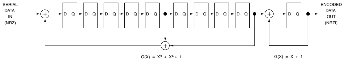
Figure 6.7. Typical Scrambler Circuit.
