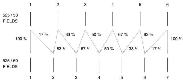
Figure 7.40. 50-Hz to 60-Hz Conversion Using Temporal Interpolation with No Motion Compensation.
