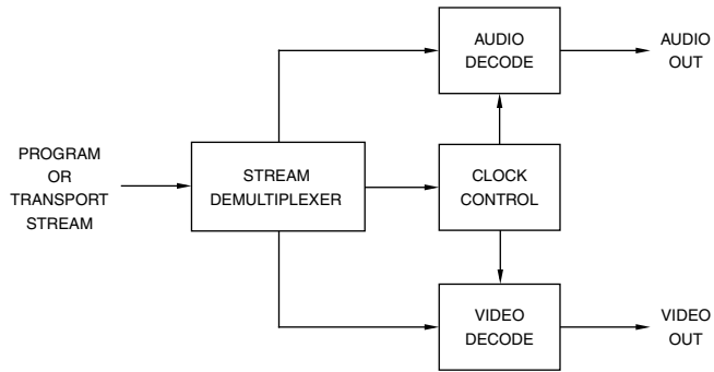
Figure 13.31. Simplified MPEG-2 Decoder Block Diagram.
