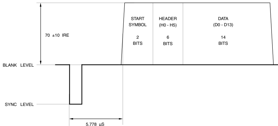
Figure 5.8. EIA-805, IEC 61880–2 and EIA-J CPR-1204–1 480p Line 41 CGMS Timing.
