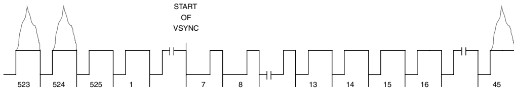
Figure 4.2. 480p Vertical Interval Timing.
