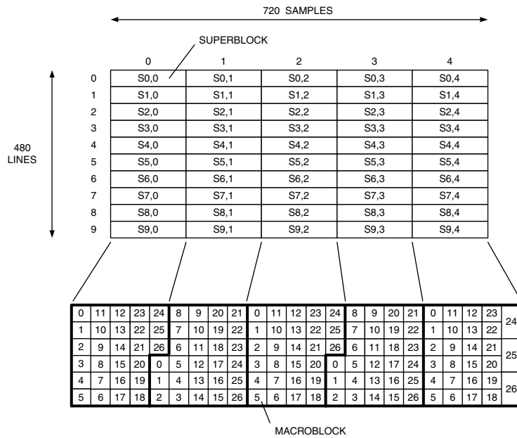
Figure 6.60. Relationship Between Super Blocks and Macroblocks (720 × 480, 4:1:1 YCbCr).
