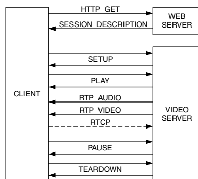
Figure 19.4. Client, Web Server and Video Server Communications.
