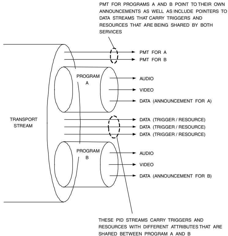
Figure 13.28. Sharing Triggers and Resources.
