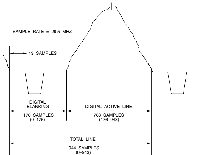
Figure 4.23. 576p Analog - Digital Relationship (4:3 Aspect Ratio, 50 Hz Refresh, 29.5 MHz Sample Clock).
