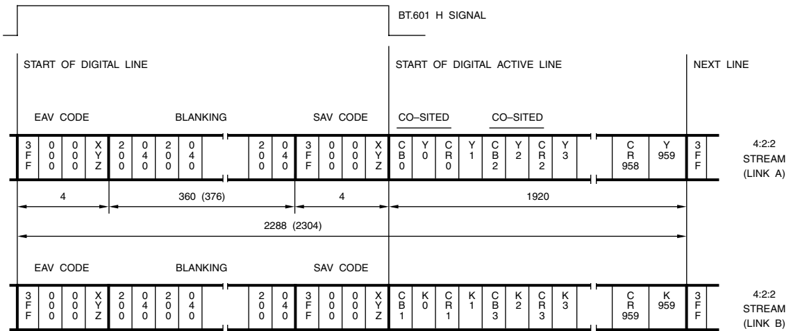
Figure 6.14. BT.1303 Parallel Interface Data For One Scan Line. 480i; 4:4:4:4 YCbCrK; 960 active samples per line; 36 MHz clock; 10-bit system. The values for 576i systems are shown in parentheses.
