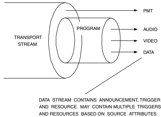
Figure 13.26. Announcement, Trigger and Resource Data Carried on a Single PID Stream.
