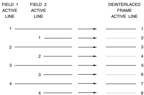
Figure 7.51. Deinterlacing Using Field Merging. Shaded scan lines are generated by using the input scan line from the next or previous field.
