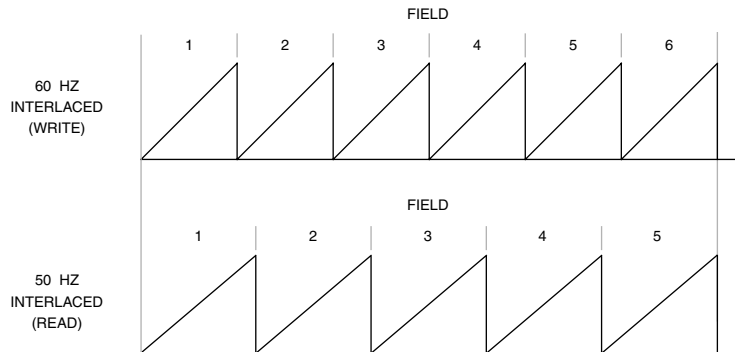
Figure 7.39. 60-Hz to 50-Hz Conversion Using a Single Field Store by Dropping One out of Every Six Fields.
