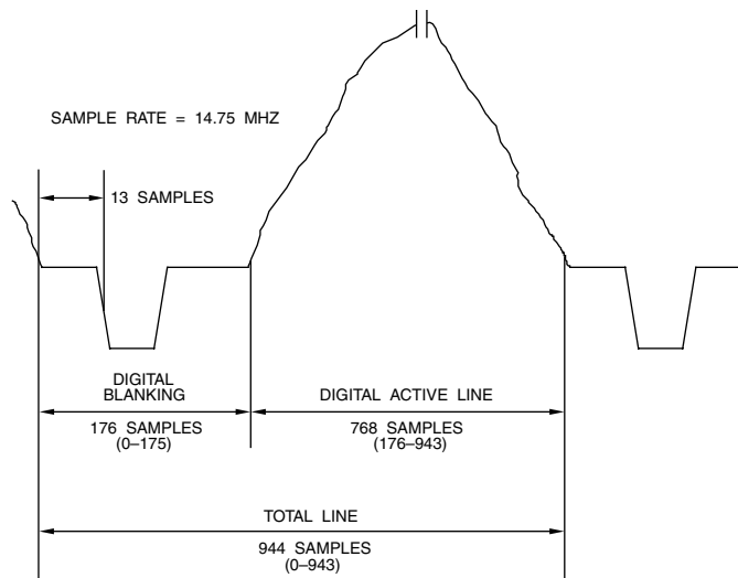
Figure 4.18. 576i Analog - Digital Relationship (4:3 Aspect Ratio, 25 Hz Refresh, 14.75 MHz Sample Clock).
