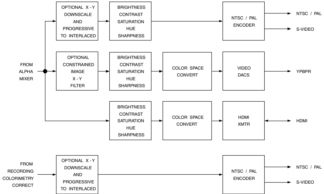
Figure 7.63. Video Output Port Processing.
