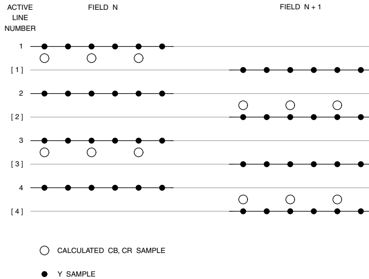
Figure 3.9. 4:2:0 Sampling for MPEG-2, MPEG-4 Part 2 and H.264. The sampling positions on the active scan lines of an interlaced picture (top_field_first = 1).
