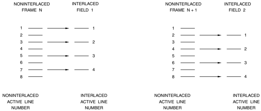
Figure 7.47. Noninterlaced-to-Interlaced Conversion Using Scan Line Decimation.
