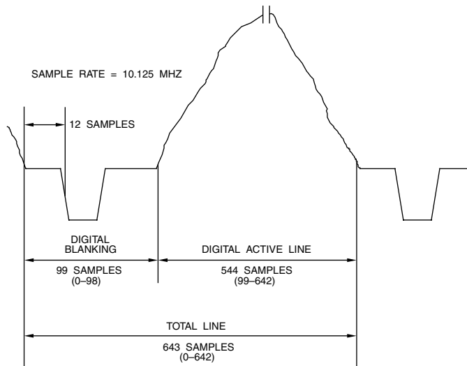
Figure 4.6. 480i Analog - Digital Relationship (4:3 Aspect Ratio, 29.97 Hz Refresh, 10.125 MHz Sample Clock).
