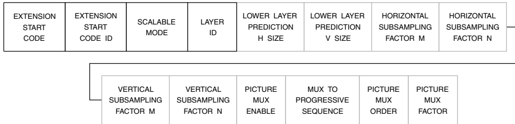
Figure 13.8. MPEG-2 Sequence Scalable Extension Structure. Marker bits not shown.
