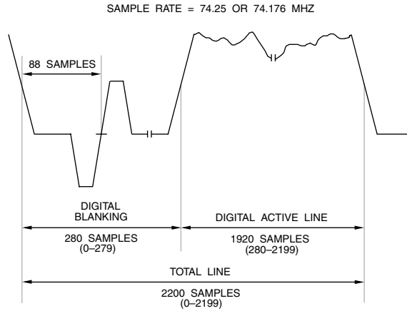
Figure 4.32. 1080i Analog - Digital Relationship (16:9 Aspect Ratio, 29.97 Hz Refresh, 74.176 MHz Sample Clock and 30 Hz Refresh, 74.25 MHz Sample Clock).
