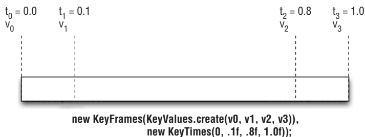
Figure 15-14 Creating KeyFrames with multiple values and times. The number of times supplied must equal the number of values.
