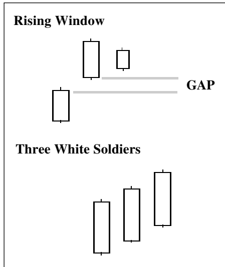
Figure 3-9: Continuation patterns.
