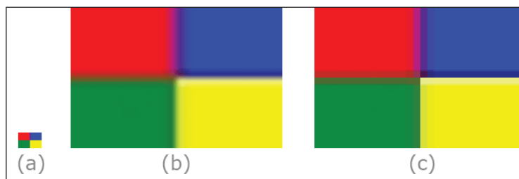
Fig 3-26: (a) Original image, (b) Enlarged with -resize , (c) Enlarged with -sample
