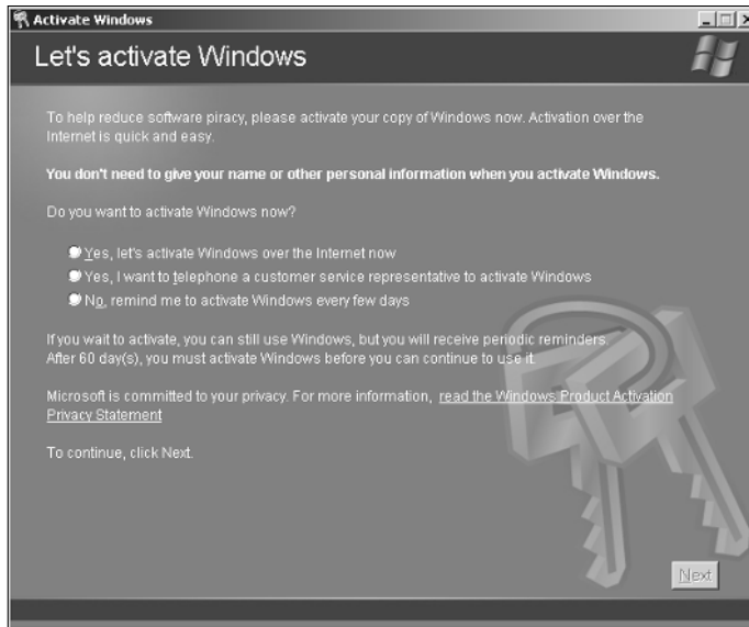
Figure 1-3: Activating Windows.
