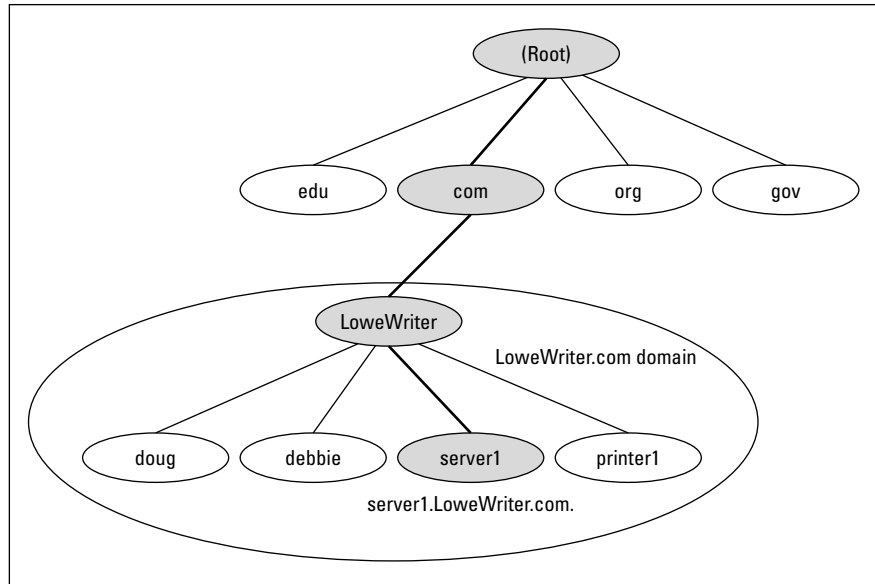
Figure 4-1: DNS names.
