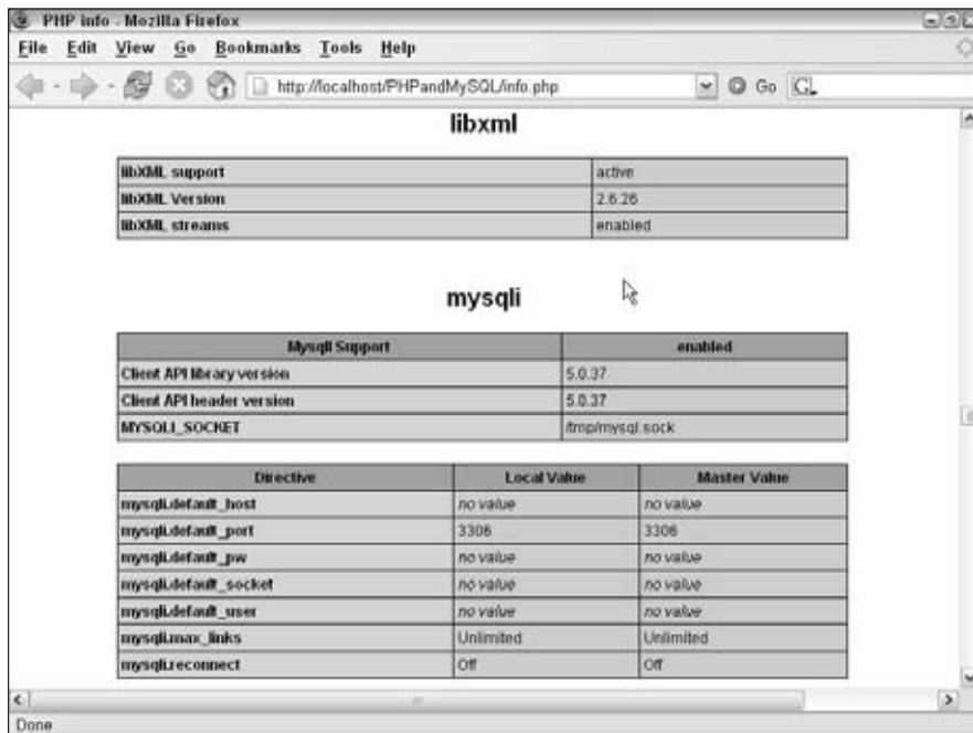
Figure 2-4: MySQL settings.
