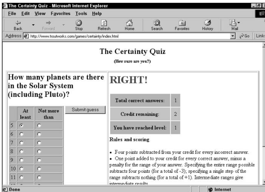
Figure 46-2: Continuing play
