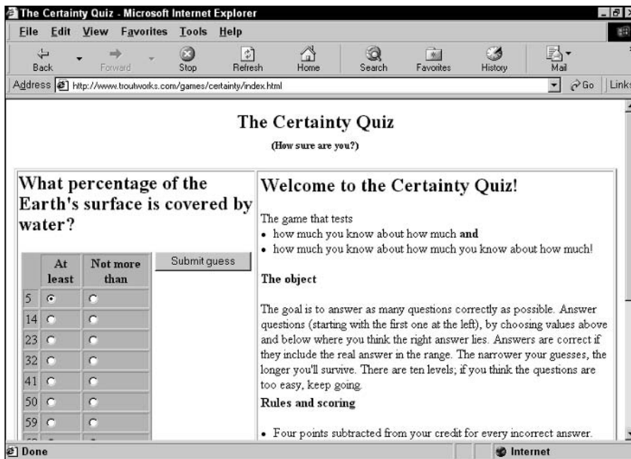
Figure 46-1: Start screen
