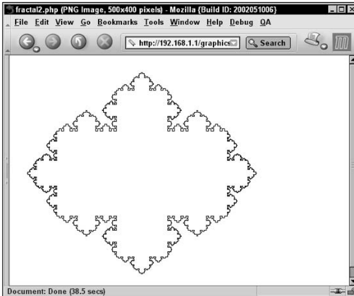
Figure 42-4: Fractal 2
