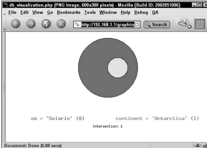
Figure 48-4: Subset
