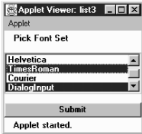
Figure 9.3: Multiselect List
