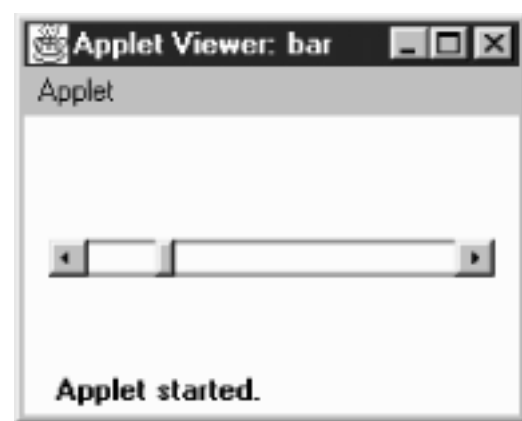
Figure 11.1: Scrollbar elements
