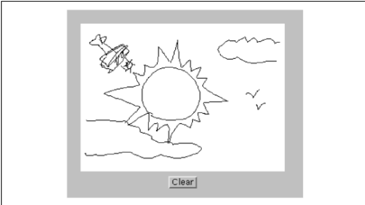
Figure 11.8: The ComponentScrollerApplet
