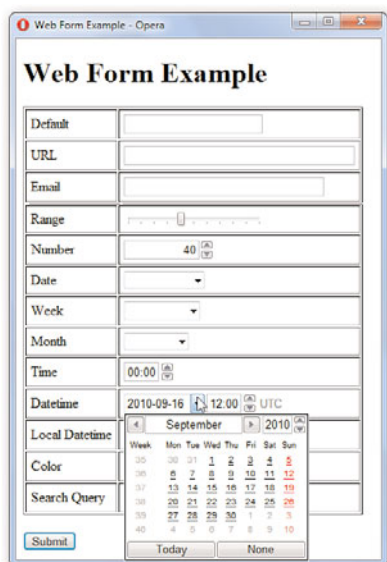
FIGURE 4.1 The webforms.html example.
