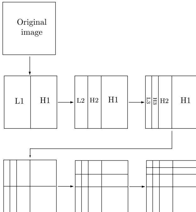
Figure 5.15: The Standard Image Wavelet Transform and Decomposition.
