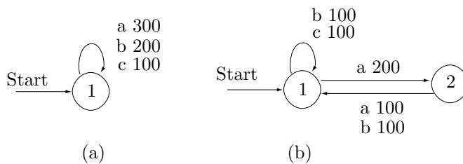
Figure 8.35: Finite-State Models for Data Compression.
