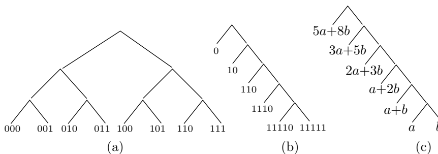
Figure 2.27: Shortest and Tallest Huffman Trees.
