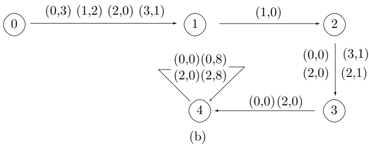
Figure 4.179: A Five-State GFA.
