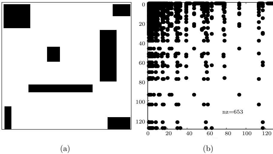
Figure 5.21: Reconstructing a 128 \times 128 Simple Image From 4% of Its Coefficients.
