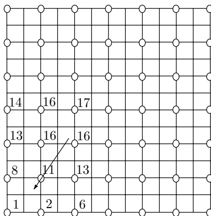
Figure 6.13: Quadrant Monotonic Search.
