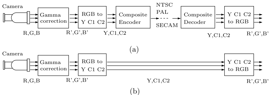
Figure 6.5: (a) Composite and (b) Component Television Transmission.
