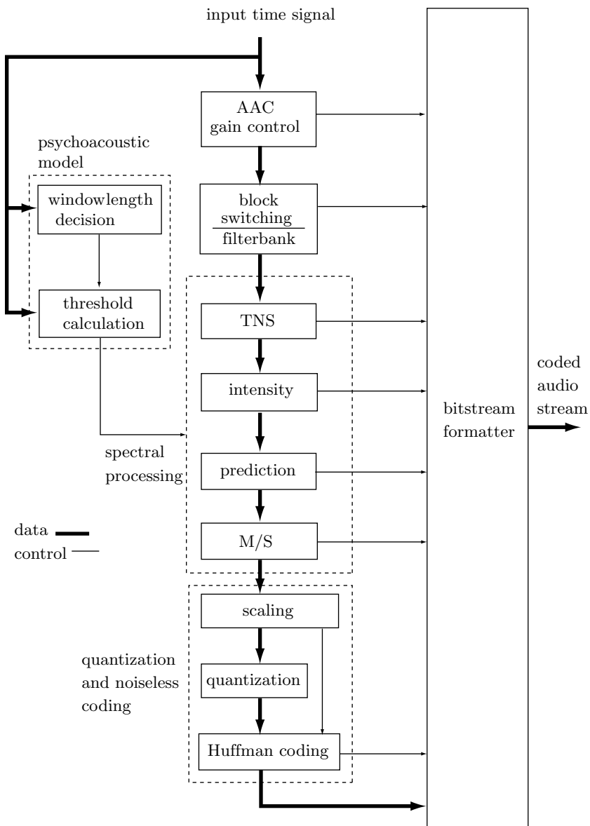
Figure 7.72: AAC Encoder.
