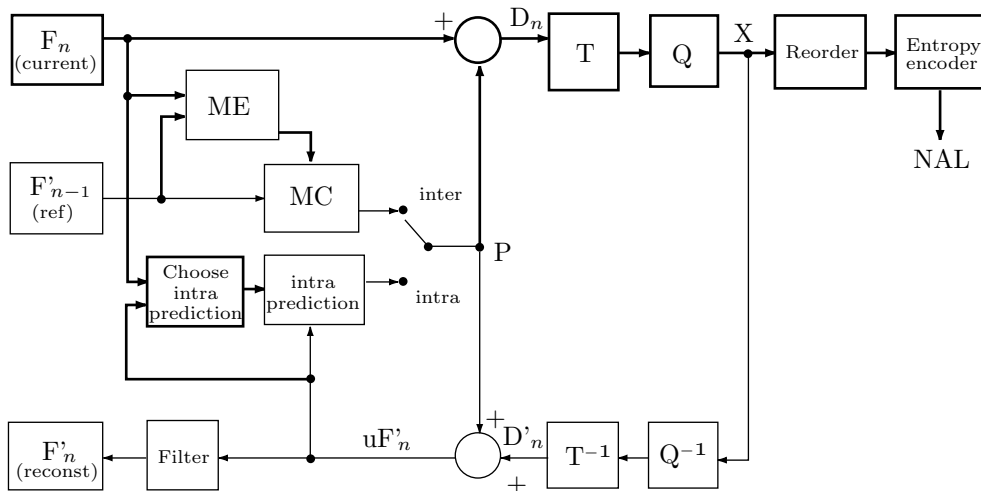
Figure 6.40: H.264 Encoder.
