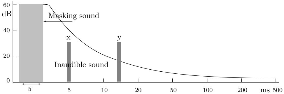
Figure 7.68: Audio Masking in Time.
