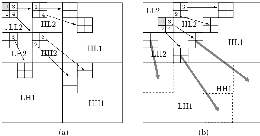
Figure 5.57: Spatial Orientation Trees in SPIHT.
