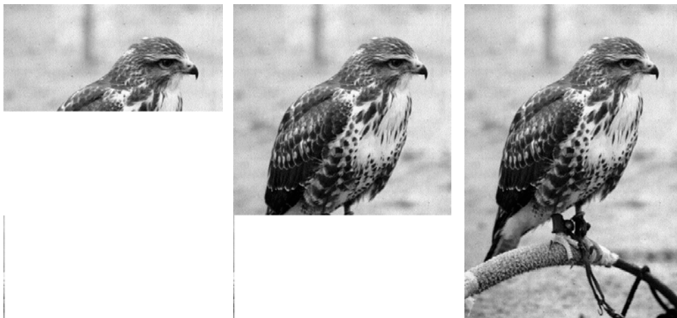
Figure 4.78: Sequential Decoding.
