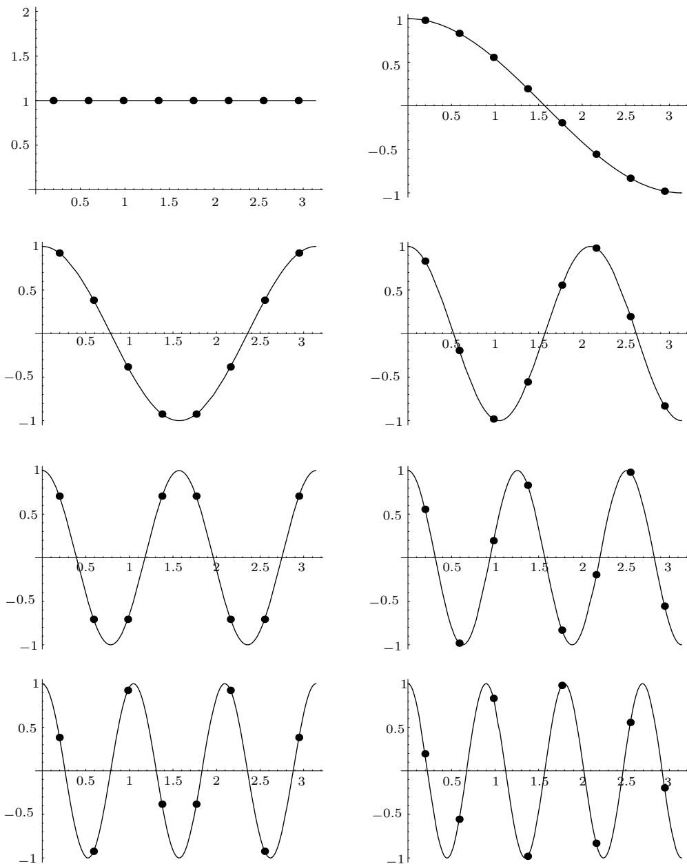
Figure 4.36: Angle and Cosine Values for an 8-Point DCT.
