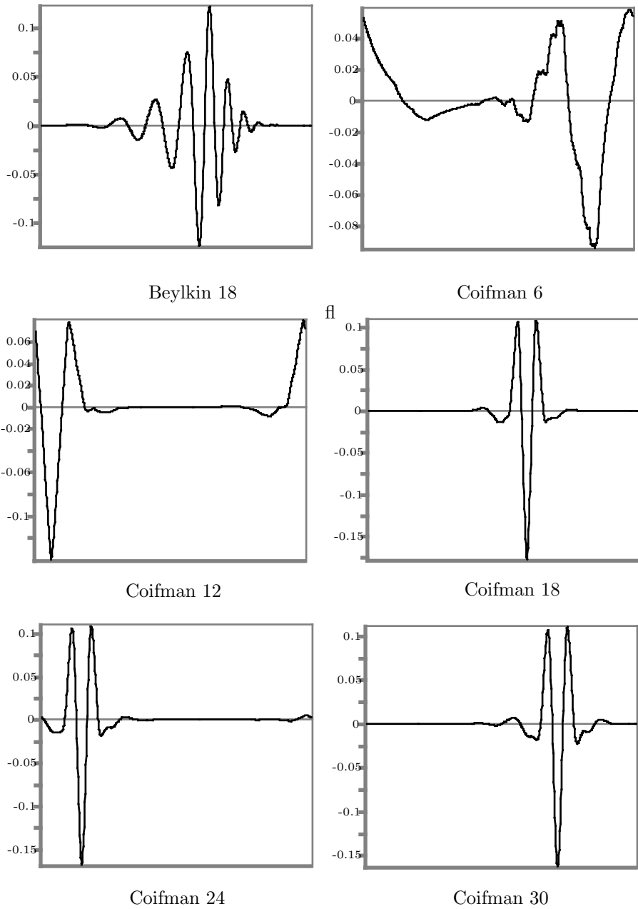
Figure 5.36: Examples of Common Wavelets.
