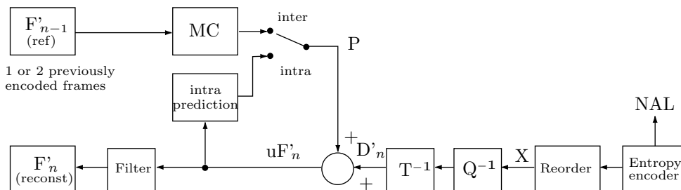
Figure 6.41: H.264 Decoder.
