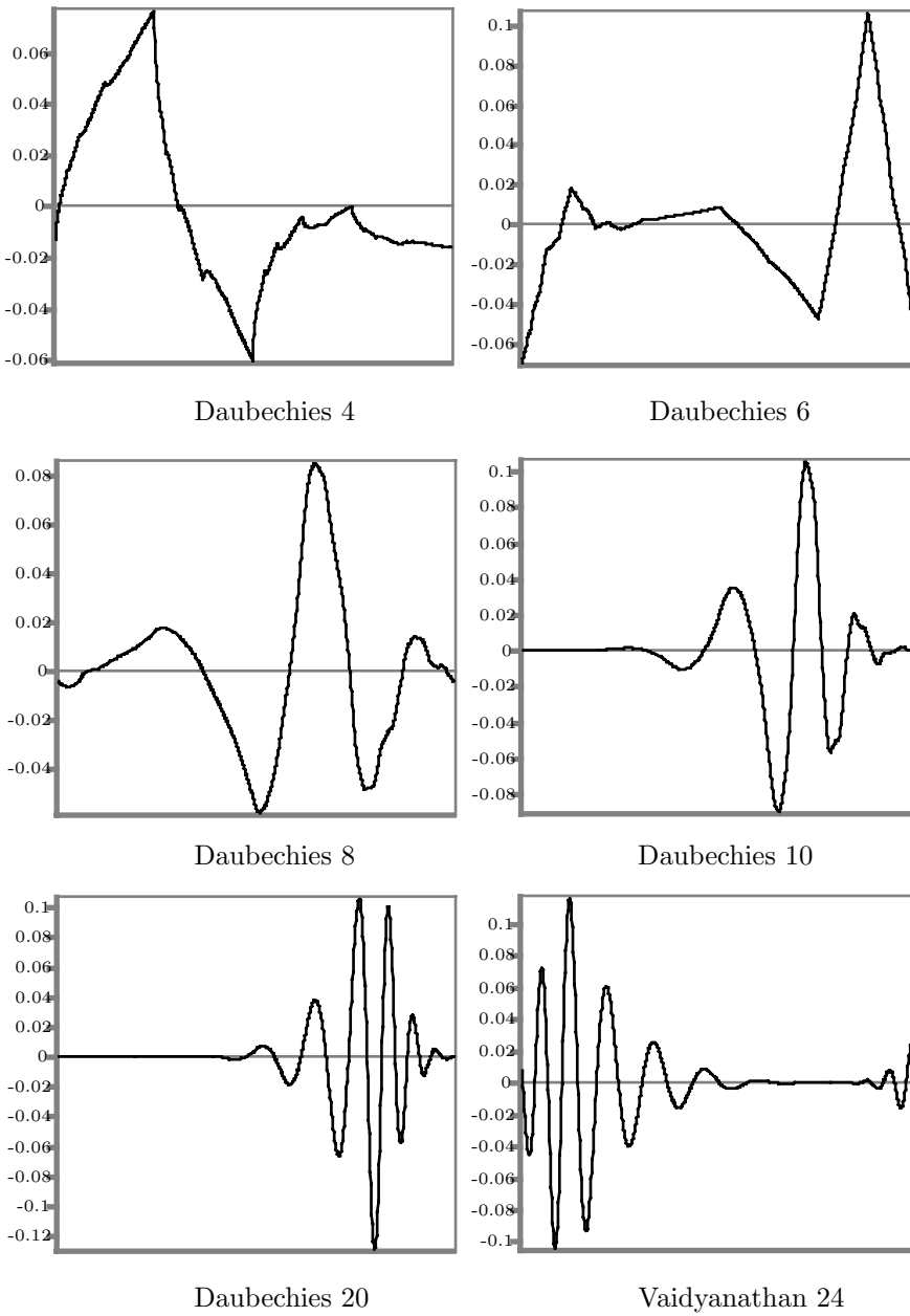
Figure 5.37: Examples of Common Wavelets.
