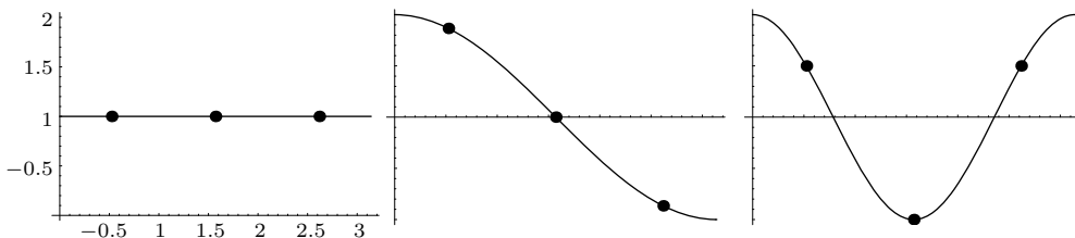
Figure 4.35: Increasing Frequencies.
