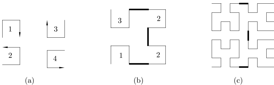
Figure 4.162: Hilbert Curves of Orders 1, 2, and 3.
