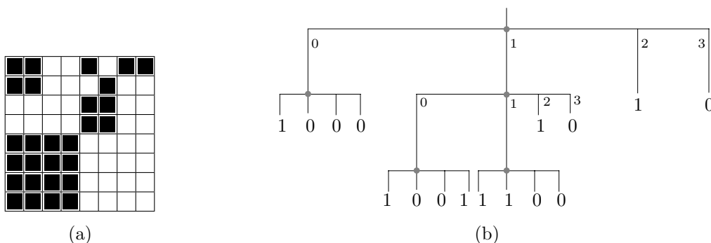
Figure 4.148: A Quadtree.
