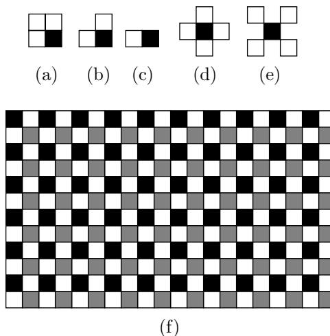
Figure 6.14: Strategies for Spatial Dependent Search Algorithms.
