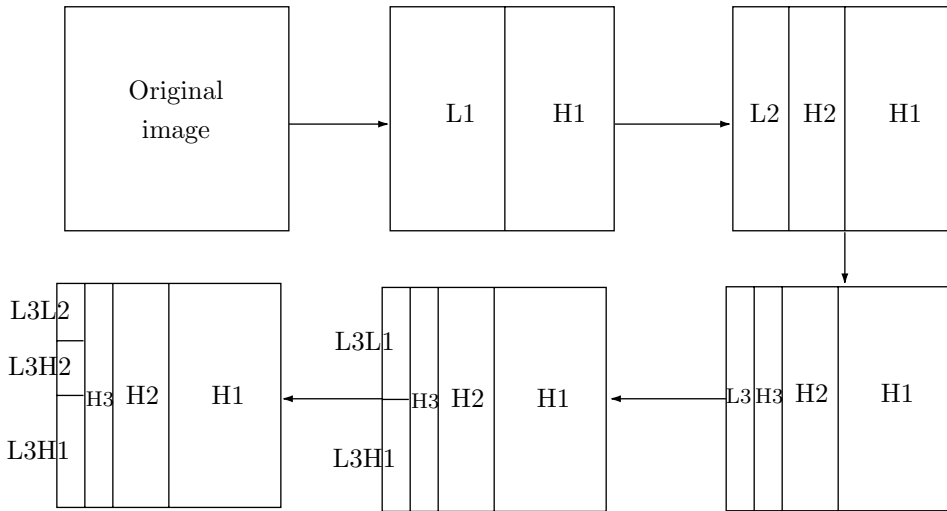
Figure 5.40: Line Wavelet Decomposition.
