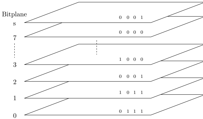
Figure 5.75: Bitplanes of Four Coefficients in a Code-Block.
