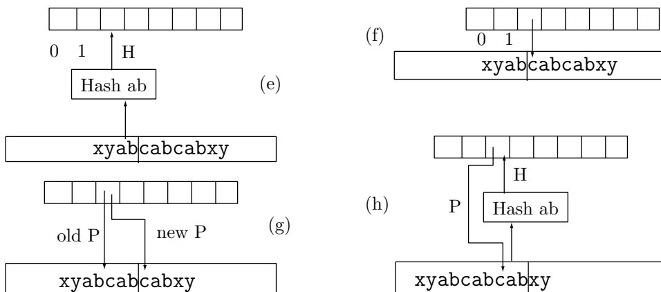
Figure 3.28 (Continued). LZP Compression of xyabcbcabxy : Part II.
