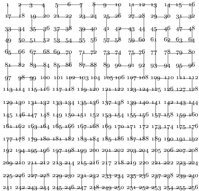
Figure 4.160: Hilbert Scan of 16 \times 16 Blocks.
