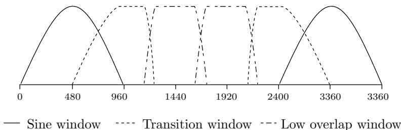
Figure 7.84: Window Shapes in AAC-LD.
