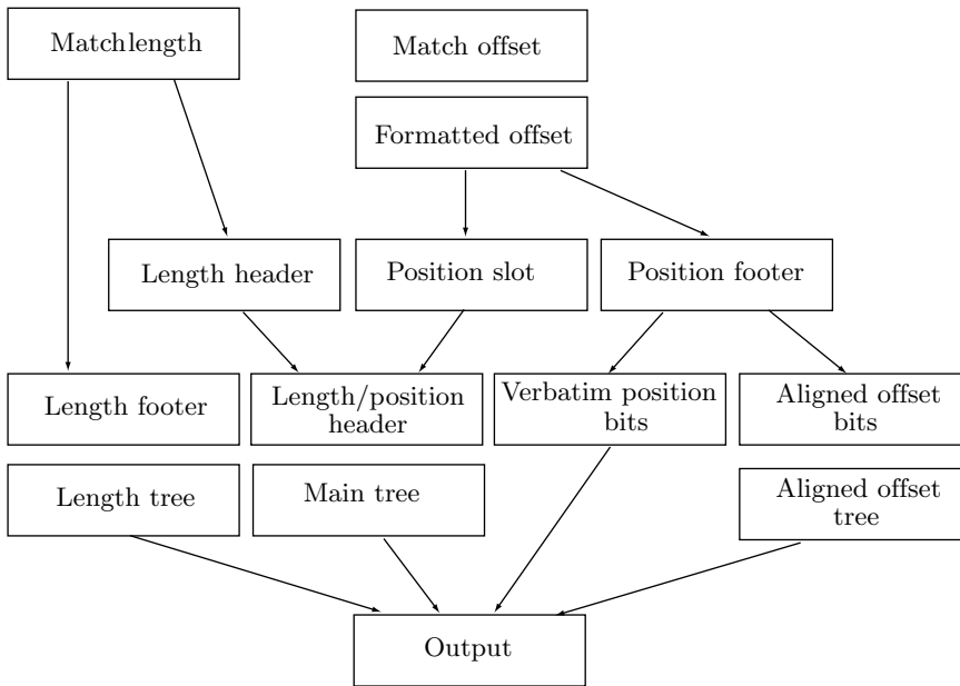
Figure 3.9: LZ78 Processing of Offsets and Lengths.
