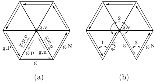
Figure 8.46: Handling Case C.
