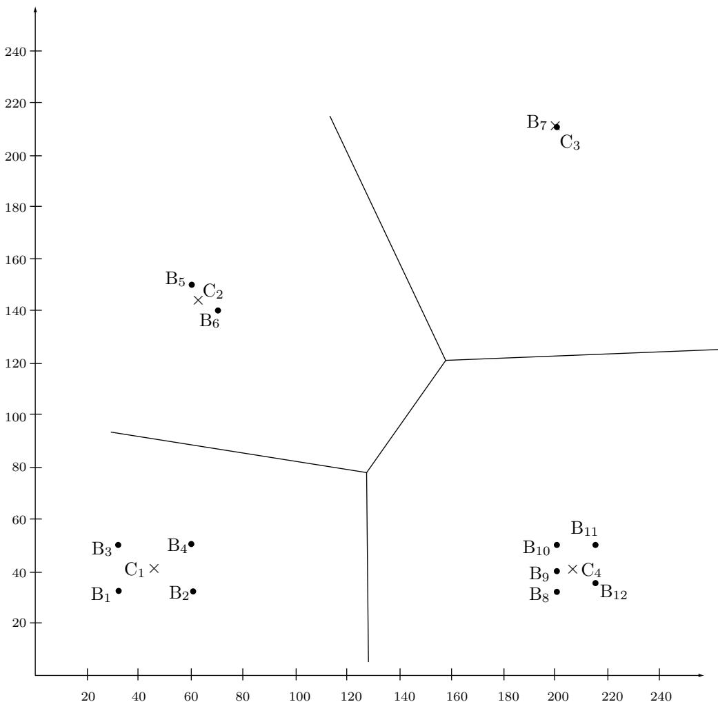
Figure Ans.33: Twelve Points and Four Codebook Entries C_i^{(1)} .
