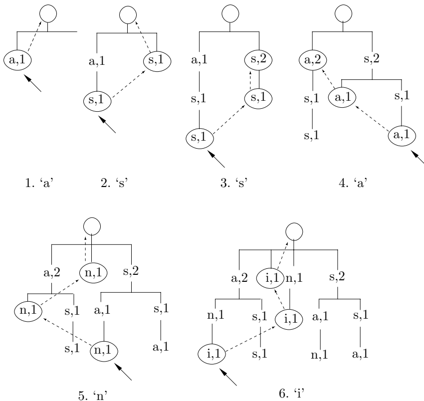
Figure 2.75: Part I. First Six Tries of "assanissimassa".
