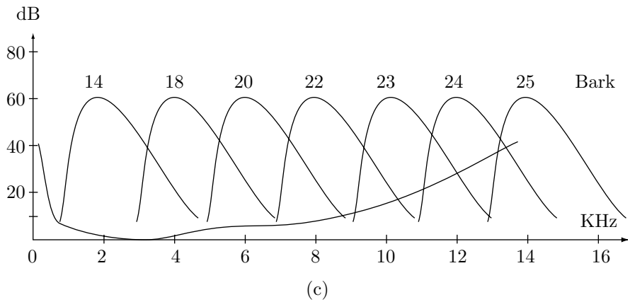
Figure 7.5: Threshold and Masking of Sound.
