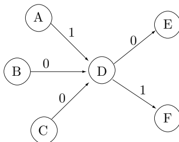
Figure 8.37: State D Is a Candidate.
