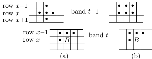
Figure 8.60: Two Alternative Predictions for Hyperspectral Data.
