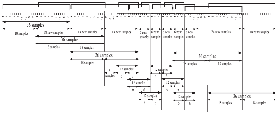
Figure 7.62: Overlapping MDCT Windows.
