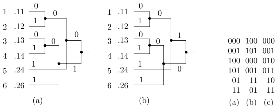
Figure 2.24: Two Huffman Code-Trees.
