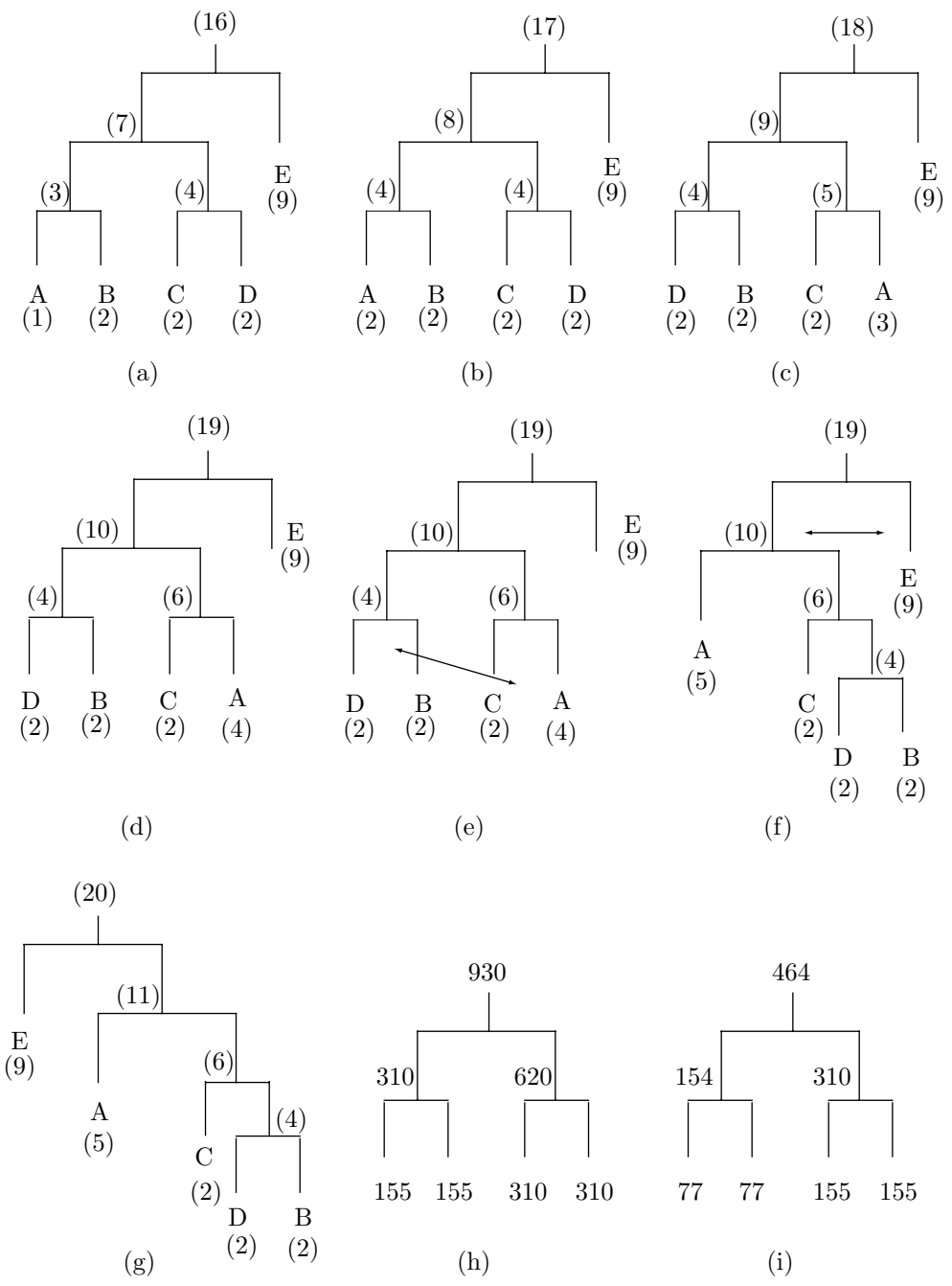
Figure 2.33: Updating the Huffman Tree.
