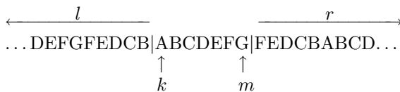
Figure 5.70: Extending a Row of Pixels.
