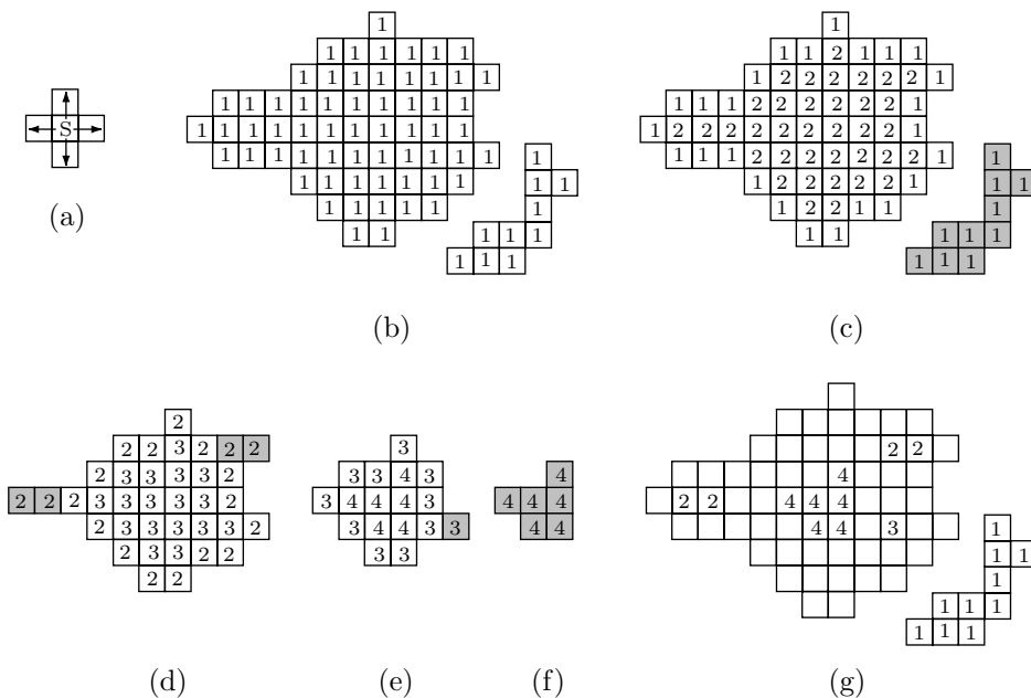
Figure 4.83: Recursive Encoding of a Pattern.
