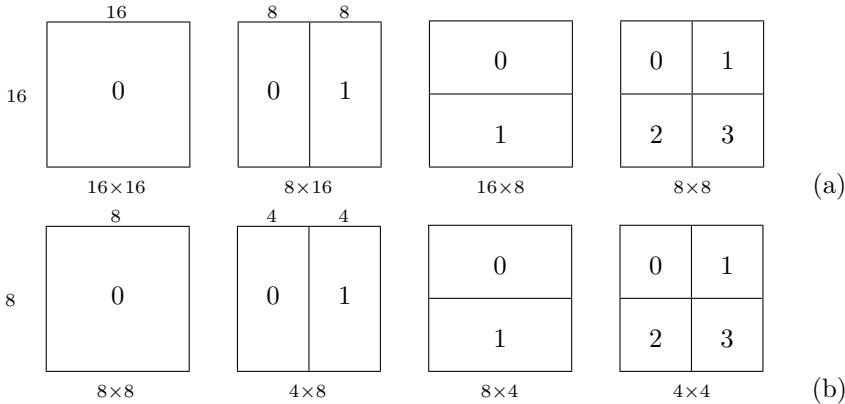
Figure 6.43: H.264 Macroblock Partitions.
