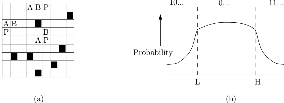
Figure 4.118: (a) The Two Neighbors. (b) The Three Regions.
