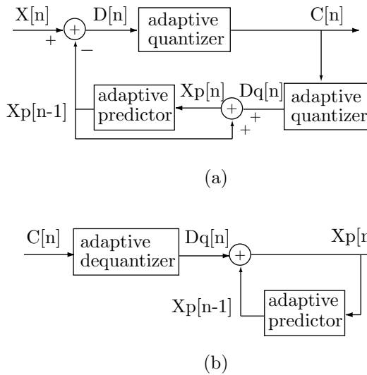
Figure 7.18: (a) ADPCM Encoder and (b) Decoder.
