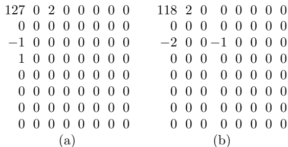
Figure 6.22: Two 8 \times 8 Blocks of DCT Quantized Coefficients.
