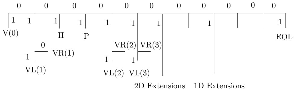
Figure 2.45: Tree of Group 3 Codes.
