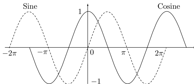
Figure 4.50: The Sine and Cosine as Odd and Even Functions, Respectively.
