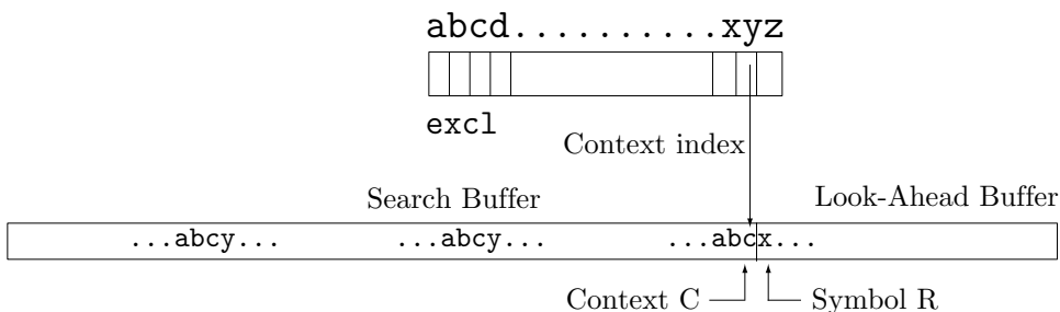
Figure 8.4: Exclusion Mechanism.
