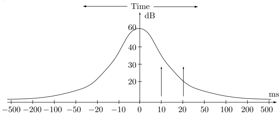
Figure 7.7: Threshold and Masking of Sound.
