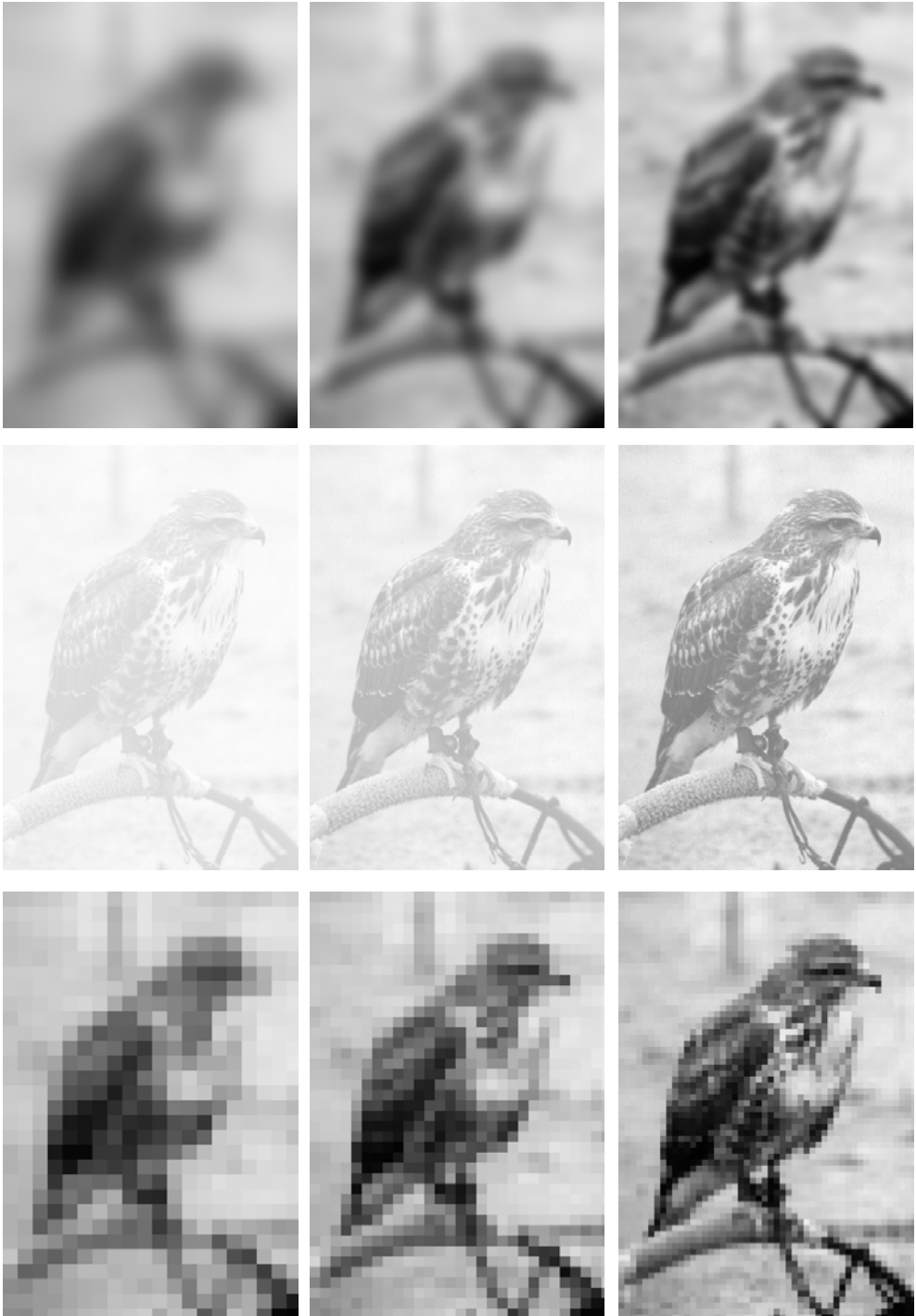
Figure 4.79: Progressive Decoding.
