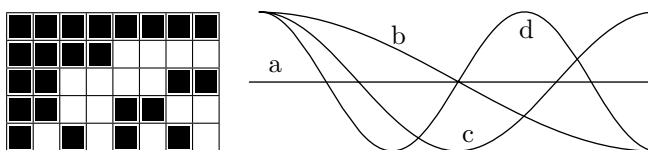
Figure 4.18: Image Frequencies.
