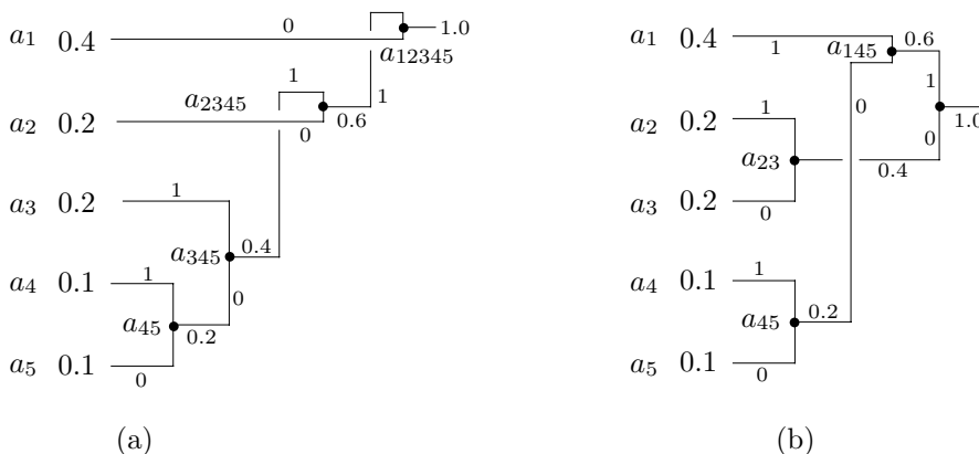
Figure 2.16: Huffman Codes.
