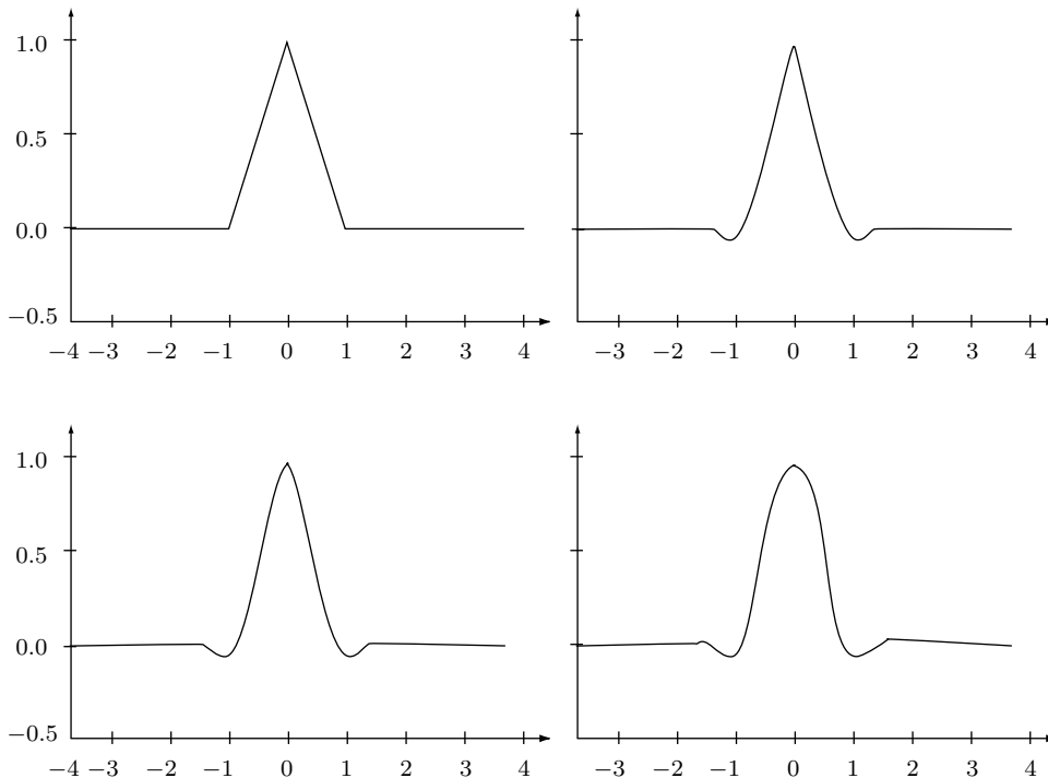
Figure 5.52: Scaling Functions \phi_{j,k}(x) for n=2, 4, 6, and 8 .
