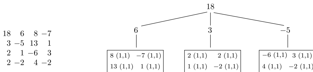
Figure 5.60: Sixteen Coefficients and One Spatial Orientation Tree.
