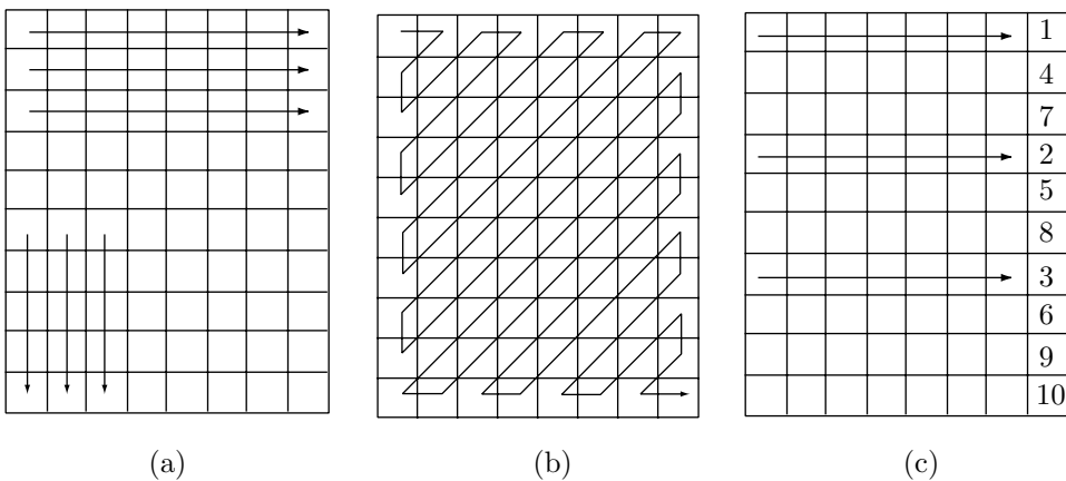
Figure 1.8: RLE Scanning.
