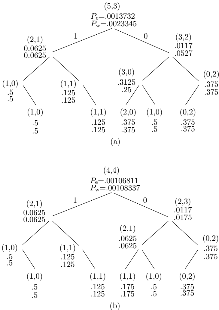
Figure 2.83: Context Trees for b_t = 0, 1 .
