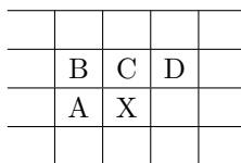
Figure 4.140: Pixel Prediction.
