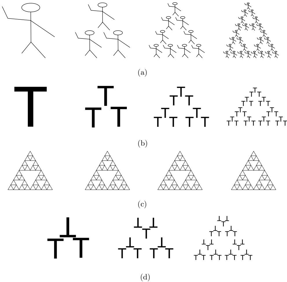
Figure 4.185: Creating the Sierpiński Gasket.
