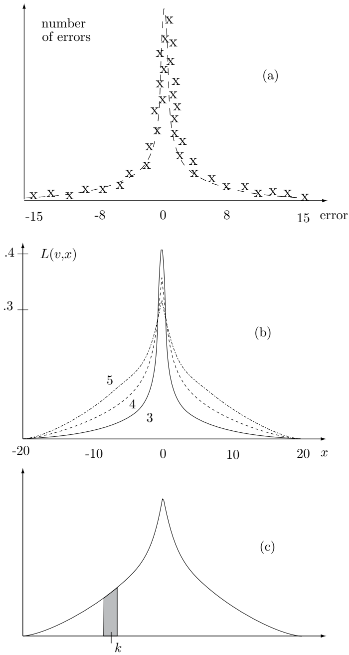
Figure 4.128: (a) Error Distribution. (b) Laplace Distributions. (c) Probability of k .
