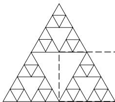
Figure 4.186: A Self-Similar Image.
