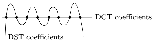
Figure 4.51: The DCT and DST of Eight Identical Data Values.
