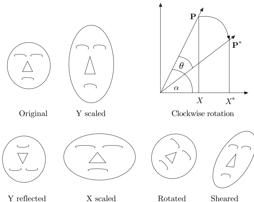
Figure 4.180: Two-Dimensional Transformations.
