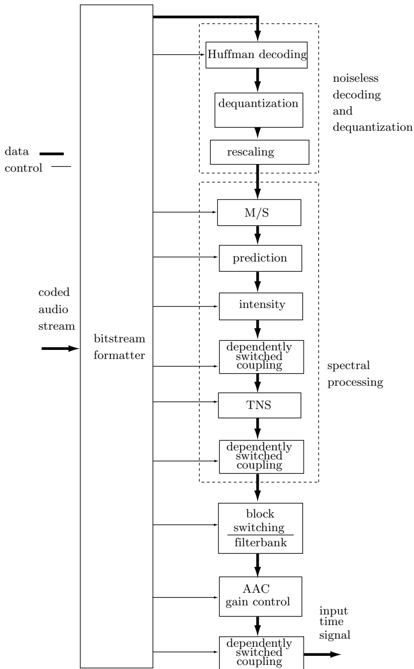
Figure 7.73: AAC Decoder.
