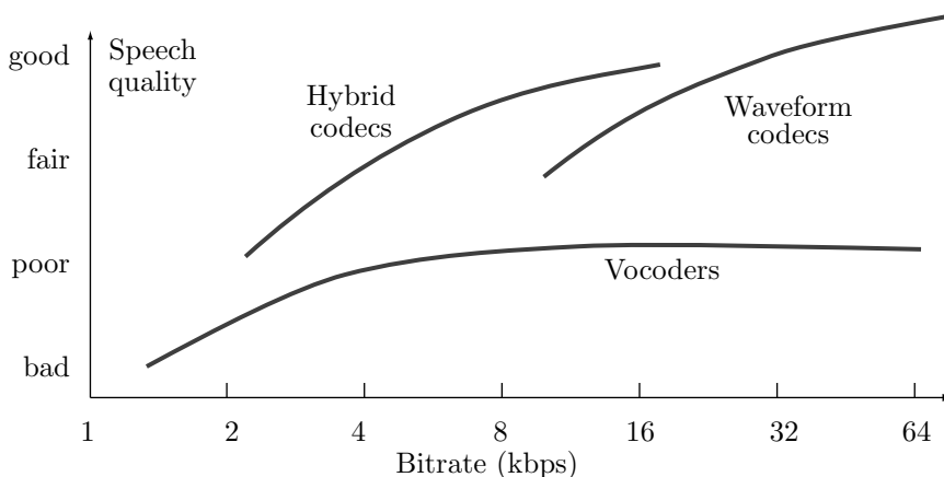
Figure 7.25: Speech Quality Versus Bitrate for Speech Codecs.
