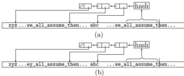
Figure 2.77: Unbounded-Length Deterministic Contexts in PPMZ.
