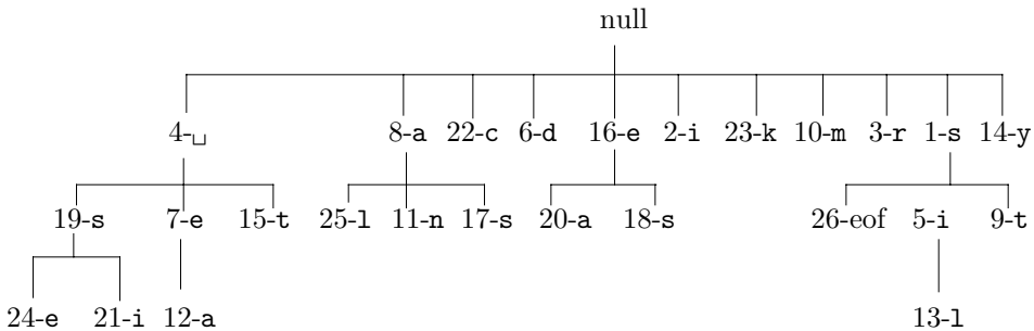
Figure 3.11: An LZ78 Dictionary Tree.
