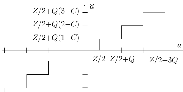
Figure 5.67: WSQ Scalar Quantization.
