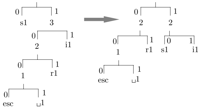
Figure Ans.13: Exercise 2.25. Part I.
