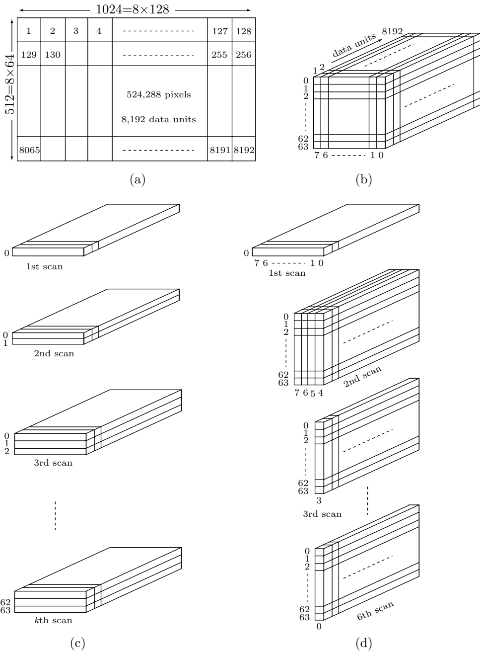
Figure 4.59: Scans in the JPEG Progressive Mode.
