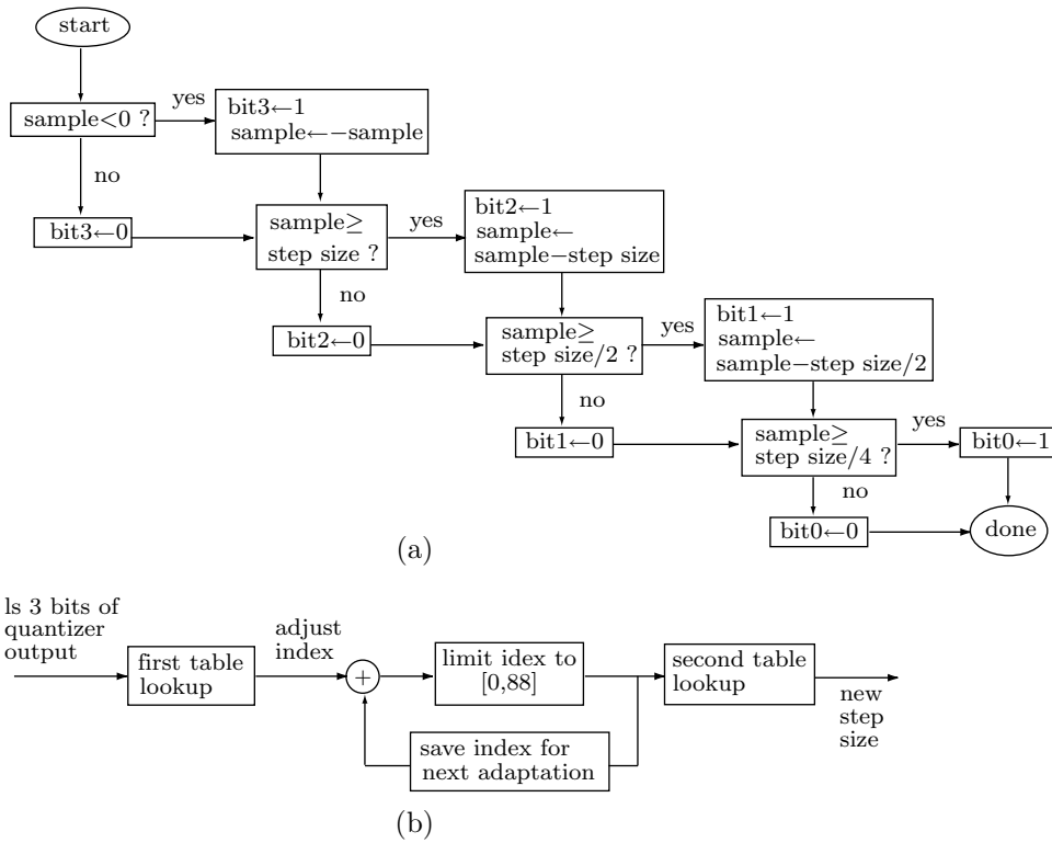
Figure 7.19: (a) IMA ADPCM Quantization. (b) Step Size Adaptation.
