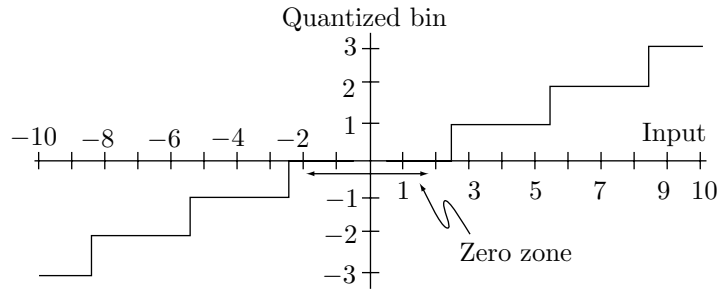
Figure 4.146: Quantization in BTPC.
