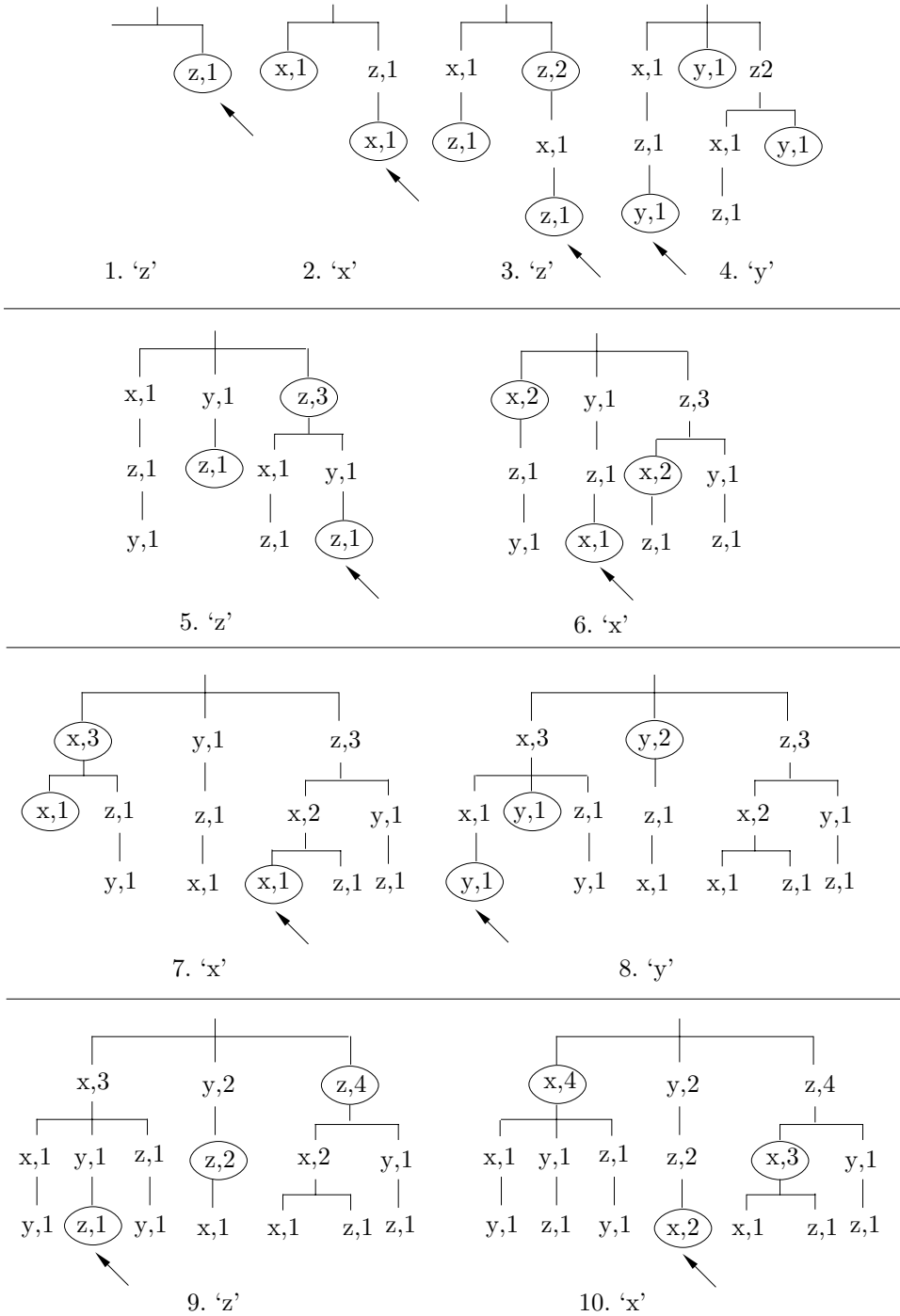
Figure 2.74: Ten Tries of "zxzyzxyzx".
