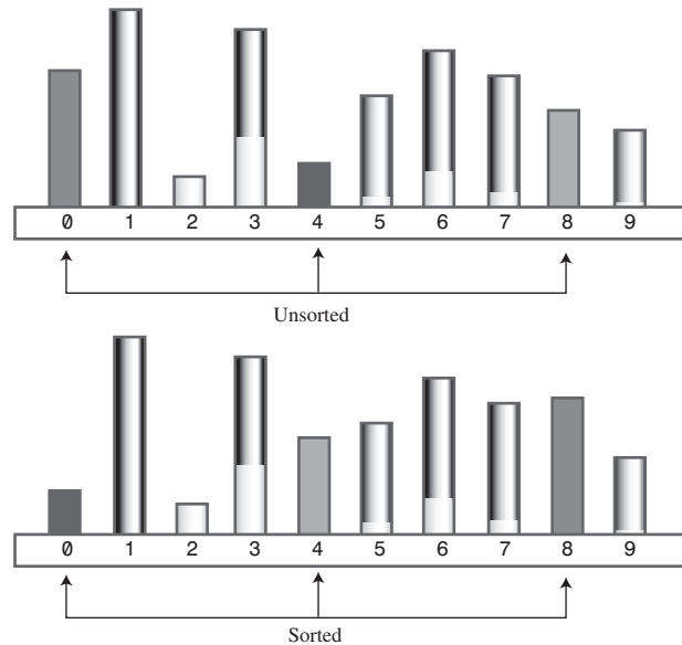
FIGURE 7.1 4-sorting 0, 4, and 8.
