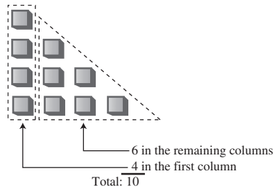
FIGURE 6.3 Triangular number as column plus triangle.
