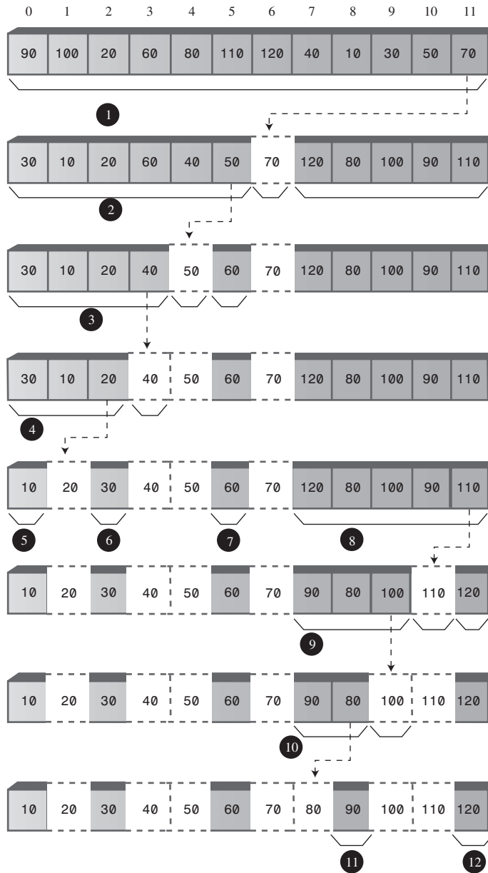
FIGURE 7.12 The quicksort process.
