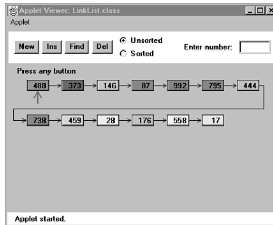
FIGURE 5.3 The LinkList Workshop applet.
