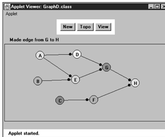
FIGURE 13.13 The GraphD workshop applet.
