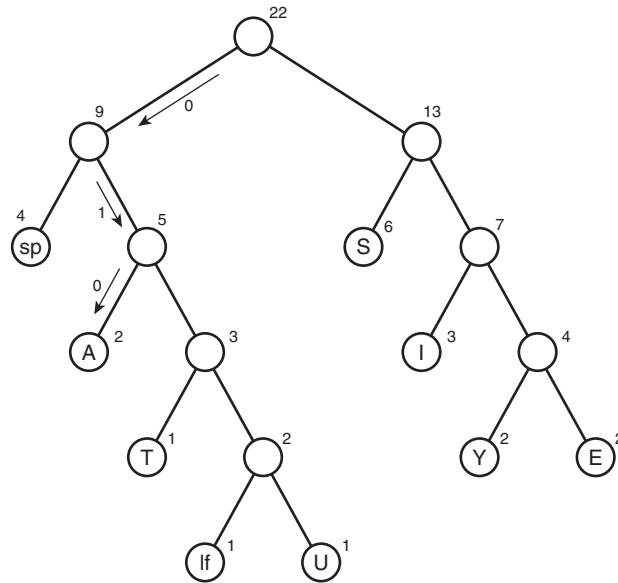
FIGURE 8.23 Huffman tree.
