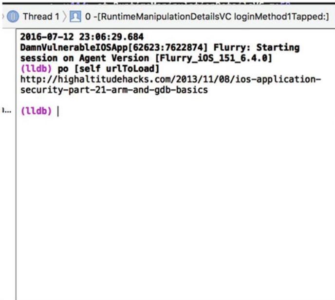
Figure 5-18. Reading variables using LLDB
