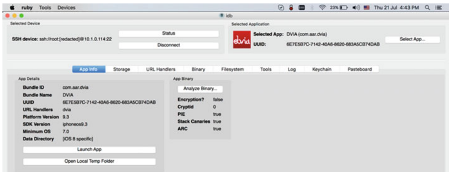
Figure 6-4. DVIA pen-testing
