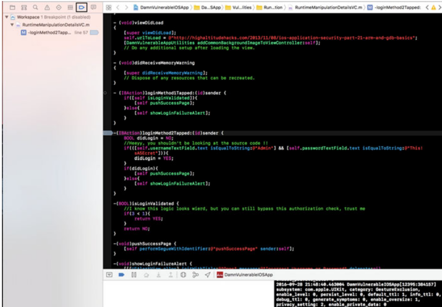
Figure 5-13. LLDB triggering
