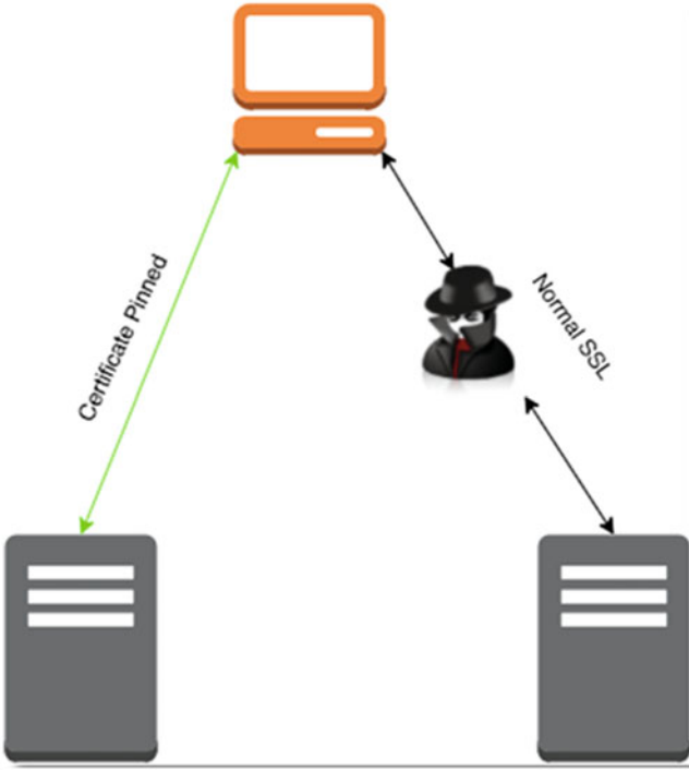
Figure 7-2. SSL Pinning
