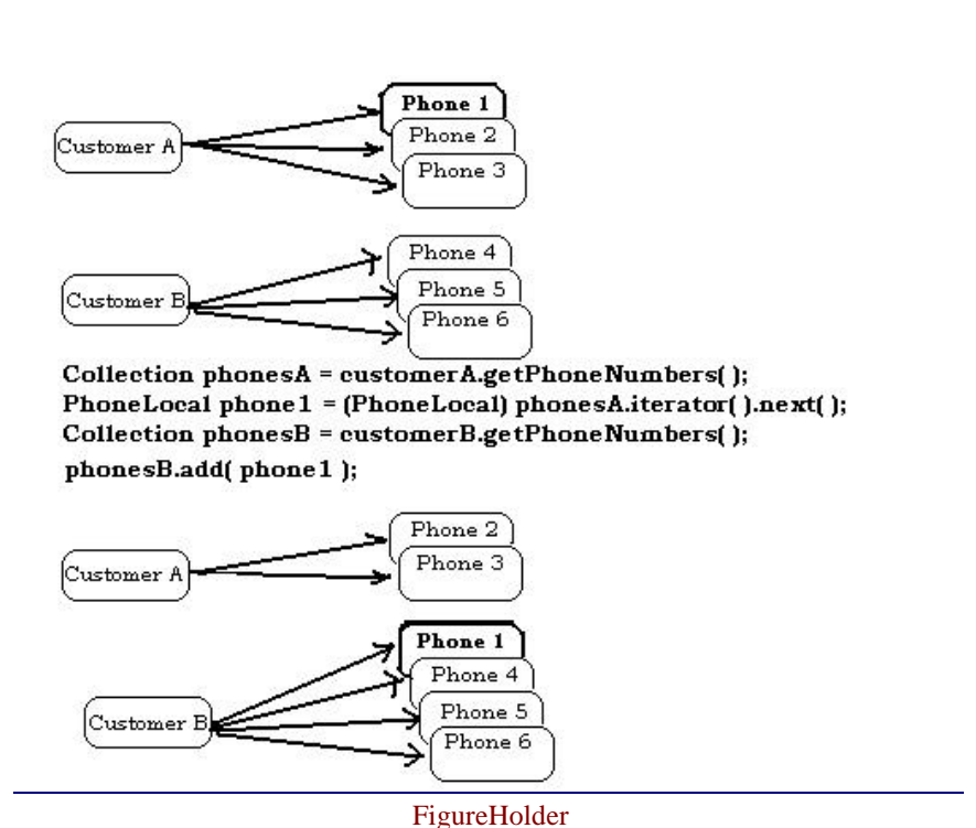
Figure 7-11: Exchanging a bean in a One-to-One unidirectional Relationship
