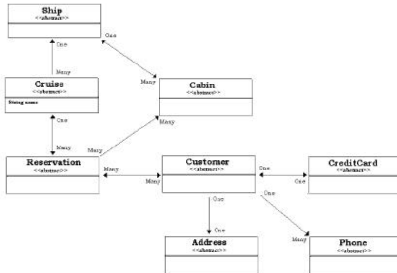
Figure 8-1: Titan Cruises Class Diagram
