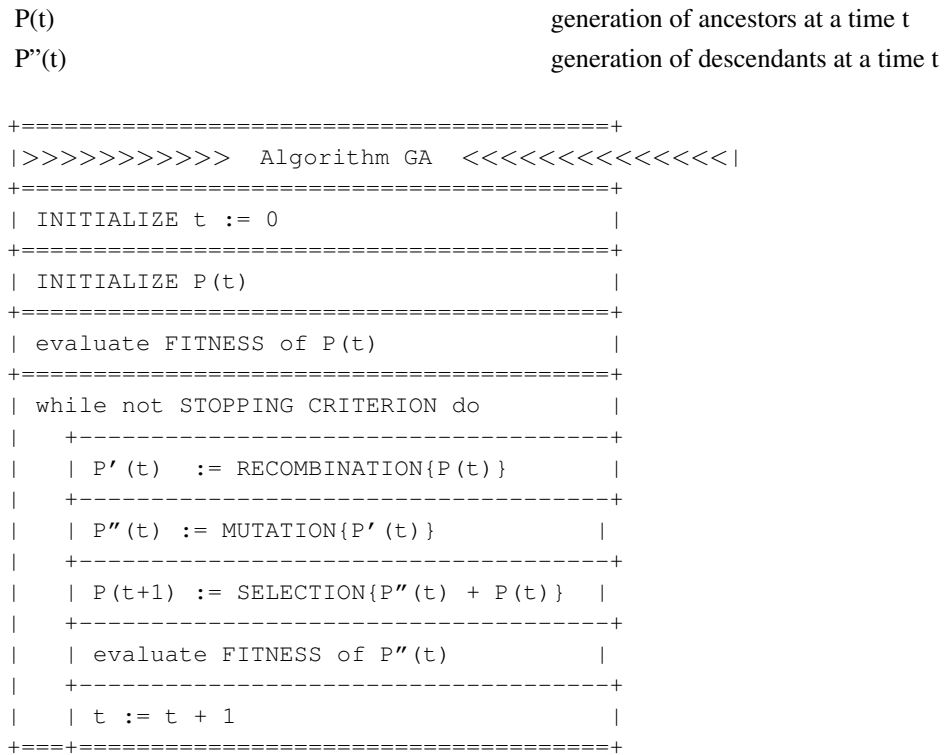
Figure 49-1. Structured Diagram of a Genetic Algorithm
