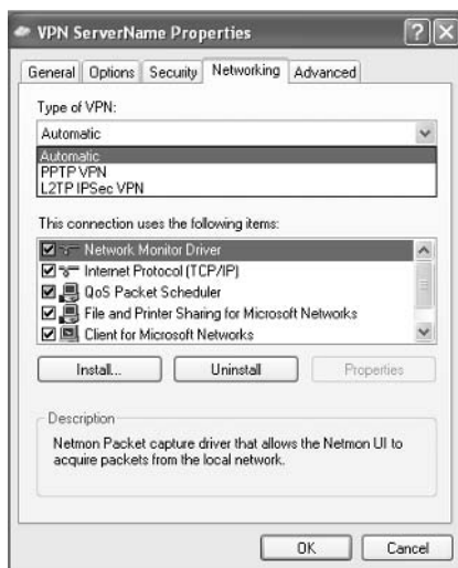
FIGURE 8.6 VPN types
