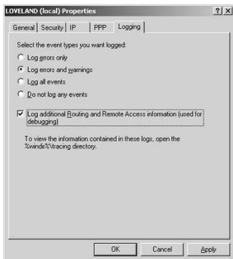
FIGURE 8.5 Event logging
