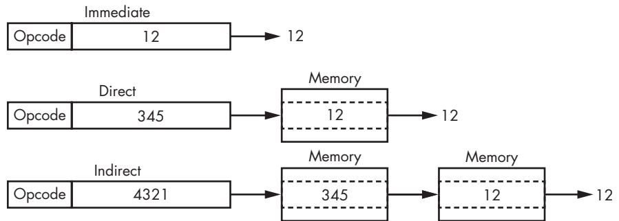
Figure 4-16: Addressing modes
