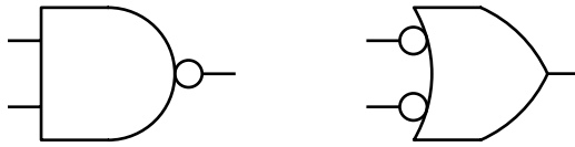
Figure 2-28: Redrawing a NAND gate using De Morgan's law
