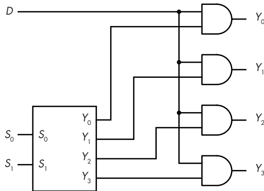
Figure 2-45: A 1:4 demultiplexer
