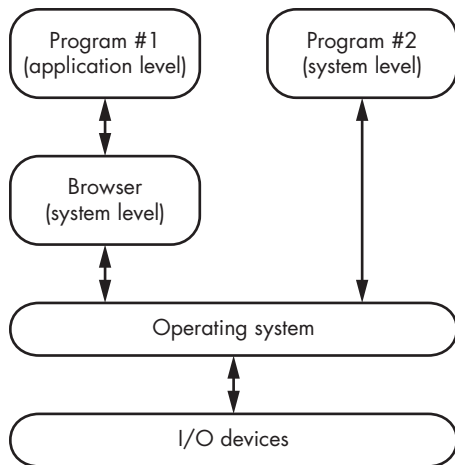
Figure 10-1: Two program scenarios
