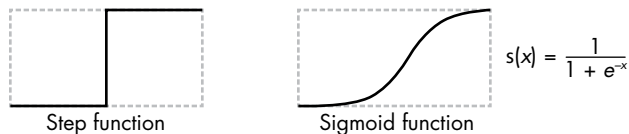
Figure 14-31: Artificial neuron transfer functions
