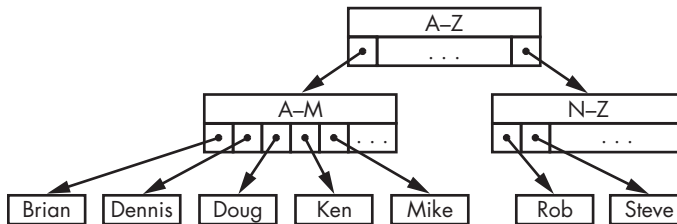
Figure 7-31: B-tree
