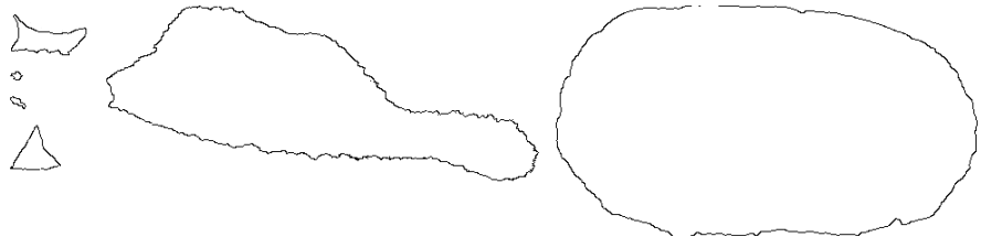
Figure 14-22: Extracted features
