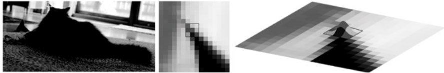
Figure 14-5: Gaussian blur
