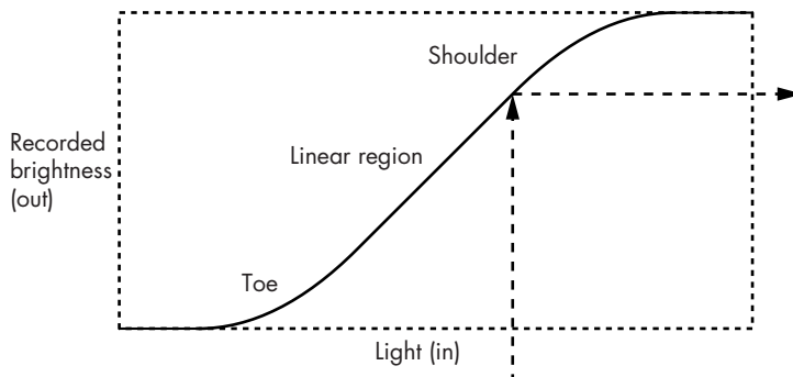
Figure 2-4: Camera sensor or film transfer function
