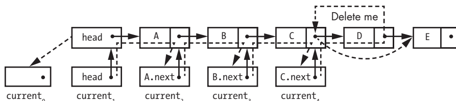
Figure 7-16: Singly linked list deletion in action
