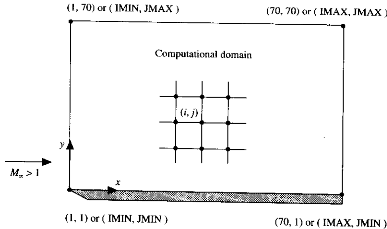
FIG. 10.3 Computational domain.
