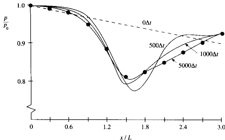
FIG. 7.17 Variation of the pressure distribution through the nozzle at different times; purely subsonic flow case with p_e/p_0 = 0.93 . Circles indicate exact analytical values.
