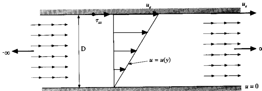
FIG. 9.1 Schematic of Couette flow.
