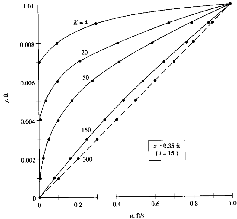
FIG. 9.10 Velocity profiles for the x component of velocity as a function of vertical distance across the duct. Profiles are shown for various iteration numbers, ranging from 4 to 300. At K = 300 , the velocity profile has converged to the Couette flow solution.
