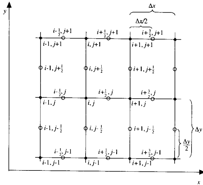
FIG. 6.15 Staggered grid.
