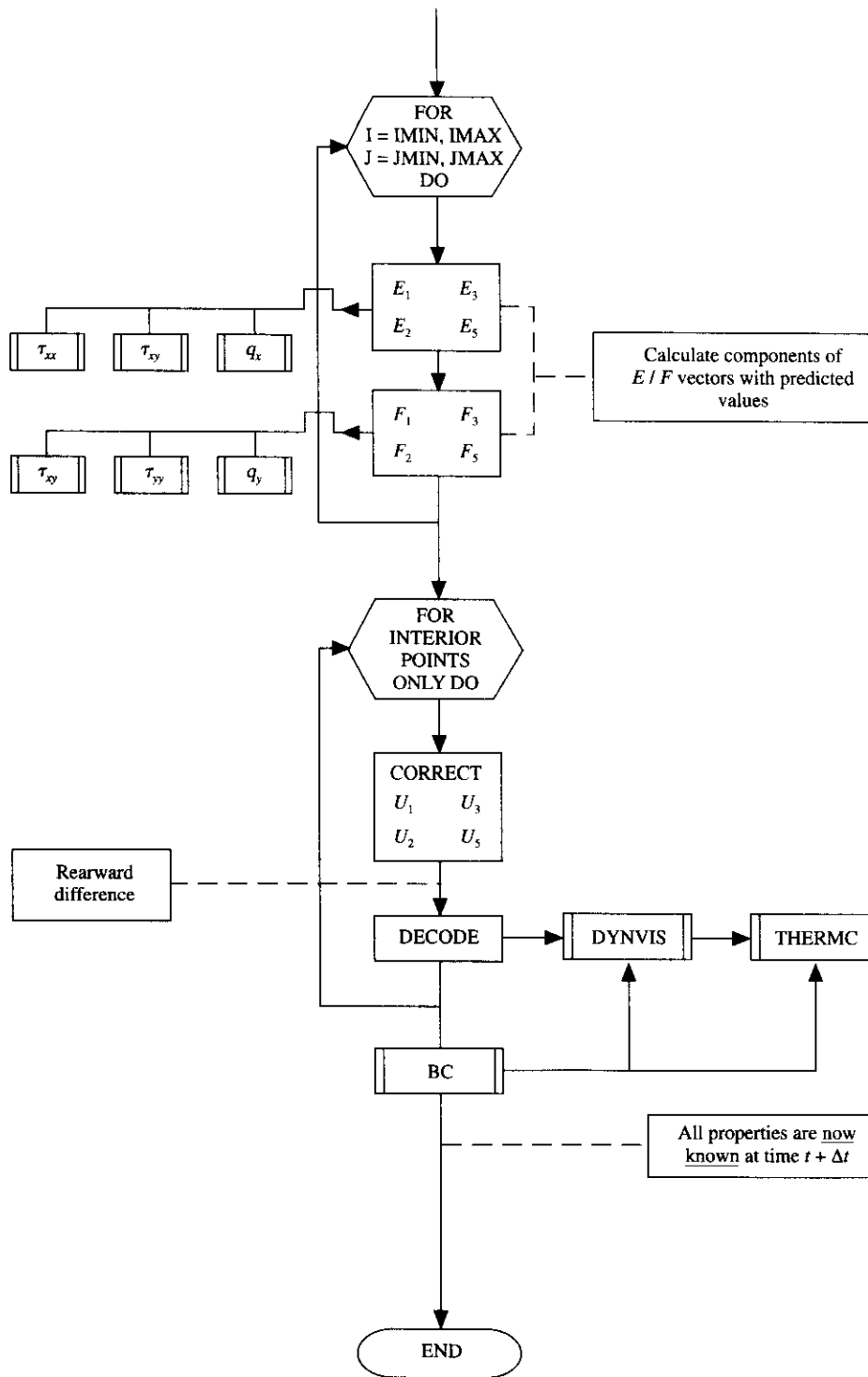
FIG. 10.8 Flowchart for MacCormack's (MAC) subroutine.
