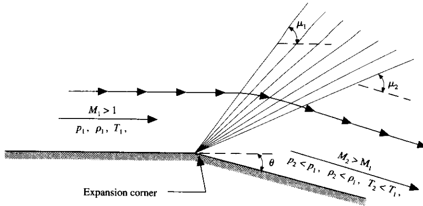
FIG. 8.1 Centered Prandtl-Meyer expansion wave.
