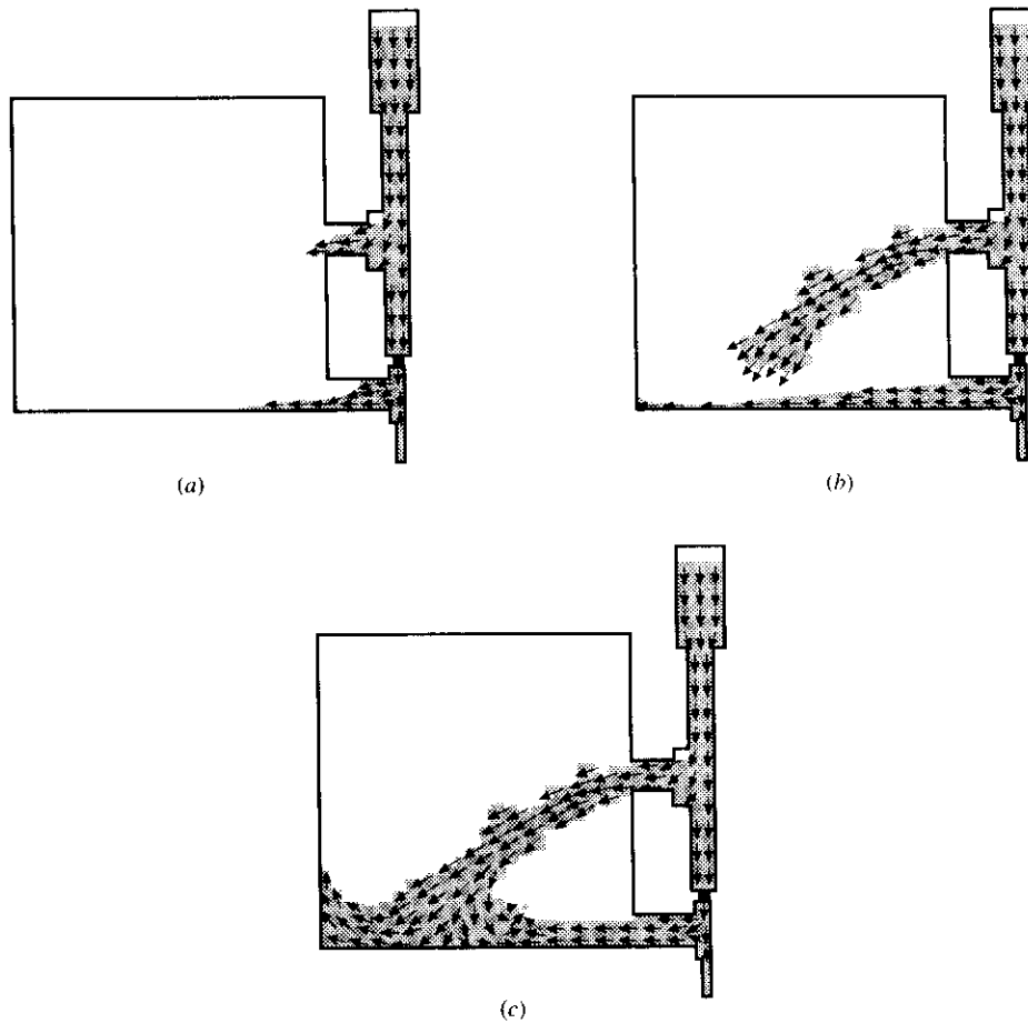
FIG. 1.15 Computed results at three different times for the velocity field set up by liquid iron flowing into a mold from two gates on the right side of the mold. (After Ref. 61.)
