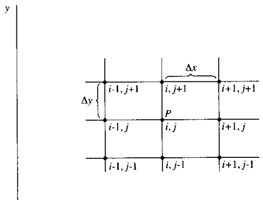
FIG. 4.1 Discrete grid points.
