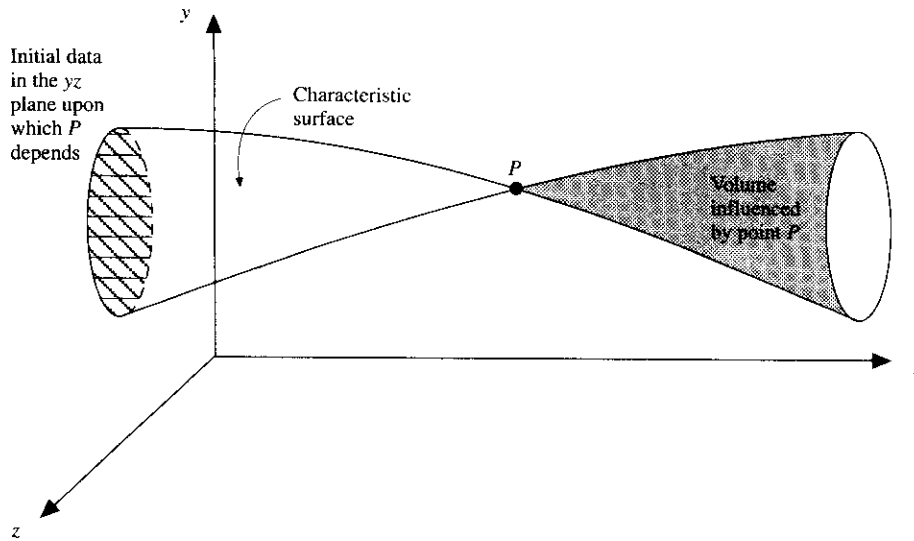
FIG. 3.5 Domain and boundaries for the solution of hyperbolic equations. Three-dimensional steady flow.
