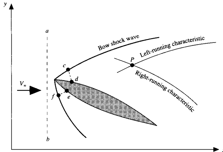
FIG. 3.4 Illustration of initial data lines for the method of characteristics.
