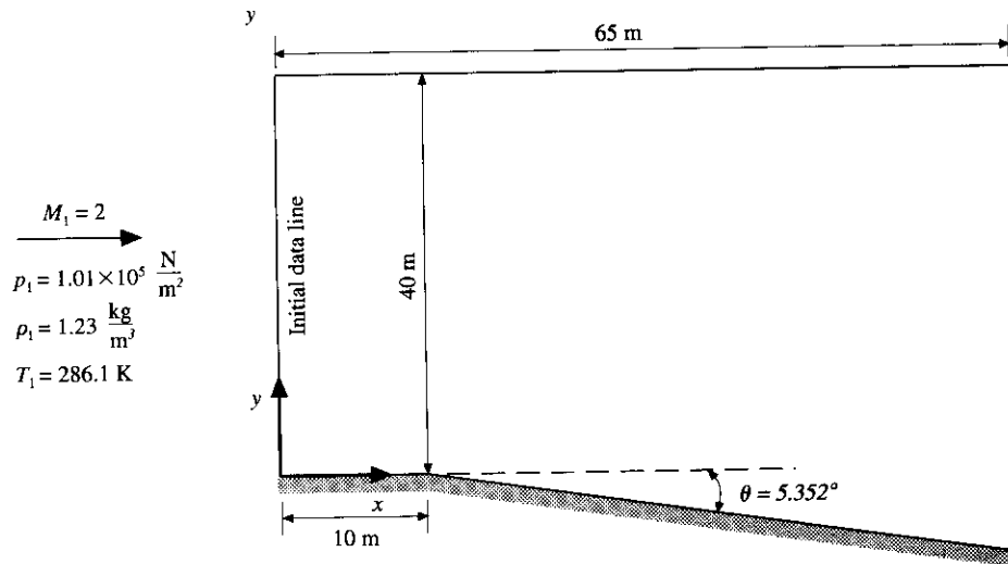
FIG. 8.4 Physical plane, drawn to scale.
