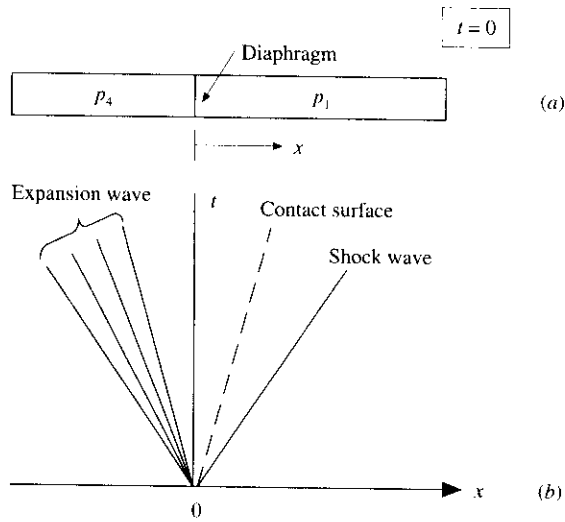
FIG. 11.6 Wave diagram.
