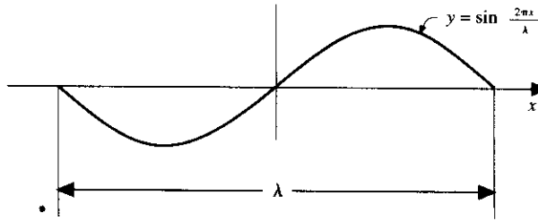
FIG. 4.10 Sine function.
