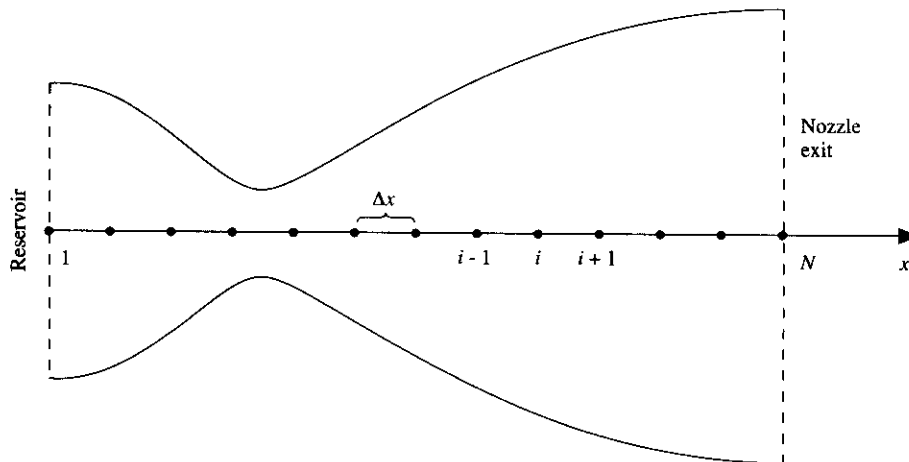
FIG. 7.5 Grid point distribution along the nozzle.
