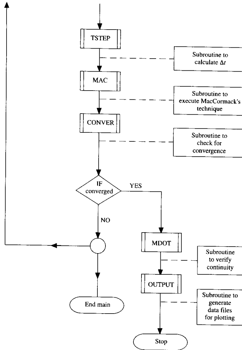
FIG. 10.7 Flowchart for the main program (MAIN).
