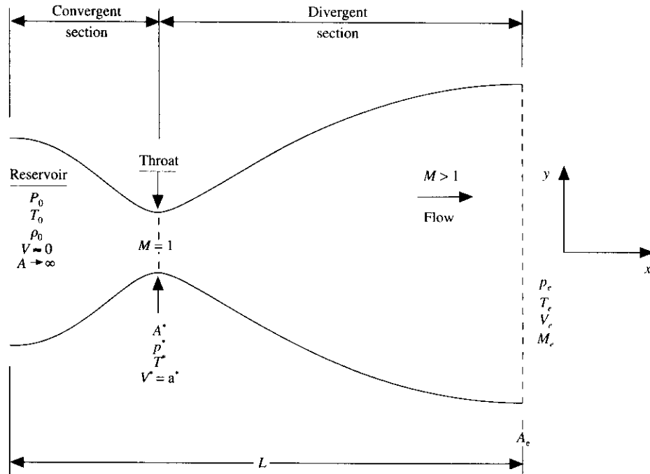
FIG. 7.1 Schematic for subsonic-supersonic isentropic nozzle flow.
