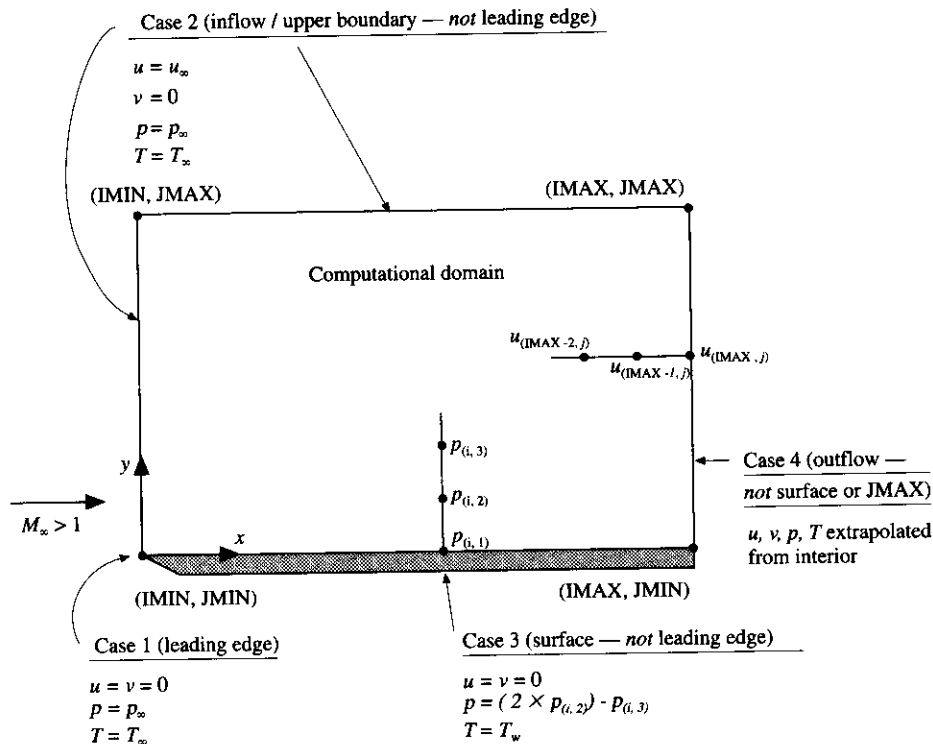
FIG. 10.5 Application of boundary conditions.
