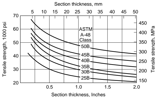
Fig. 6.3.3 The influence of casting section thickness on the tensile strength and hardness for a series of gray irons classified by their strength as cast in 1.2-in (30-mm)-diameter, B bars. (Steel Founders Society of America.)
