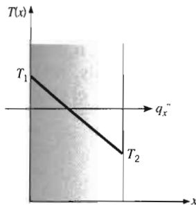
FIGURE 2.2 The relationship between coordinate system, heat flow direction, and temperature gradient in one dimension.
