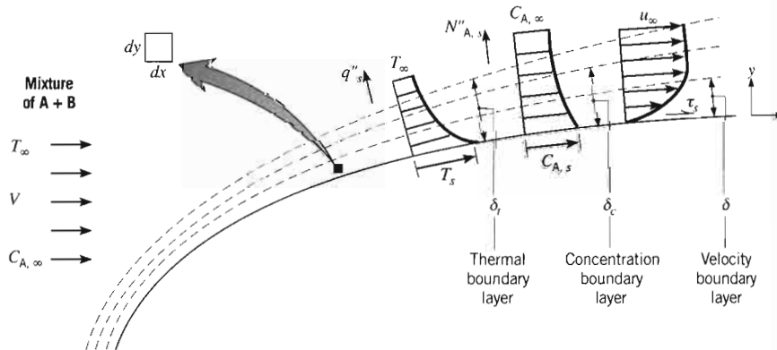
FIGURE 6.9 Development of the velocity, thermal, and concentration boundary layers for an arbitrary surface.
