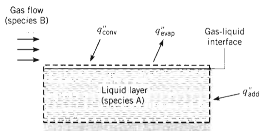
FIGURE 6.10 Latent and sensible heat exchange at a gas-liquid interface.
