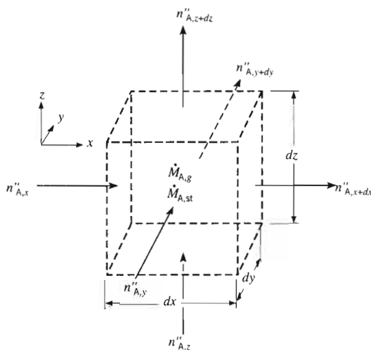
FIGURE 14.4 Differential control volume, dx dy dz , for species diffusion analysis in Cartesian coordinates.
