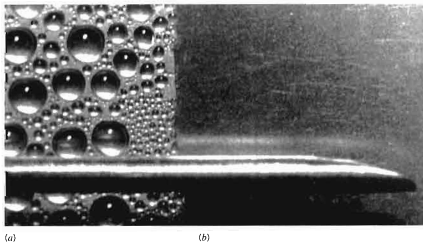
FIGURE 10.10 Condensation on a vertical surface. (a) Dropwise. (b) Film. Photograph courtesy of Professor J. W. Westwater, University of Illinois at Champaign-Urbana.
