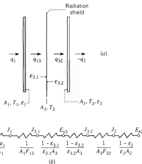
FIGURE 13.11 Radiation exchange between large parallel planes with a radiation shield. (a) Schematic. (b) Network representation.
