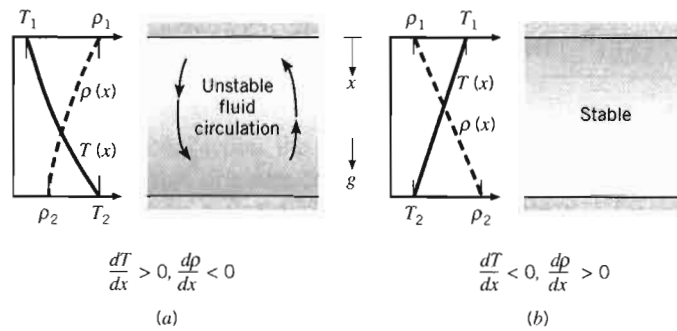
FIGURE 9.1 Conditions in a fluid between large horizontal plates at different temperatures. (a) Unstable temperature gradient. (b) Stable temperature gradient.
