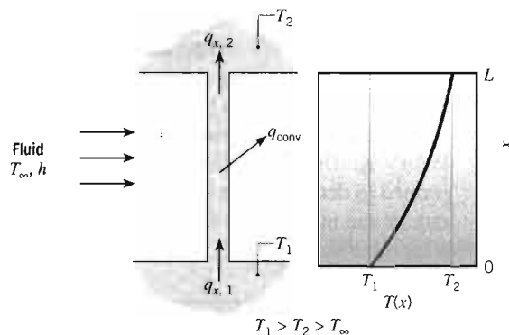
FIGURE 3.11 Combined conduction and convection in a structural element.
