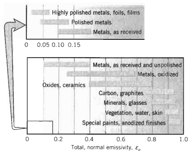
FIGURE 12.19 Representative values of the total, normal emissivity \epsilon_n .
