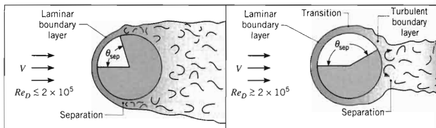
FIGURE 7.7 The effect of turbulence on separation.
