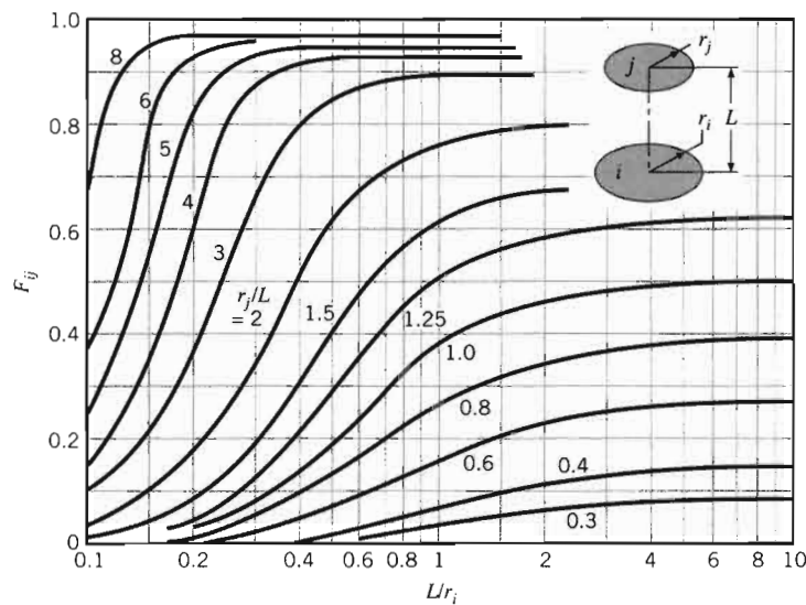
FIGURE 13.5 View factor for coaxial parallel disks.
