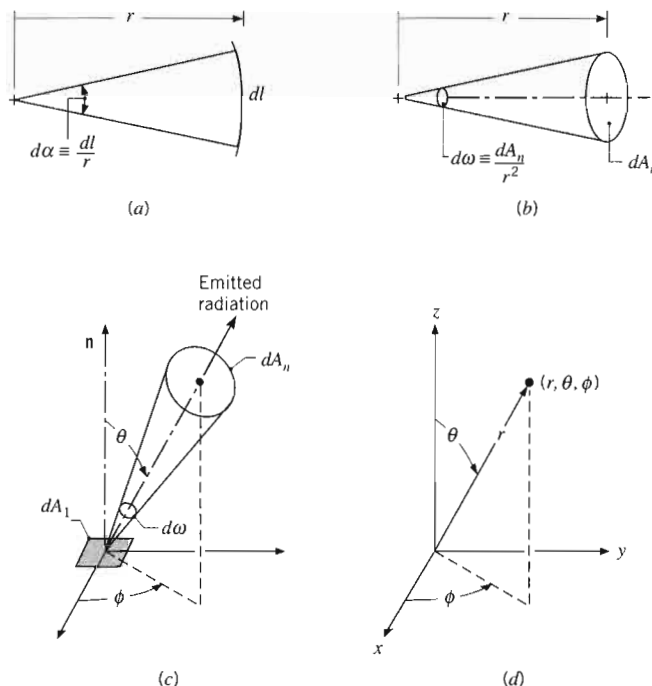
FIGURE 12.5 Mathematical definitions. (a) Plane angle. (b) Solid angle. (c) Emission of radiation from a differential area dA_1 into a solid angle d\omega subtended by dA_n at a point on dA_n . (d) The spherical coordinate system.
