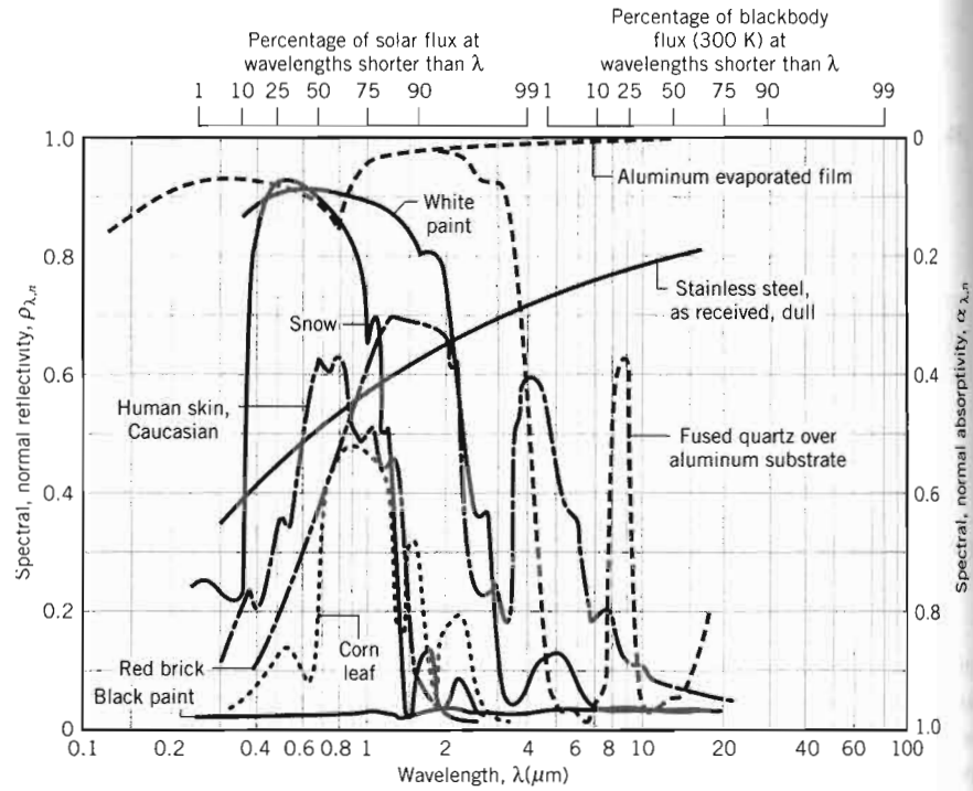
FIGURE 12.22 Spectral dependence of the spectral, normal absorptivity \alpha_{\lambda,n} and reflectivity \rho_{\lambda,n} of selected opaque materials.
