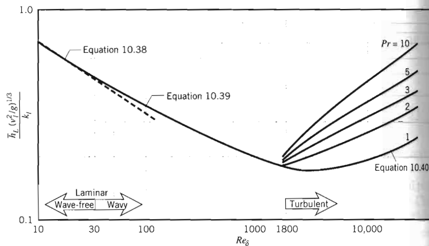
FIGURE 10.13 Modified Nusselt number for condensation on a vertical plate.
