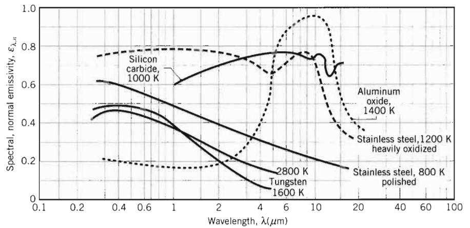
FIGURE 12.17 Spectral dependence of the spectral, normal emissivity \epsilon_{\lambda,n} of selected materials.
