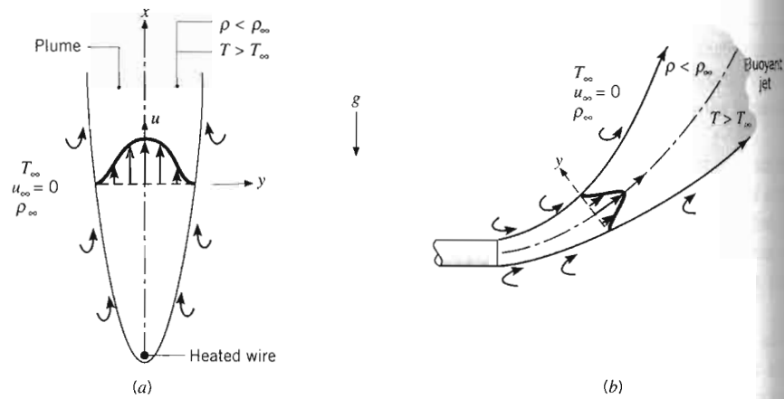
FIGURE 9.2 Buoyancy-driven free boundary layer flows in an extensive, quiescent medium. (a) Plume formation above a heated wire. (b) Buoyant jet associated with a heated discharge.
