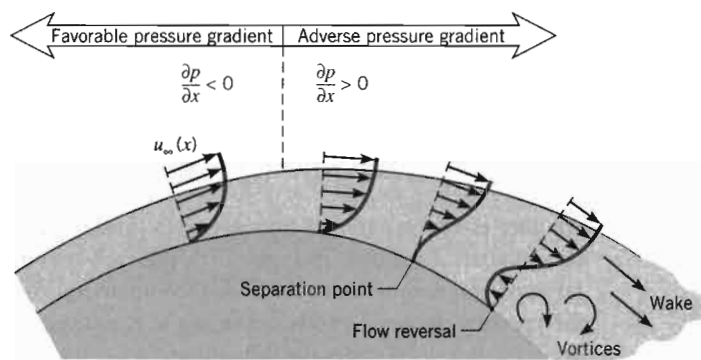
FIGURE 7.6 Velocity profile associated with separation on a circular cylinder in cross flow.
