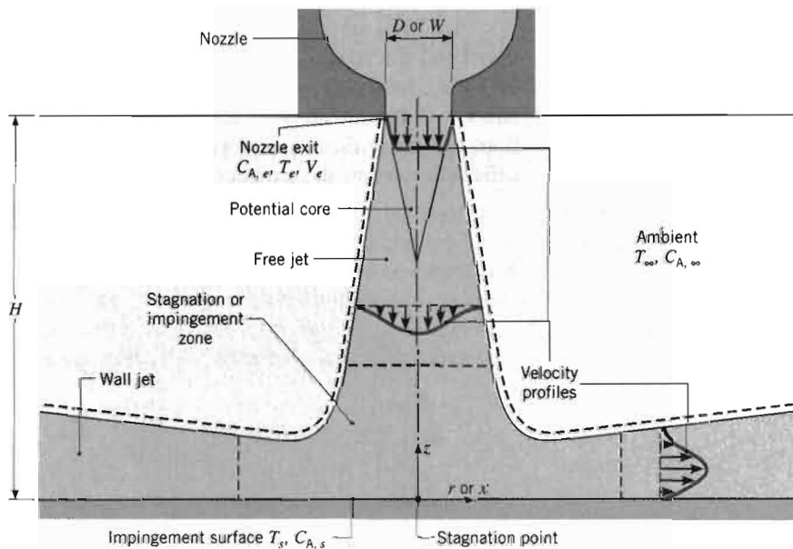
FIGURE 7.15 Surface impingement of a single round or slot gas jet.
