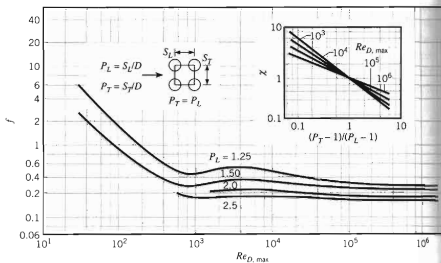
FIGURE 7.13 Friction factor f and correction factor \chi for Equation 7.69. In-line tube bundle arrangement [15]. Used with permission.
