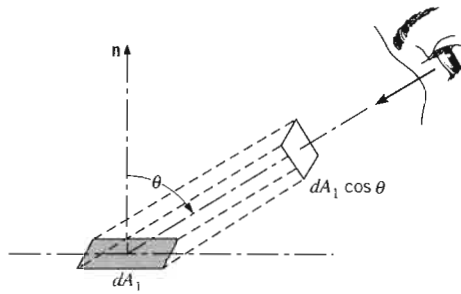
FIGURE 12.7 The projection of dA_1 normal to the direction of radiation.
