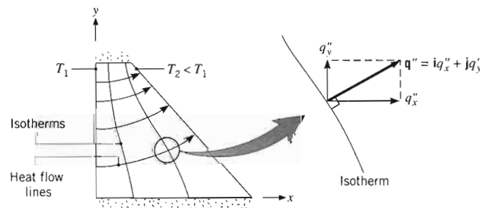
FIGURE 4.1 Two-dimensional conduction.
