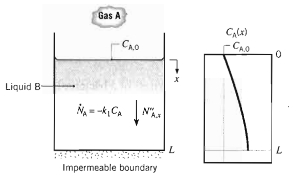
FIGURE 14.8 Diffusion and homogeneous reaction of gas A in liquid B.
