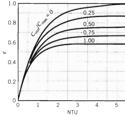
FIGURE 11.12 Effectiveness of a shell-and-tube heat exchanger with one shell and any multiple of two tube passes (two, four, etc. tube passes) (Equation 11.30).
