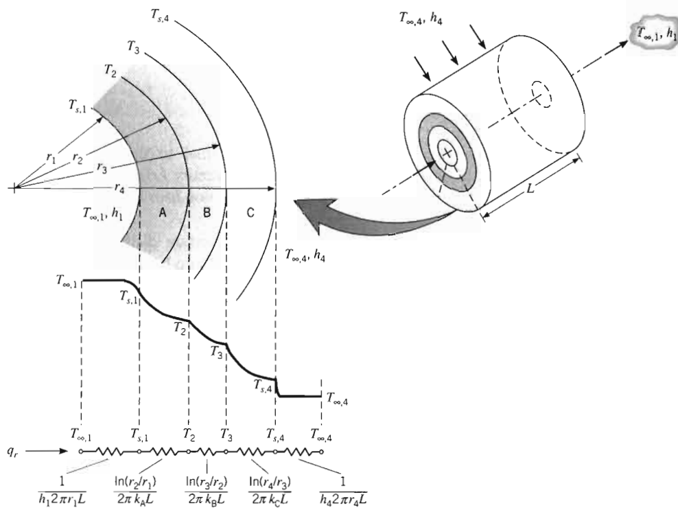
FIGURE 3.7 Temperature distribution for a composite cylindrical wall.
