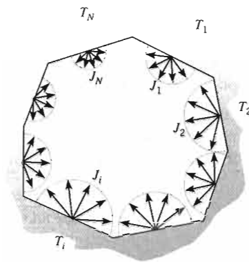
FIGURE 13.2 Radiation exchange in an enclosure.
