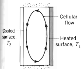
FIGURE 9.12 Cellular flow in a vertical cavity with different sidewall temperatures.
