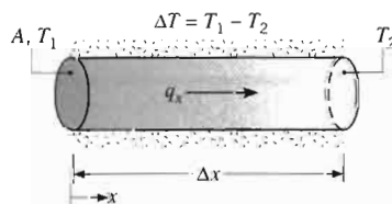
FIGURE 2.1 Steady-state heat conduction experiment.
