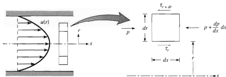
FIGURE 8.2 Force balance on a differential element for laminar, fully developed flow in a circular tube.
