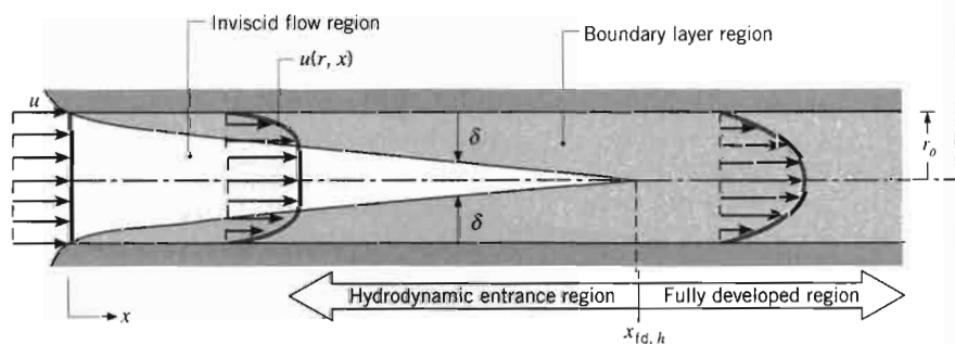
FIGURE 8.1 Laminar, hydrodynamic boundary layer development in a circular tube.
