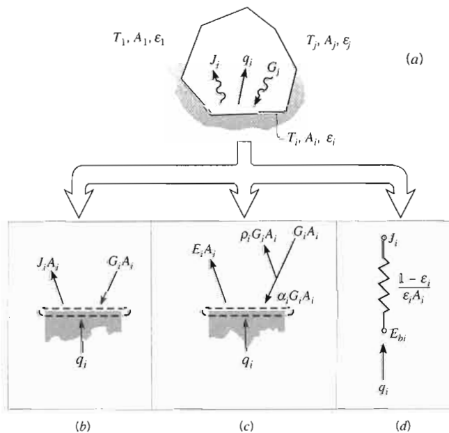
FIGURE 13.8 Radiation exchange in an enclosure of diffuse, gray surfaces with a nonparticipating medium. (a) Schematic of the enclosure. (b) Radiative balance according to Equation 13.9. (c) Radiative balance according to Equation 13.11. (d) Network element representing the net radiation transfer from a surface.
