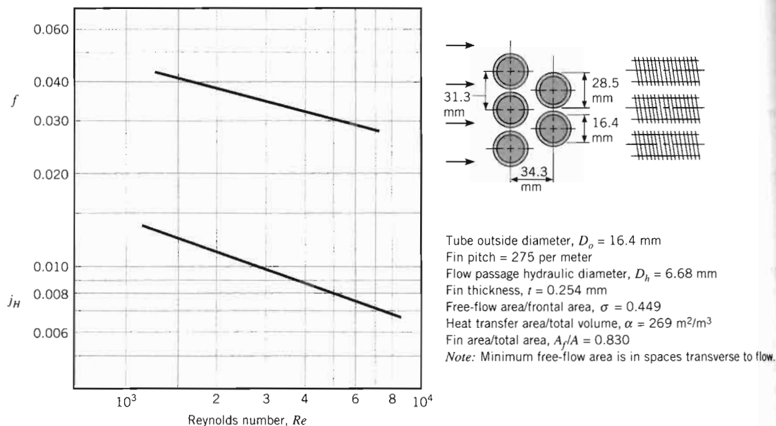
FIGURE 11.16 Heat transfer and friction factor for a circular tube–circular fin heat exchanger, surface CF-7.0-5/8J from Kays and London [5].
