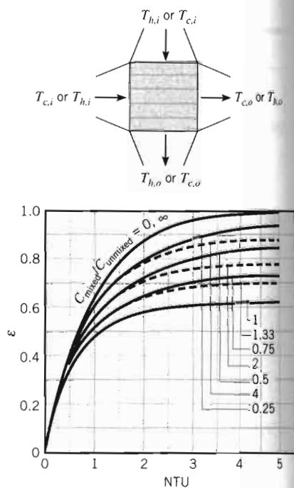
FIGURE 11.15 Effectiveness of a single-pass, cross-flow heat exchanger with one fluid mixed and the other unmixed (Equations 11.33, 11.34).
