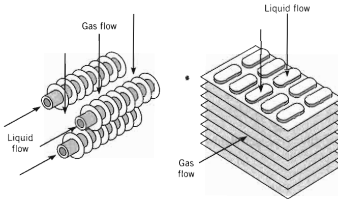
FIGURE 3.13 Schematic of typical finned-tube heat exchangers.
