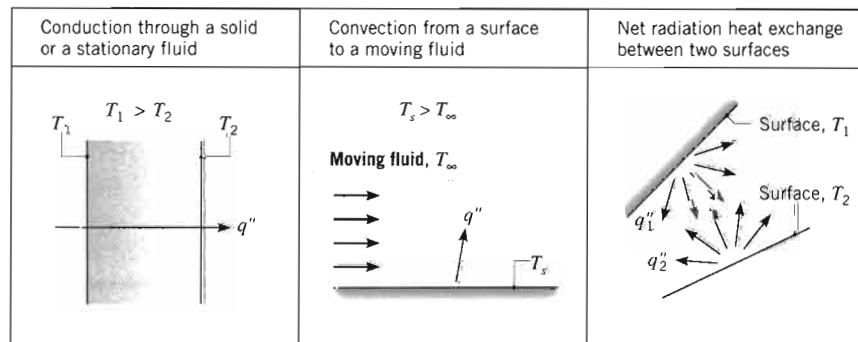
FIGURE 1.1 Conduction, convection, and radiation heat transfer modes.
