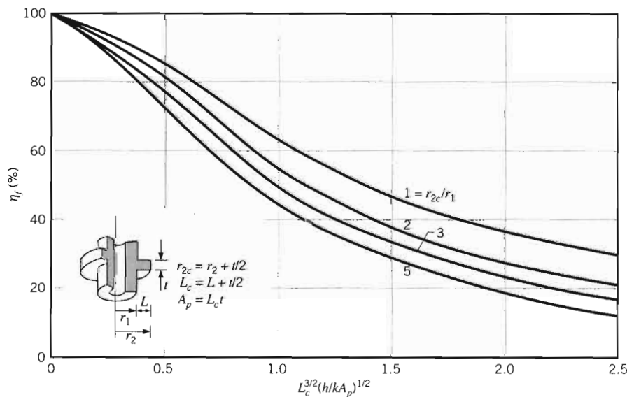
FIGURE 3.19 Efficiency of annular fins of rectangular profile.
