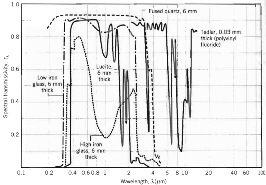
FIGURE 12.23 Spectral dependence of the spectral transmissivities \tau_{\lambda} of selected semitransparent materials.
