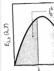
FIGURE 12.13 Emission from a band of the spectral band.
