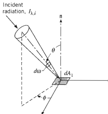
FIGURE 12.9 Directional nature of incident radiation.
