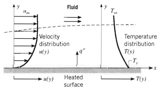
FIGURE 1.4 Boundary layer development in convection heat transfer.
