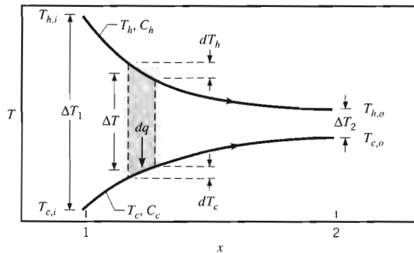
FIGURE 11.7 Temperature distributions for a parallel-flow heat exchanger.
