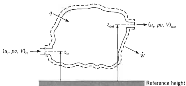
FIGURE 1.8 Conservation of energy for a steady-flow, open system.
