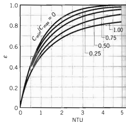
FIGURE 11.11 Effectiveness of a counterflow heat exchanger (Equation 11.29).
