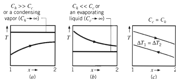
FIGURE 11.9 Special heat exchanger conditions. (a) C_h \gg C_c or a condensing vapor ( C_h \rightarrow \infty ). (b) An evaporating liquid or C_h \ll C_c . (c) A counterflow heat exchanger with equivalent fluid heat capacities ( C_h = C_c ).
