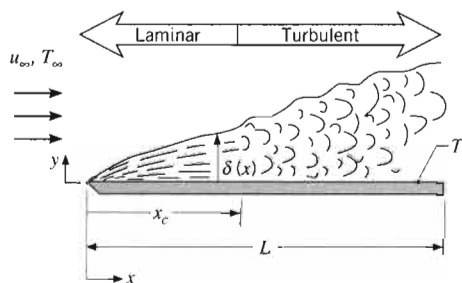
FIGURE 7.3 The flat plate in parallel flow.
