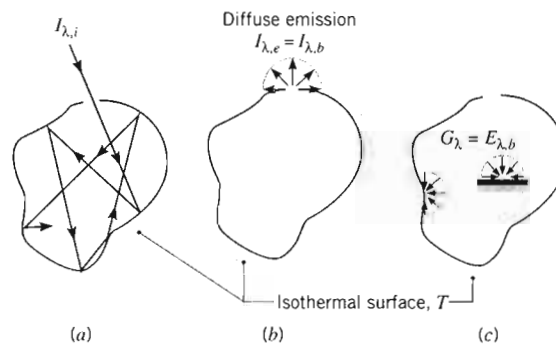
FIGURE 12.11 Characteristics of an isothermal blackbody cavity. (a) Complete absorption. (b) Diffuse emission from an aperture. (c) Diffuse irradiation of interior surfaces.
