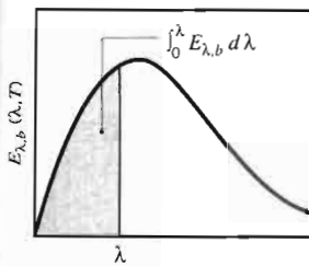
FIGURE 12.13 Radiation emission from a blackbody in the spectral band 0 to \lambda .
