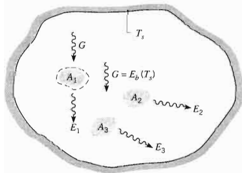
FIGURE 12.24 Radiative exchange in an isothermal enclosure.
