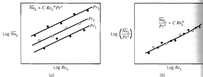
FIGURE 7.2 Dimensionless representation of convection heat transfer measurements.
