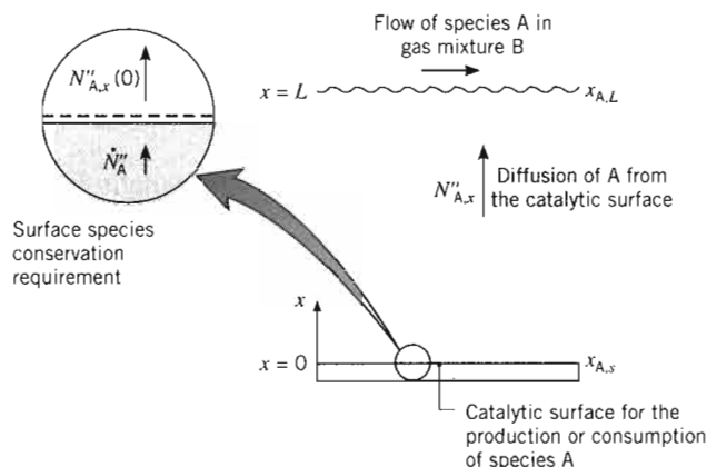
FIGURE 14.7 One-dimensional diffusion with heterogeneous catalysis.
