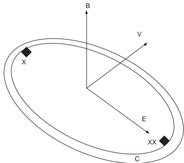
Figure 2 Sketch showing the Faraday effect, which forms the basis of the electromagnetic current meter. The effect results in a potential difference E = BVL induced between two electrodes (X and XX) with a separation L when a conductor (sea water) moves at a resolved velocity V perpendicular to the line X-XX and perpendicular to a magnetic field with a flux density of B induced by coil C.
