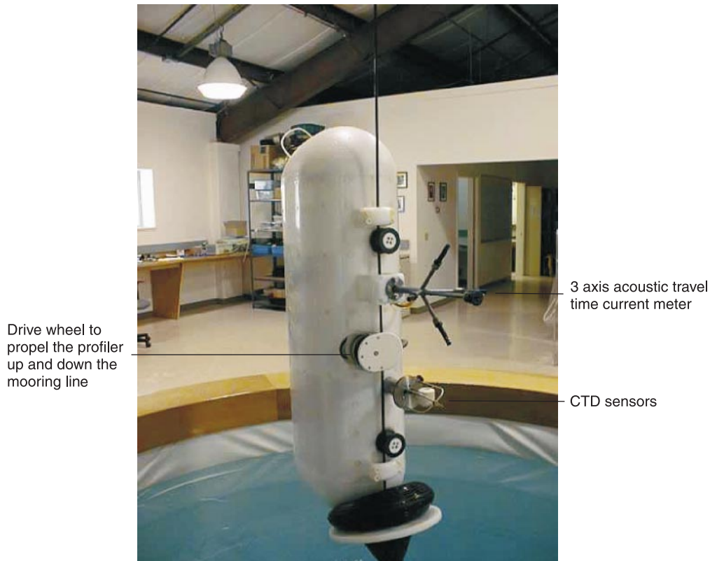
Figure 3 Acoustic travel time current meter as one instrument among many on a package capable of crawling up and down a wire mooring to obtain profiles of properties in water depths of up to 5000m. (Illustration courtesy of McLane Research Inc.)
