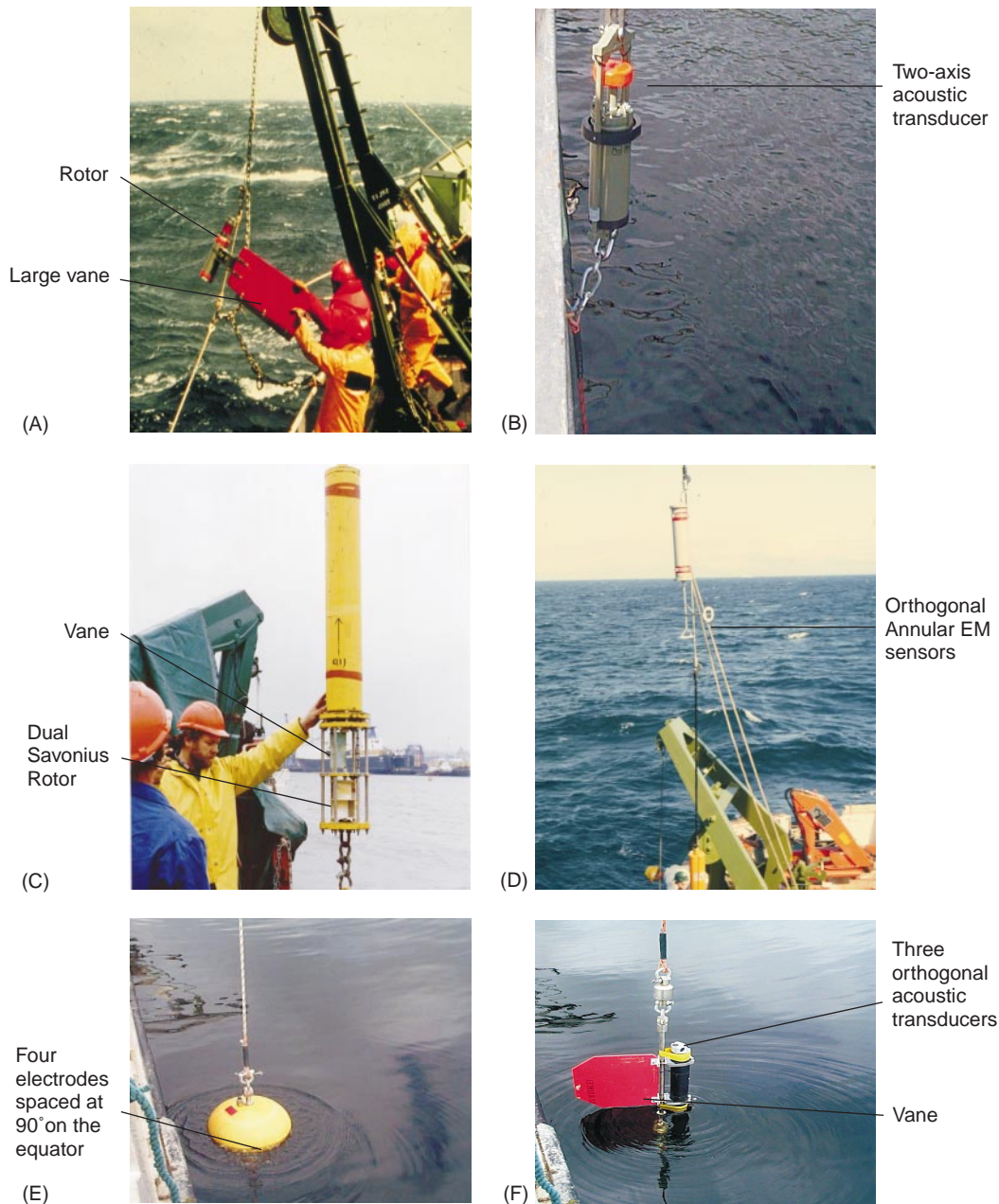
Figure 1 Current meters based on different sensors. (A) Aanderaa RCM4 deep ocean rotor-vane instrument; (B) Aanderaa RCM9 single cell Doppler current meter; (C) EG&G Vector averaging current meter with dual Savonius rotor (at the base) and small vane (immediately above); (D) Vector averaging electromagnetic current meter based on an annular sensor; (E) Interocean S4 electromagnetic current meter; (F) Nortek Aquadopp high precision single cell Doppler instrument, capable of measuring horizontal and vertical currents.
