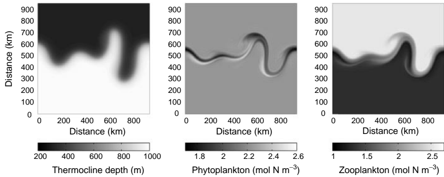
Figure 9 Results from a coupled model of the Gulf Stream: thermocline depth (left), phytoplankton concentration (middle), and zooplankton concentration (right). (Courtesy of GR Flierl, Massachusetts Institute of Technology.)
