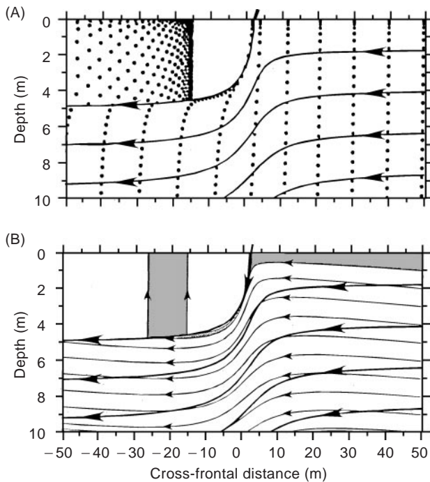
Figure 13 Surface-seeking organisms aggregating at a propagating front. Modeled particle locations (dots, panel (A)) and particle streamlines (thin lines, panel (B)) in the cross-frontal flow. The front is centered at x = 0 , and the coordinate system translates to the right with the motion of the front. Flow streamlines are represented in both panels as bold lines; they differ from particle streamlines due to propagation of the front. The shaded area in (B) indicates the region in which cells are focused into the frontal zone, forming a dense band at x = -20 m. (Reproduced with permission from Franks, 1997.)
