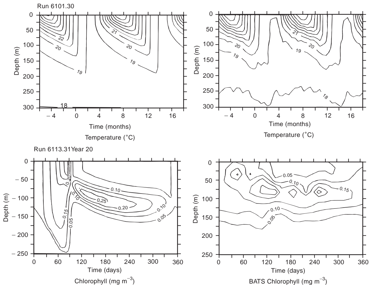
Figure 6 Simulated (left) and observed (right) seasonal cycles of temperature and chlorophyll at the BATS site. (Reproduced with permission from Doney SC, Glover DM and Najjar RG (1996) A new coupled, one-dimensional biological-physical model for the upper ocean: applications to the JGOFS Bermuda Atlantic Time-series Study (BATS) site. Deep-Sea Research II 43: 591-624.)
