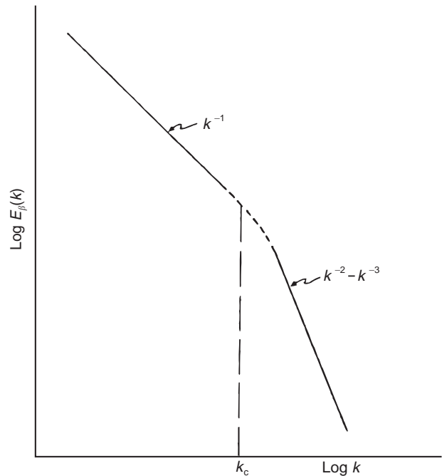
Figure 3 A theoretical spectrum for the spatial variability of phytoplankton, E_p(k) , as a function of wavenumber, k , displayed on a log-log plot. To the left of the critical wavenumber k_c , biological processes dominate, resulting in a k^{-1} dependence. The high wavenumber region to the right of k_c where turbulent motions dominate, has a dependence between k^{-2} and k^{-3} . (Reproduced with permission from Denman KL and Platt T (1976). The variance spectrum of phytoplankton in a turbulent ocean. Journal of Marine Research 34: 593–601.)
