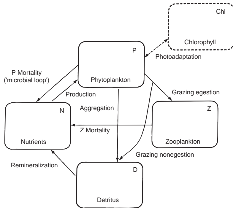
Figure 5 A four-compartment planktonic ecosystem model showing the pathways for nitrogen flow. (Reproduced with permission from Doney SC, Glover DM and Najjar RG (1996) A new coupled, one-dimensional biological-physical model for the upper ocean: applications to the JGOFS Bermuda Atlantic Time-series Study (BATS) site. Deep-Sea Research II 43: 591–624.)
