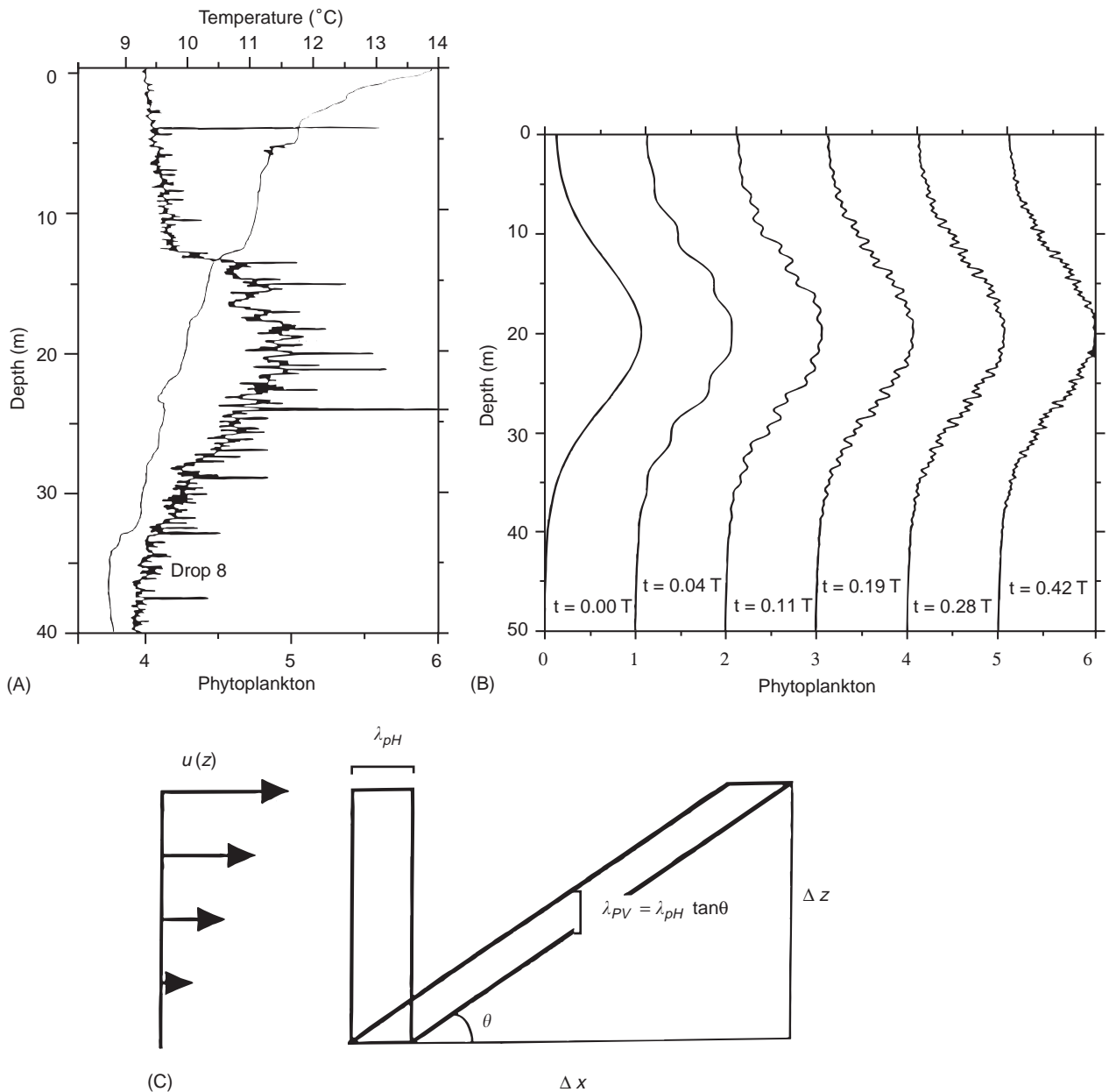
Figure 7 (A) Observations of thin layer structure in a high-resolution profile of fluorescence (thick line, arbitrary units). The thin line shows the corresponding temperature structure. (Data courtesy of Dr T. Cowles.) (B) Simulated vertical profiles of phytoplankton concentration (arbitrary units) at six sequential times. Each profile is offset from the previous by 1 phytoplankton unit. The times are given as fractions of the period of the near-inertial wave used to drive the model. (C) A schematic diagram of the layering process. Vertical shear stretches a vertical column of a property horizontally through an angle \theta , creating a layer in the vertical profile. (Reproduced with permission from Franks PJS (1995) Thin layers of phytoplankton: a model of formation by near-inertial wave shear. Deep-Sea Research 42: 75–91.)
