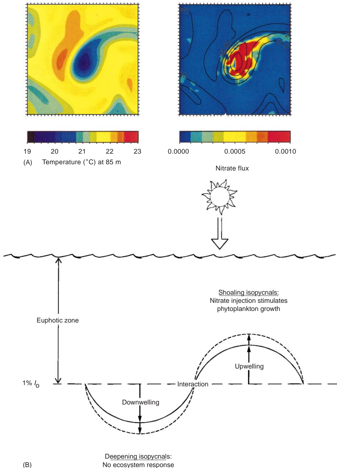
Figure 10 (A) A simulated eddy-driven nutrient injection event: snapshots of temperature at 85 m (left column, °C) and nitrate flux across the base of the euphotic zone (right column, moles of nitrogen \text{m}^{-2} \text{d}^{-1} ). For convenience, temperature contours from the left-hand panels are overlaid on the nutrient flux distributions. The area shown here is a 500 km on a side domain. (The simulation is described in McGillicuddy DJ and Robinson AR (1997) Eddy induced nutrient supply and new production in the Sargasso Sea. Deep-Sea Research I 44(8): 1427–1450.) (B) A schematic representation of the eddy upwelling mechanism. The solid line depicts the vertical deflection of an individual isopycnal caused by the presence of two adjacent eddies of opposite sign. The dashed line indicates how the isopycnal might be subsequently perturbed by interaction of the two eddies. (Reproduced with permission from McGillicuddy DJ et al. (1998) Influence of mesoscale eddies on new production in the Sargasso Sea. Nature 394: 263–265).
