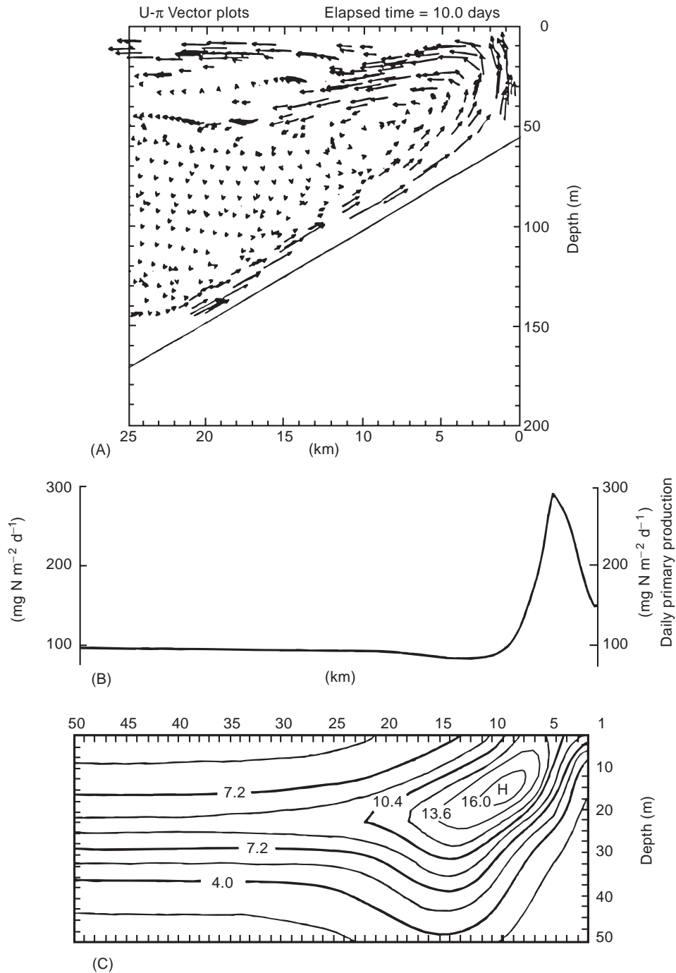
Figure 11 Snapshot from a two-dimensional coupled model of coastal upwelling. (A) Circulation in the transverse plane normal to the coast (maximum horizontal and vertical velocities are -6.1 and 0.05 \text{ cm s}^{-1} , respectively); (B) daily gross primary production; (C) phytoplankton distribution (contour interval is 1.6 \mu\text{g} at \text{NI}^{-1} ). (Adapted with permission from Wroblewski JS (1977) A model of plume formation during variable Oregon upwelling. Journal of Marine Research 35(2): 357-394.)
