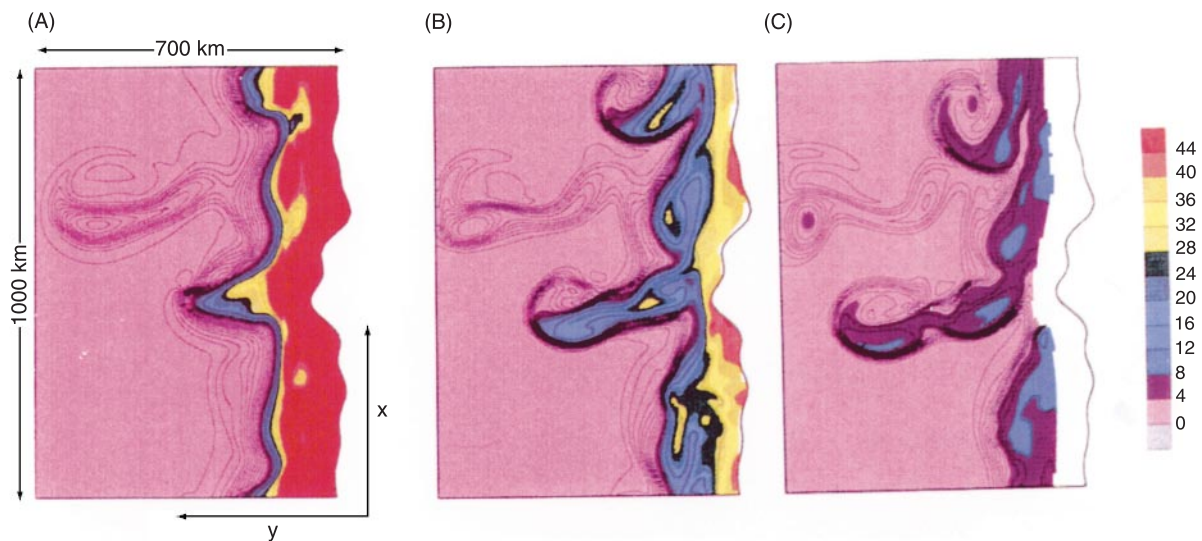
Figure 12 Modeled distributions of phytoplankton (color shading, \text{mg nitrogen m}^{-3} ) in the Coastal Transition Zone off California. Instantaneous snapshots in panels (A–C) are separated by time intervals of 10 days. Contour lines indicate the depth of the euphotic zone, defined as the depth at which photosynthetically available radiation is 1% of its value at the surface. Contours range from 30 to 180 m, 40 to 180 m, and 60 to 180 m in panels (A), (B), and (C) respectively. (Reproduced with permission from Moisan et al. (1996) Modeling nutrient and plankton processes in the California coastal transition zone 2. A three-dimensional physical-bio-optical model. Journal of Geophysical Research 101(C10): 22677–22691.
