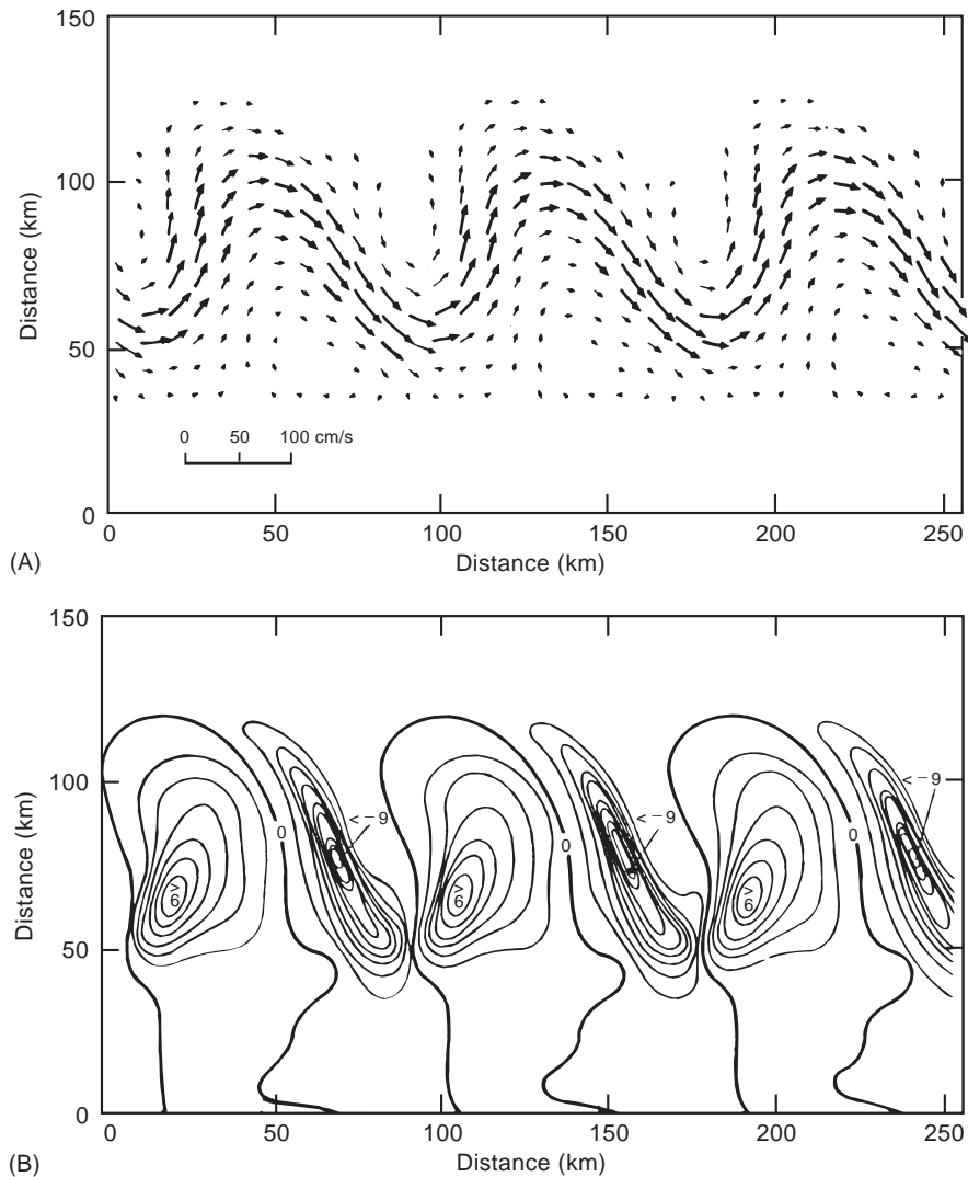
Figure 8 Simulation of a meandering mesoscale jet: (A) velocity on an isopycnal surface with a mean depth of 20 m; (B) vertical velocity ( \text{m d}^{-1} ) on the same isopycnal surface as in (A). Note the consistent pattern of the vertical motion with respect to the structure of the jet. (Reproduced with permission from Woods JD (1988) Mesoscale upwelling and primary production. In: Rothschild BJ (ed) Toward a Theory on Physical-Biological Interactions in the World Ocean . London: Kluwer Academic.)
