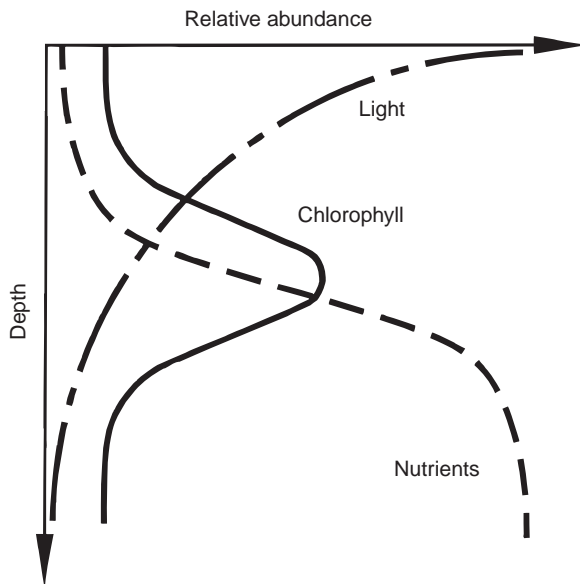
Figure 4 Schematic representation of the deep chlorophyll maximum in relation to ambient light and nutrient profiles in the euphotic zone (typically 10s to 100s of meters in vertical extent).
