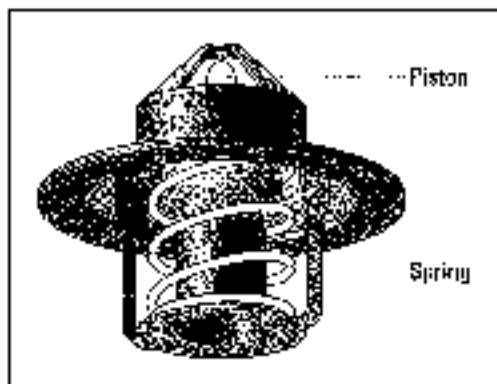
Figure 8-1 A thermostat.
