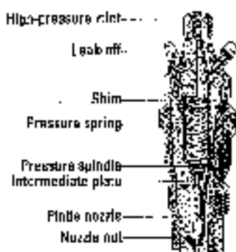
Figure 7-4: Anatomy of a fuel injector.
