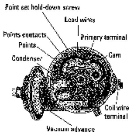
Figure 12-15: The anatomy of a non- electronic distributor.
