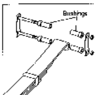
Figure 16-8: Leaf springs have rubber bushings to cushion them.
