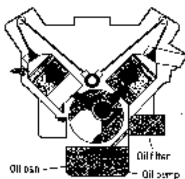
Figure 4-10: The lubrication system.
