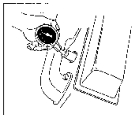
Figure 13-19: Checking compression.
