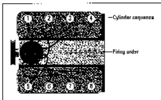
Figure 12-5: The cylinder sequence and firing order of a Ford V-8 engine.
