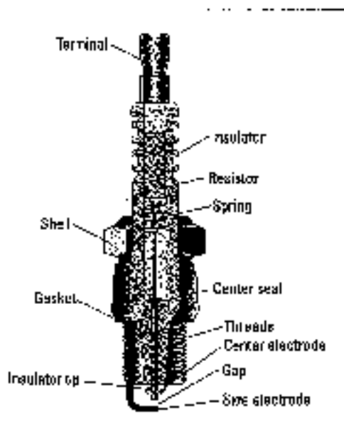
Figure 5-12: Anatomy of a spark plug.
