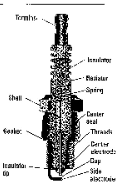
Figure 12-10: The anatomy of a spark plug.
