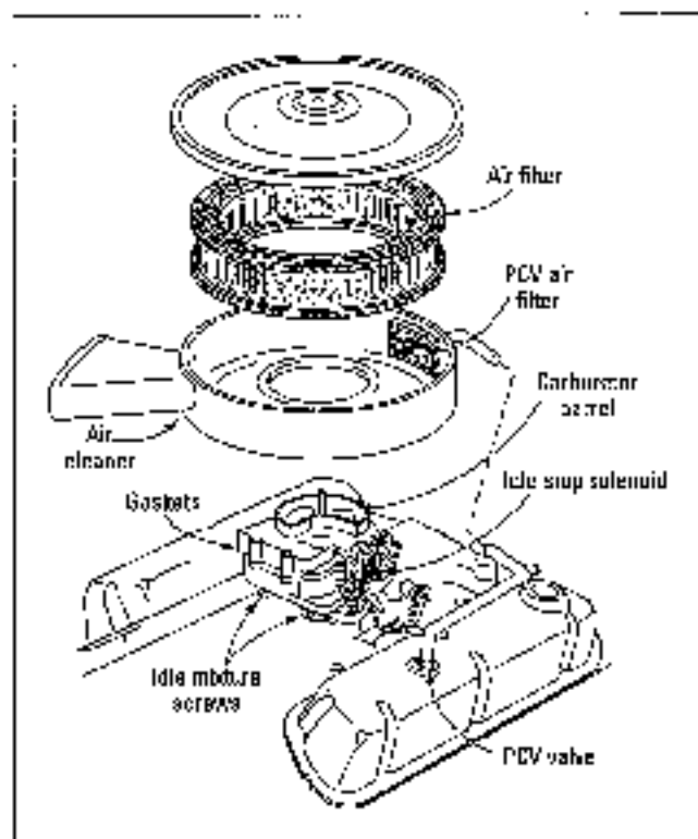
Figure 6-3: The carburetor.
