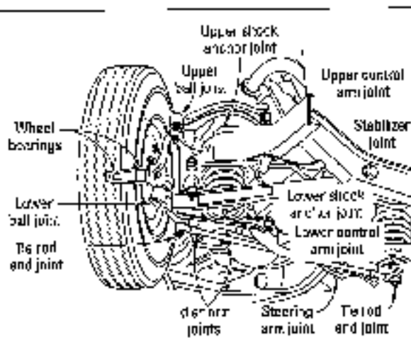
Figure 16-4: Some of the places to look for grease fittings on your car.
