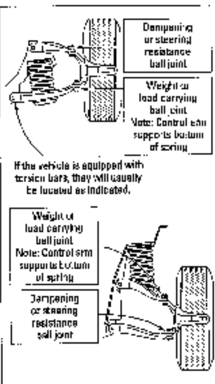
Figure 16-7: Bushings and ball joints on front coil springs. Front coil springs can sit on either the upper or the lower control arms. They are cushioned by ball joints.
