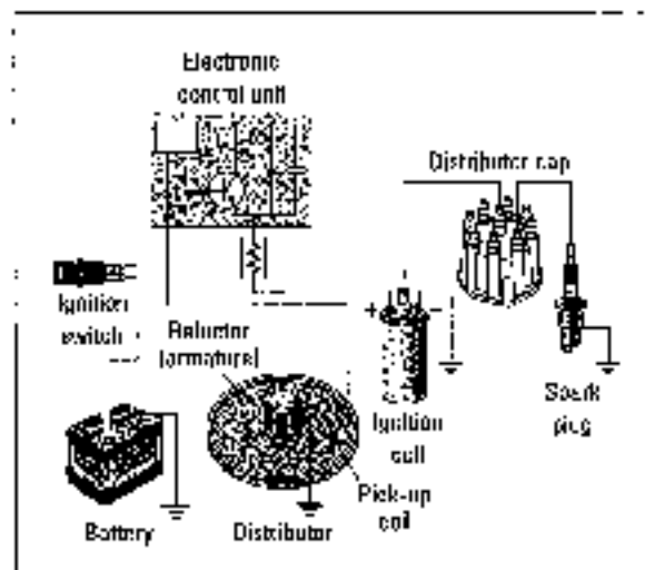
Figure 5-9: An electronic ignition system.
