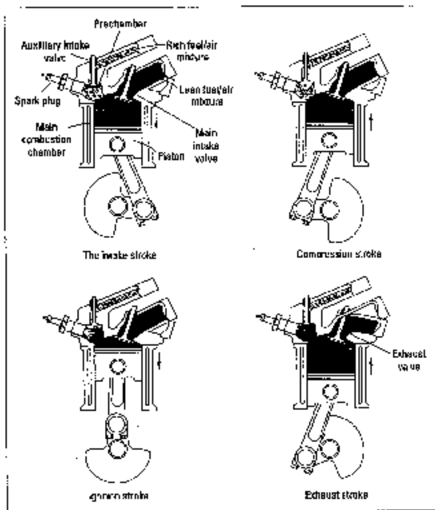
Figure 6-10: The four- stroke power cycle in a stratified charge engine.
