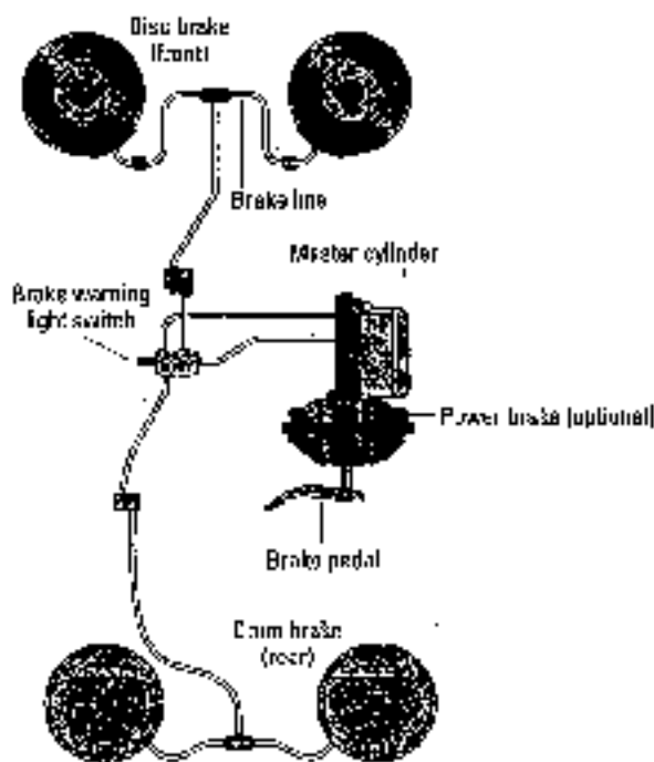
Figure 10-4: The brake system
