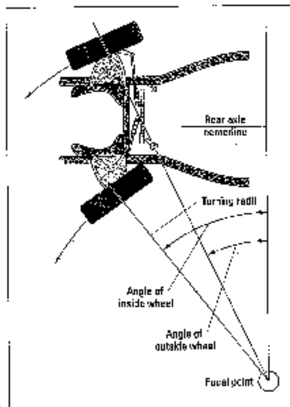
Figure 19-7: Turning radius.
