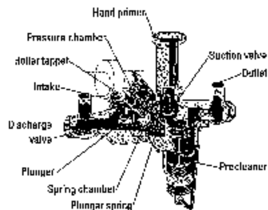
Figure 7-6: Fuel transfer pump.
