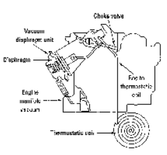
Figure 13-17: This thermostatic coil choke.
