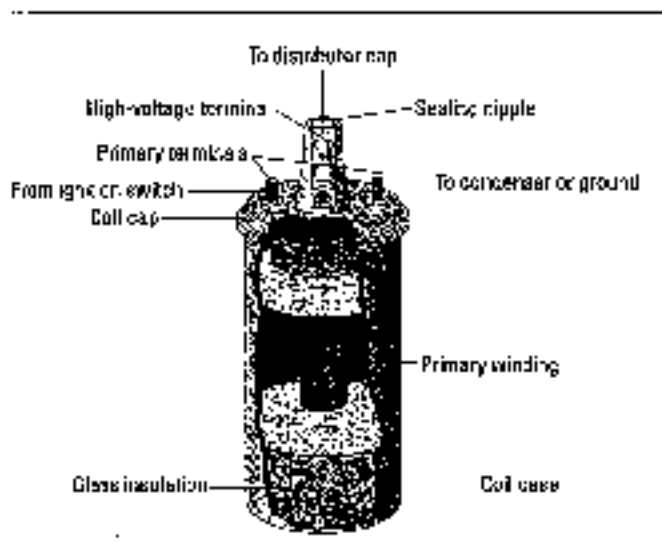
Figure 5-11: The anatomy of a coil.
