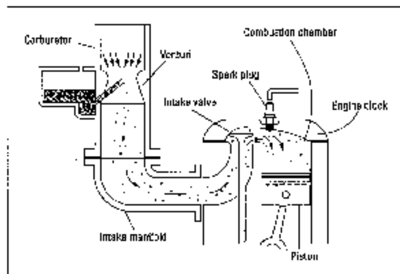
Figure 6-8: The path the fuel/air mix- ture takes to the engine.
