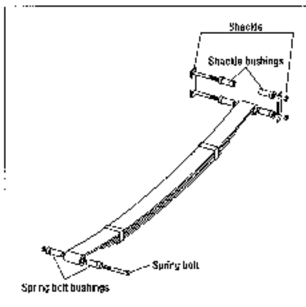
Figure 11-6 Leaf springs bend but do not break because they can slide flexibly on one another.
