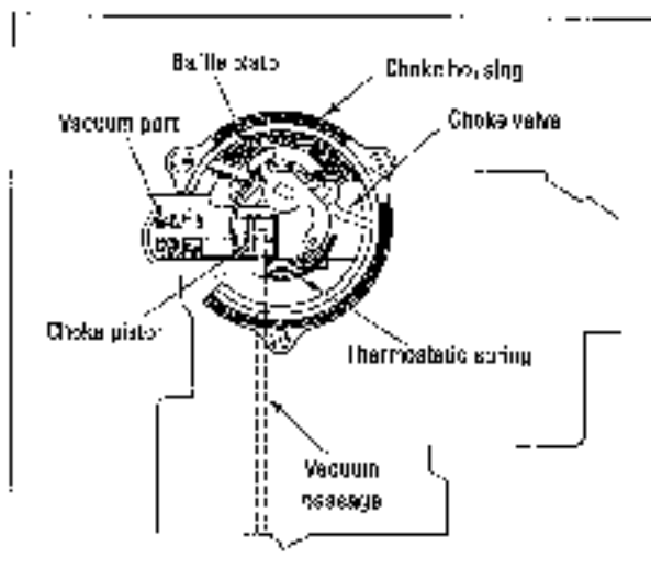
Figure 13-16 Thermostatic spring choke.
