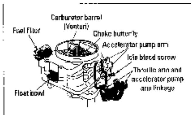
Figure 13-8: A typical carburetor.
