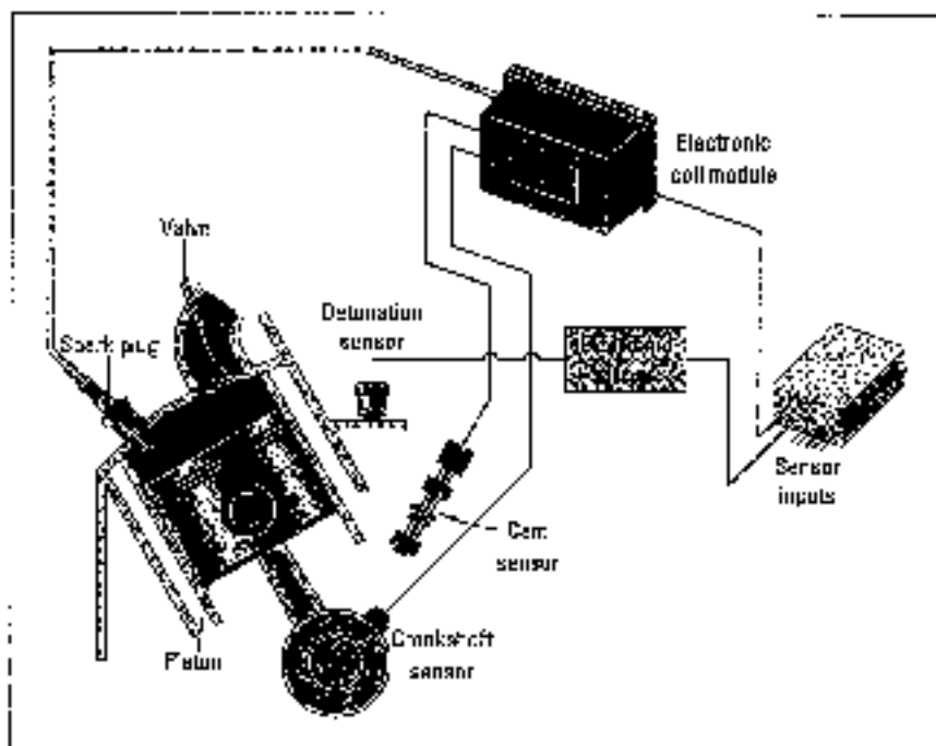
Figure 5-16: A distributorless electronic ignition system.
