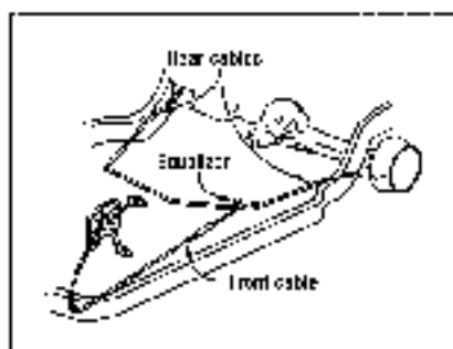
Figure 10-9: An integral parking brake system.
