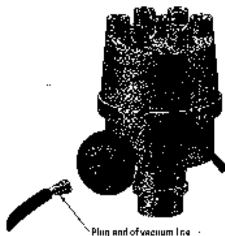
Figure 12-50: Dis- connecting the vacuum advance.
