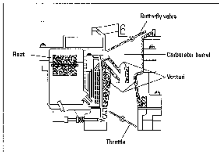
Figure 6-5: The carburetor.
