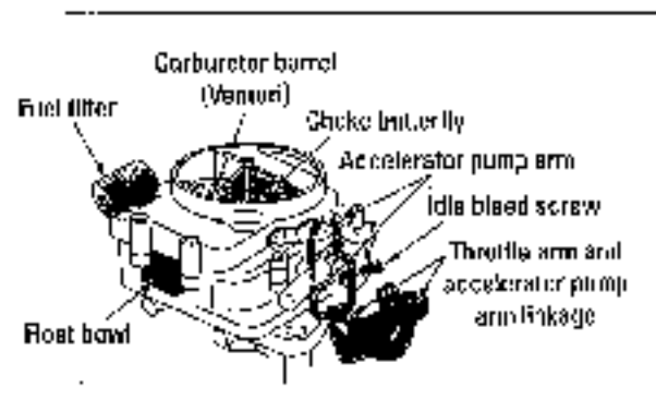
Figure 21-1: A typical carburetor.
