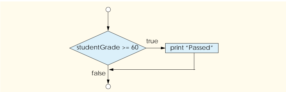
Fig. 4.3 Flowcharting a single-selection if structure.
