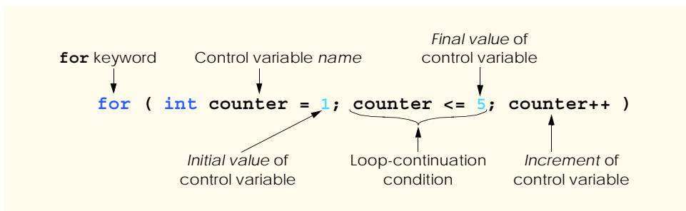
Fig. 5.3 Components of a typical for header.
