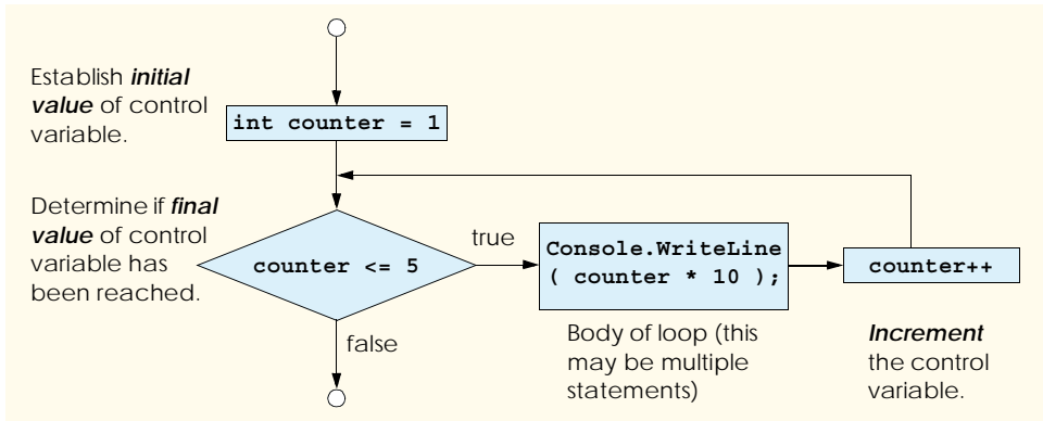
Fig. 5.4 Flowcharting a typical for repetition structure.
