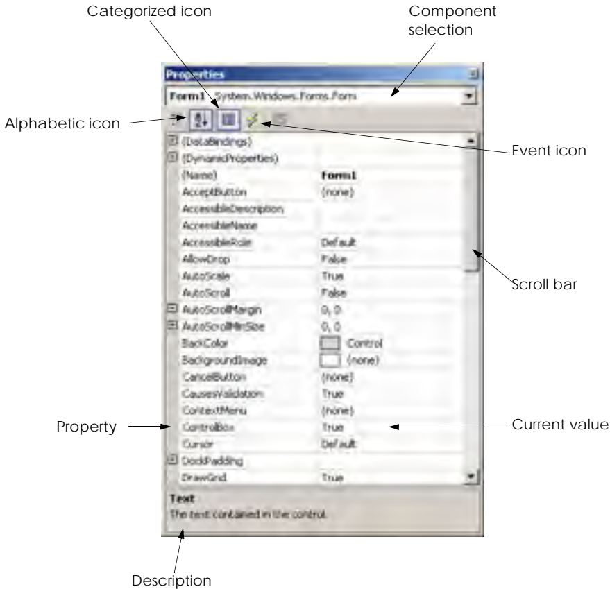
Fig. 2.12 Properties window.
