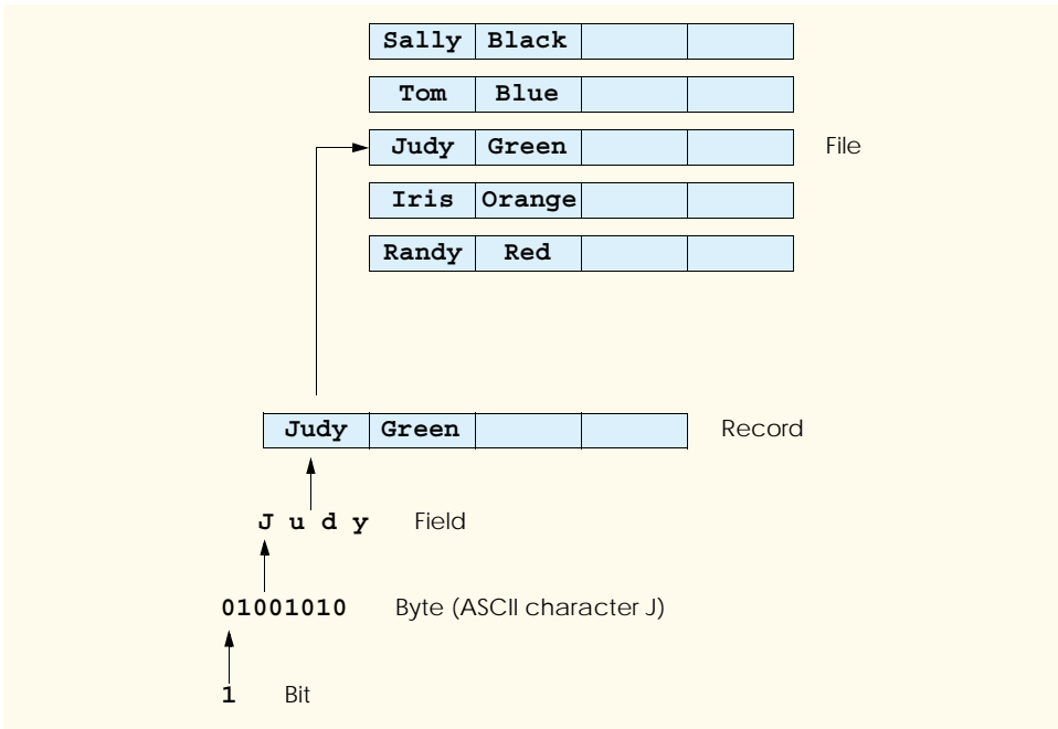
Fig. 17.1 Data hierarchy.
