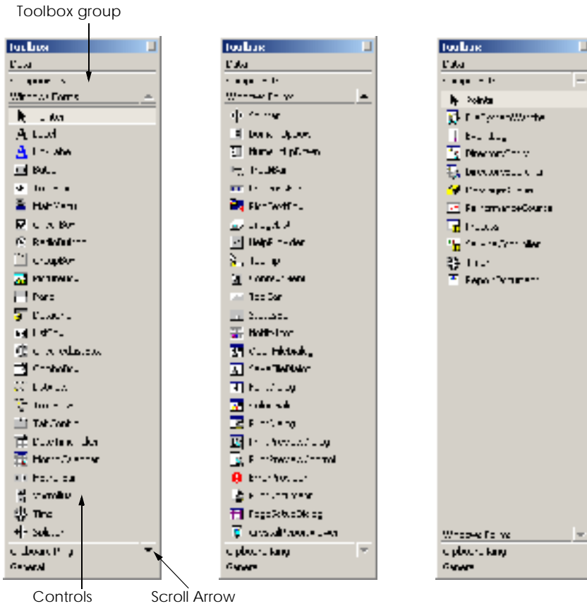
Fig. 2.10 Toolbox window.
