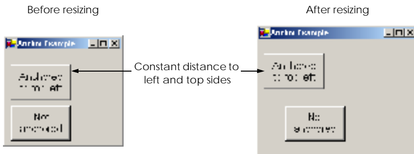
Fig. 12.11 Anchoring demonstration.
