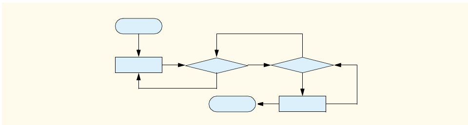
Fig. 5.28 Unstructured flowchart.
