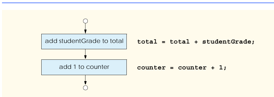
Fig. 4.1 Flowcharting C#'s sequence structure.
