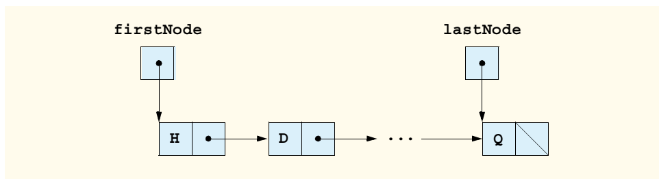
Fig. 23.3 A graphical representation of a linked list.
