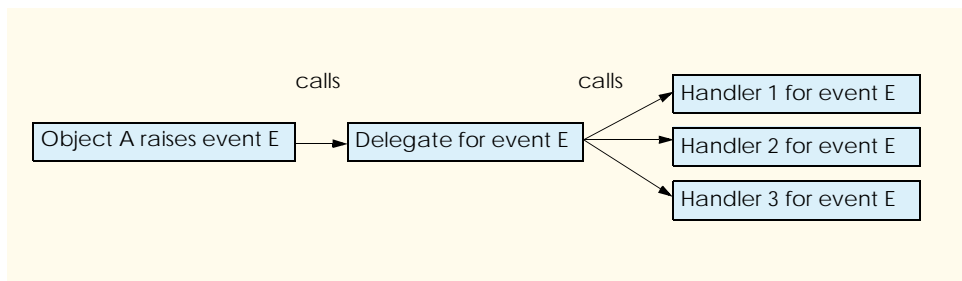
Fig. 12.5 Event-handling model using delegates.
