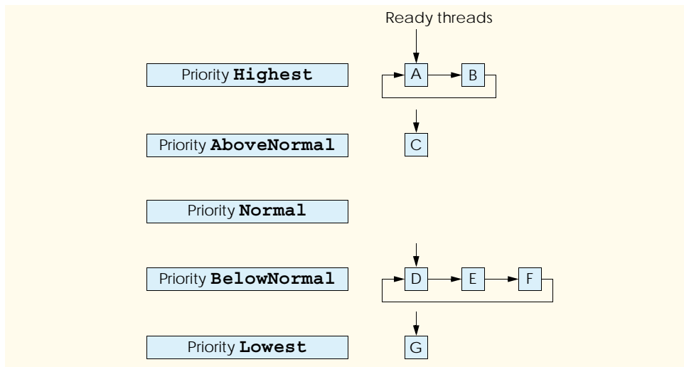
Fig. 14.2 Thread-priority scheduling.
