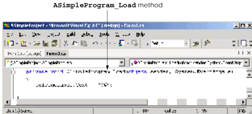
Fig. 4.23 Method FrmASimpleProgram_Load .
