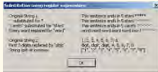
Fig. 15.23 Regex methods Replace and Split . (Part 2 of 2.)
