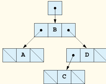
Fig. 23.15 A graphical representation of a binary tree.
