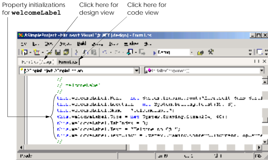
Fig. 4.18 Code generated by the IDE for welcomeLabel .
