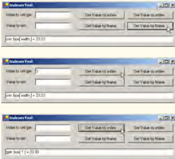
Fig. 8.16 Indexers provide subscripted access to an object's members. (Part 6 of 6.)
