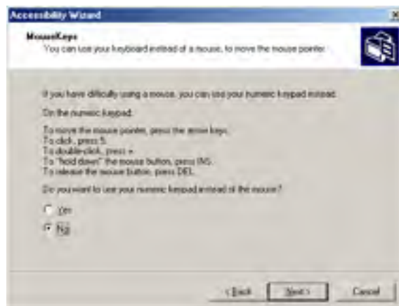
Fig. 24.34 MouseKeys window.
