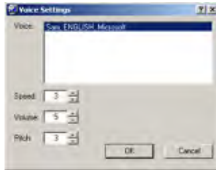
Fig. 24.40 Voice-settings window.
