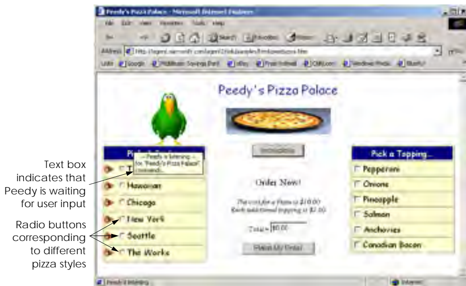
Fig. 16.32 Peedy waiting for speech input.
