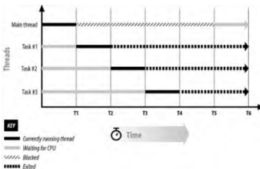
Figure 9-1. A simple thread-state diagram
