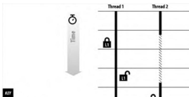
Figure 3-1. Acquiring and releasing a lock
