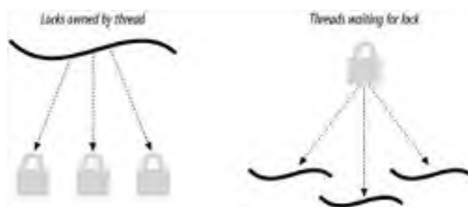
Figure 6-1. Lock trees
