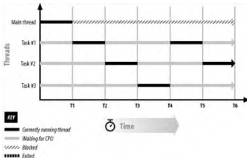
Figure 9-2. Thread states with OS scheduling
