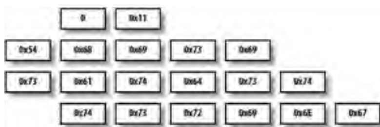
Figure 12-2. Byte representation of a UTF-encoded string
