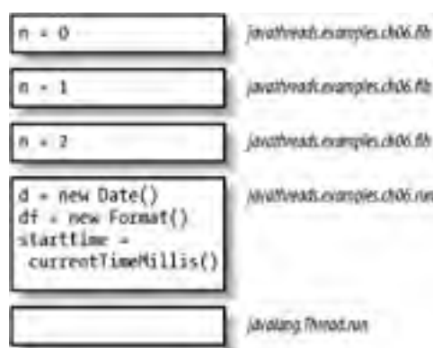
Figure 13-4. A Java thread's stack
