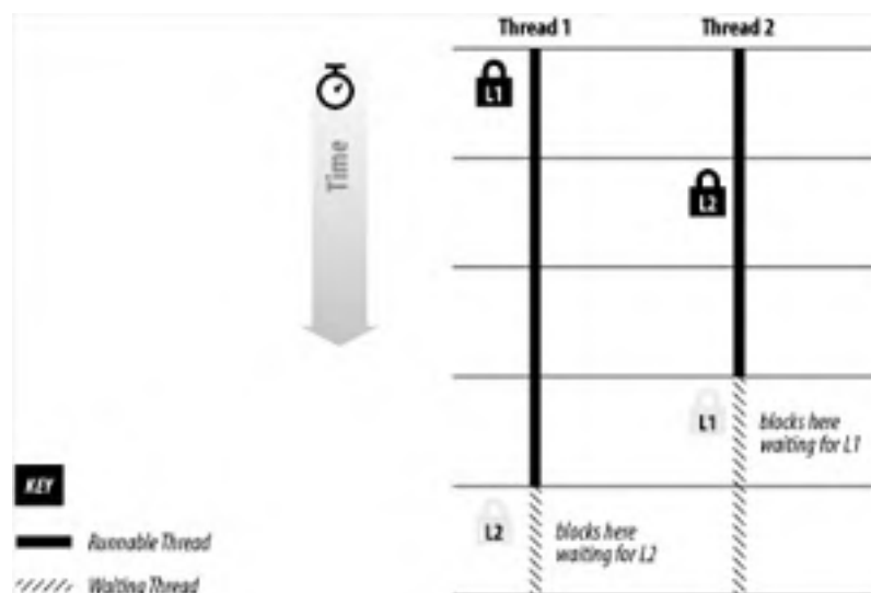
Figure 3-2. Deadlock in the ScoreLabel class
