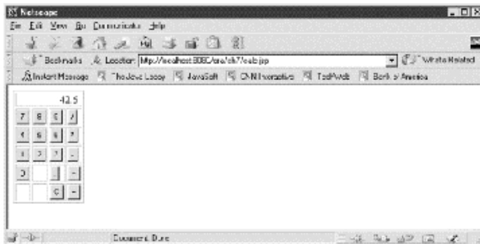
Figure 7.4. Calculator page
