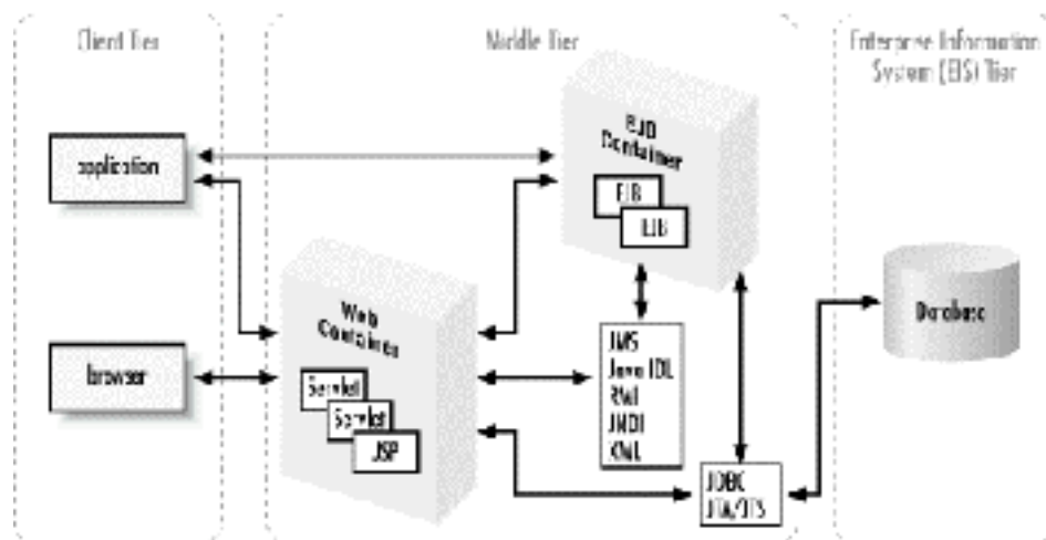
Figure 13.1. J2EE overview
