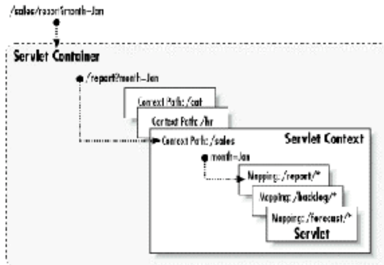
Figure 2.6. Request dispatching
