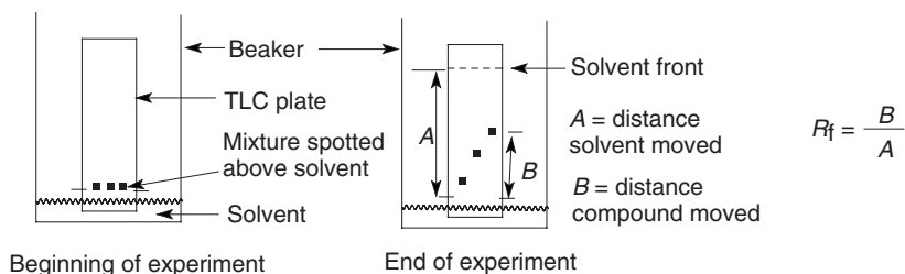
Fig. 10-1. TLC experiment.
