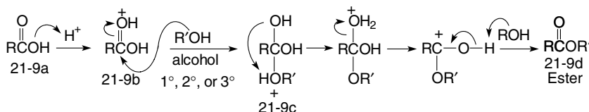
Fig. 21-9. Synthesis of esters.
