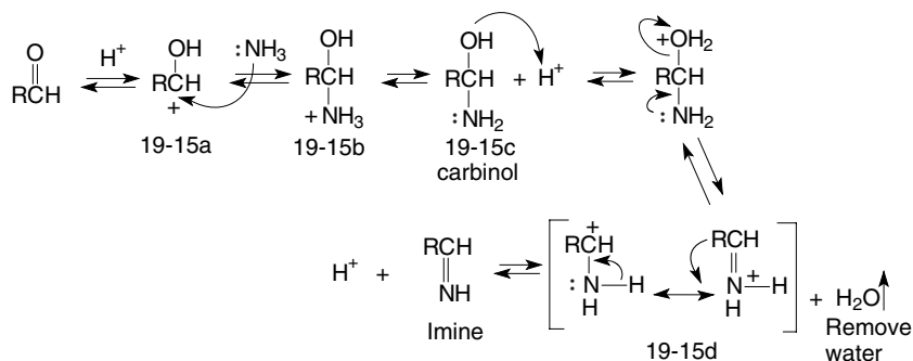
Fig. 19-15. Imine formation.
