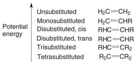
Fig. 6-5. Relative stability of substituted alkenes.
