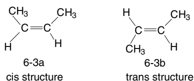
Fig. 6-3. Cis and trans structures.
