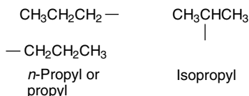
Fig. 4-7. Propyl and isopropyl groups.
