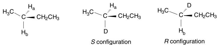
Fig. 5-23. Prochiral atoms.
