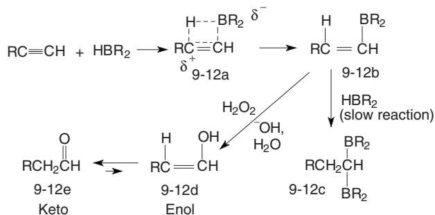
Fig. 9-12. Hydroboration-oxidation of an alkyne.
