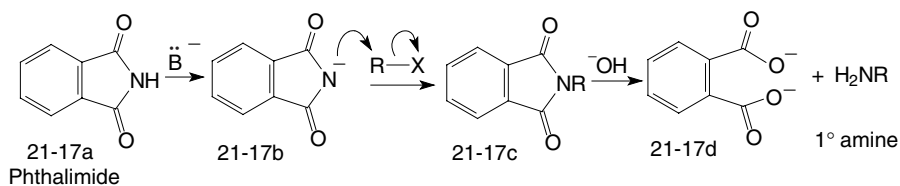
Fig. 21-17. Gabriel amine synthesis.
