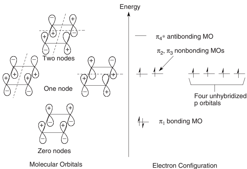
Fig. 17-9. Molecular orbital description of 1,3-cyclobutadiene.
