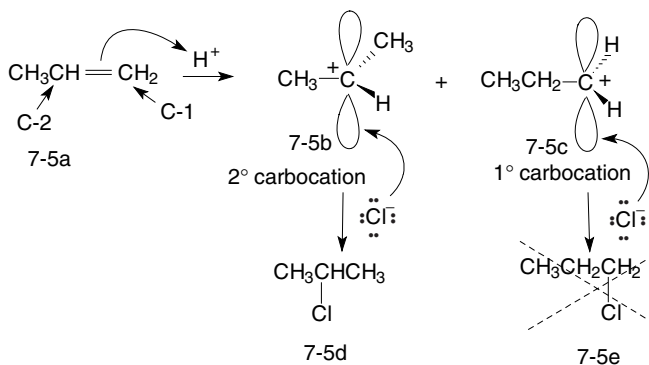
Fig. 7-5. Addition of HCl to propylene.
