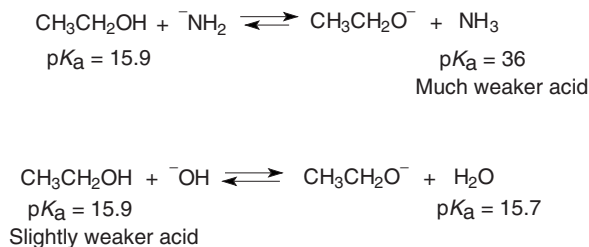
Fig. 13-3. Acid-base reactions of alcohols.
