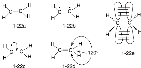
Fig. 1-22. Structure of ethylene (ethene).
