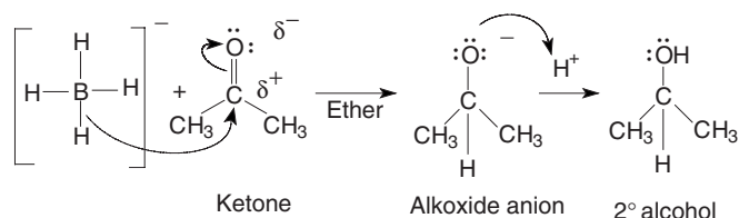
Fig. 13-6. Reduction of the carbonyl function.
