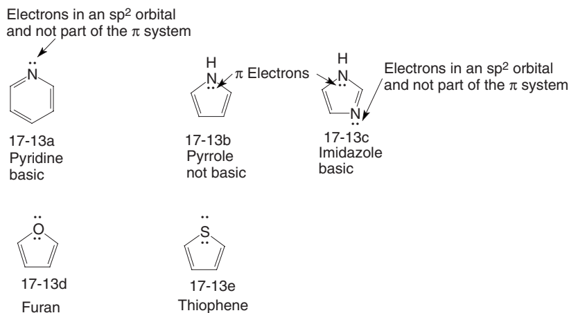
Fig. 17-13. Aromatic heterocycles.
