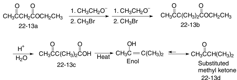
Fig. 22-13. Acetoacetic ester synthesis.
