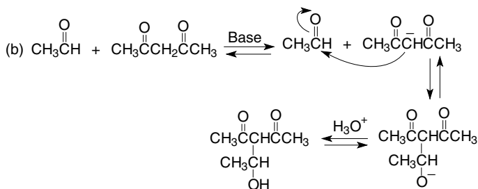
Fig. 23-3. Mixed aldol reaction.
