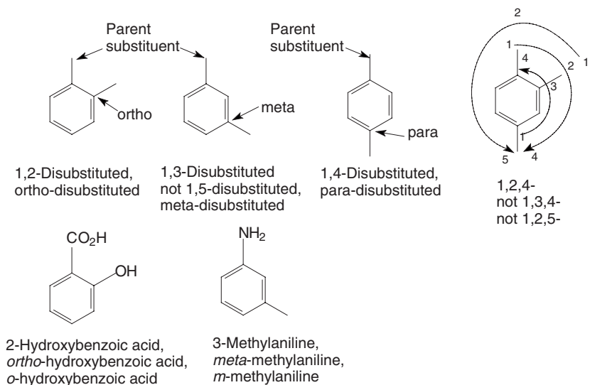
Fig. 17-2. Disubstituted benzenes.
