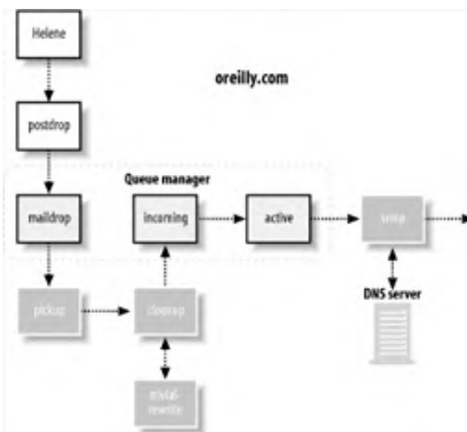
Figure 3-4. Tracing message delivery 1
