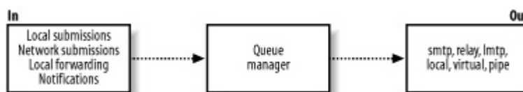
Figure 3-1. Broad view of the Postfix architecture
