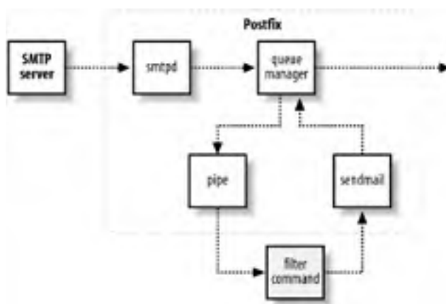
Figure 14-1. Mail-filtering command
