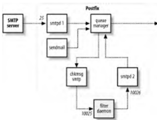
Figure 14-2. Mail-filtering daemon
