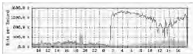
Figure 22-1. Vineyard.NET MRTG monitor
