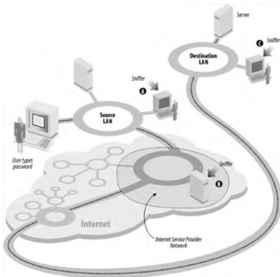
Figure 19-2. Password sniffing
