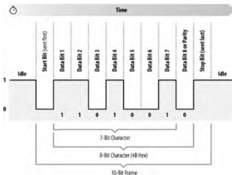
Figure 10-1. A serial interface sending the letter K (ASCII 75)
