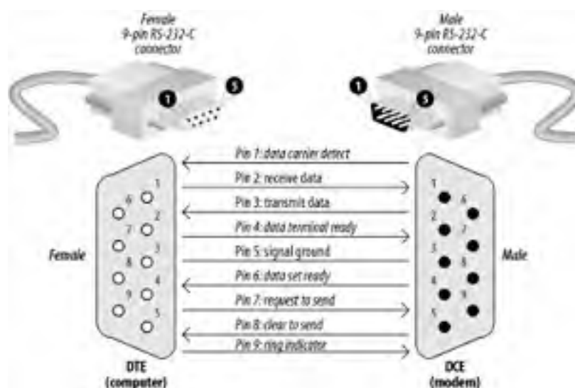
Figure 10-3. The standard 9-pin RS-232-C connector
