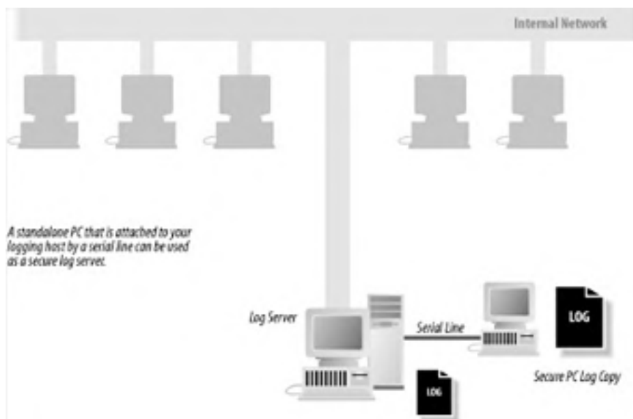
Figure 21-1. Secure logging host
