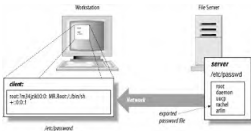
Figure 14-1. How NIS works
