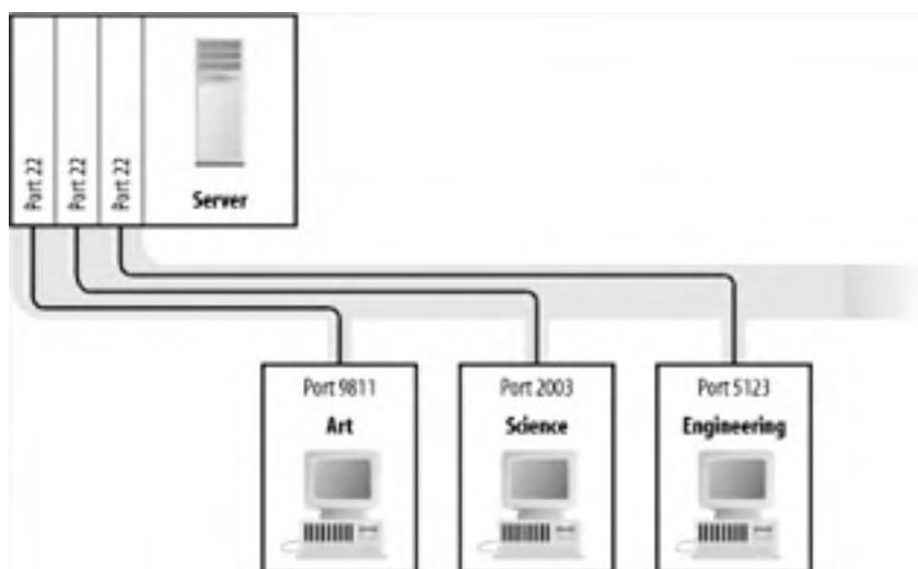
Figure 11-6. A few Internet connections with port numbers
