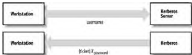
Figure 14-3. Initial Kerberos authentication
