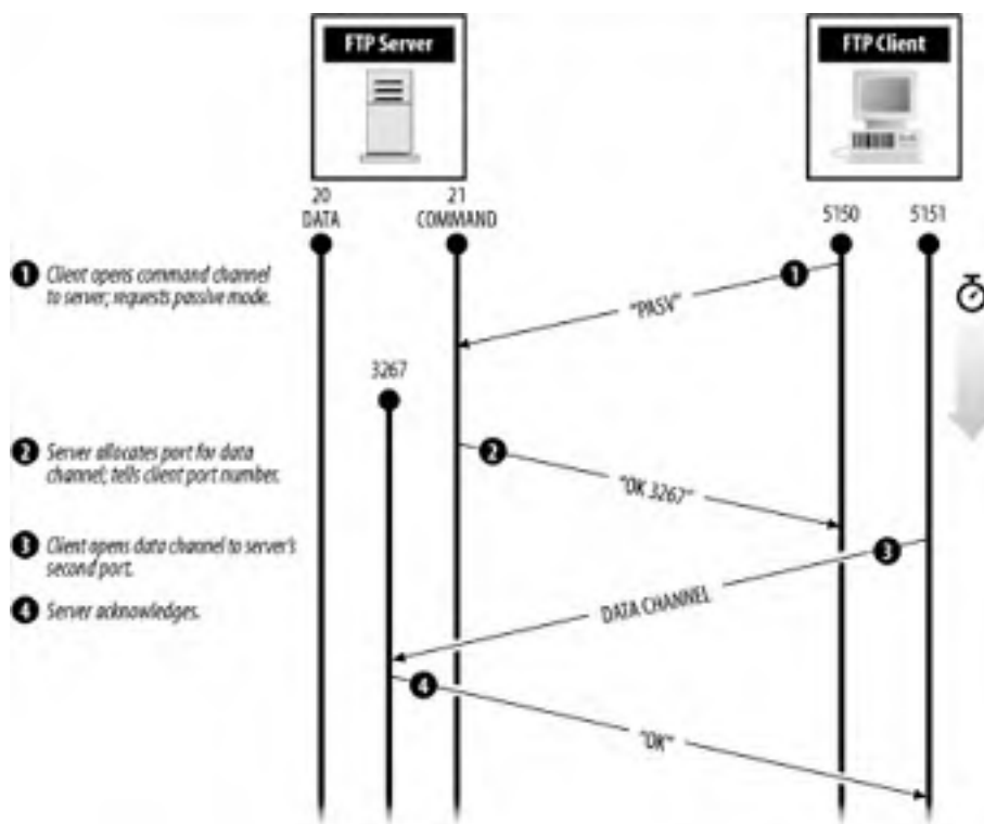
Figure 12-2. Passive-mode FTP connection
