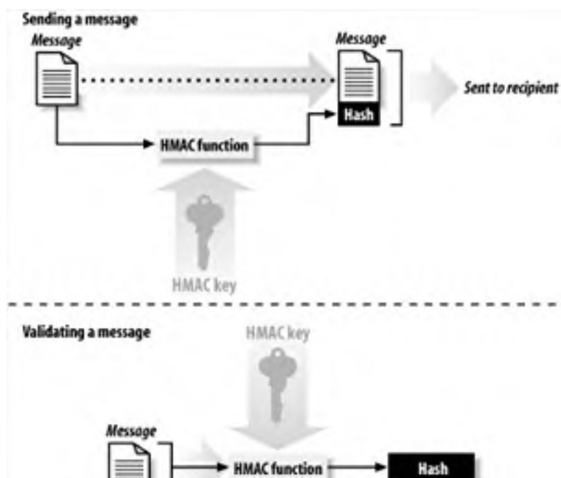
Figure 7-5. Using an HMAC to verify the authenticity and integrity of a message
