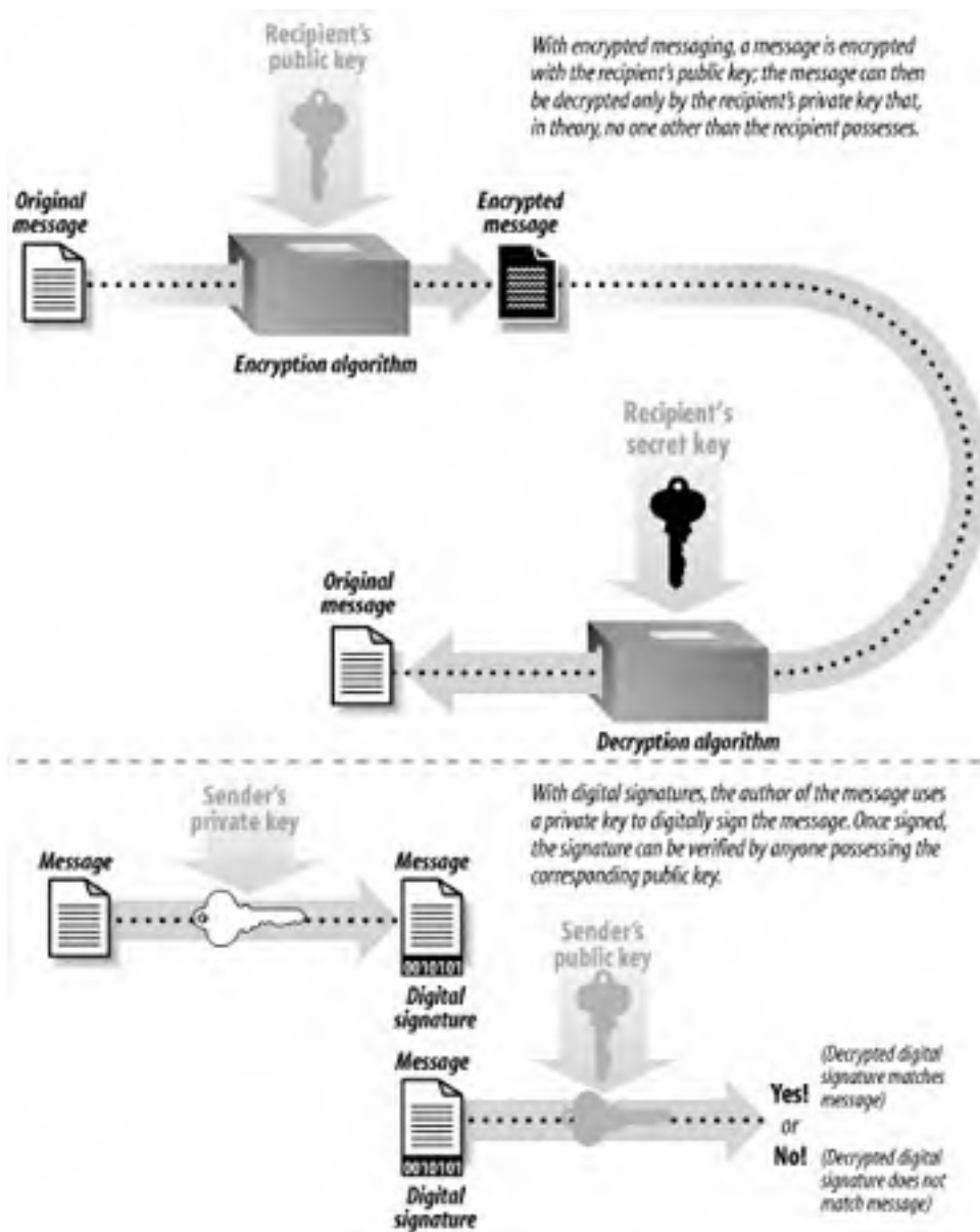
Figure 7-2. Public key cryptography can be used for encrypted messaging or for digital signatures
