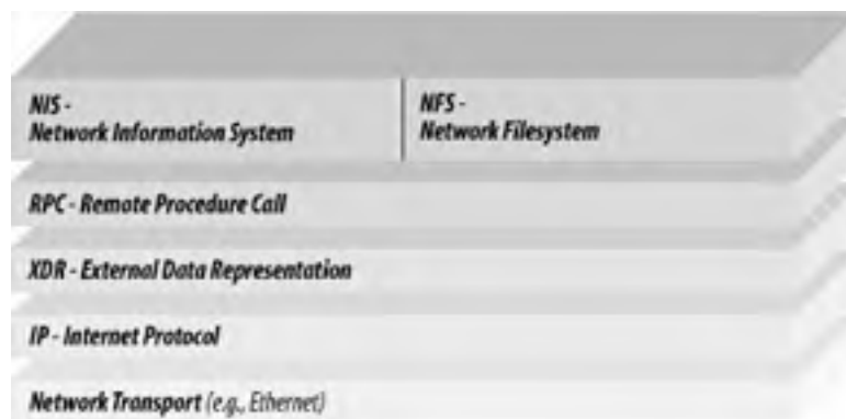
Figure 15-1. NFS protocol stack
