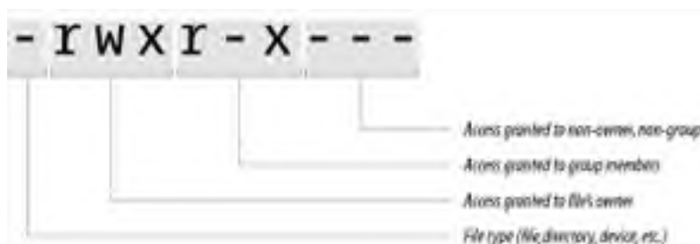
Figure 6-2. Basic permissions
