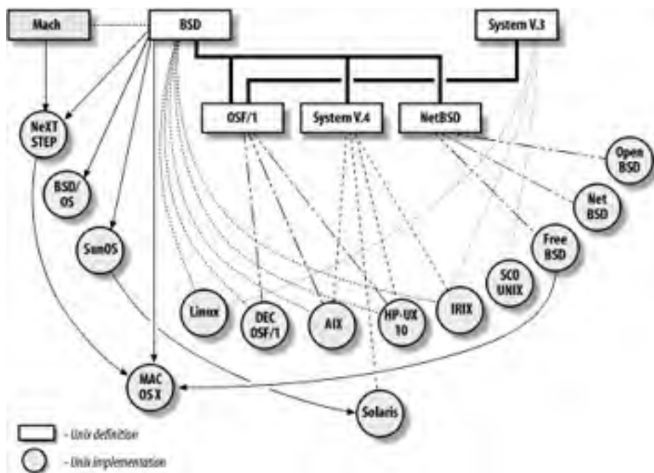
Figure 2-1. Unix variants
