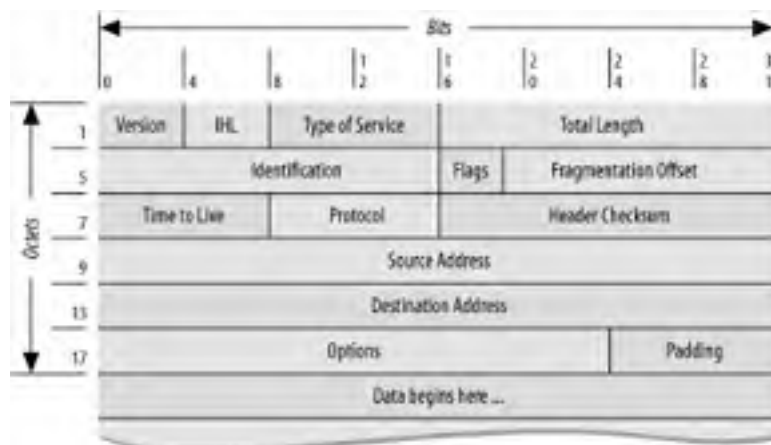
Figure 11-3. IP header and packet
