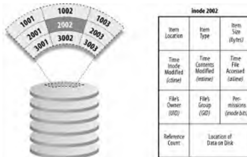
Figure 6-1. Files and inodes
