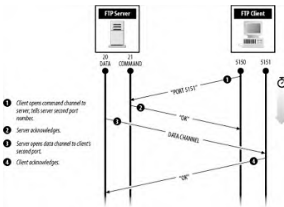
Figure 12-1. Active-mode FTP connection
