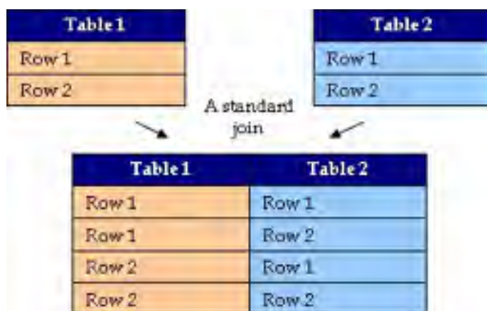
Standard joins take all possible combinations of rows
