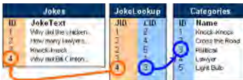
The JokeLookup table associates pairs of rows from the Jokes and Categories tables
